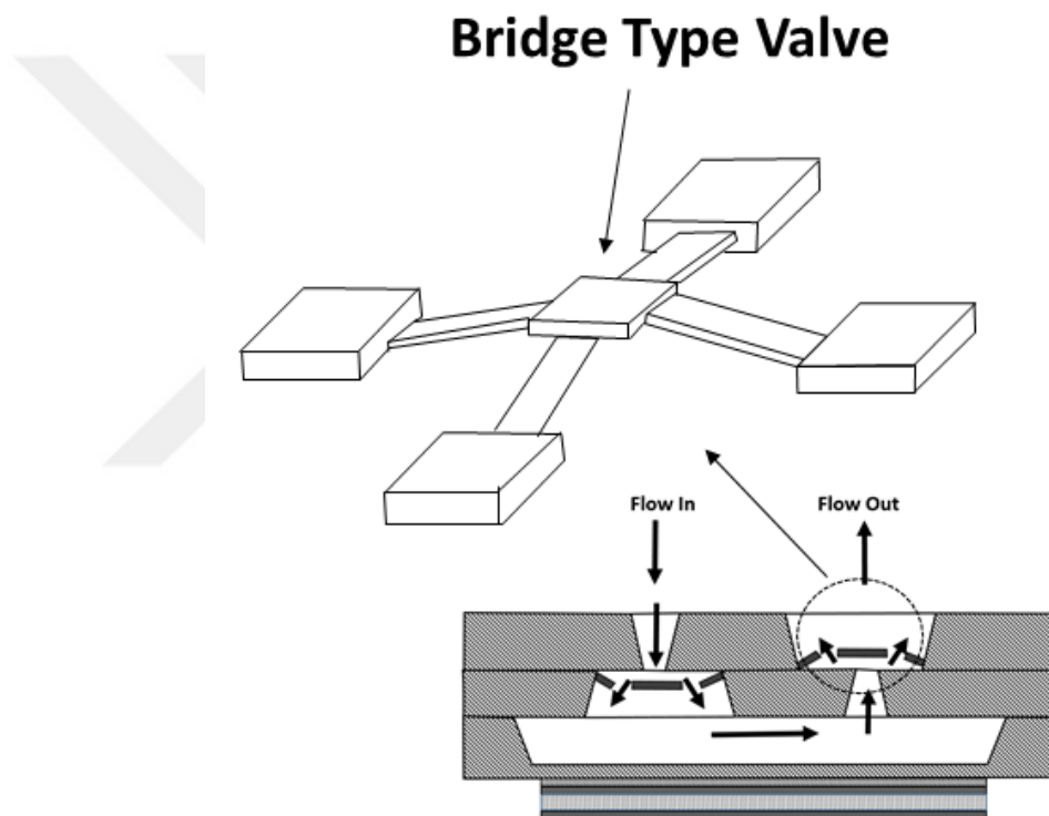
(b) Detailed visualization of the bridge type valve
