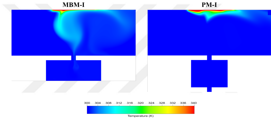
(b) Temperature contours, MBM-I and PM-I
