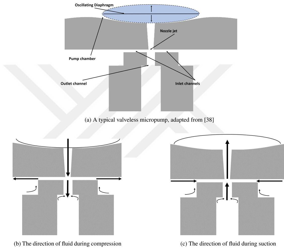
Figure 1.7: The working principle of the VLP: the flow directions, adapted from [38]
