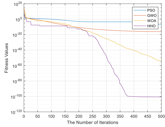
Figure 3.11: Convergence Curve of PSO, GWO, WOA, and HHO for F 2 Function
