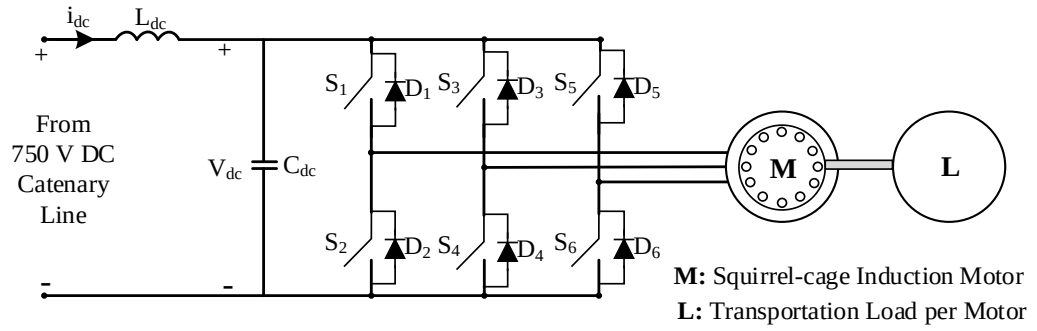
Figure 1.11: Variable Frequency Motor Drive
