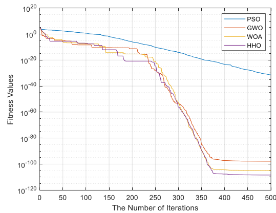
Figure 3.10: Convergence Curve of PSO, GWO, WOA, and HHO for F_1 Function
