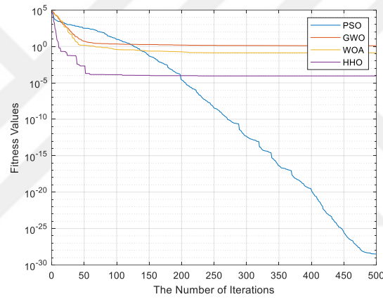
Figure 3.15: Convergence Curve of PSO, GWO, WOA, and HHO for F_6 Function
