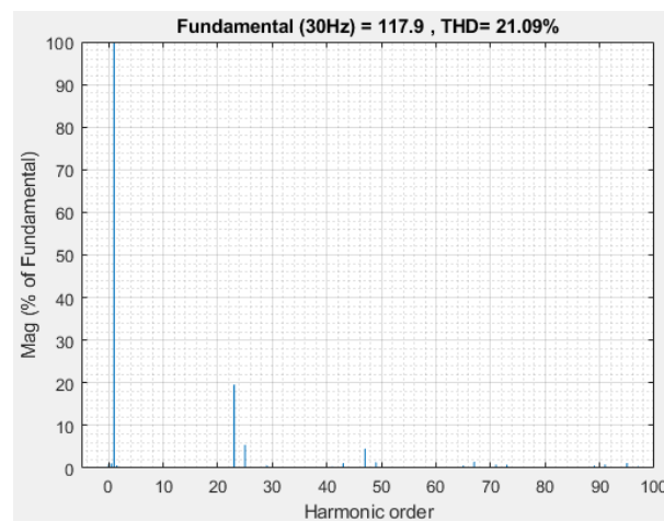
Figure 4.7: Inverter Output Voltage and Current Waveforms Obtained Switching Angles by HHO and Their FFT Distributions at 30 Hz, Full-Load, 565 V DC-Link Voltage
