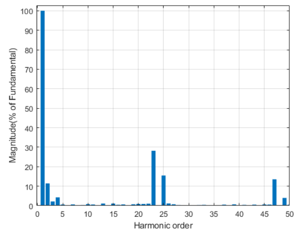
Figure 6.6: Inverter Output Voltage and Current Waveforms Obtained Switching Angles by HHO and Their FFT Distributions at 30 Hz, Full-Load at Point B, 565 V DC-Link Voltage
