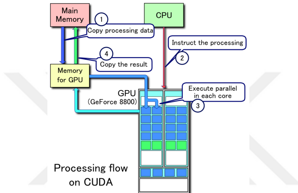
Figure 5.5: The flowchart of GPU programming
