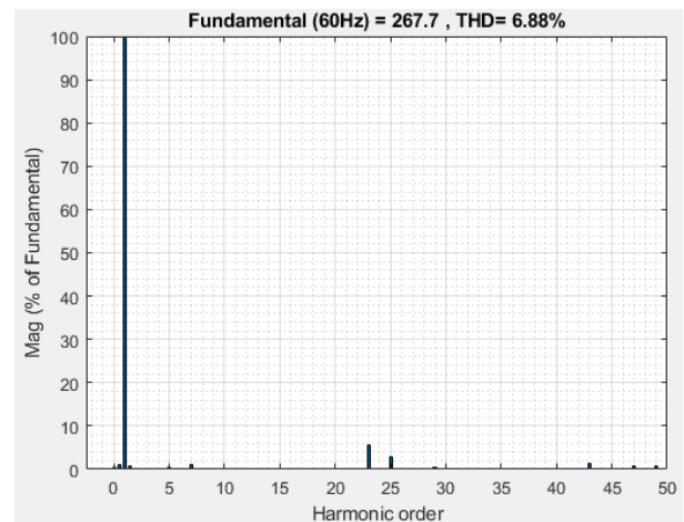
Figure 4.3: Inverter Output Voltage and Current Waveforms Obtained Switching Angles by GWO and Their FFT Distributions at 60 Hz, Full-Load, 750 V DC-Link Voltage
