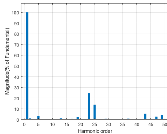
Figure 6.8: Inverter Output Voltage and Current Waveforms Obtained Switching Angles by HHO and Their FFT Distributions at 60 Hz, Full-Load at A point, 750 V DC-Link Voltage
