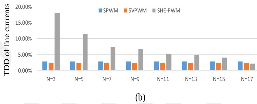
Figure 7.2: Comparison of SPWM, SVPWM and SHEM-PWM in view of TDD variations of motor line currents, (a). At operating point A, f_{sw} = 21f_1 = 1260 Hz for SPWM, SVPWM and f_{sw} = (2N+1)60 Hz for SHEM; (b). At operating point D, f_{sw} = f_c = 3255 Hz for SPWM, SVPWM and f_{sw} = (2N+1)155 Hz for SHEM
