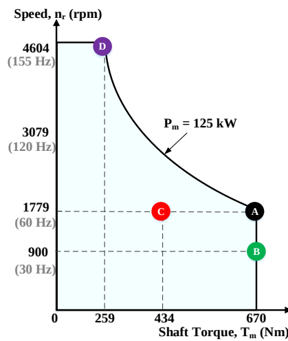
Figure 6.4: Speed Versus Torque Diagram for the Sample Traction Motor
