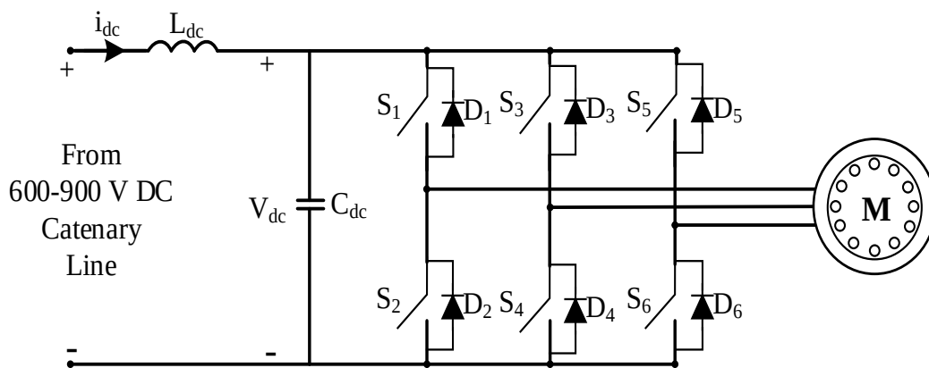
Figure 2.6: Three-phase Two-level Traction Inverter Motor Drive
