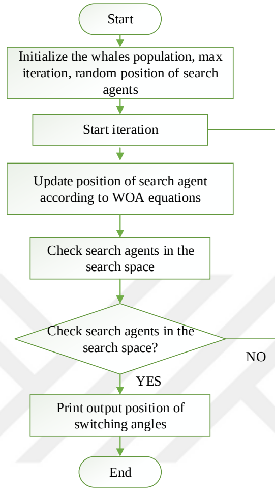
Figure 3.7: General Flowchart of WOA Algorithm.
