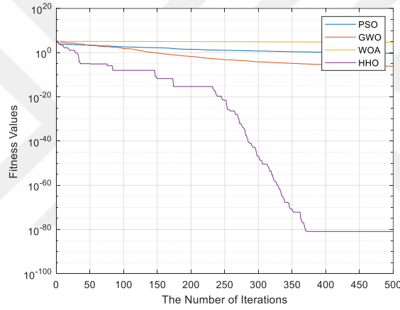
Figure 3.12: Convergence Curve of PSO, GWO, WOA, and HHO for F 3 Function
