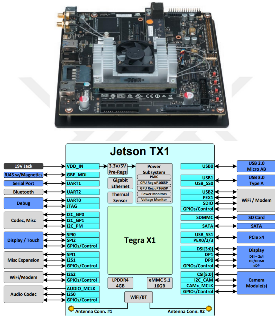
Figure 5.3: Jetson TX1 Block Diagram for general application
