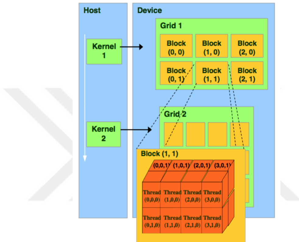
Figure 5.4: CUDA block scalability across different kinds of GPUs
