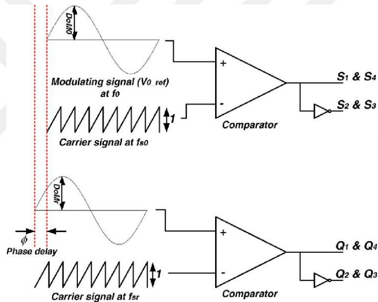
Figure 1.4: Analog Scheme for SPWM Implementation
