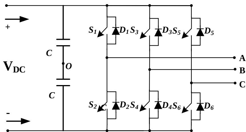
Figure 2.3: Three-Phase Full-Bridge Inverter
