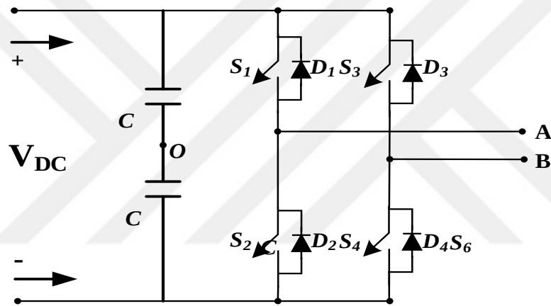
Figure 2.2: Single-Phase Full-Bridge Inverter
