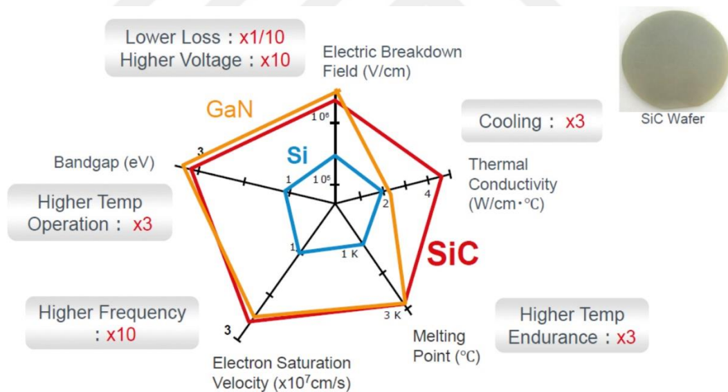
Figure 6.1: Semiconductor Material Comparison of Si, SiC, and GaN
