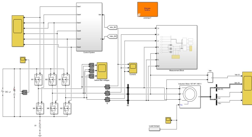
Figure 4.1: MATLAB/Simulink Circuit Diagram of LRT motor drive
