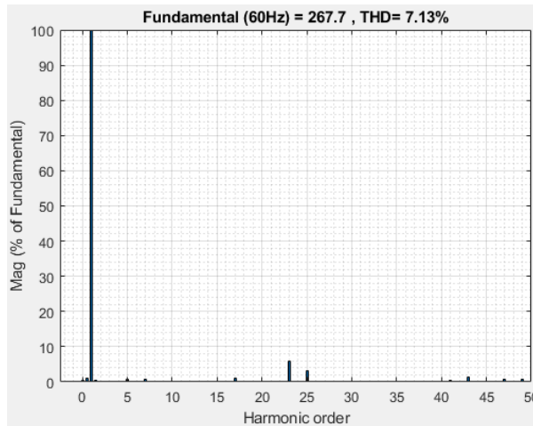
Figure 4.4: Inverter Output Voltage and Current Waveforms Obtained Switching Angles by WOA and Their FFT Distributions at 60 Hz, Full-Load, 750 V DC-Link Voltage
