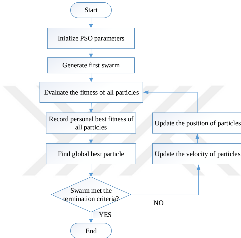
Figure 3.2: Basic Flowchart of PSO
