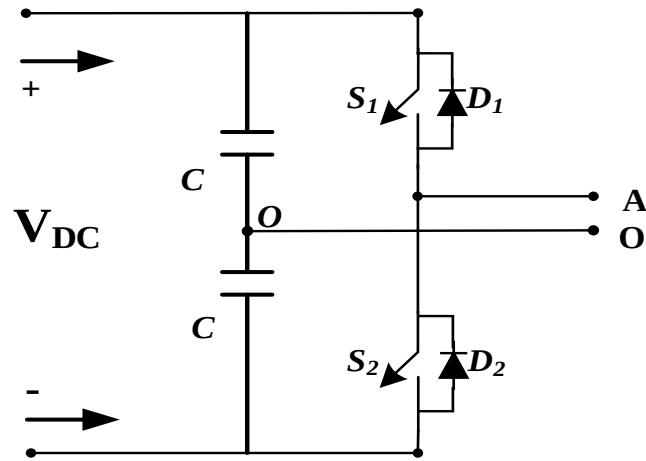
Figure 2 1: Single-Phase Half-Bridge Inverter
