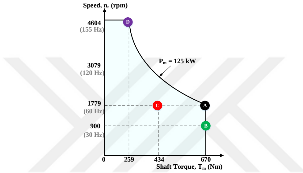
Figure 7.1: Speed Versus Torque Diagram for the Sample Traction Motor
