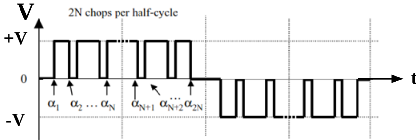
Figure 1.8: Two-level VSI Voltage Waveform Applied to SHE-PWM
