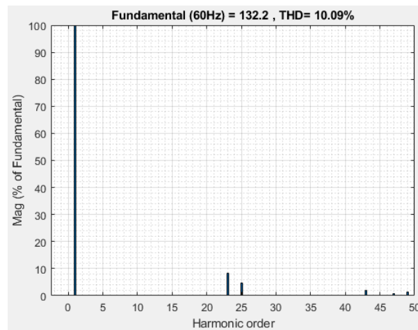
Figure 4.6: Inverter Output Voltage and Current Waveforms Obtained Switching Angles by HHO and Their FFT Distributions at 60 Hz, Half-Load, 565 V DC-Link Voltage
