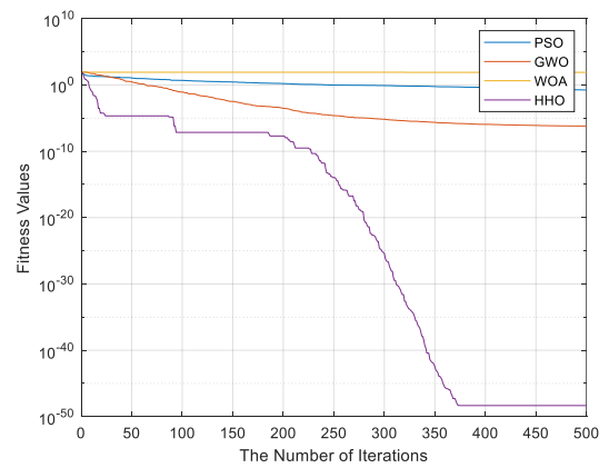
Figure 3.13: Convergence Curve of PSO, GWO, WOA, and HHO for F 4 Function
