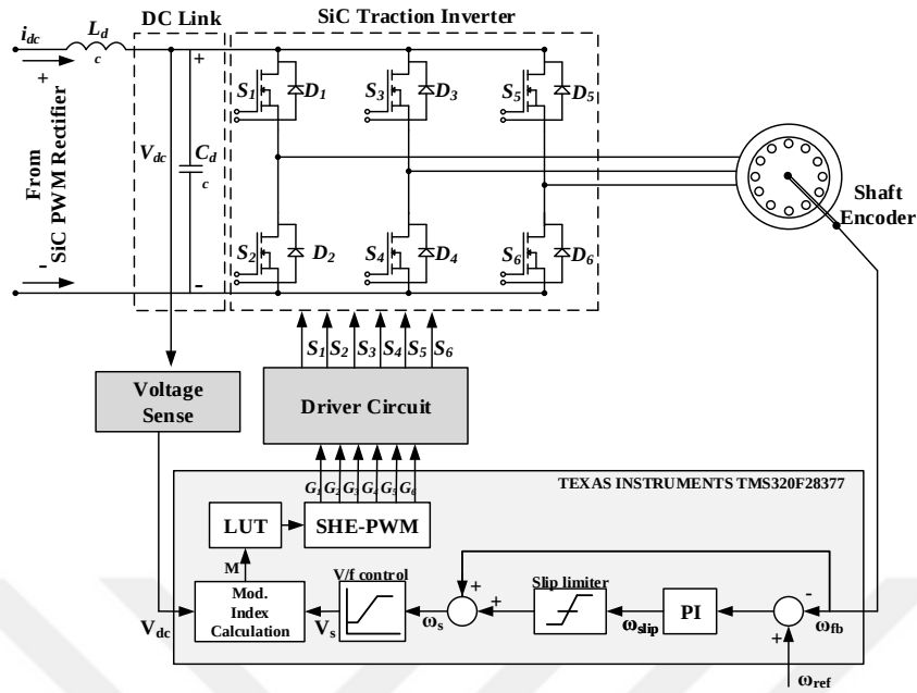
Figure 6.3: Control Scheme of SHE-PWM SiC Traction Inverter
