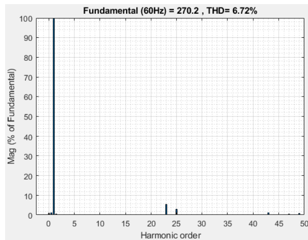
Figure 4.8: Inverter Output Voltage and Current Waveforms Obtained Switching Angles by HHO and Their FFT Distributions at 60 Hz, Full-Load, 750 V DC-Link Voltage
