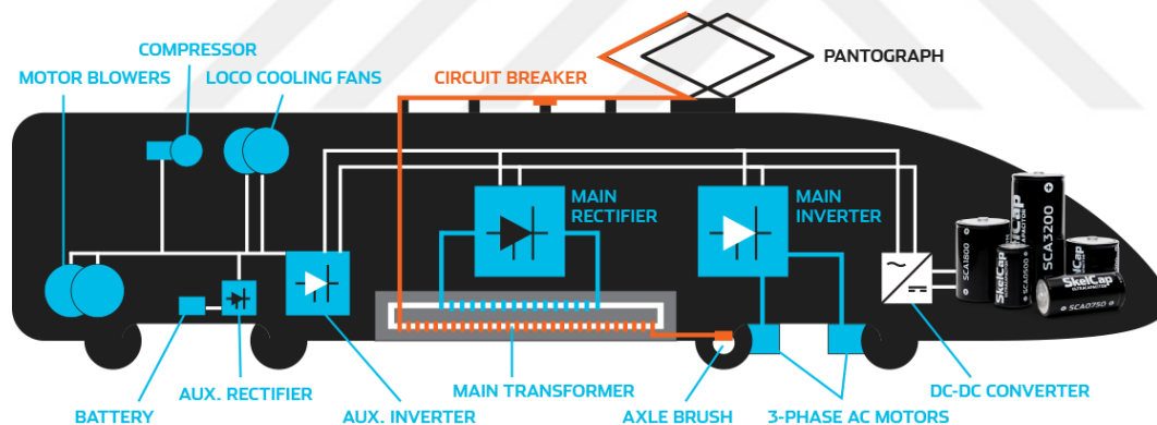
Figure 2.4: Main components of a locomotive [113]
