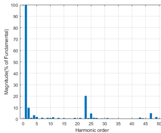
Figure 6.7: Inverter Output Voltage and Current Waveforms Obtained Switching Angles by HHO and Their FFT Distributions at 60 Hz, Half-Load at C point, 565 V DC-Link Voltage
