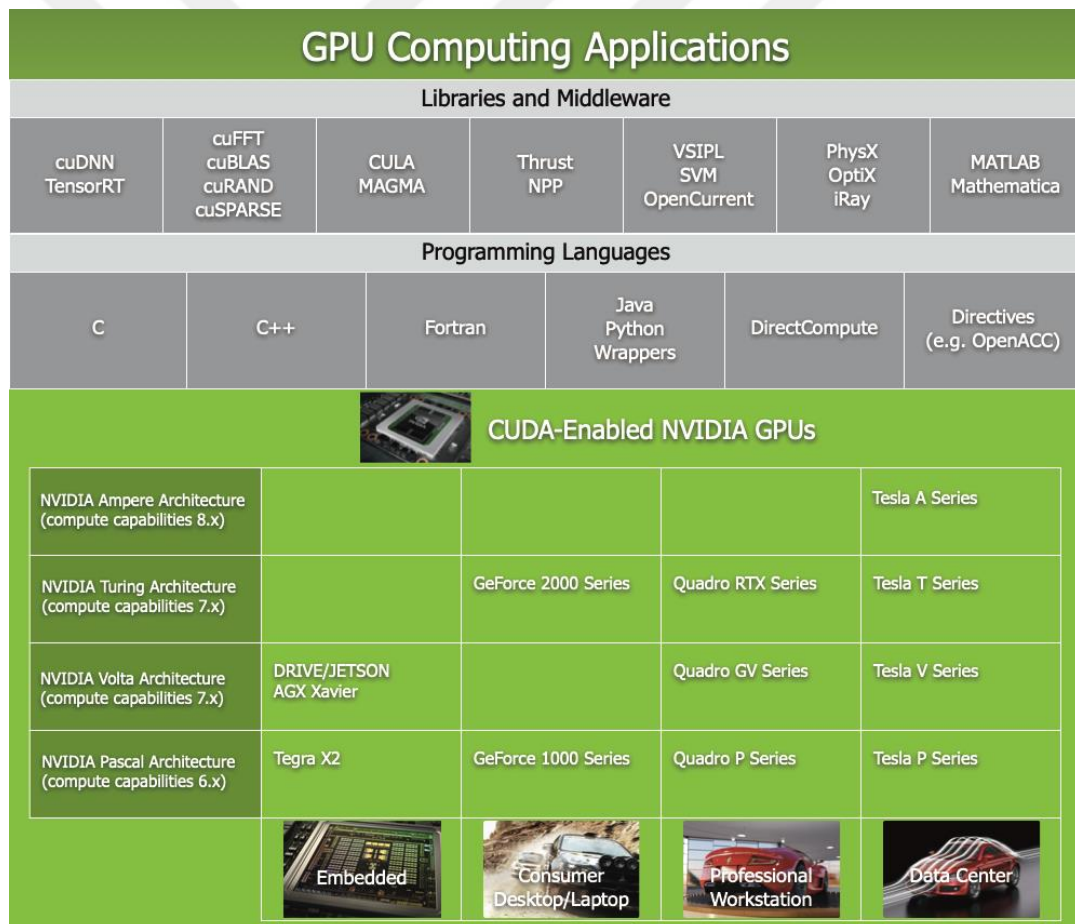
Figure 5.1: GPU computing applications
