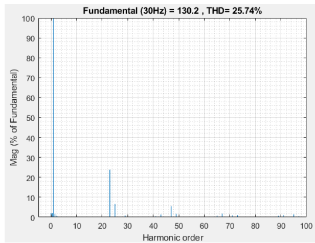
Figure 4.10: Inverter Output Voltage and Current Waveforms Obtained Switching Angles by HHO and Their FFT Distributions at 30 Hz, Full-Load, 750 V DC-Link Voltage
