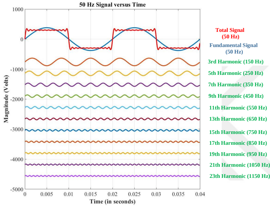
Figure 3.16: 50 Hz Voltage Signal and Harmonics up to 1150 Hz
