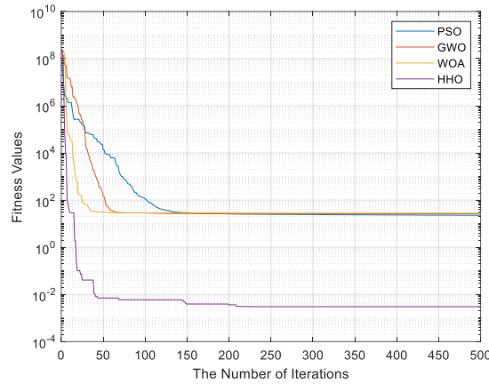
Figure 3.14: Convergence Curve of PSO, GWO, WOA, and HHO for F_5 Function
