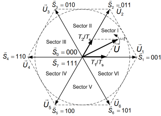
Figure 1.7: Voltage Vector Space
