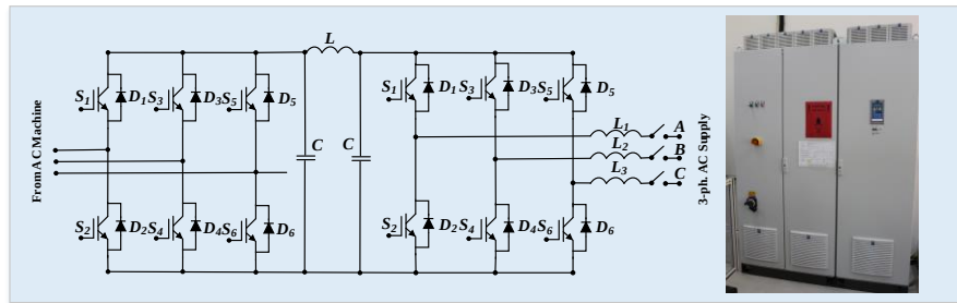
Figure 6.2: Traction System Laboratory Prototype for Railway Transportation, and the Block Diagrams of the System
