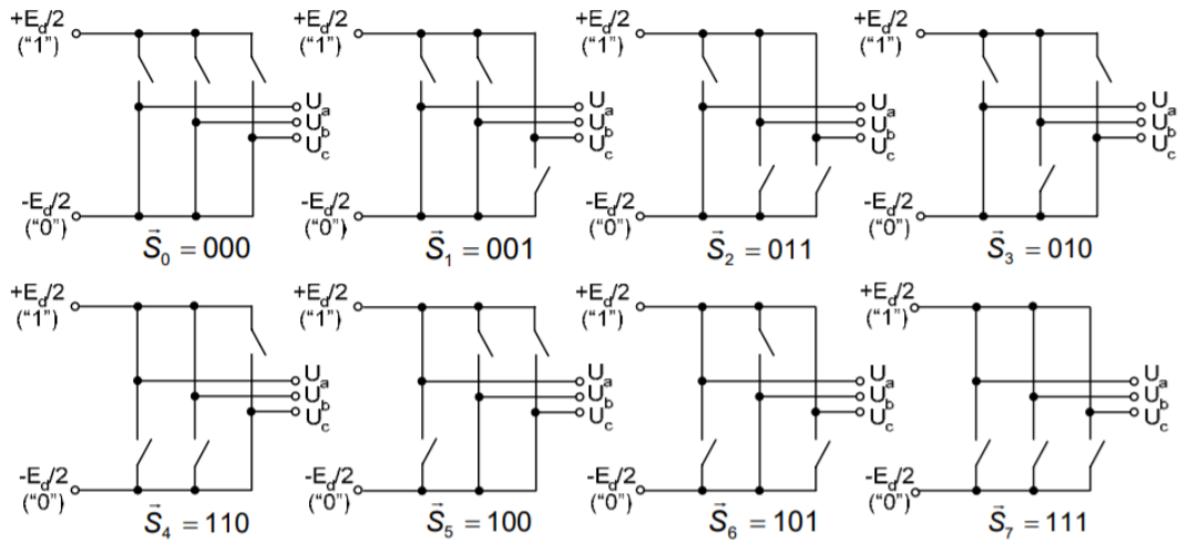
Figure 1.6: Eight Switch States
