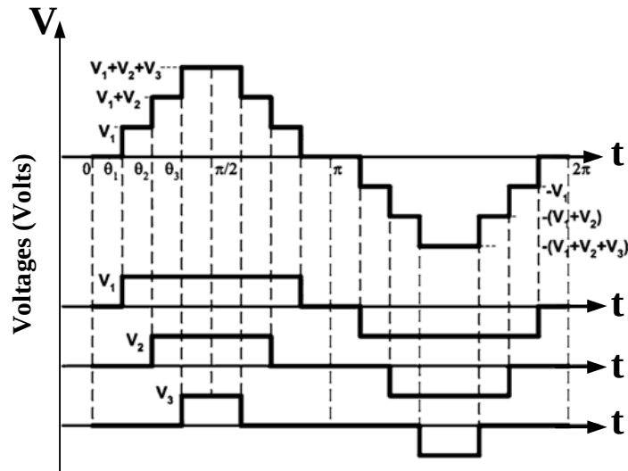
Figure 1.9: Seven-level VSI Voltage Waveform Applied to SHE-PWM
