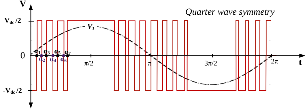
Figure 3.17: Definition of Seven SHEM Angles on Line-to-neutral Voltage Waveform Based on Quarter Wave Symmetry (Range of SHEM Angles in This Figure is 0-60°, v_1(t) is the Fundamental Component of Voltage for Modulation Index M=0.8 )
