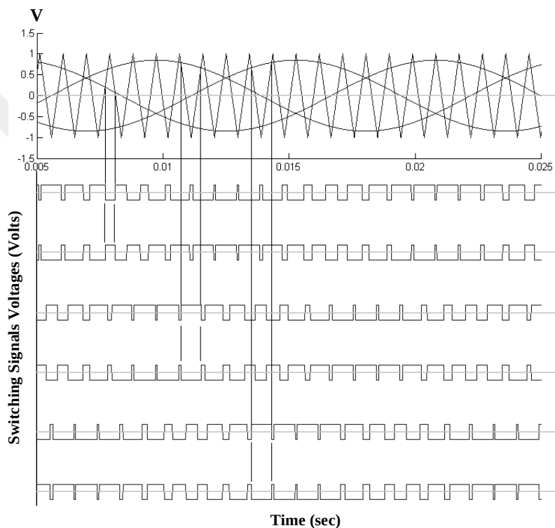
Figure 1.5: SPWM method gate signals
