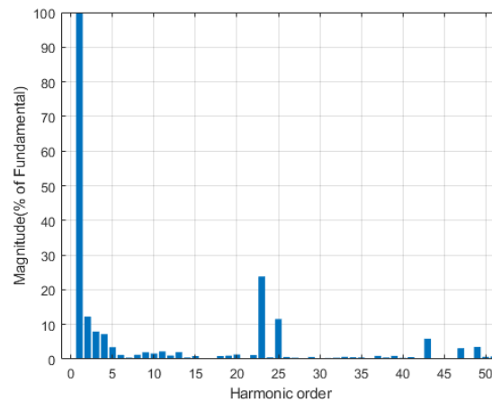
Figure 6.5: Inverter Output Voltage and Current Waveforms Obtained Switching Angles by HHO and Their FFT Distributions at 60 Hz, Full-Load at Point A, 565 V DC-Link Voltage
