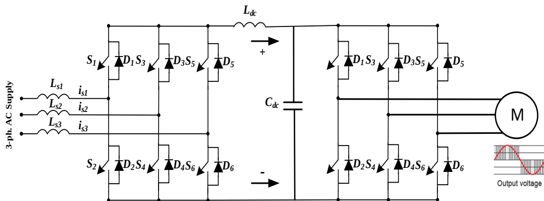
Figure 1.1: A Simple Diagram of Variable Frequency Drive
