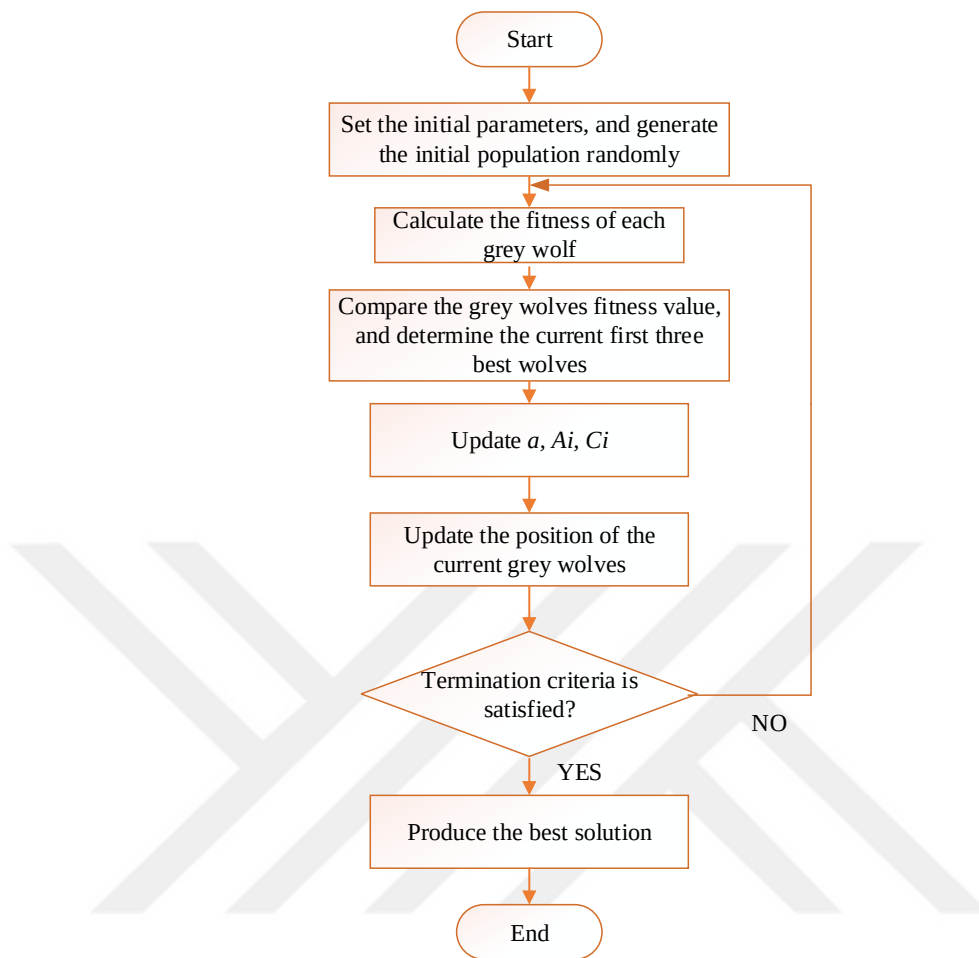
Figure 3.5: The Flowchart of the GWO Algorithm
