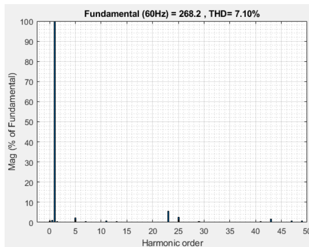
Figure 4.2: Inverter Output Voltage and Current Waveforms Obtained Switching Angles by PSO and Their FFT Distributions at 60 Hz, Full-Load, 750 V DC-Link Voltage
