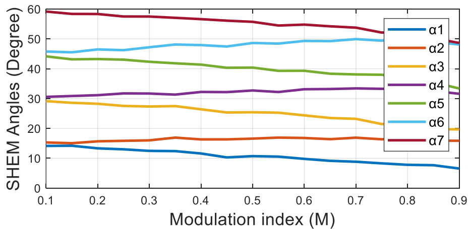
Figure 2.7: Switching Angles versus Modulation Index Distribution of the VSI
