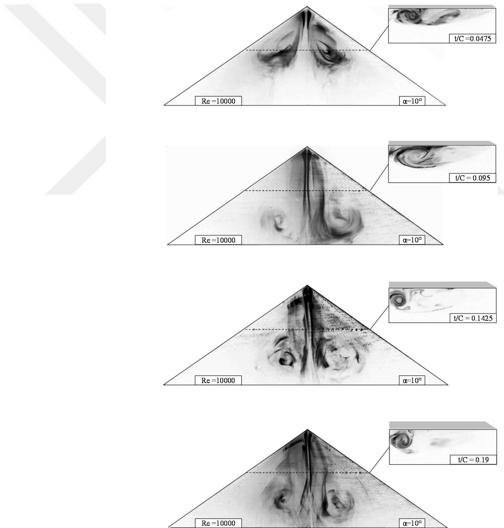
B.1 Surface and cross flow smoke visualizations for all wings at \alpha= 10^\circ for Re=10000
