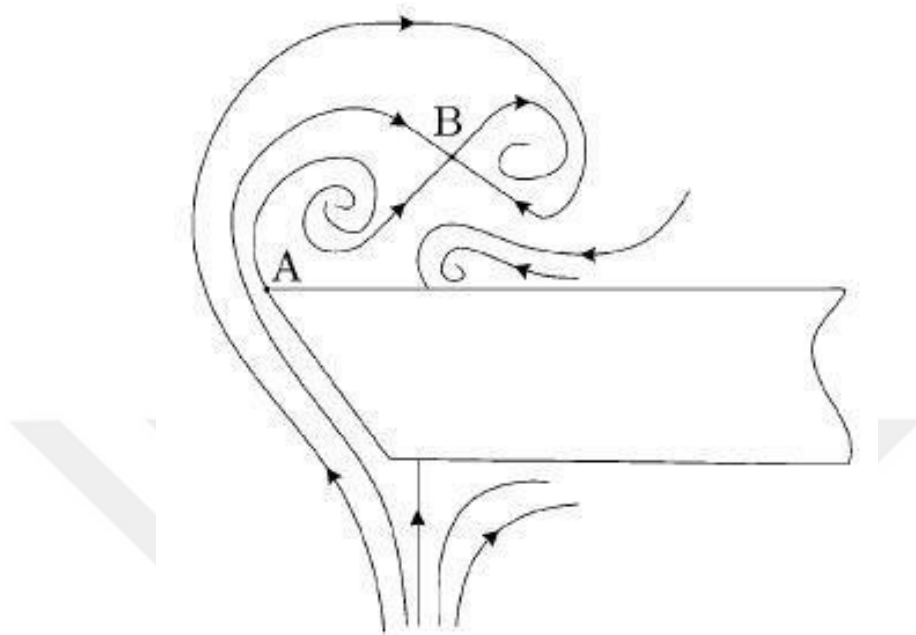
Figure 2.1 Sketch of dual vortex formation [37].
