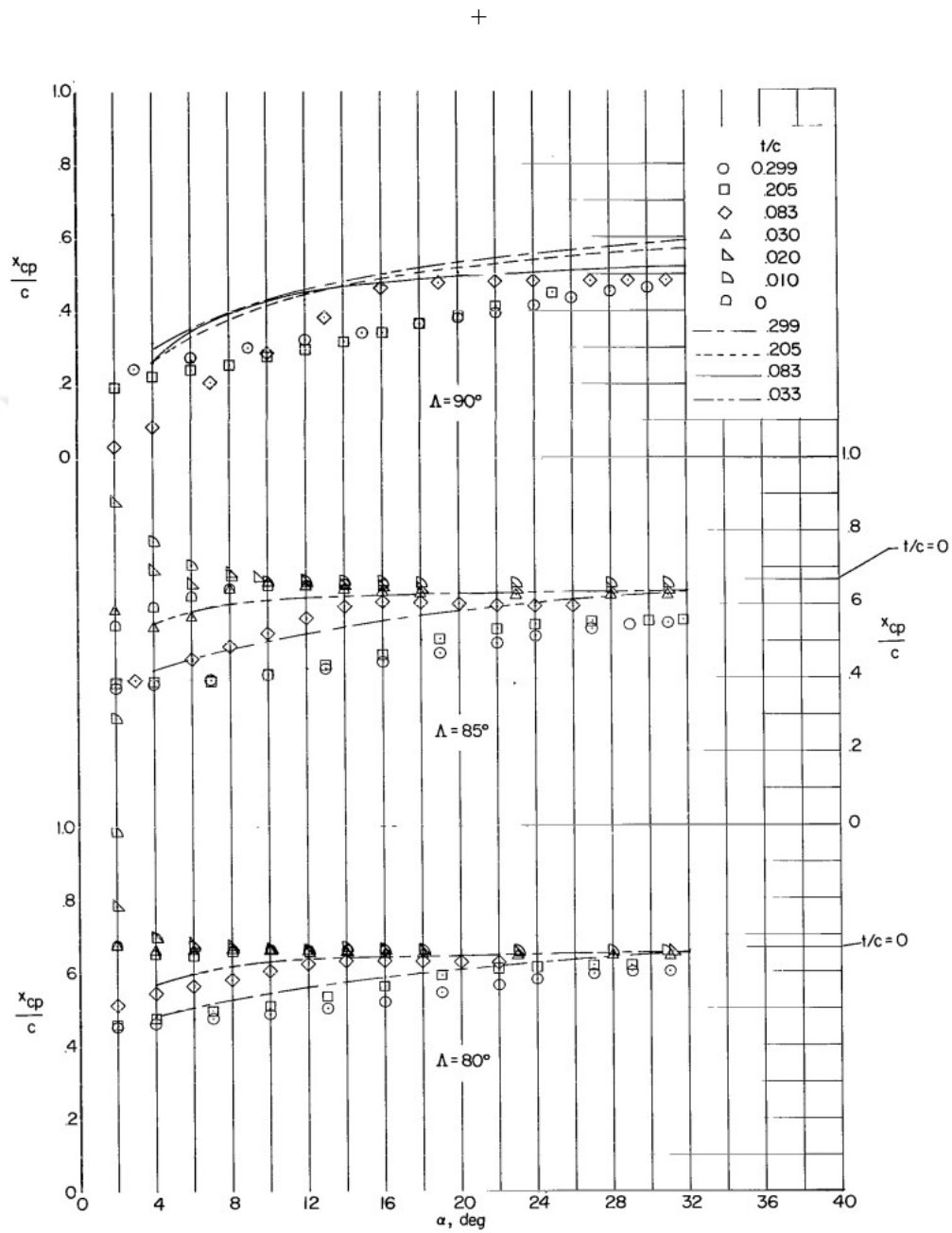
Figure 2.11 Variation of center of pressure with angle of attack [14].
