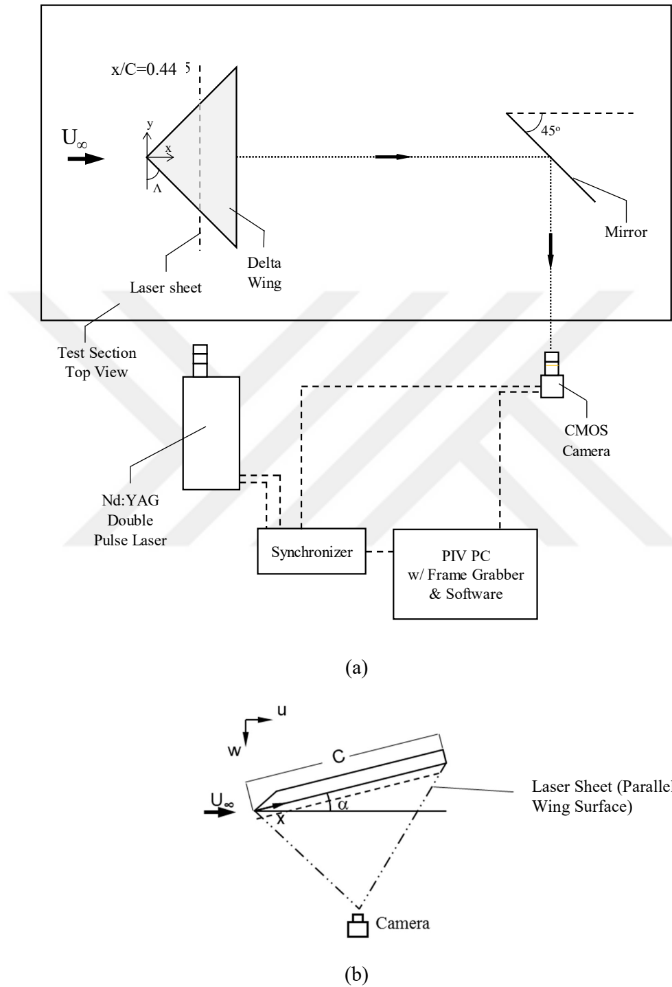
Figure 3.6 Schematic representation of the cross and surface flow PIV experiment set-up.
