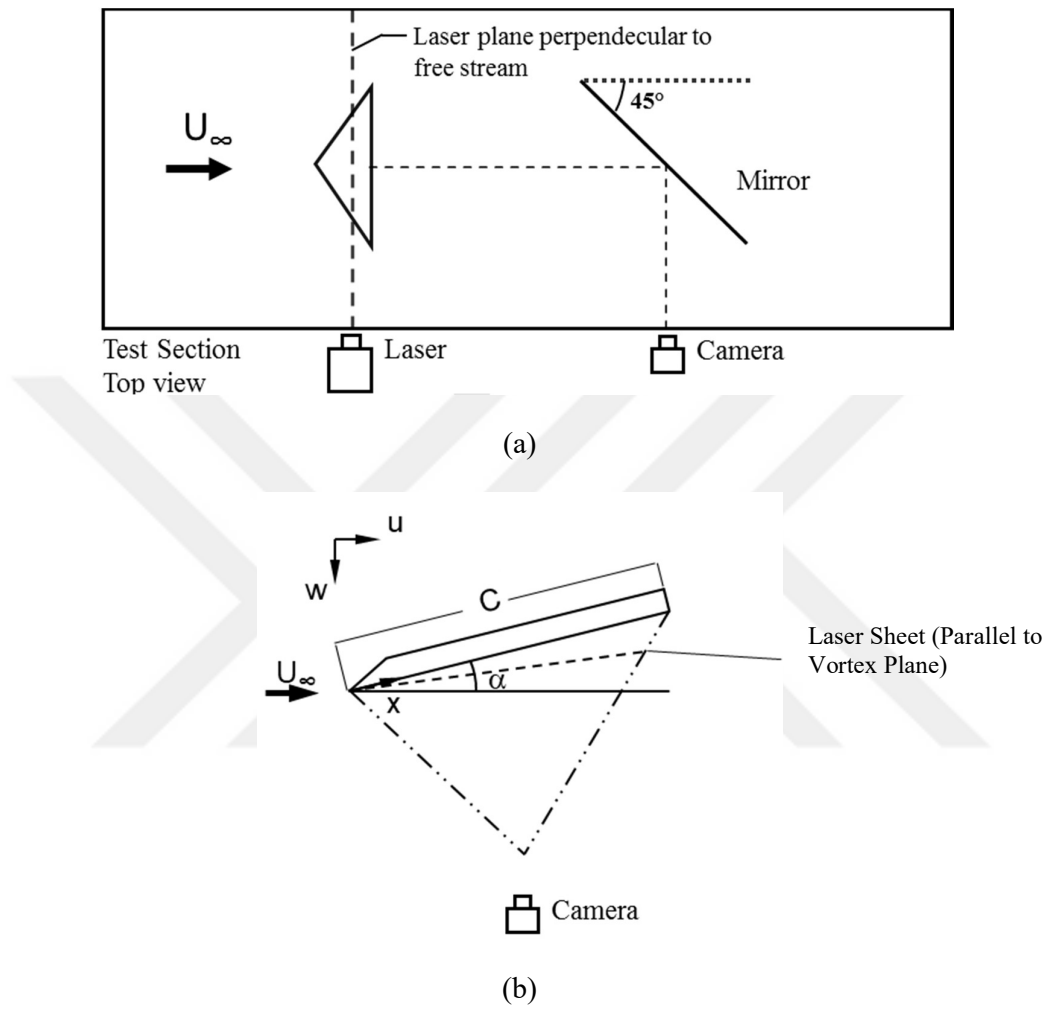
Figure 3.4 Schematics of (a) cross and (b) surface flow laser-illuminated smoke visualization experiment set-up.
