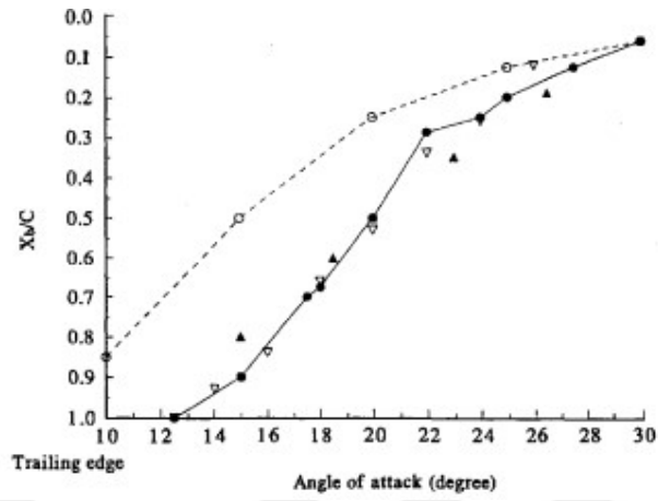
Figure 2.13 Comparison of vortex breakdown location: \Delta , Wentz et al [13]; and \nabla , Miao et al [16]; \circ , thick delta wing; \bullet , thin delta wing [62].
