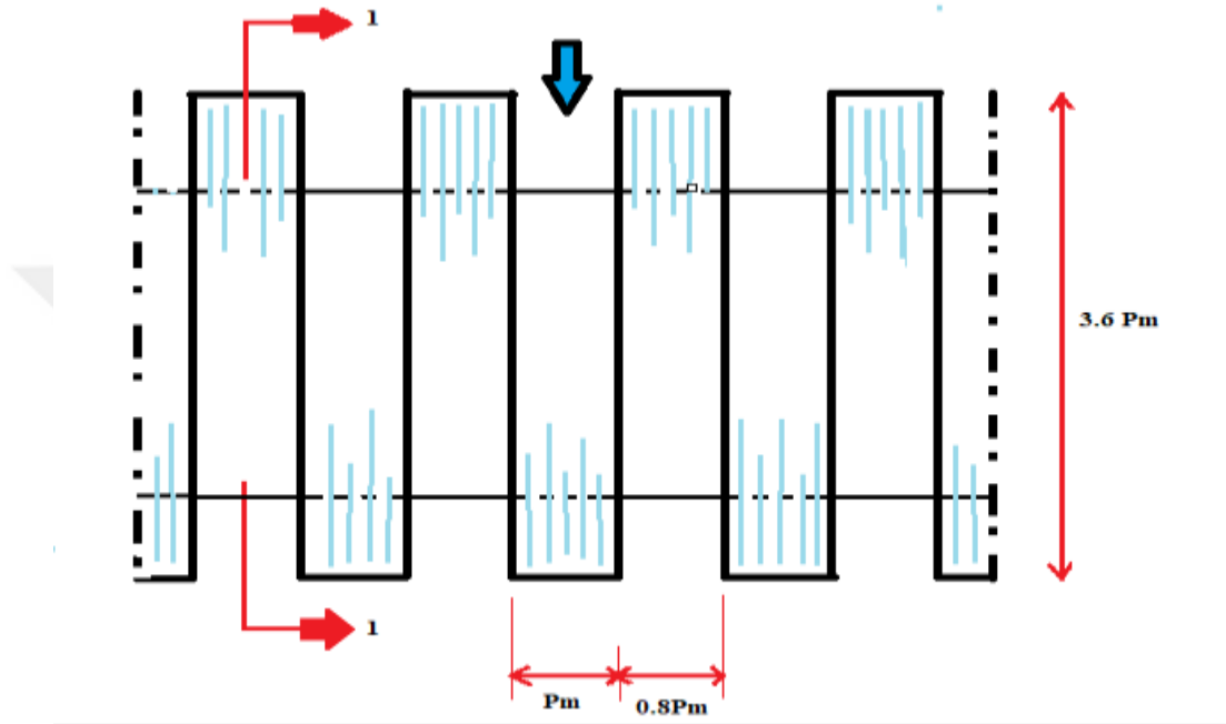
Figure 3.4: Plan View of the PKW
