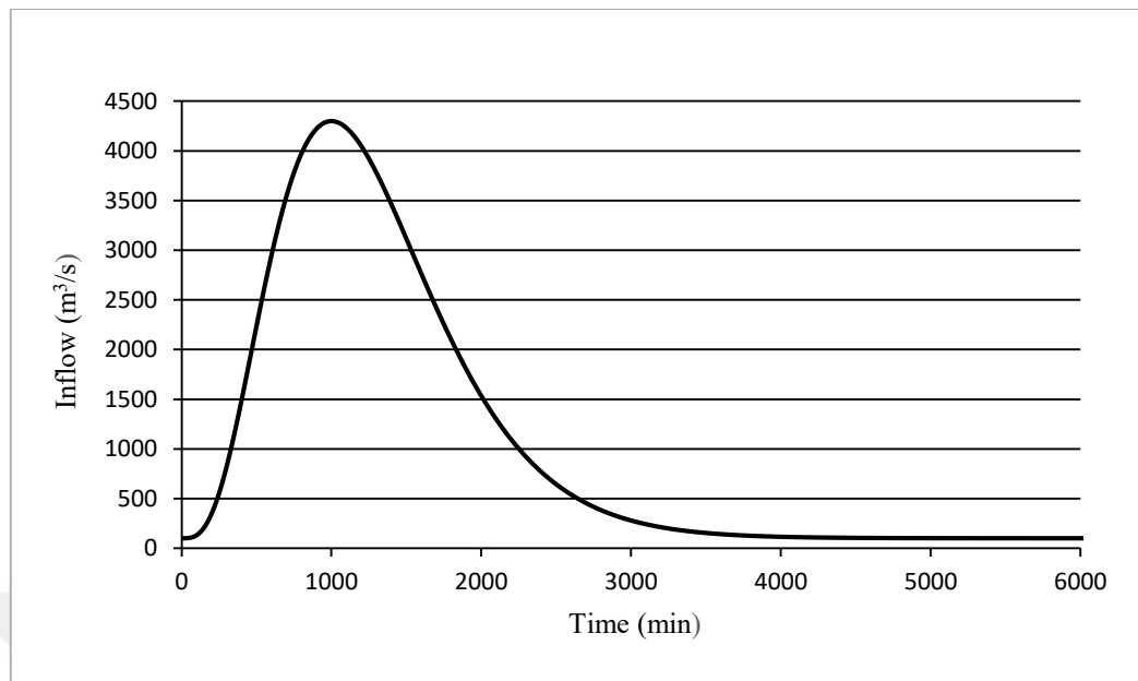
Figure 3.3: Inflow Hydrograph
