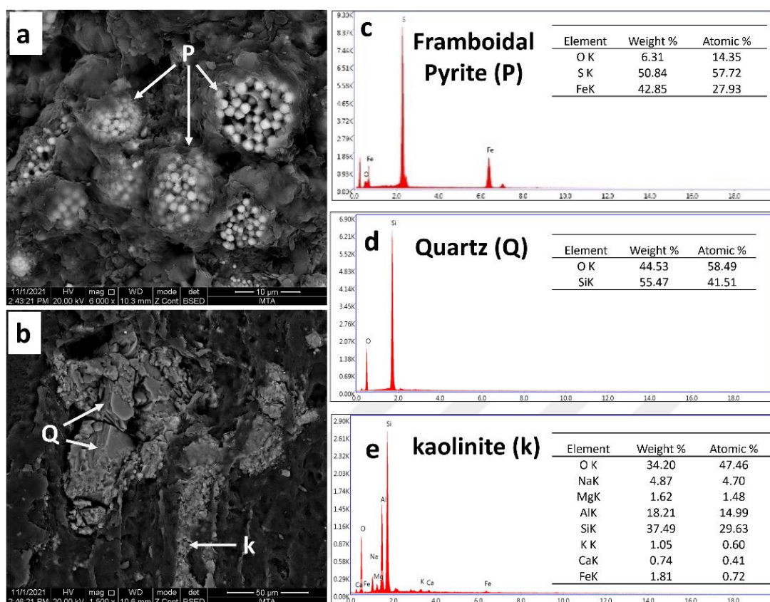
Figure 4.10 SEM-EDS analysis of mineral content present in cleaned Oltu-stone wastes. a). SEM image of framboidal pyrite. b). SEM image of quartz and kaolinite. c). EDS spectrum of framboidal pyrite. d). EDS spectrum of quartz. e). EDS spectrum of kaolinite
