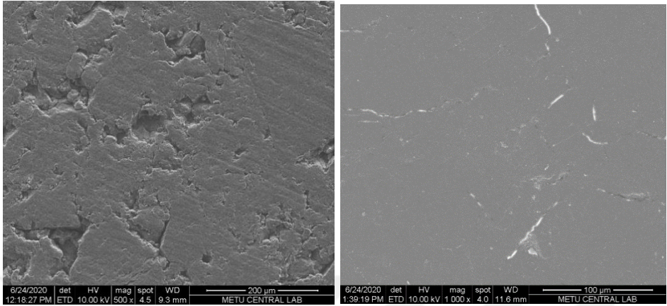
Figure B.1 Pressed Oltu-stone by a) Method-A (MA) b). Method-C (MC)
