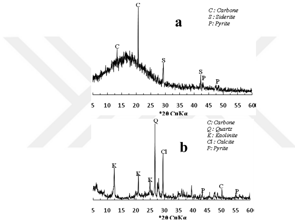
Figure 2.10 a)-The XRD pattern of Oltu-stone and b)- Oltu-stone bearing rock deposits (Kalkan et al., 2012)
