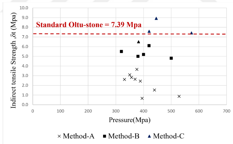
Figure 4.20 Indirect Tensile strength of Oltu-stone agglomerates produced by different methodologies.
