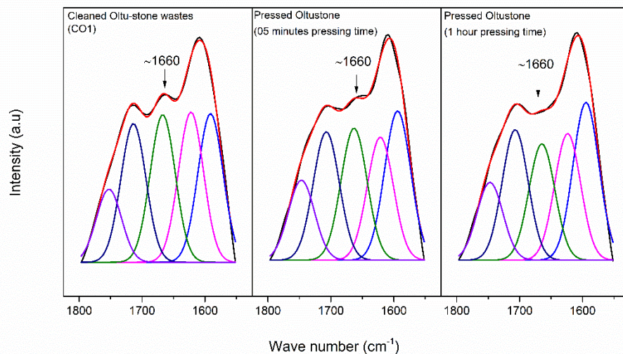
Figure 4.35 FTIR fitted curve of 1800-1550 \text{cm}^{-1} , showing an effect of pressing time on a conjugated carbonyl.
