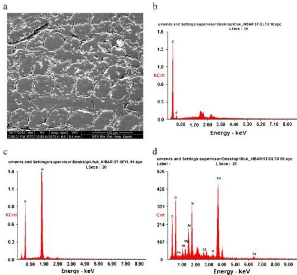
Figure 2.9 SEM-EDS examination of Oltu-stone (a). Oltu-stone cellular structure. (b) EDS results at the boundary of the cell. c)- EDS analysis of the inner cell core (d). EDS results of rarely found elements in Oltu-stone. (Toprak, 2013)
