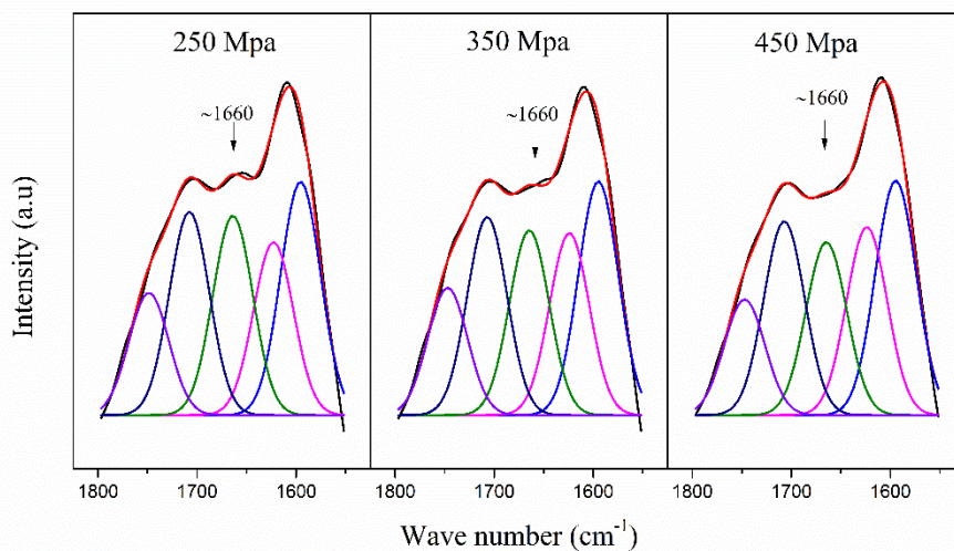
Figure 4.36 FTIR fitted curve of 1800-1550 \text{cm}^{-1} , showing an effect of pressure on a conjugated carbonyl.
