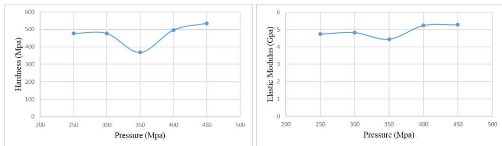
Figure 4.28 Effect of different pressure with constant pressing time (60 minutes) on hardness and elastic modulus.
