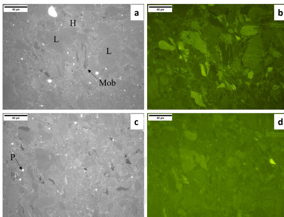
Figure 4.31 Pressed Oltu-stone a). radial surface showing mobilization (Mob) of liptinite content in coarse particles due to heat-pressure treatment. b). Panel-a under blue light excitation. c). cross-section part showing the homogenous distribution of macerals. d). Panel-c under blue light excitation. (L=liptinite, H=huminite, P=pyrite)
