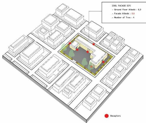
Figure 3.8. The Cool Facade intervention
