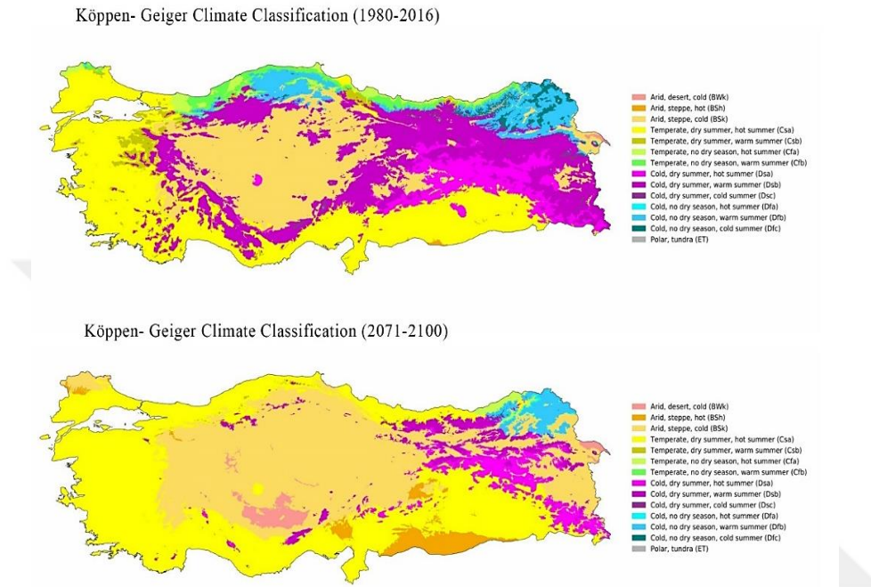
Figure 2.3 Future climate scenario for Turkey (Beck et al., 2018)
