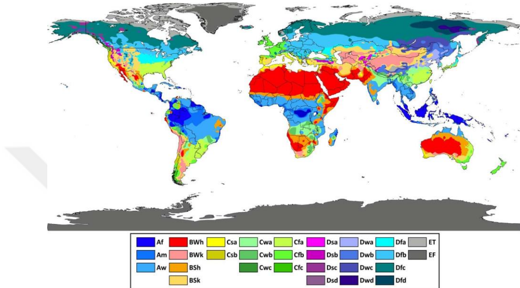
Figure 2.2 Köppen-Geiger climate classification map (Beck et al., 2018)
