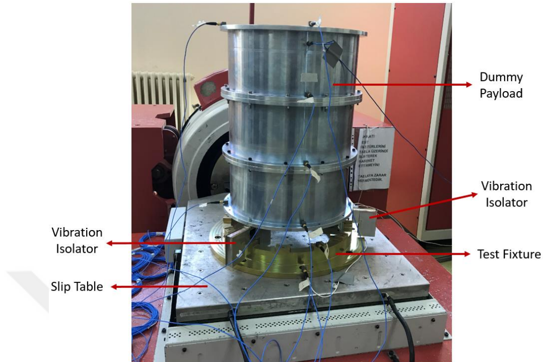
Figure 6-34 The experimental setup for vibration tests in lateral direction
