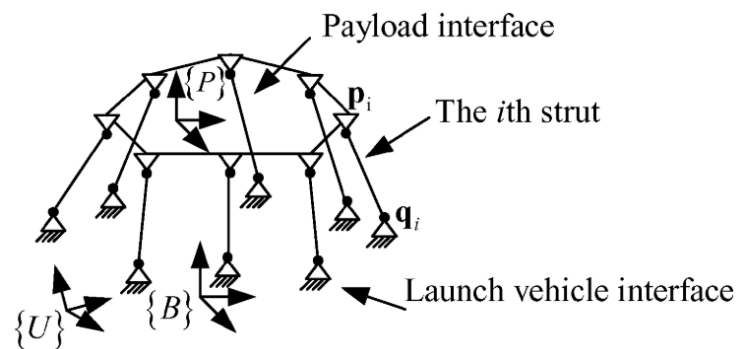
Figure 2-1 Typical octostrut vibration isolation platform
