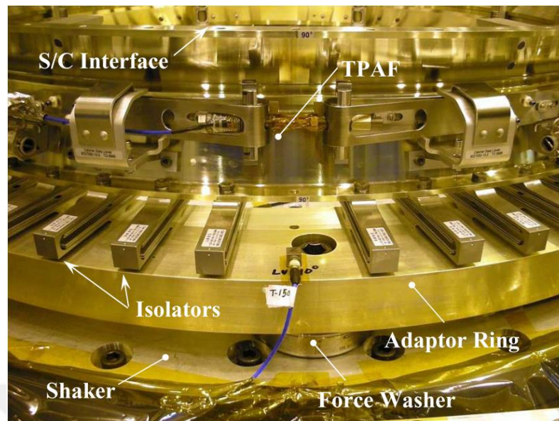
Figure 2-11 SoftRide UniFlex Isolators in OCO Test Configuration [30]
