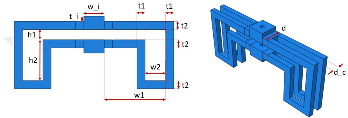
Figure 5-12 Design Parameters of S1-Vibration Isolator
