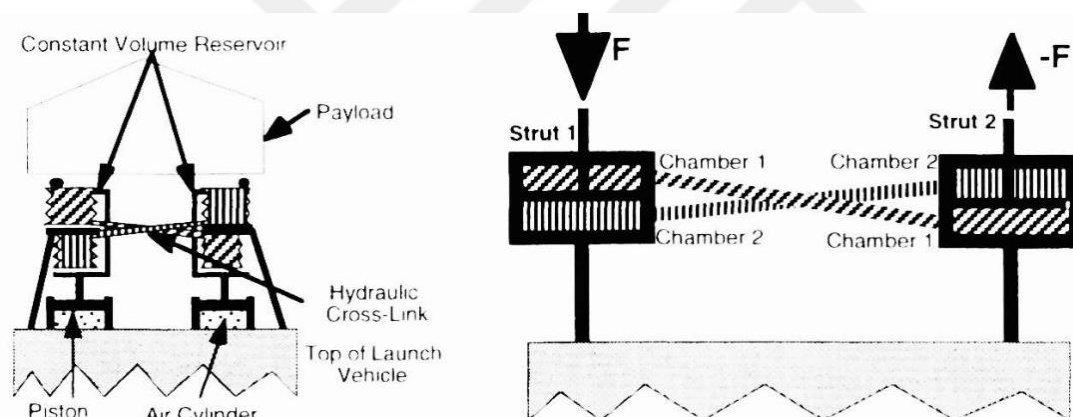
Figure 2-2 Vibration isolation concept in the LVIS program [16]
