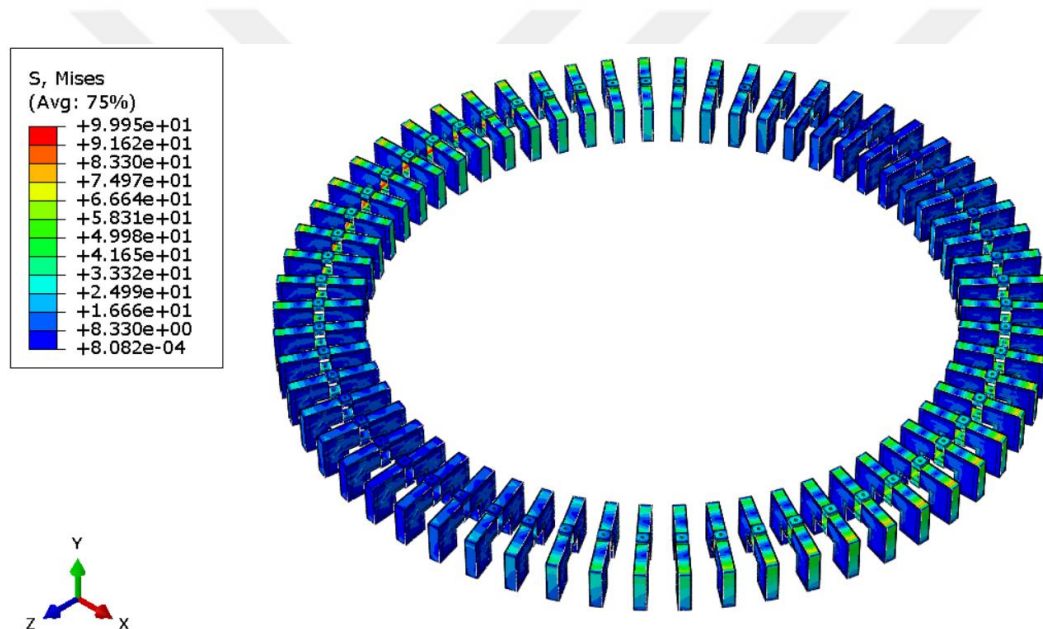
Figure 6-29 S1 VIS – Stress results of quasi-static load analysis in lateral direction
