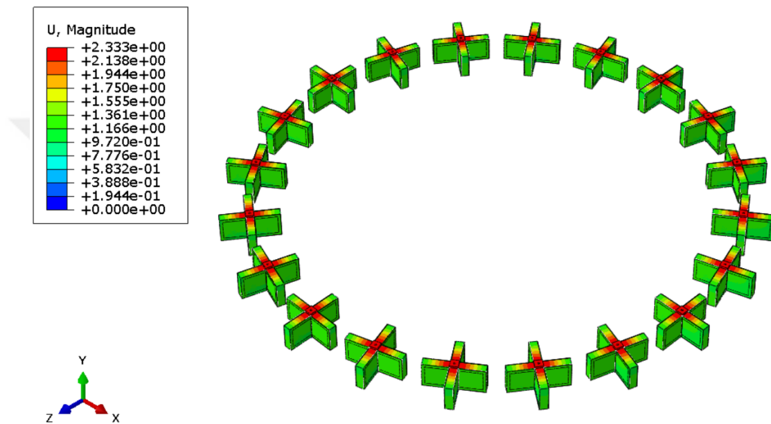
Figure 6-21 T2 VIS – Displacement results of quasi-static load analysis in longitudinal direction
