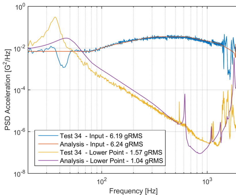
Figure 6-100 S1 – The comparison of Test 34 and random vibration analysis results for lower point
