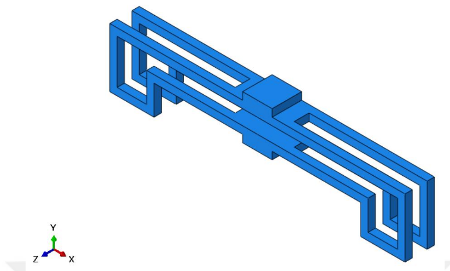
Figure 4-8 Conceptual design of S1 vibration isolator based on similar vibration isolators
