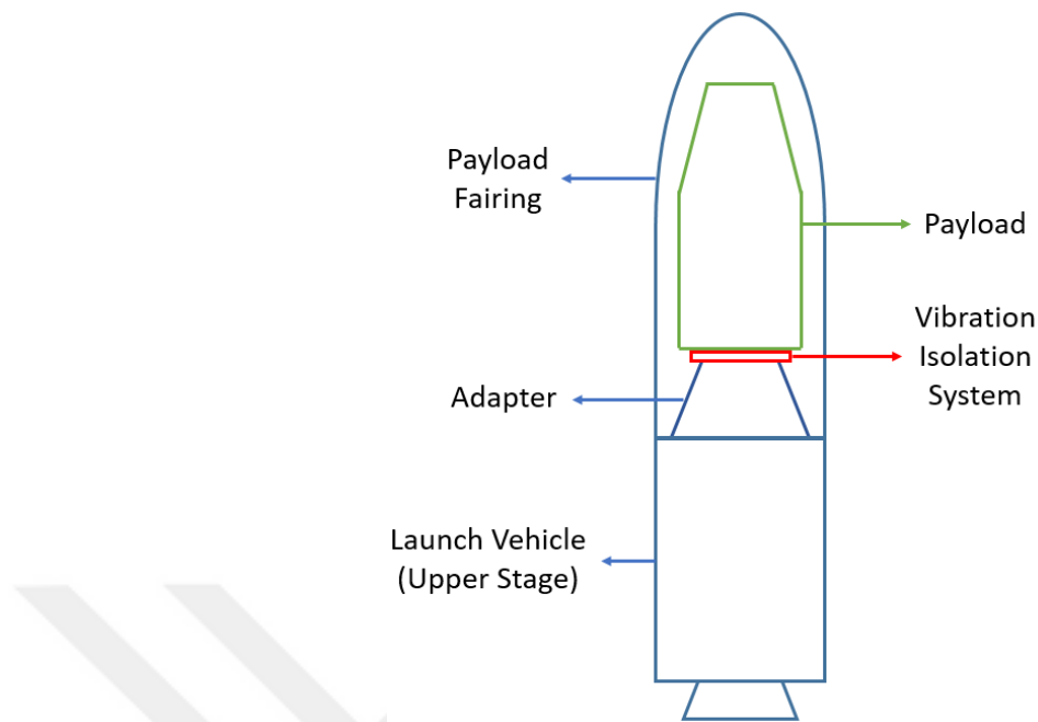
Figure 1-6 Vibration Isolation System at Payload-Launch Vehicle Interface
