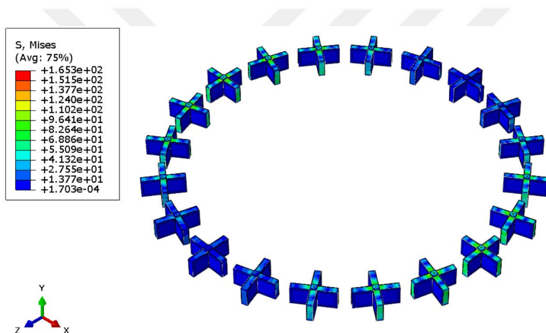
Figure 6-20 T2 VIS – Stress results of quasi-static load analysis in lateral direction
