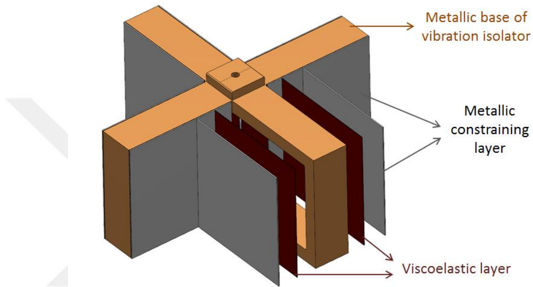
Figure 5-9 T2-Vibration isolator with damping application
