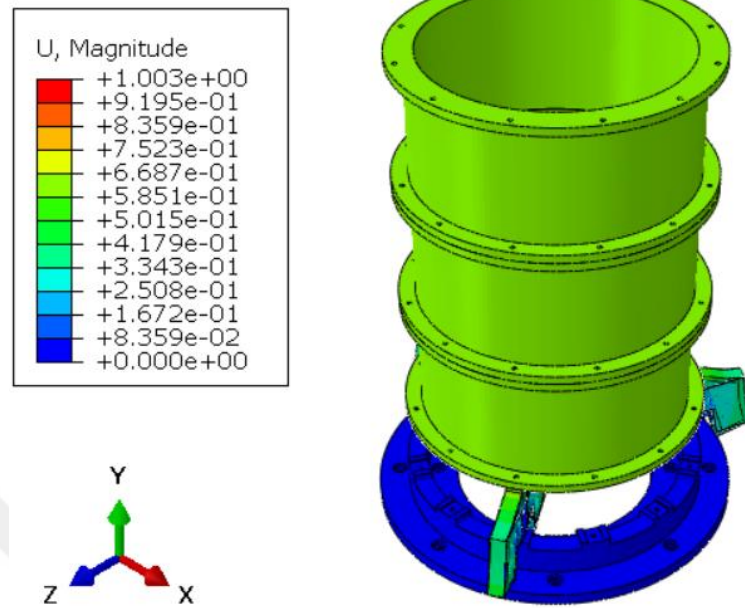
Figure 6-88 Axial mode shape of S1 test configuration, 46 Hz
