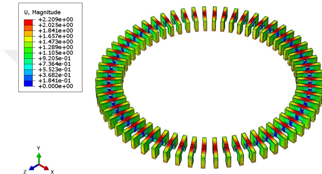
Figure 6-30 S1 VIS – Displacement results of quasi-static load analysis in longitudinal direction
