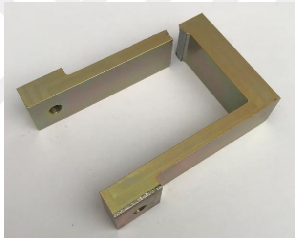
Figure 6-62 Broken T1 vibration isolator
