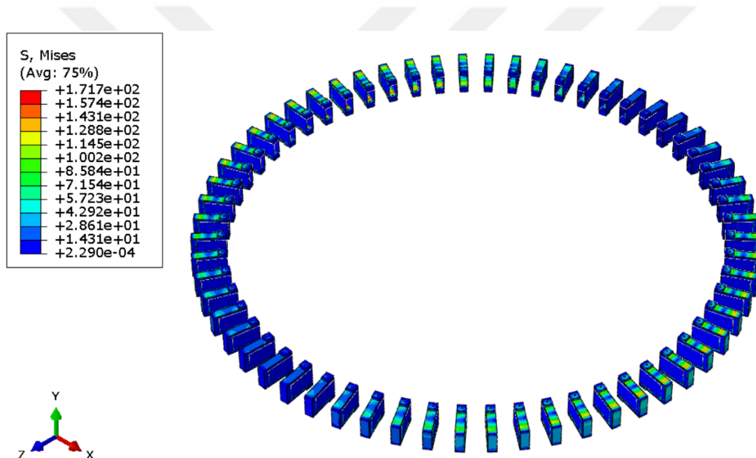
Figure 6-11 T1 VIS – Stress results of quasi-static load analysis in lateral direction
