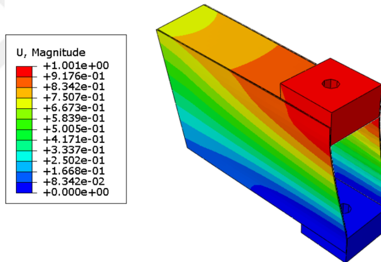
Figure 5-7 Internal resonance of T1 for BC-2, 484 Hz
