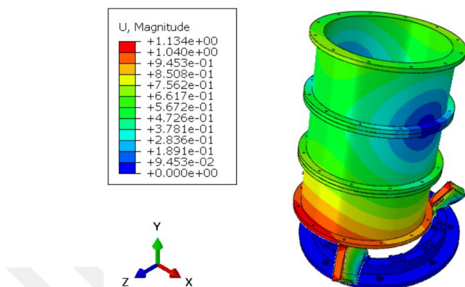
Figure 6-42 Lateral mode shape of T1 test configuration, 50 Hz
