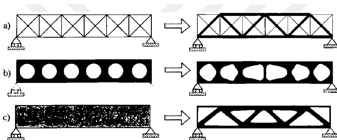
Figure 4-1 Three classes of structural optimization. a) Sizing, b) shape, c) topology. [65]
