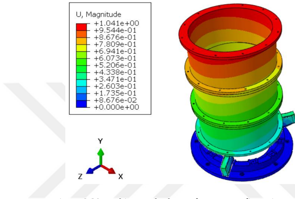
Figure 6-39 Rocking mode shape of T1 test configuration, 14 Hz
