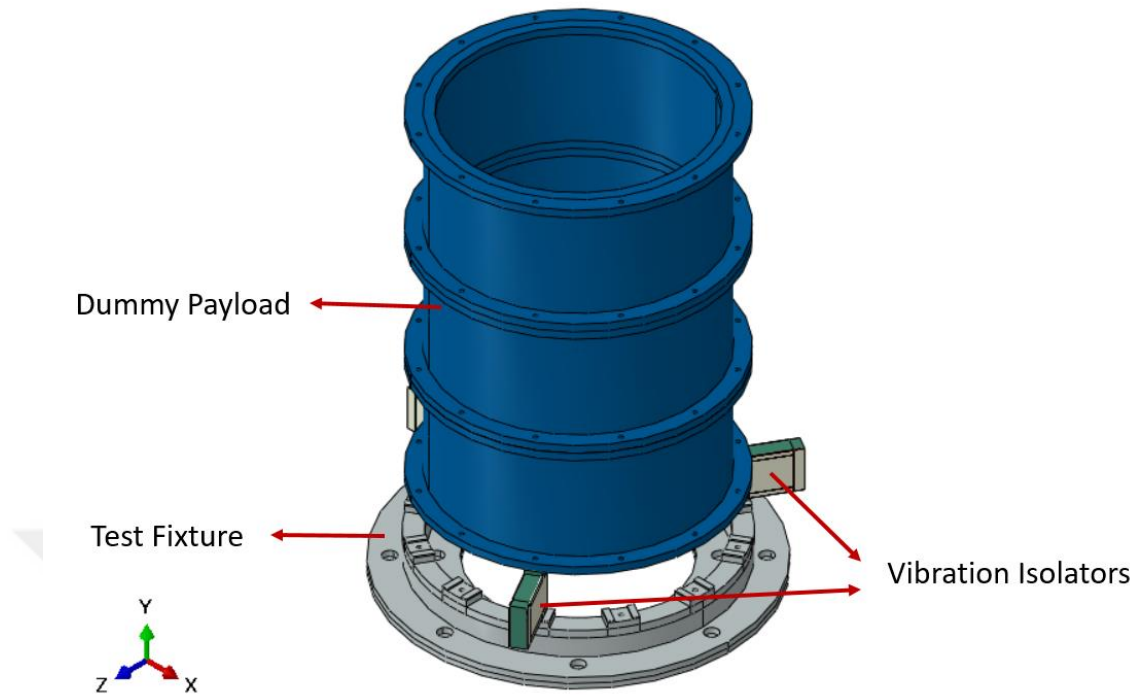
Figure 6-32 Finite element model of test configuration of VIS
