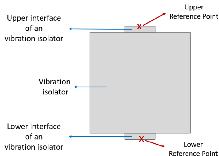
Figure 5-2 Schematic view of vibration isolator
