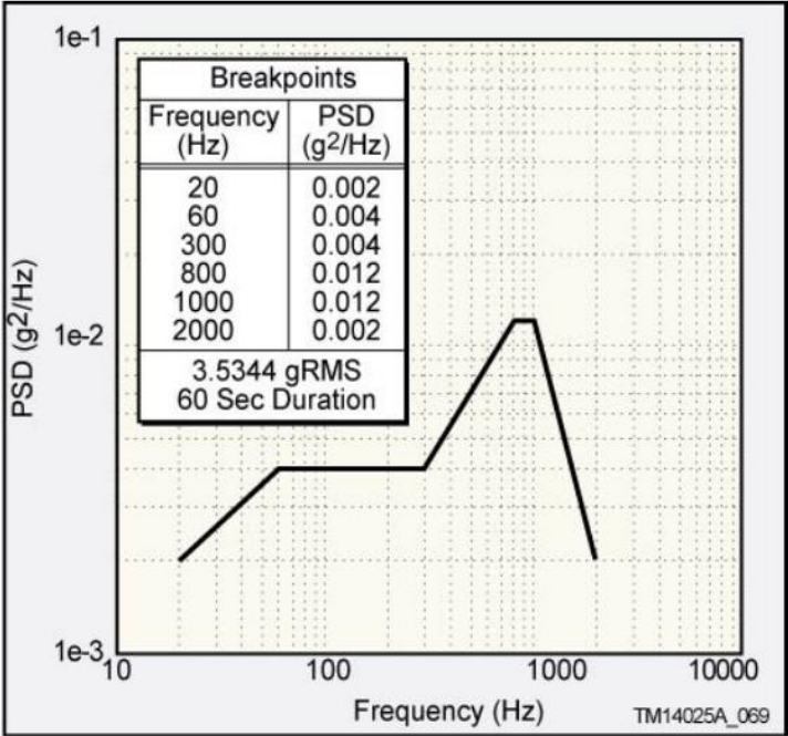
Figure 1-4 Minotaur - Payload random vibration environment during launch [4]
