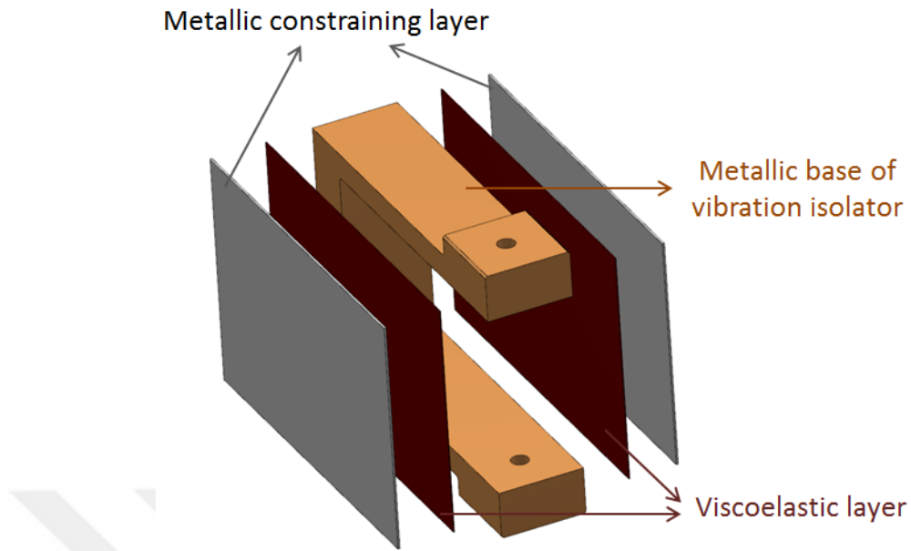
Figure 5-5 Damping concept – D3
