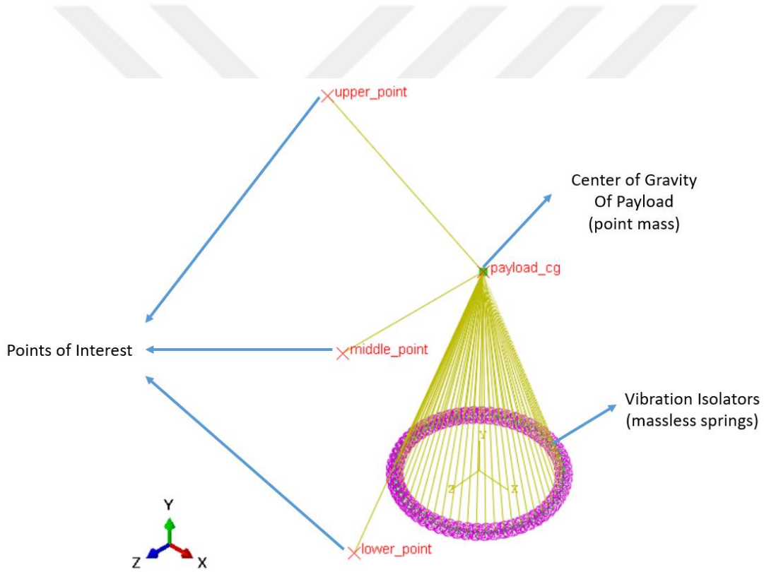
Figure 3-4 Schematic View of Vibration Isolation System
