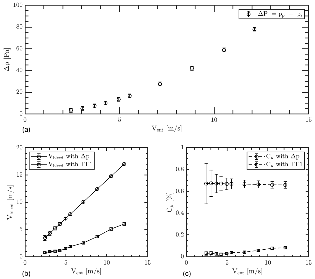
Figure 4.2: Stage 2, tunnel on measurements: (a) Pressure difference across the bleed hole with respect to bleed entrance velocity V_{\text{ent}} = U_\infty , ( 0.9 \times 10^4 \leq \text{Re} \leq 1.1 \times 10^5 ), (b) Bleed velocity V_{\text{bleed}} , and (c) Momentum coefficient estimation C_\mu , pressure difference \Delta p (circle markers), and hot wire TF1 (square markers).
