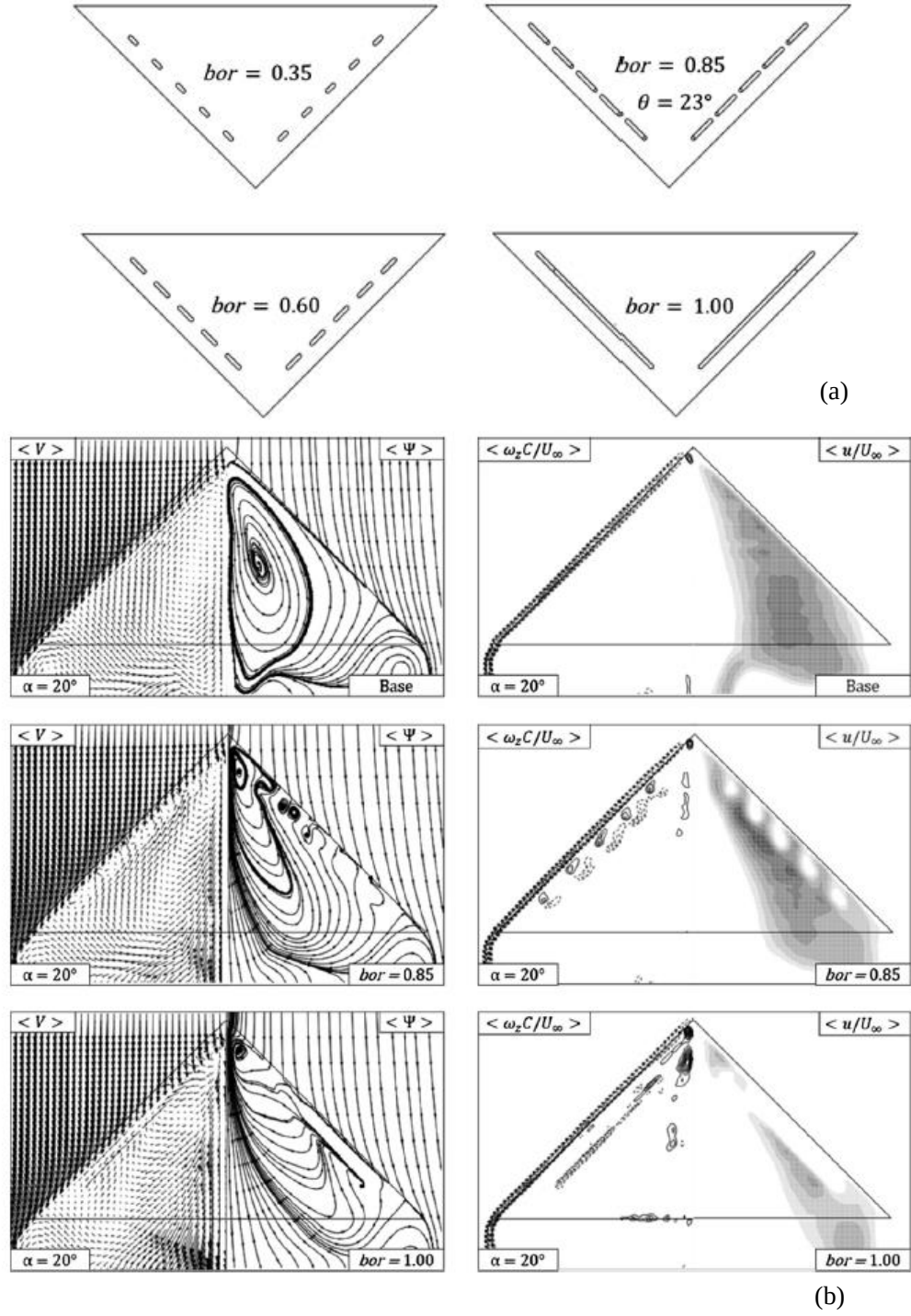
Figure 2.28: (a) Schematic representation of bleeding wings with different bleed opening ratios. (b) Time-averaged surface PIV comparisons at Re = 5 \times 10^4 and \alpha = 20^\circ [53].
