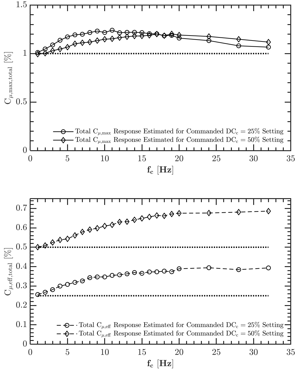
Figure 7.1: Overall calculated maximum C_{\mu,\max} and effective C_{\mu,\text{eff}} momentum coefficient response in comparison to commanded settings.
