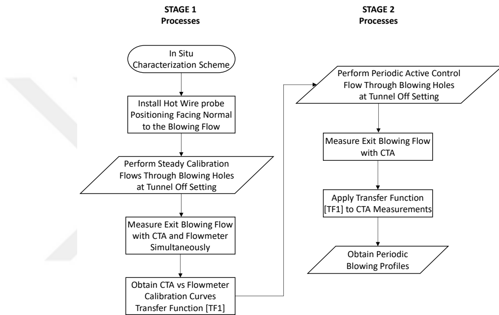
Figure 3.25: Active flow control in situ calibration process flow chart.
