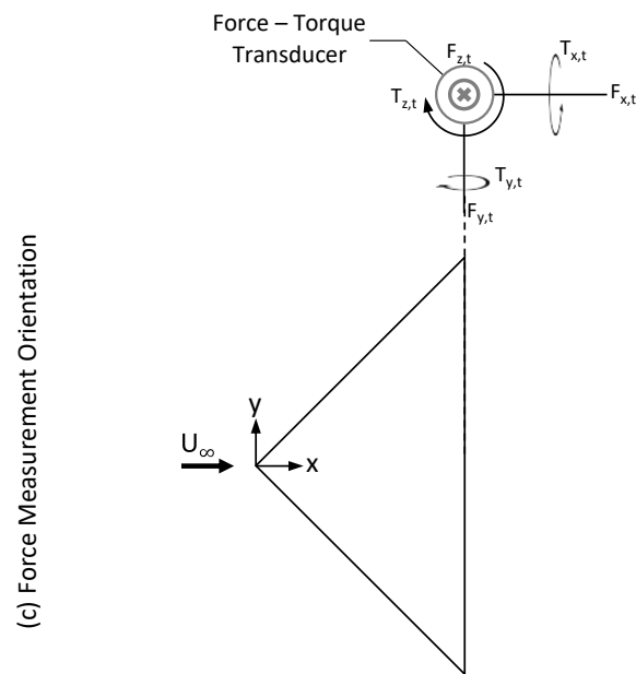
Figure 3.22: Schematic representation of the utilized measurement techniques: (a) Near surface PIV plane, (b) Pressure measurement plane, and (c) Force measurement orientation.
