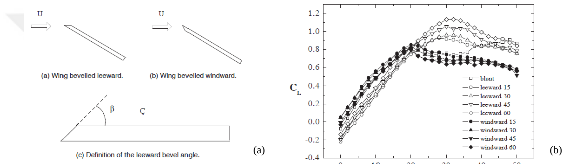
Figure 2.20: Effect of bevel direction and angle [41] for \Lambda = 50^\circ non-slender delta wing: (a) schematic of edge modifications, (b) lift coefficient distributions.
