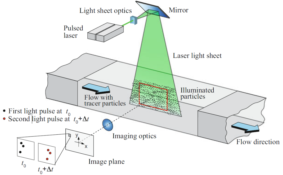
Figure 3.5: Sample experimental arrangement for a planar 2C-2D PIV setup in a wind tunnel [94].
