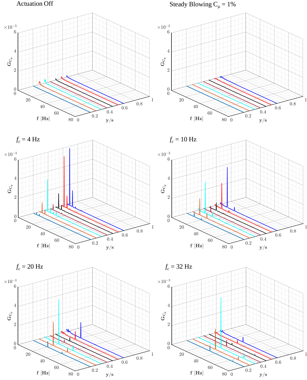
Figure 7.9: One sided power spectral density of C_p distribution at half span for regular square wave blowing ( f_c = [4, 10, 20, 32] \text{ Hz} , DC_c = 25\% , C_{\mu, \max} = 1\% ) in comparison to steady blowing ( C_\mu = 1\% ) at \alpha = 16^\circ , Re = 9 \times 10^4 .
