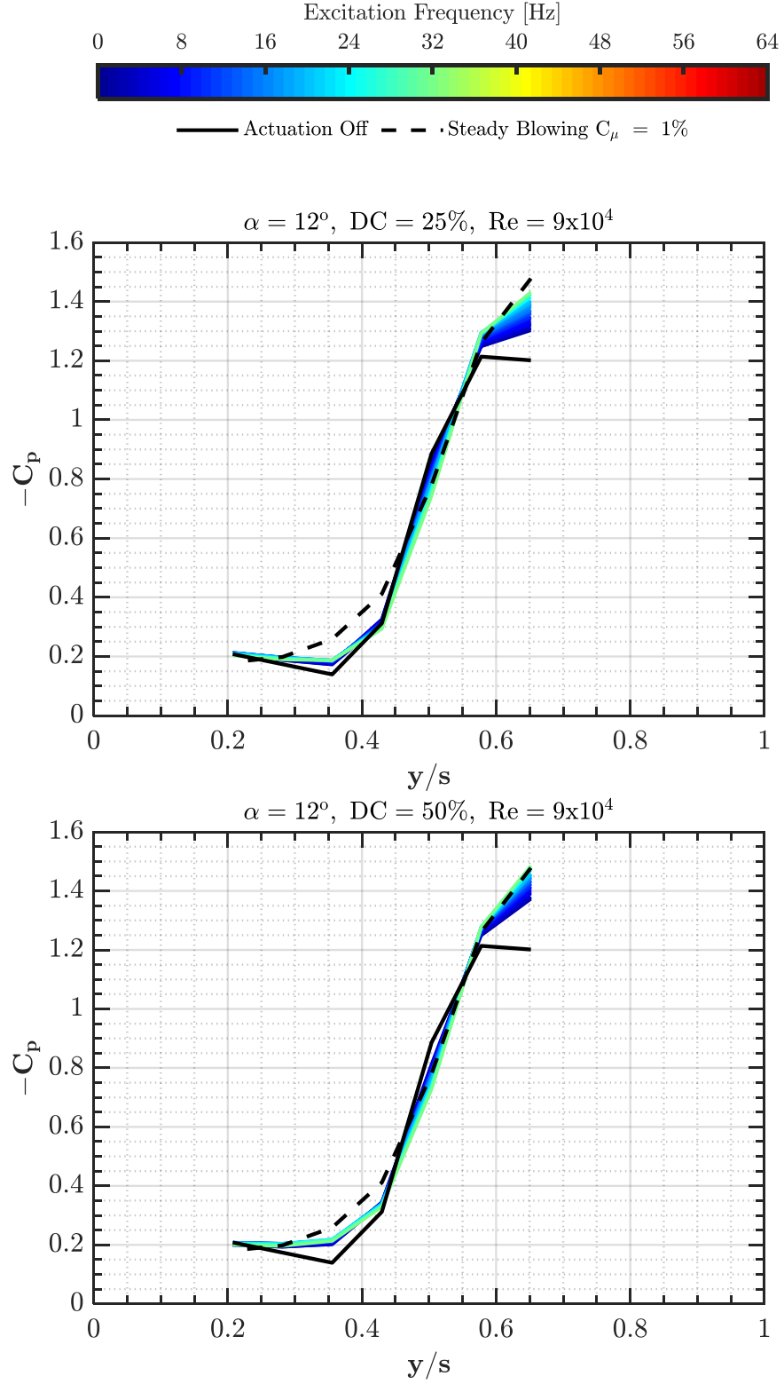
Figure 7.2: -C_p distribution at half span for regular square wave blowing ( f_c = 1-32 Hz, DC_c = 25, 50\% , C_{\mu, \max} = 1\% ) in comparison to steady blowing cases ( C_\mu = 1\% ) at \alpha = 12^\circ , Re = 9 \times 10^4 .
