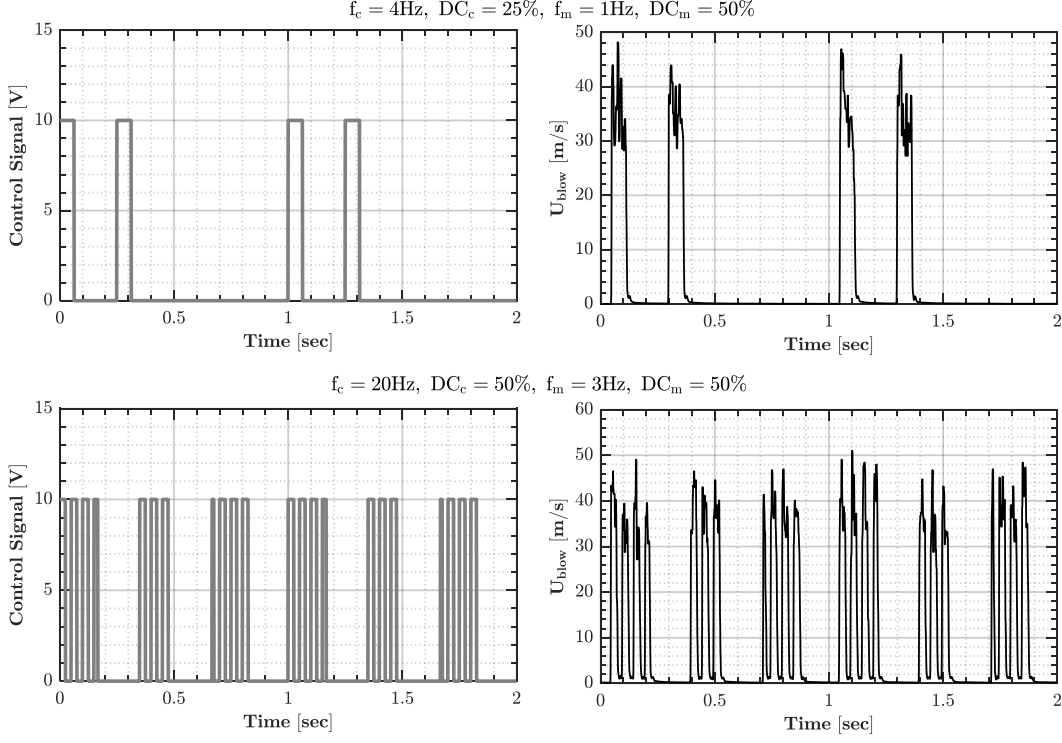
Figure 3.28: Sample burst modulated square wave control signal and CTA response measurements for #1 Blowing Hole: (a) f_c = 4\text{ Hz} , DC_c = 25\% and f_m = 1\text{ Hz} , DC_c = 50\% , (b) f_c = 20\text{ Hz} , DC_c = 50\% and f_m = 3\text{ Hz} , DC_c = 50\% .
