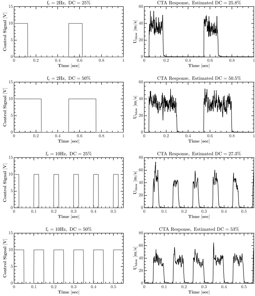
Figure 6.2: Sample square wave control signal and CTA response measurements for #1 blowing hole: f_c = 2 and 10\text{ Hz} , DC = 25\% and 50\% .
