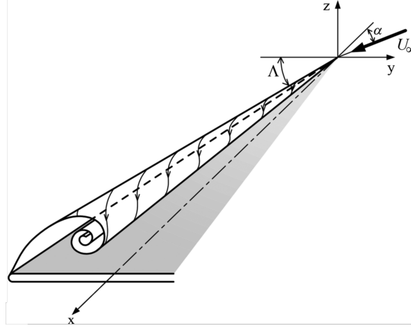
Figure 1.1: Designation of delta wing leading edge vortex formation; principal axis, sweep angle [3].
