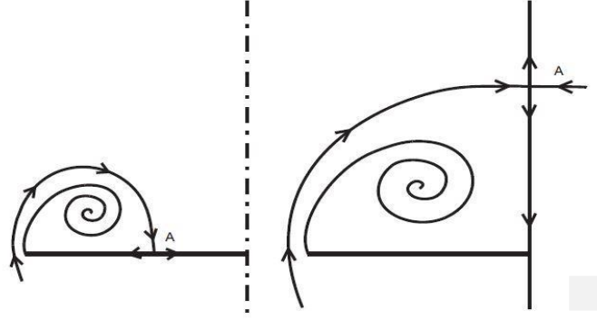
Figure 2.7: Flow reattachment process: Non-slender (left) and slender (right) wings [25].
