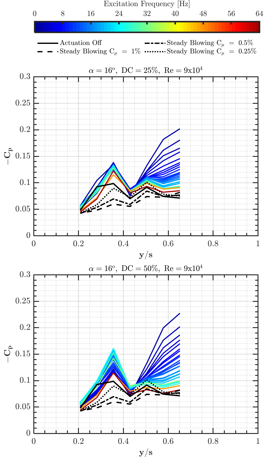
Figure 7.7: RMS of C_p distribution at half span for regular square wave blowing ( f_c = 1 - 64 Hz, DC_c = 25, 50\% , C_{\mu, \max} = 1\% ) in comparison to steady blowing cases ( C_\mu = 0.25\%, 0.5\%, 1\% ) at \alpha = 16^\circ , Re = 9 \times 10^4 .
