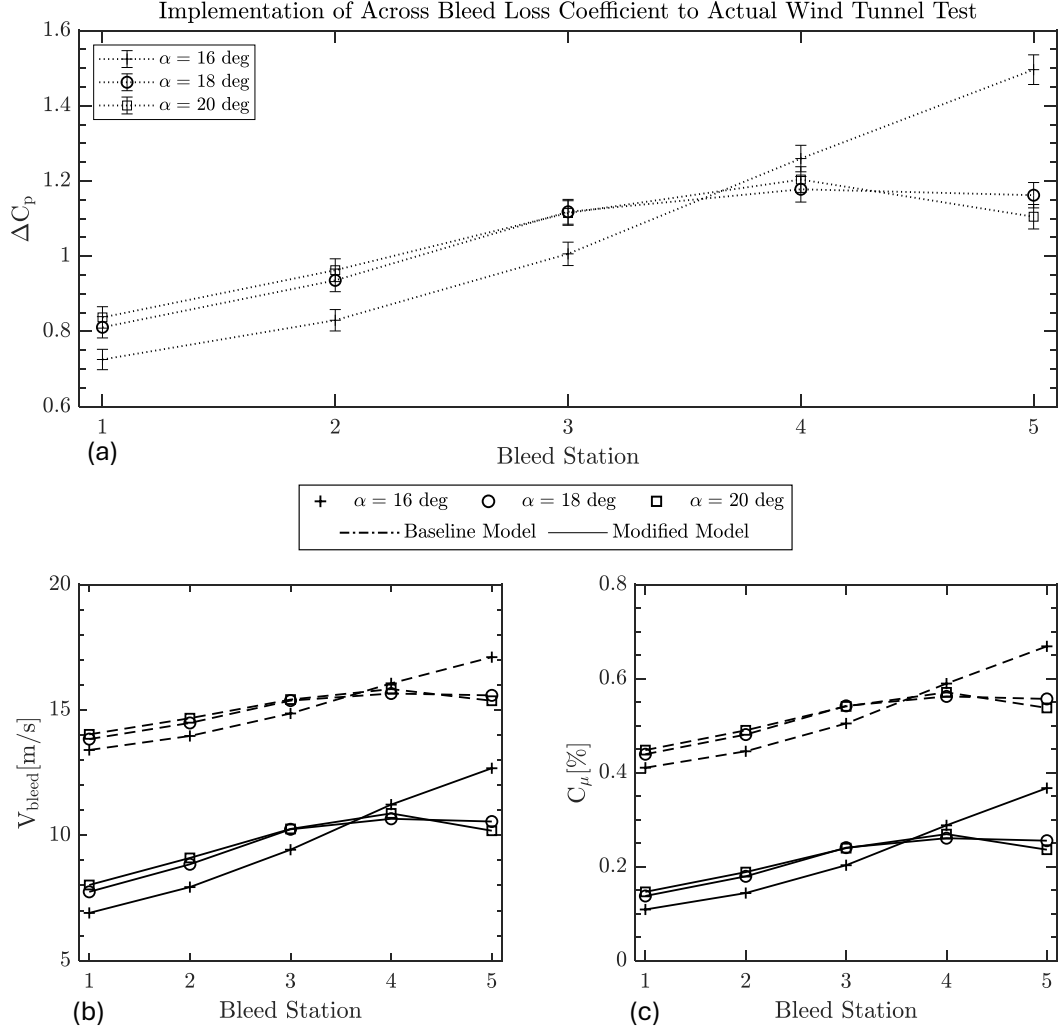
Figure 4.4: Implementation of the presented method to actual wind tunnel tests at \text{Re} = 1.1 \times 10^5 and \alpha = 16^\circ , \alpha = 18^\circ , \alpha = 20^\circ : (a) Pressure difference across the bleed slots 1–5, (b) Estimated bleed velocity V_{\text{bleed}} , baseline model, and modified model using the extended Bernoulli equation with k_{\text{across}} \sim 1.8 , (c) Corresponding bleed momentum coefficients.
