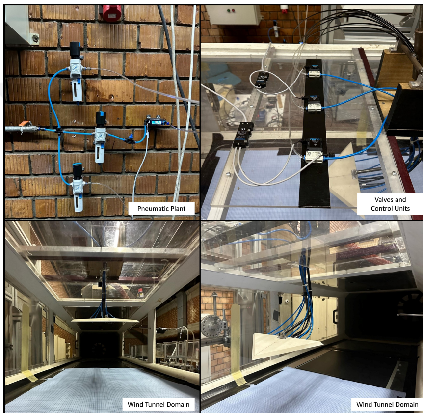
Figure 3.11: Flow control setup: pneumatic plant and wind tunnel domain.
