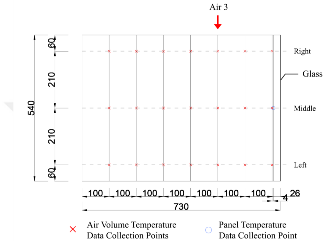
Figure 4.13 Air 3 Layer's Location Plan
