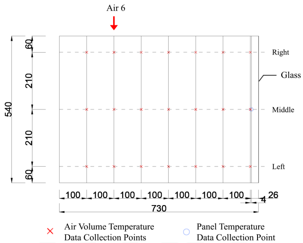
Figure 4.19 Air 6 Layer's Location Plan
