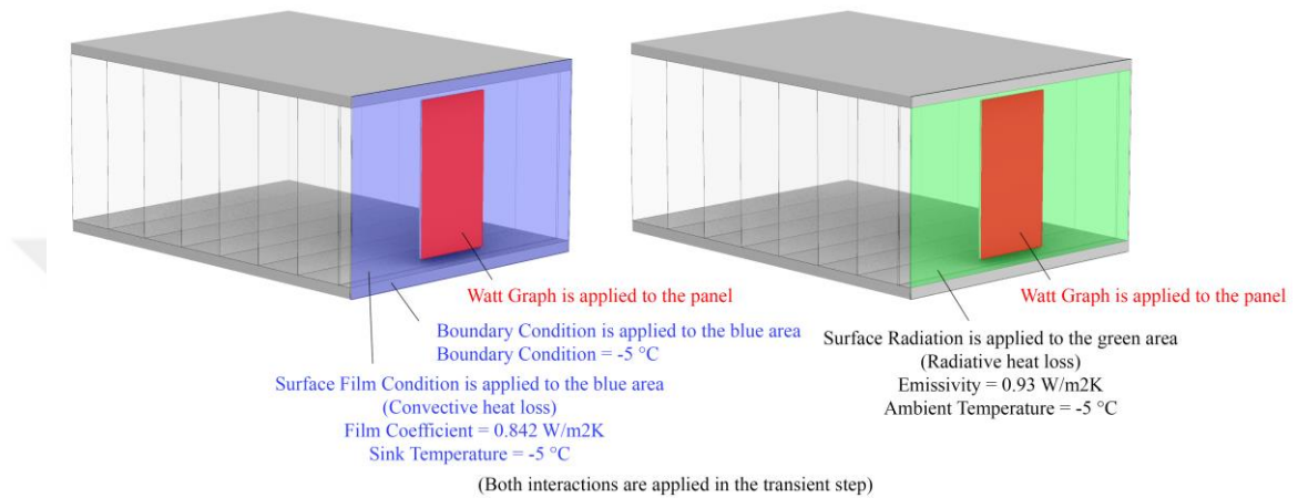
Figure 3.17 The Energy Analysis Interactions (Load (applied to red plane), Boundary Condition (applied to blue plane), Surface Film Condition (applied to blue plane), Surface Radiation (applied to green plane) )
