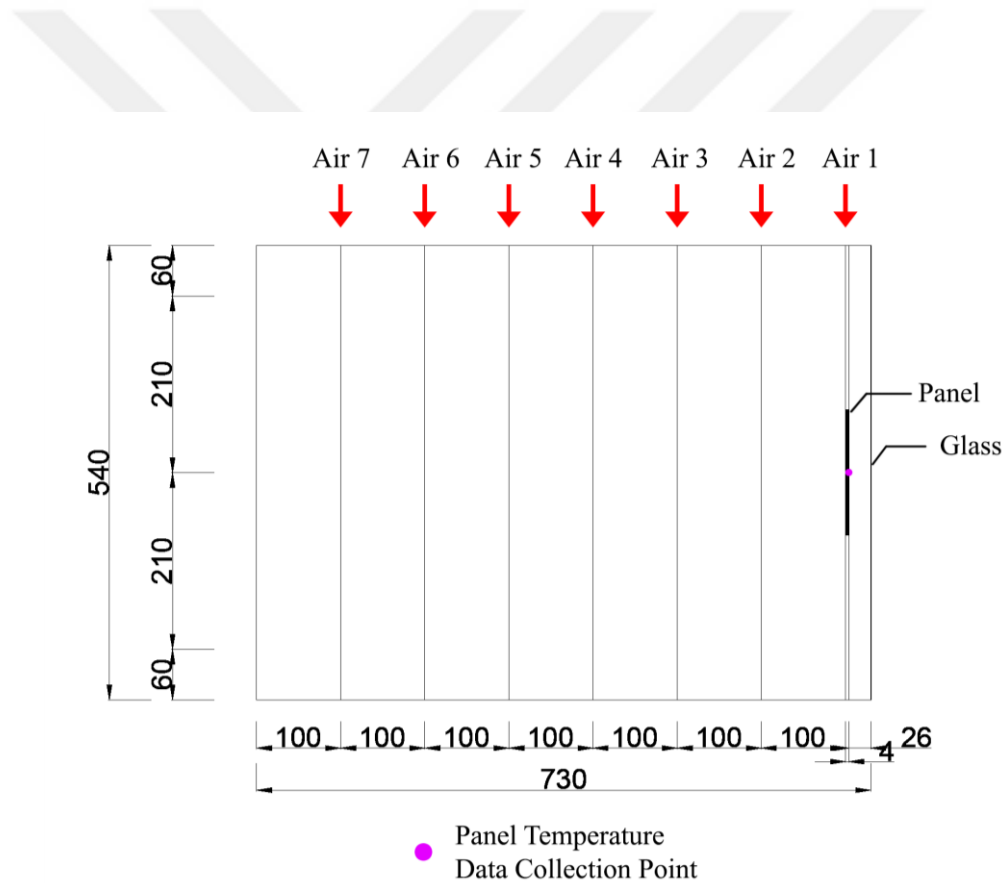
Figure 4.23 Panel Temperature Data Collection Point Plan
