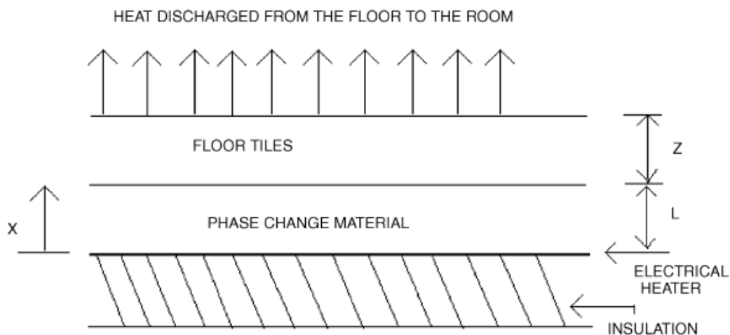
Figure 2.4 Section of the PCM applied electrical floor heating system used for computer simulation (Farid & Chen, 1999)
