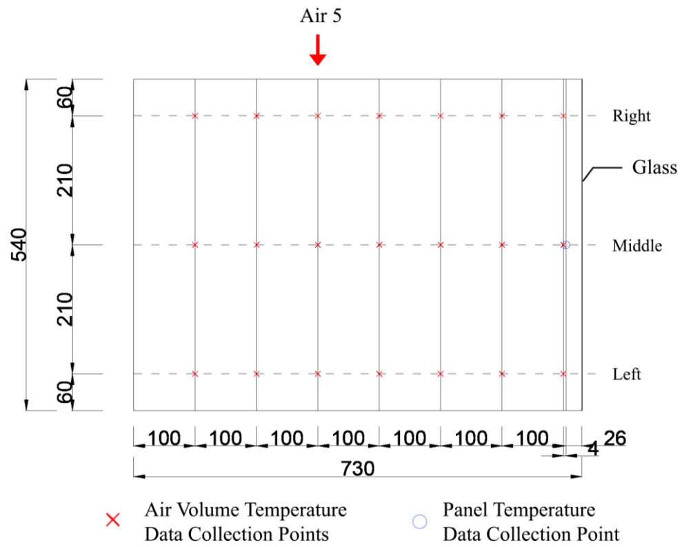
Figure 4.17 Air 5 Layer's Location Plan
