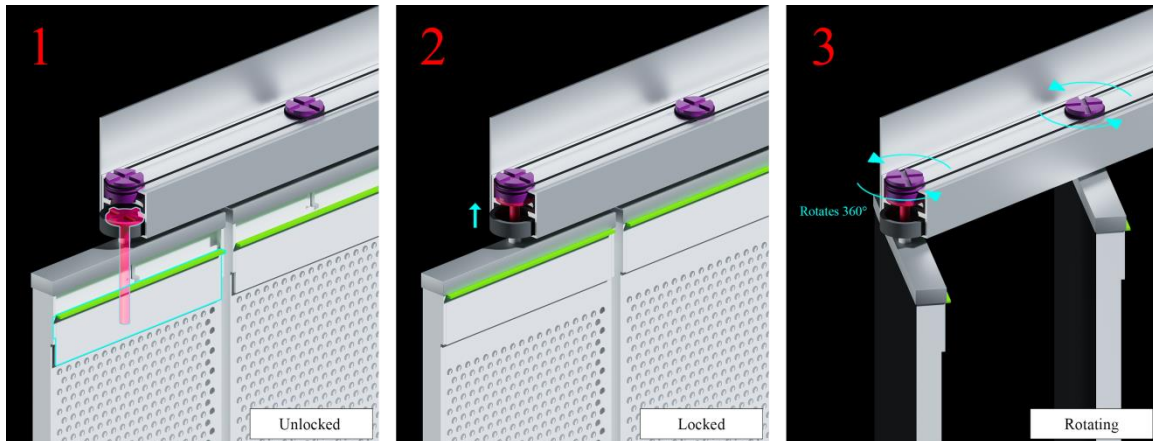
Figure 3.5 Suntracking Mechanism
