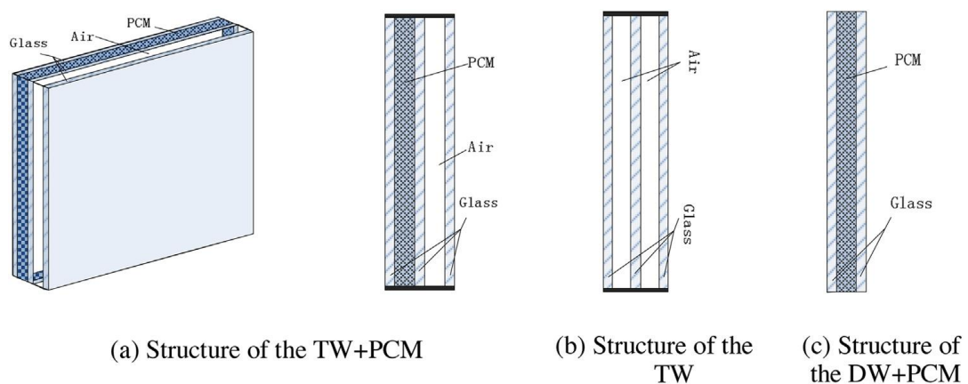
Figure 2.3 Structure comparison of three different kinds of windows, TW(Triple Pane Window), DW (Double Pane Window) (Li et al., 2016)
