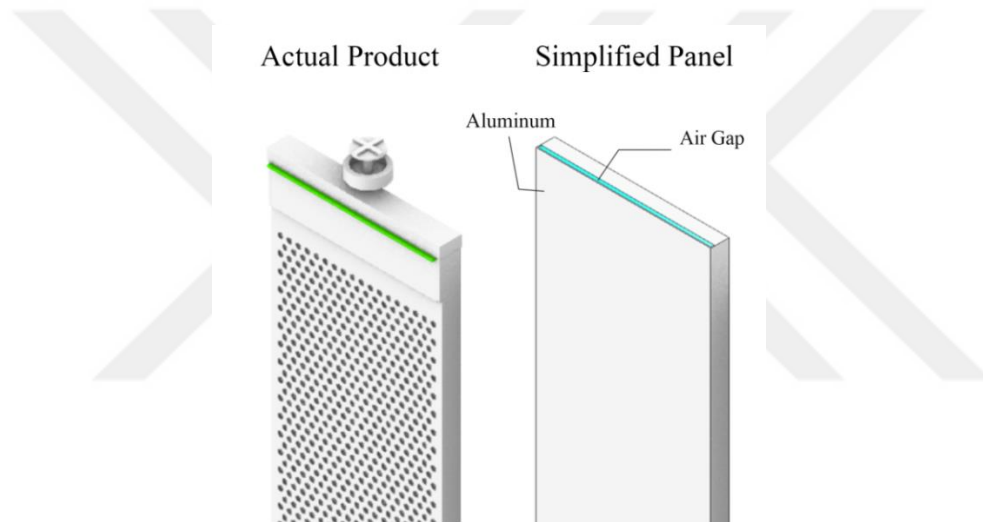
Figure 3.11 Actual Product and Simplified Panel are shown to represent the perforated surface and its simplified version as a flat aluminum surface enclosure that has an air gap inside
