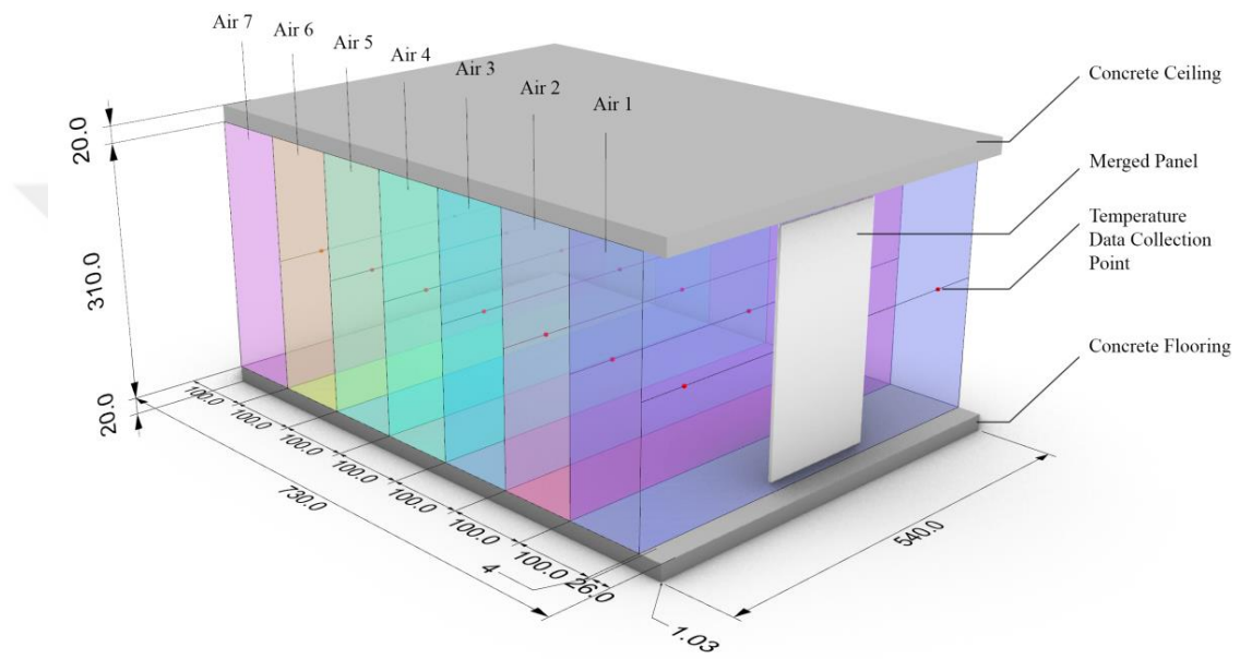
Figure 3.13 The Energy Analysis Model, Panel is shown with white, Indoor air volume is divided to 7 parts of 1 meter air volumes (dimensions are in cm)
