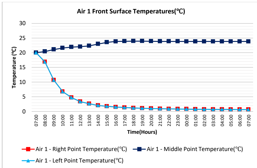
Figure 4.10 Air 1 Front Surface Temperatures(°C)
