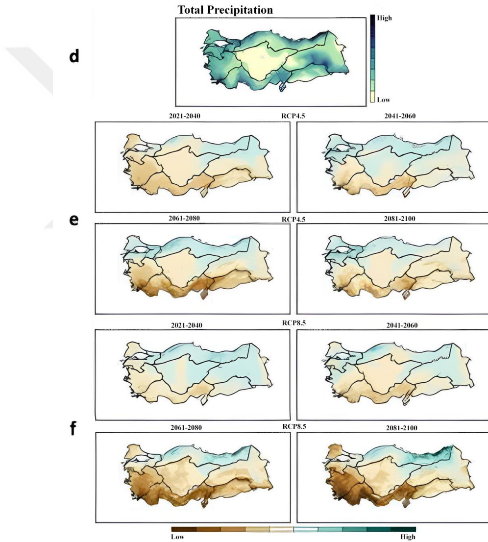
Figure 3.2. Total Precipitation (d) in the Reference Period with Changes in RCP4.5 Scenario (e) and RCP8.5 Scenario (f)
