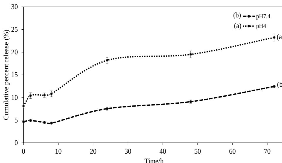
Figure 3.14 Cumulative release of DOX from GO in PBS at pH values (a) 4, (b) 7.4. at 37°C for 72 h. The values given are the mean \pm SD and (n = 3).
