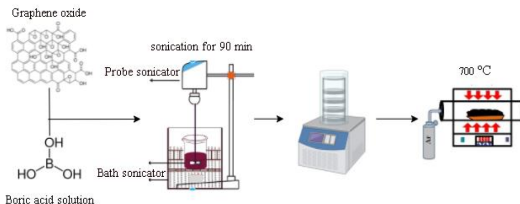
Figure 2.4 B-GO synthesis flow diagram.
