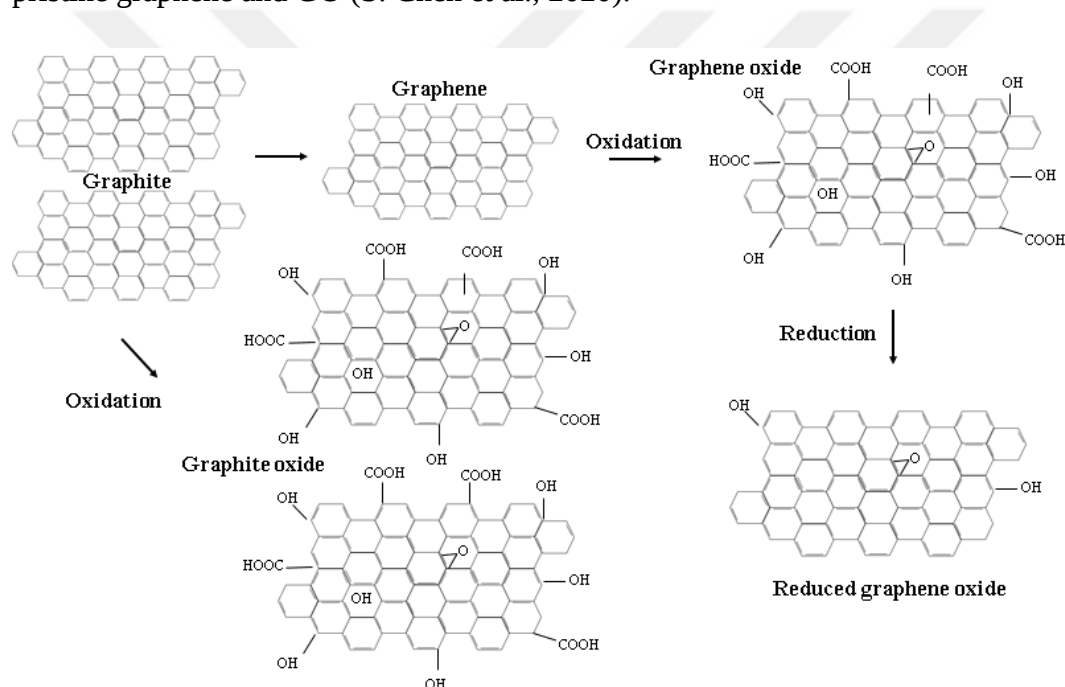
Figure 1.2 Structure of graphite, graphite oxide, graphene and its derivatives.
