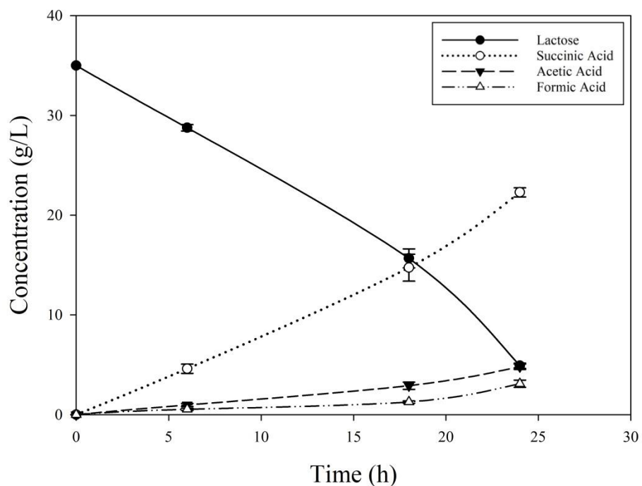
Figure 4.13 Substrate consumption and organic acid accumulation profile of batch immobilized cell fermentation with lactose as carbon source
