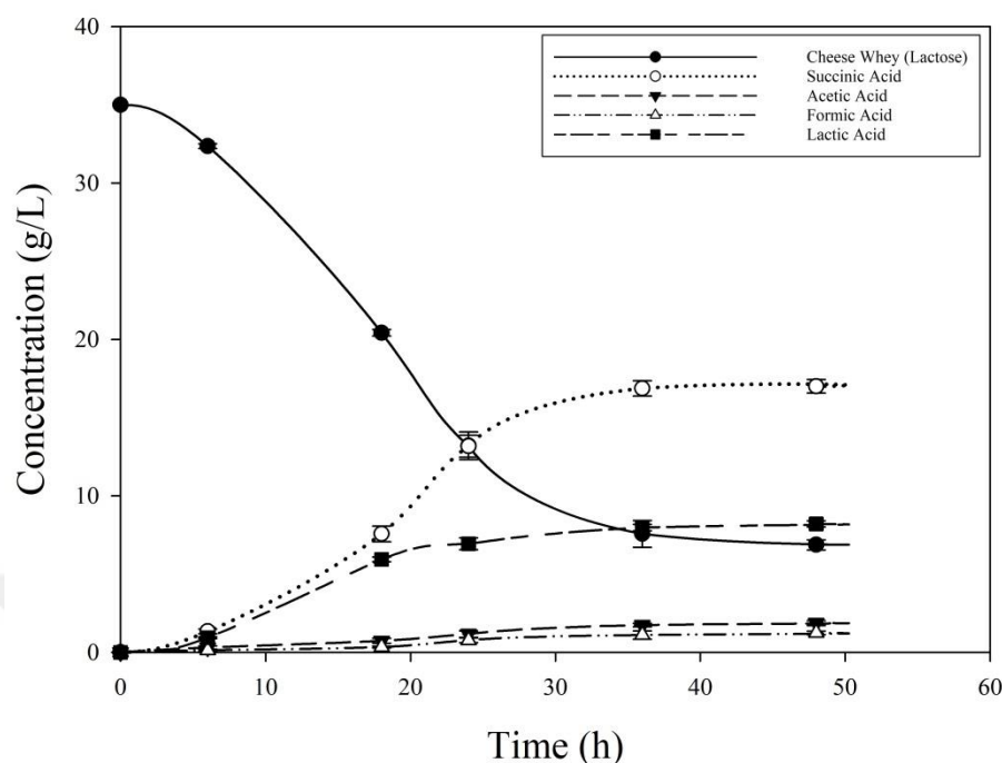
Figure 4.3 Substrate consumption and organic acid production results for shake flask fermentations using cheese whey (lactose) as carbon source
