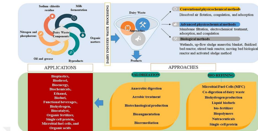
Figure 2.2 Overall scheme of dairy waste valorization applications (Kumar Awasthi et al., 2022)
