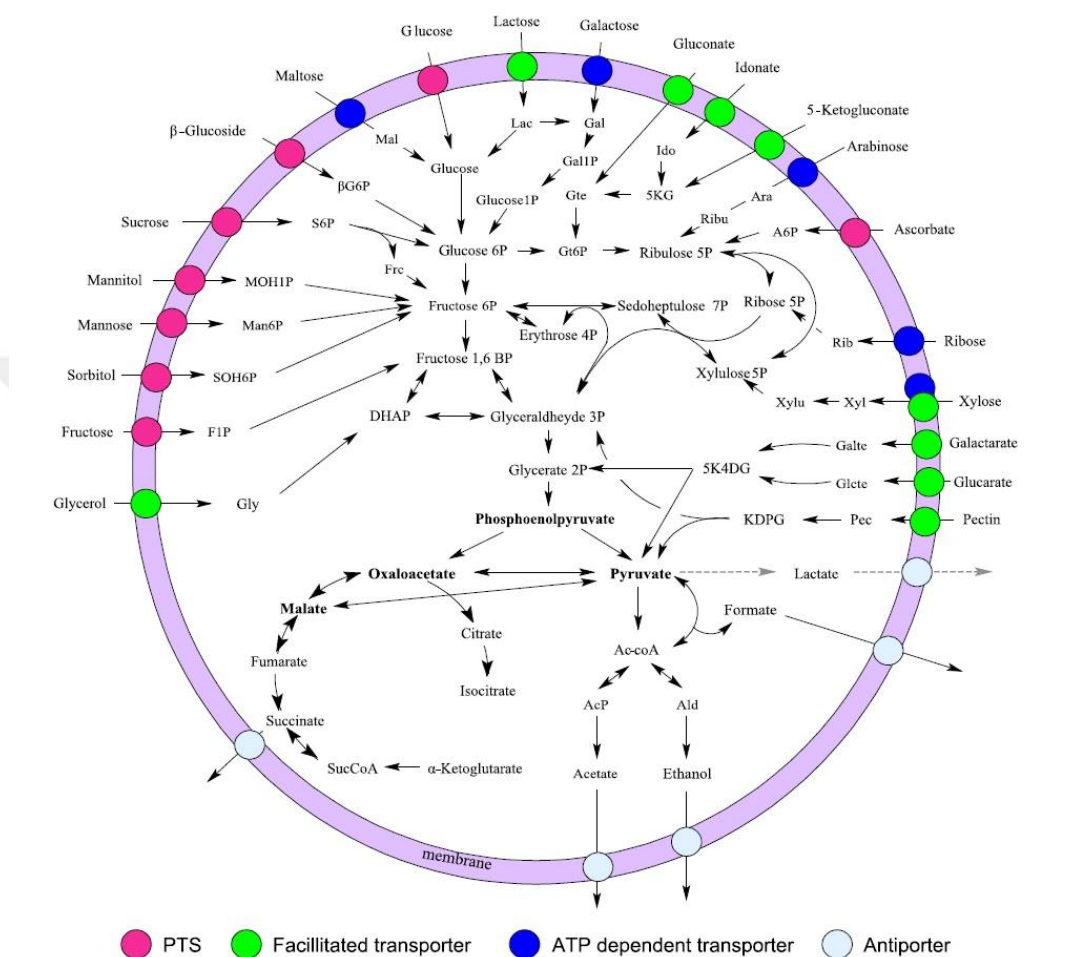
Figure 2.8 Metabolic pathways and possible sugar transporters of Actinobacillus succinogenes . (5K4DG: 5-dehydro-4-deoxy-D-glucarate; 5KG: 5-ketogluconate; A6P: Ascorbate-6-phosphate; AcCoA: Acetyl-CoA; AcP: acetyl-phosphate; Ald: Aldehyde; Ara: Arabinose; DHAP: dihydroxyacetone phosphate; E4P: Erythrose-4-phosphate; F1,6P: Fructose-1,6-biphosphate; F1P: Fructose-1-phosphshate; F6P: Fructose-6-phosphate; G1P: Glucose-1-phosphate; Gal: Galactose; Gal1P: Galactose-1-phosphate; Galte: Galactarate; Glc: Glucose; Glcte: Glucarate; Gly: Glycerol; Gt6P: Gluconate-6-phosphate; Gte: Gluconate; Ido:Idonate; KDPG: 2-keto-3-deoxy-6-phosphogluconate; Lac: Lactose; Mal: Maltose; Man6P: Mannose-6-phosphate; MOH1P: Mannitol-1-phosphate; Pec: Pectin; R5P: Ribose-5-phosphate; Rib: Ribose; Ribu: Ribulose; Ru5P: Ribulose-5-phosphate; S6P: Sucrose-6-phosphate; S7P: Sedoheptulose-7-phosphate; SOH6P: Sorbitol-6-phosphate; SucCoA: Succinyl-CoA; Xu5P: Xylulose-5-phosphate; Xyl: Xylose; Xylu: Xylulose; \beta G6P: \beta -Glucoside-6-phosphate.) (Pateraki et al., 2016)
