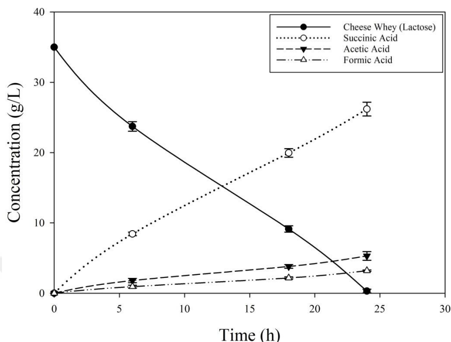
Figure 4.14 Substrate consumption and organic acid accumulation profile of batch immobilized cell fermentation with cheese whey as carbon source
