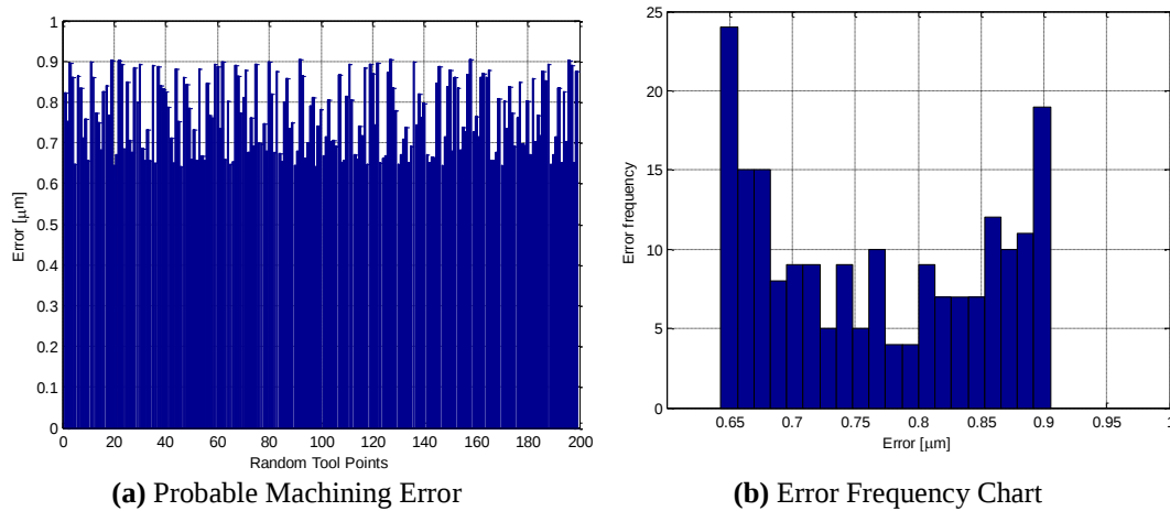
Figure 5.29. Simulation Results for Surface E1 - Part 5
