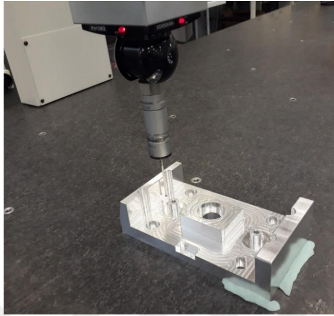
Figure 6.12. Measurement of a test part
