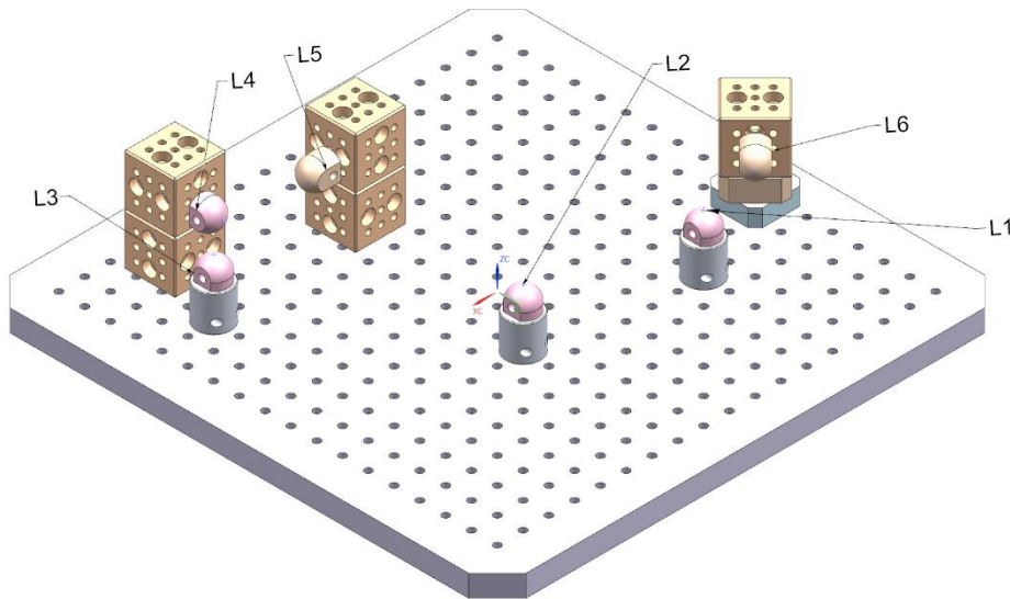
Figure 5.8. Locator Configuration – without Part 2
