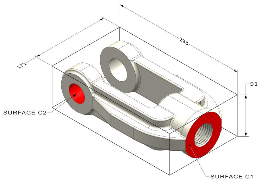
Figure 5.13. Suspension Fork
