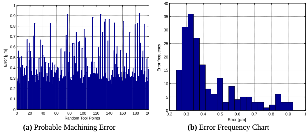
Figure 5.24. Simulation Results for Surface D2 - Part 4
