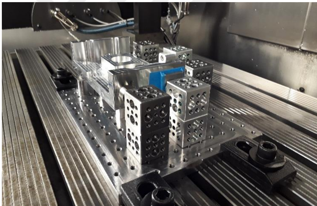
Figure 6.6. Loaded (semi-finished) workpiece to the Cubefix
