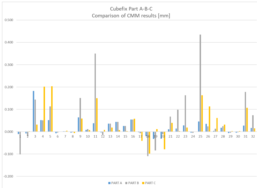
Figure 6.14. CMM results for all the test parts
