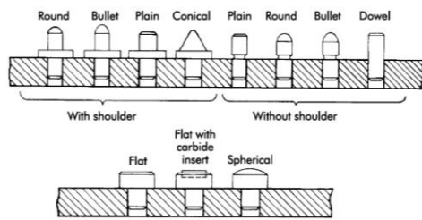
Figure 2.7. Locating Pins [43]
