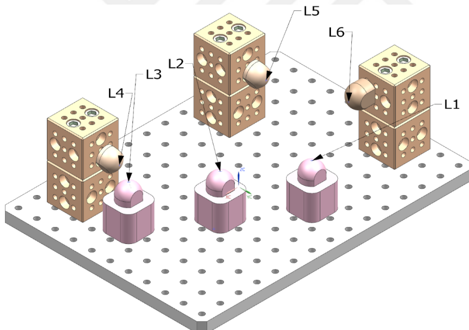
Figure 5.36. Locator configuration for under-constrained case
