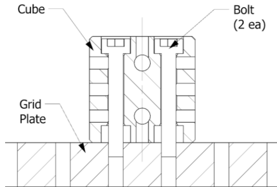
Figure 3.4. Section view of the cube and grid plate
