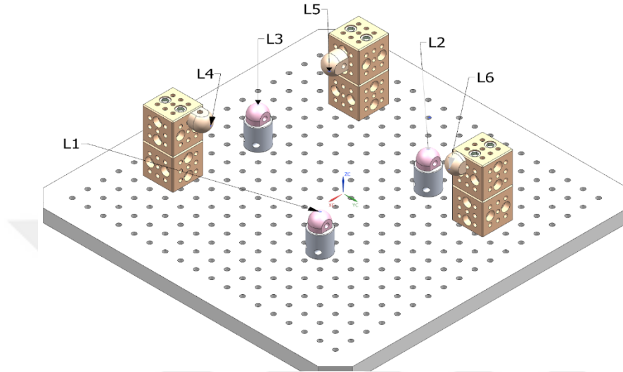
Figure 5.20. Locator Configuration – without Part 4
