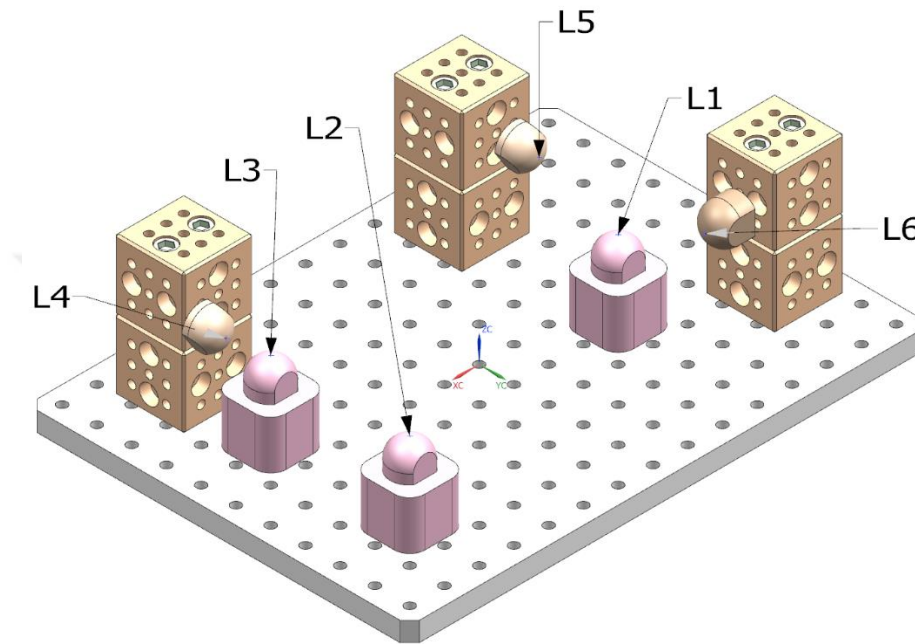
Figure 5.32. Locator Configuration – without Part 6
