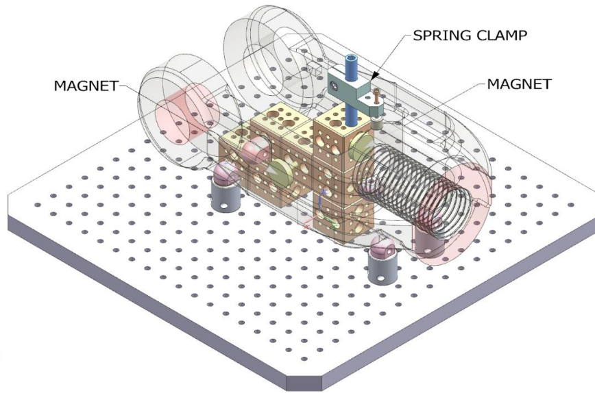
Figure 5.16. Full fixture configuration – Part 3
