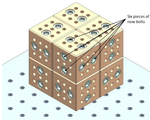
Figure 3.10. New Cube element fixed by 6 bolts
