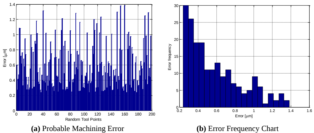
Figure 5.35. Simulation Results for Part 6
