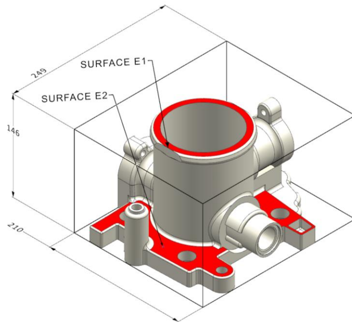
Figure 5.25. Throttle Body
