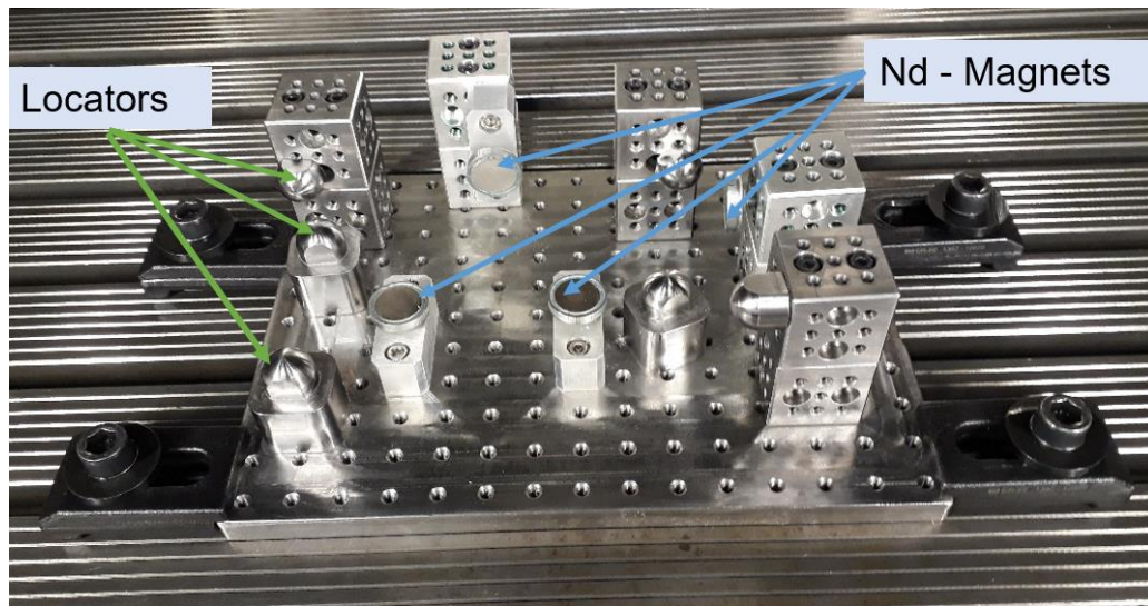
Figure 6.5. Cubefix arrangement
