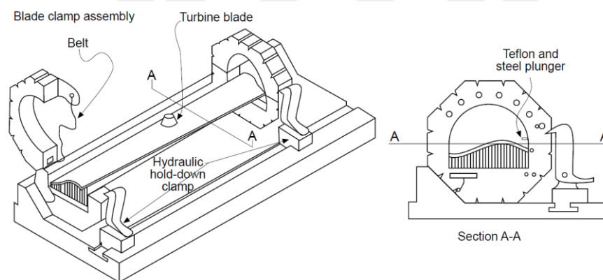
Figure 2.3. A flexible fixture system for turbine blades [45]
