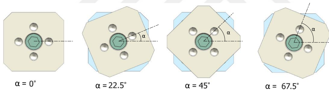
Figure 3.16. Angular positions of Index Adjuster
