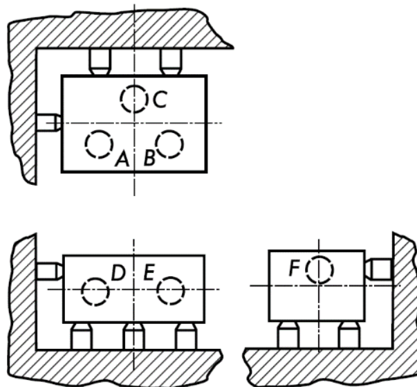
Figure 1.4. Six point locating ( 3-2-1 ) method [43]
