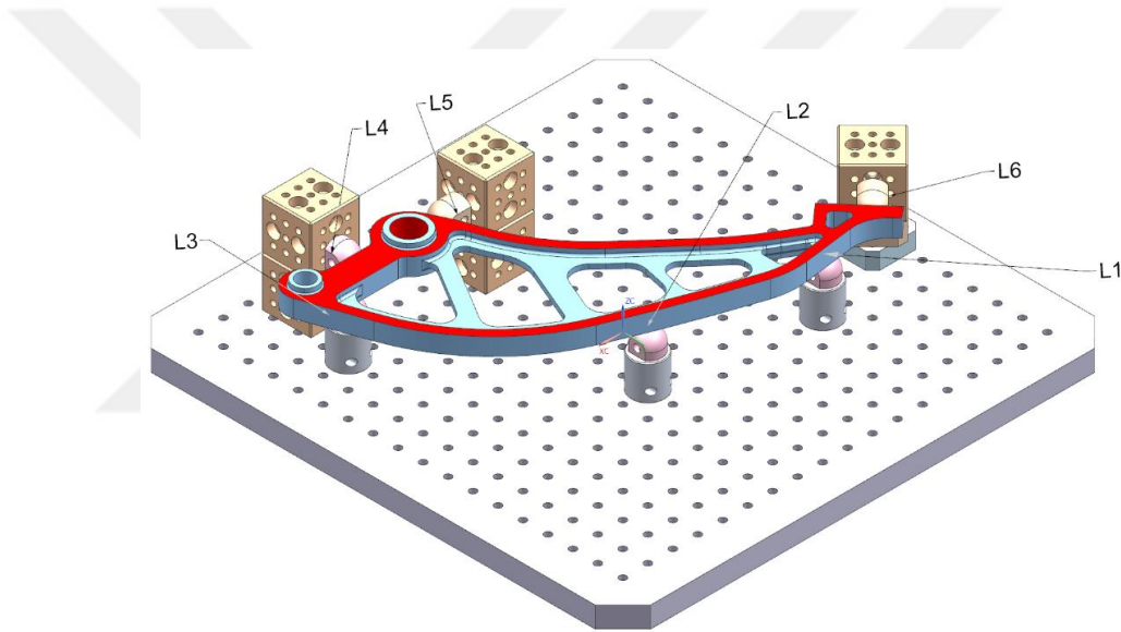
Figure 5.9. Locator Configuration for Part 2
