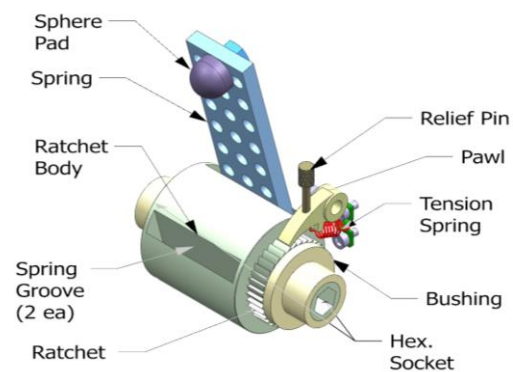
Figure 3.26. Ratchet Clamp attached to a Cube Figure 3.27. Inner structure of the ratchet clamp
