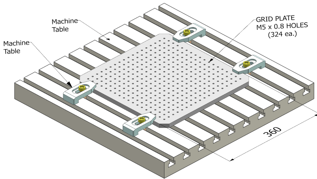
Figure 3.1. Grid Plate Loaded on the Machine Table
