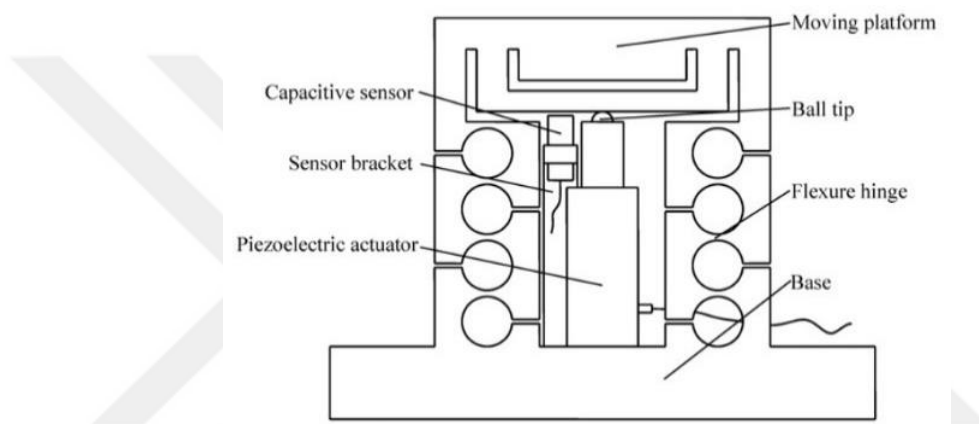
Figure 2.2. Mechanism for an ultraprecise system [24]
