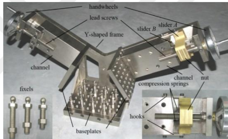
Figure 2.1. A Fixture study [10]
