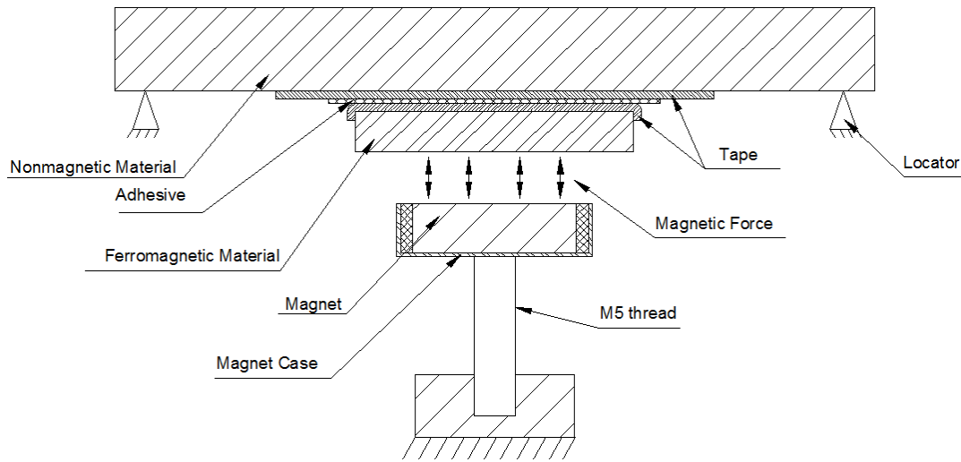
Figure 3.31. Magnetic Clamping Method for Nonmagnetic Materials
