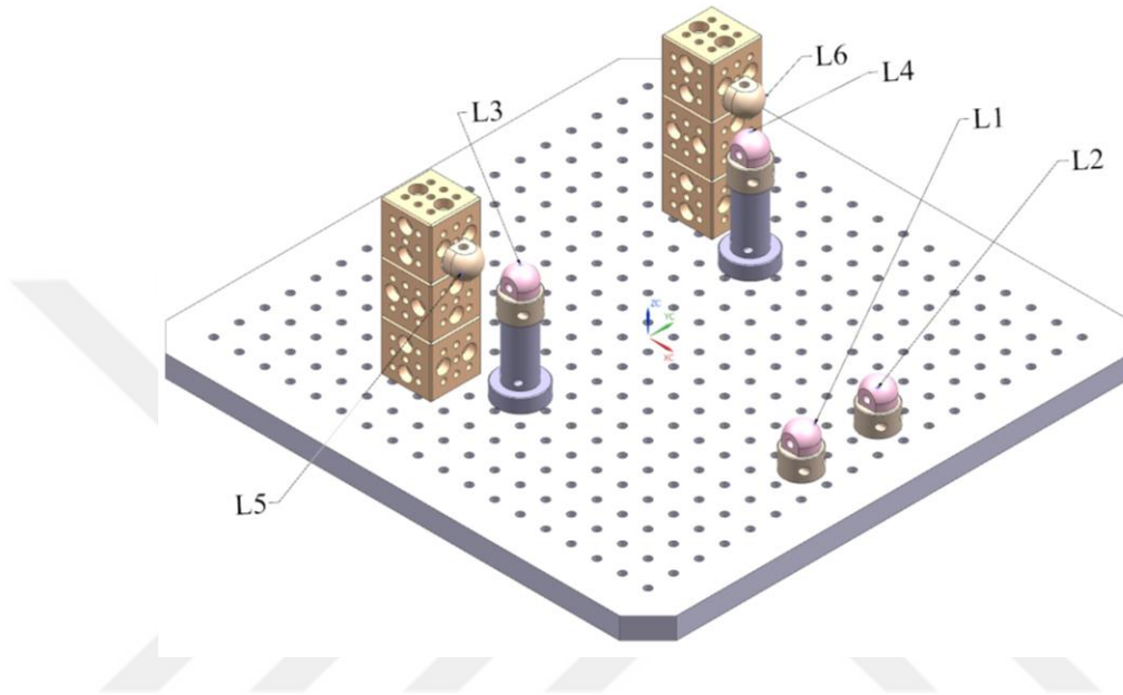
Figure 5.2. Locator Configuration – without Part 1
