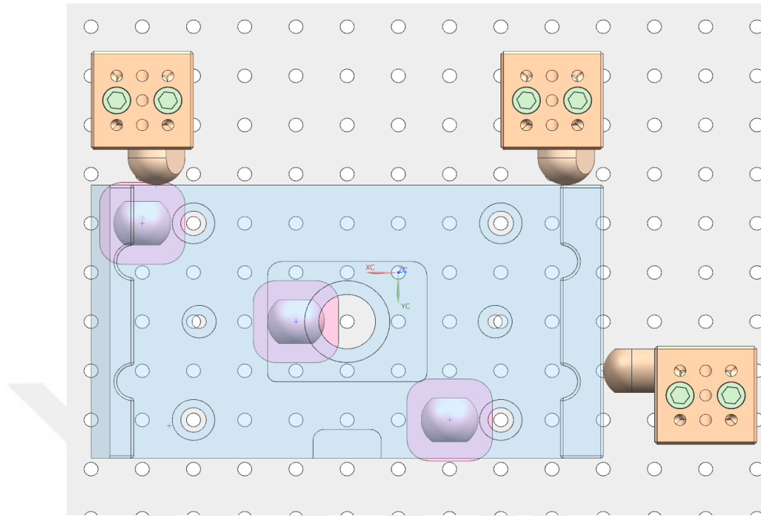
Figure 5.37. Under-Constraint locator configuration for Part 6 - Top view
