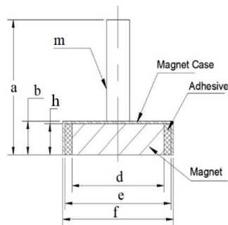
Figure 3.28. Section view of magnets
