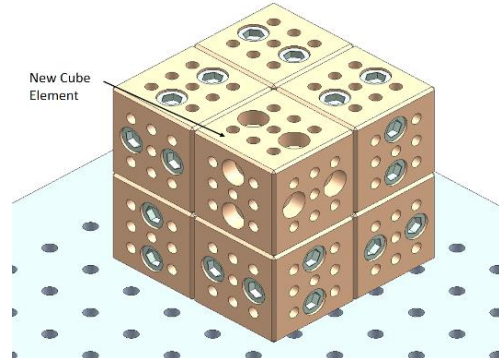
Figure 3.9. Placement of new cube element
