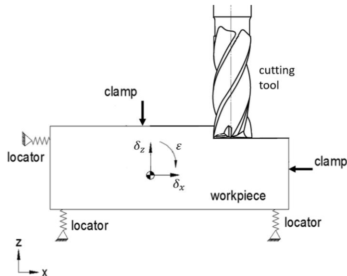
Figure 1.5. Forces acting on workpiece during machining
