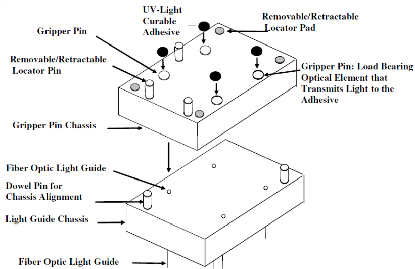
Figure 2.12. Light Activated Adhesive Gripper Method [33]
