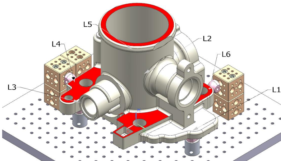
Figure 5.27. Locator Configuration for Part 5
