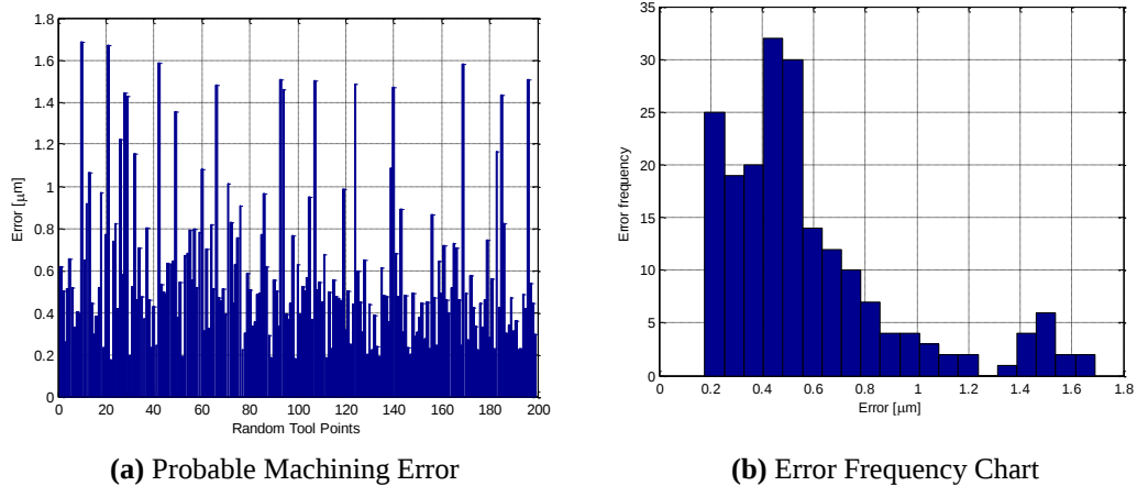
Figure 5.23. Simulation Results for Surface D1 - Part 4
