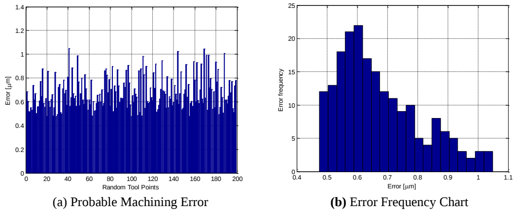
Figure 5.6. Simulation Results for Surface A2 - Part 1
