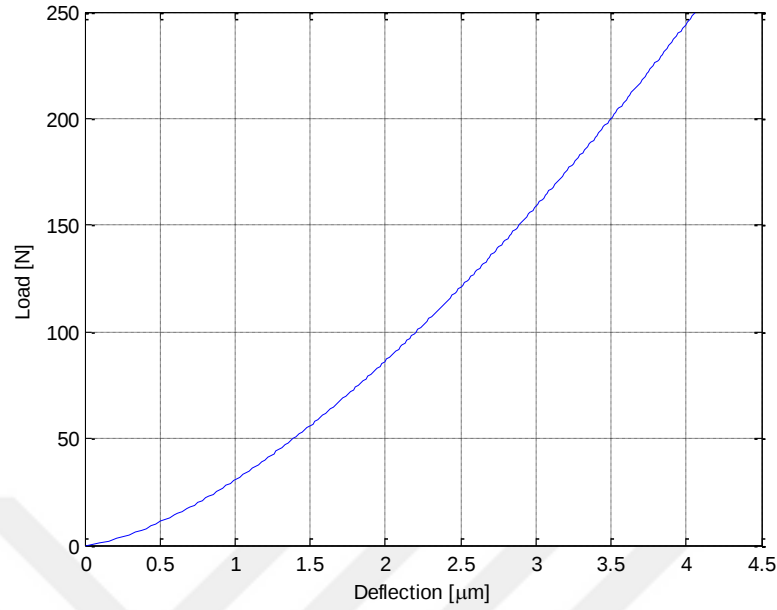
Figure 4.5. Locators deflection with respect to the load.
