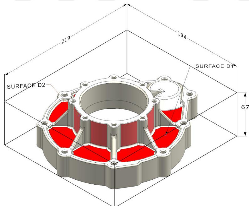
Figure 5.19. Gearbox Casing
