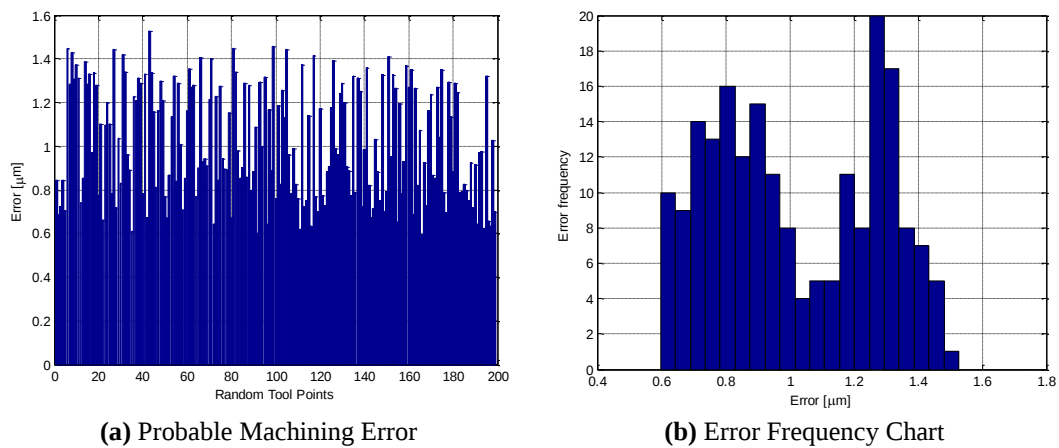
Figure 5.5. Simulation Results for Surface A1 - Part 1
