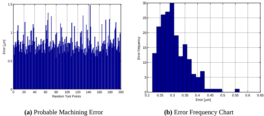
Figure 5.17. Simulation Results for Surface C1 – Part 3
