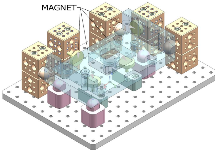
Figure 5.34. Full fixture configuration – Part 6
