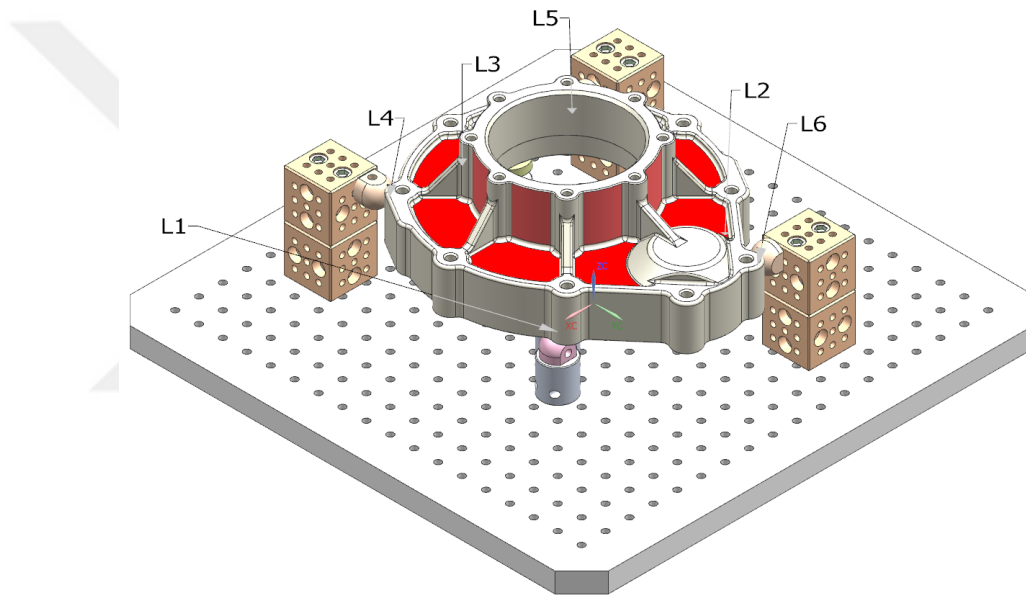
Figure 5.21. Locator Configuration for Part 4
