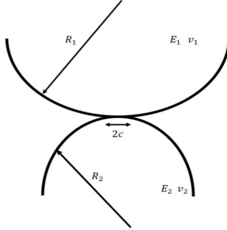
Figure 4.4. Elastic bodies in contact.
