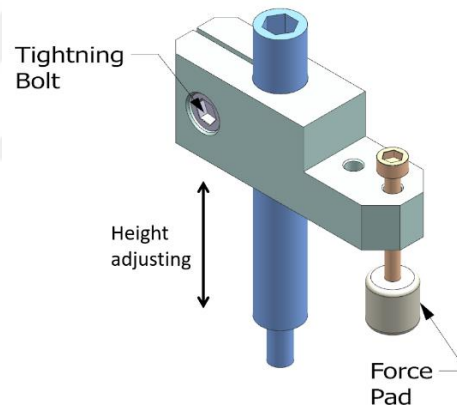
Figure 3.25. Spring Clamp – Config. B
