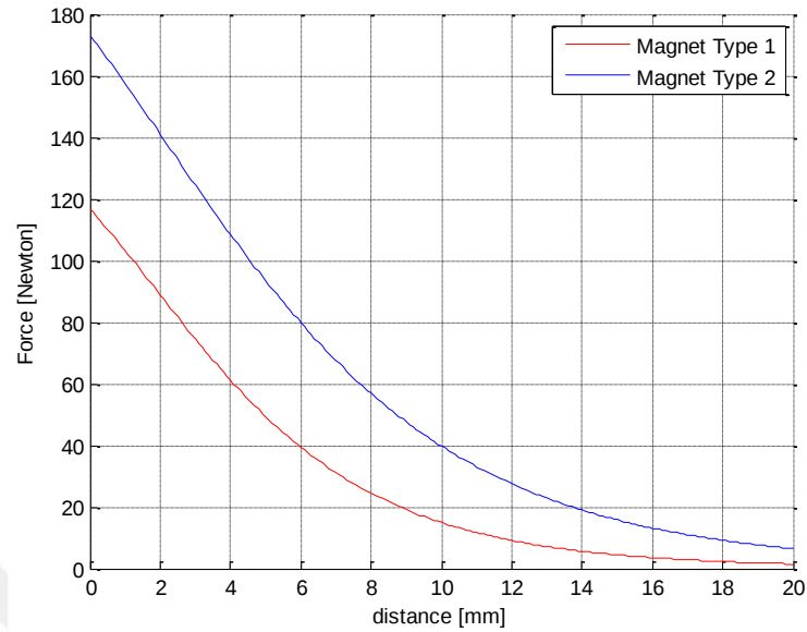
Figure 3.30. Magnetic (reluctance) force variation with respect to the air gap.
