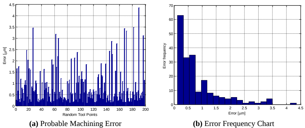
Figure 5.11. Simulation Results for Surface B1 - Part 2
