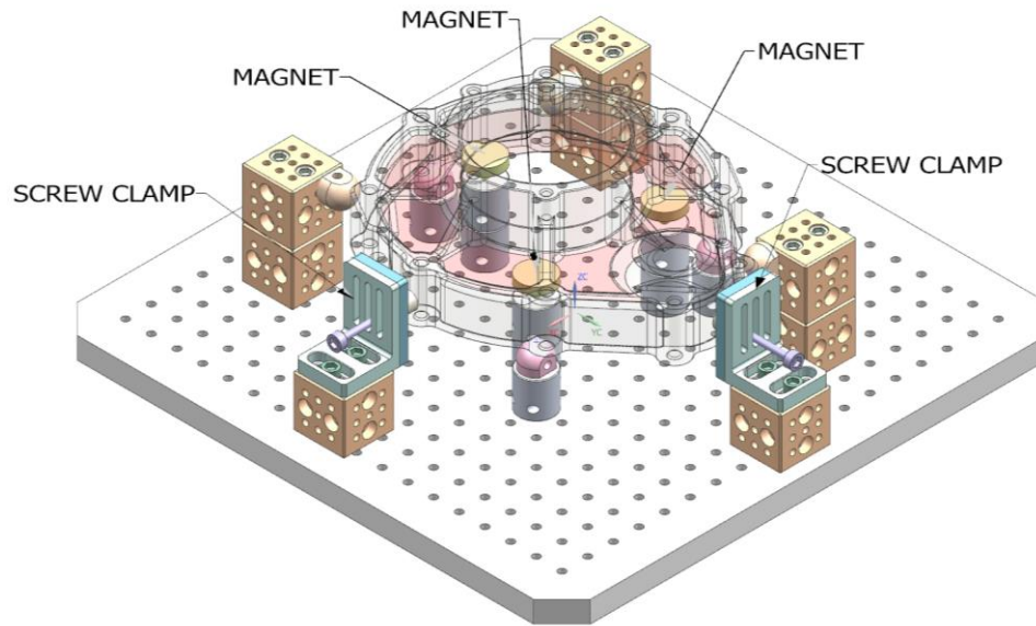
Figure 5.22. Full fixture configuration – Part 4
