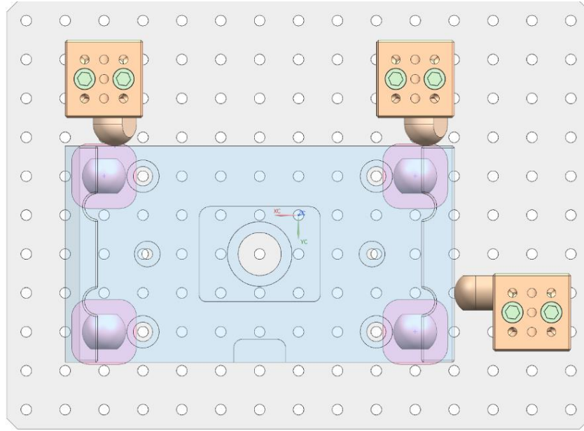
Figure 5.39. Over-Constrained locator configuration for Part 6 – Top view
