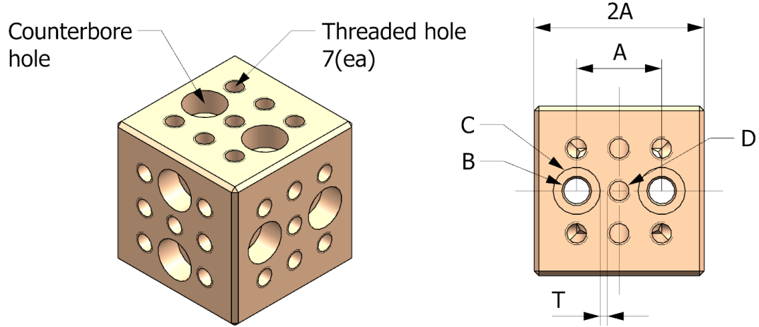
Figure 3.2. Cube element and its parameters
