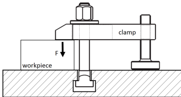
Figure 2.6. Clamp fixing the workpiece
