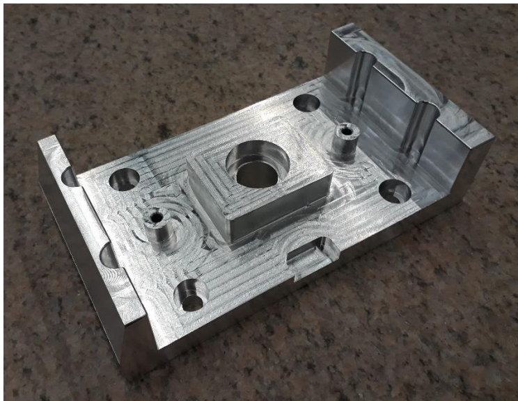
Figure 6.2. Semi-finished part
