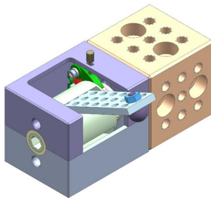
Figure 3.26. Ratchet Clamp attached to a Cube Figure 3.27. Inner structure of the ratchet clamp
