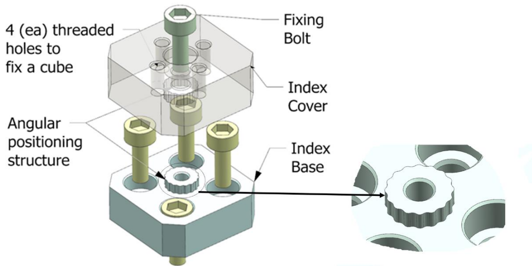
Figure 3.15. Index adjuster exploded view
