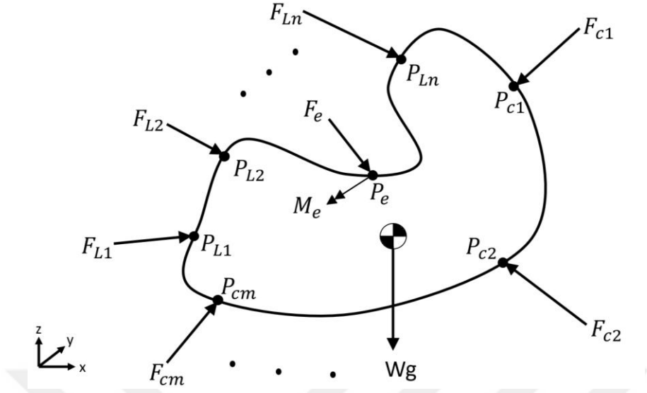
Figure 4.2. Free Body Diagram of a Generic Workpiece.
