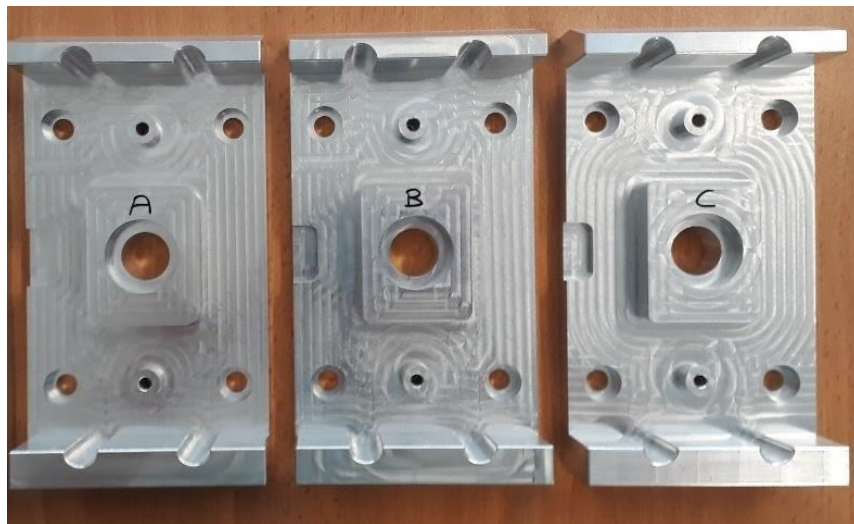
Figure 6.10. Manufactured test parts using Cubefix
