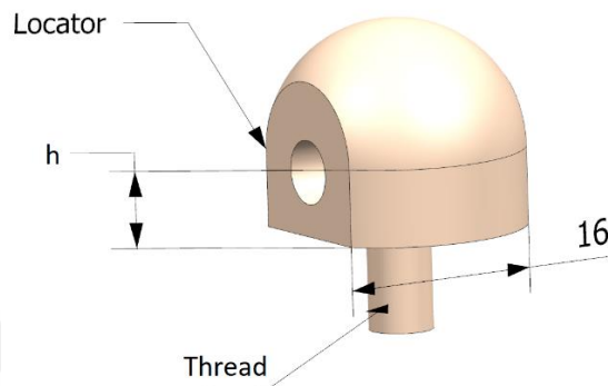
Figure 3.17. Locator
