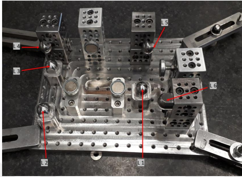
Figure 6.16. Locator numbers
