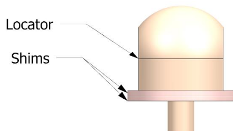
Figure 3.21. Fine tuning the height of the locator
