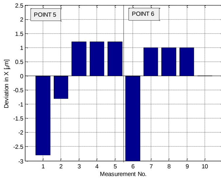
Figure 6.19. Deviation in X axis.
