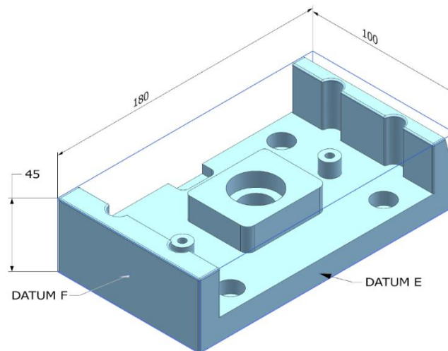
Figure 5.31. Target Piece
