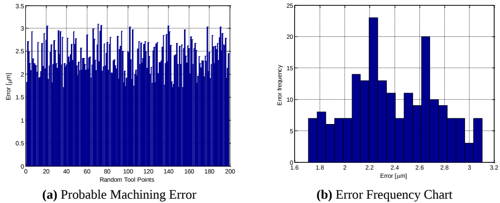
Figure 5.18. Simulation Results for Surface C2 – Part 3
