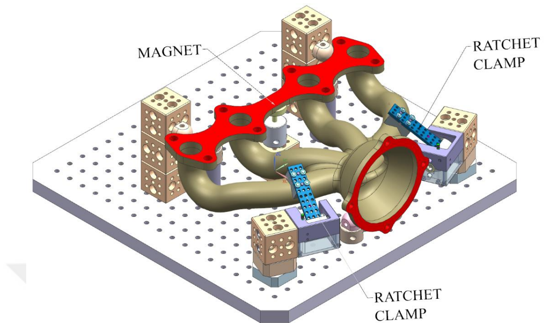
Figure 5.4. Full fixture configuration – Part 1
