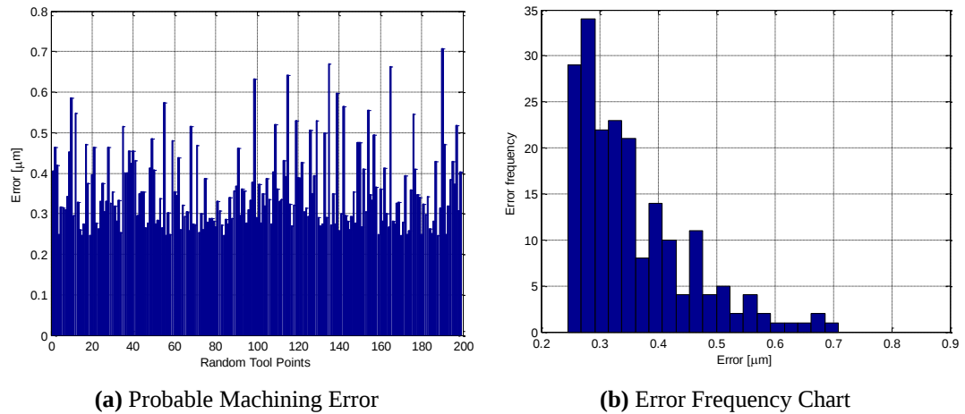
Figure 5.30. Simulation Results for Surface E2 - Part 5
