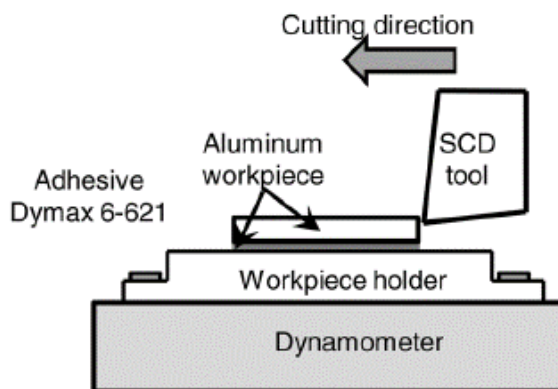
Figure 2.11. Fixturing method [32]
