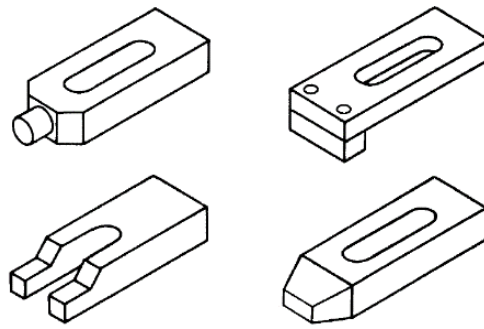
Figure 2.5. Clamps [27]
