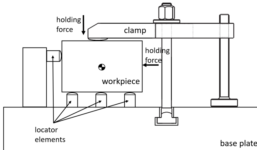
Figure 1.2. Locating of a workpiece
