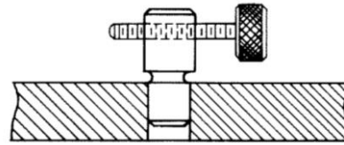
Figure 2.8. Adjustable Locator [43]
