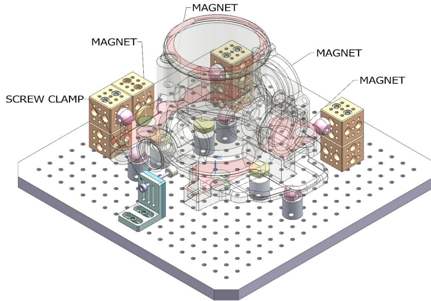
Figure 5.28. Full fixture configuration – Part 5
