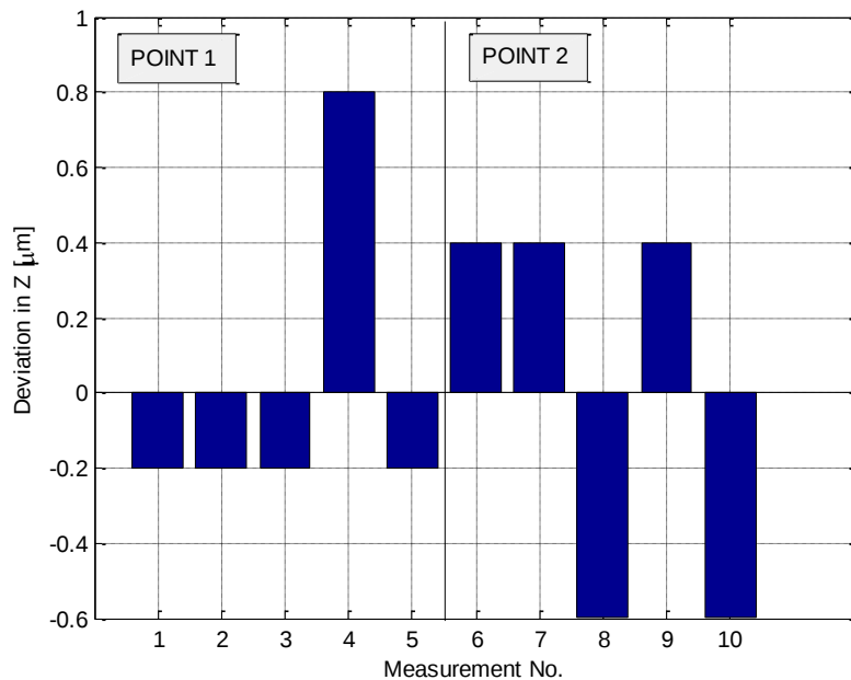
Figure 6.17. Deviation in Z axis.
