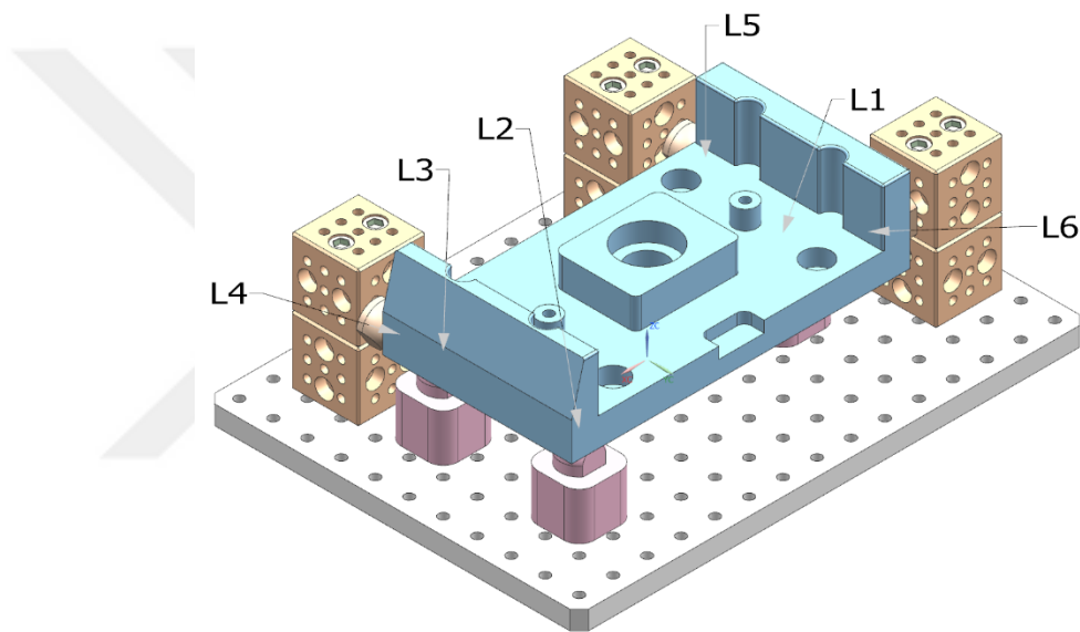
Figure 5.33. Locator Configuration for Part 6
