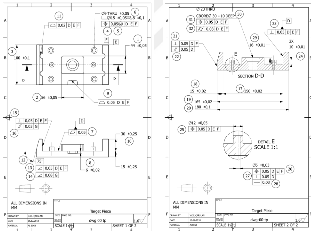
Figure 6.13. Dimensional and geometric tolerances on the test pieces
