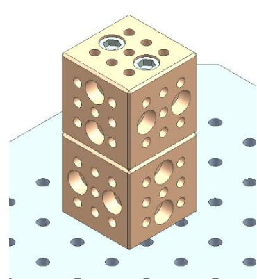
Figure 3.7. Bolts are tightened to fix the cube
