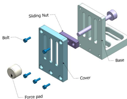
Figure 3.22. Exploded view of Screw Clamp
