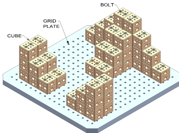
Figure 3.12. A fixture configuration with cubes
