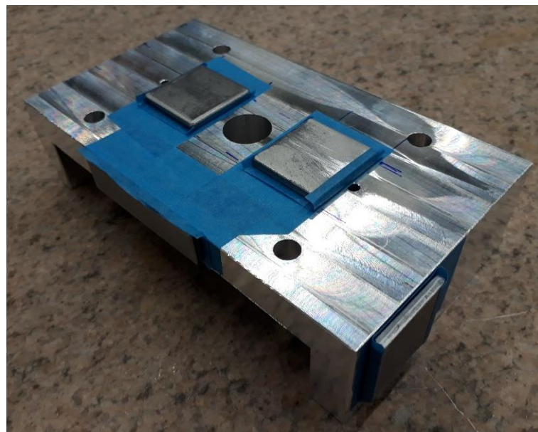
Figure 6.4. Prepared workpiece for finishing operations
