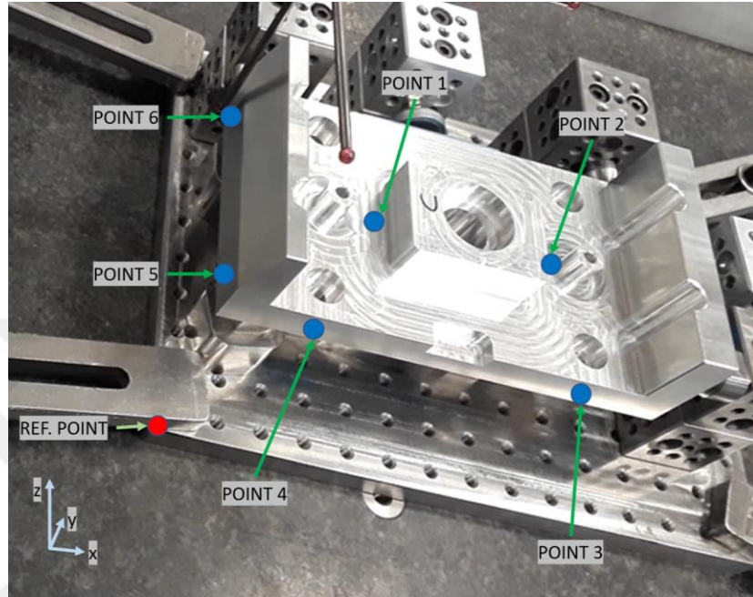
Figure 6.15. Inspected Points at CMM
