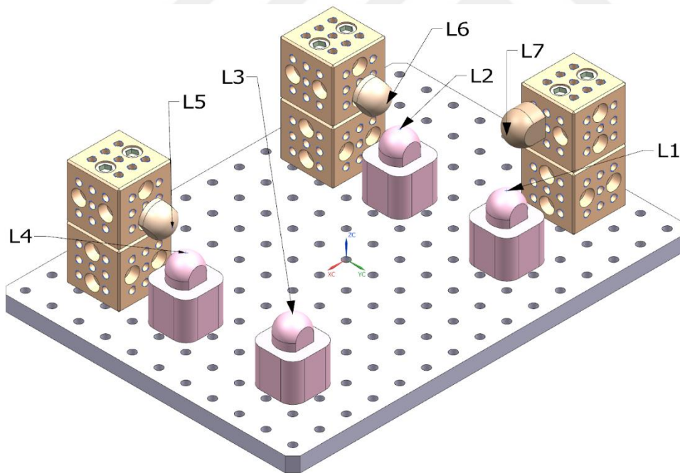
Figure 5.38. Locator configuration for over-constrained case
