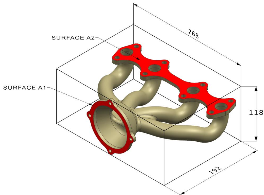
Figure 5.1. Exhaust Manifold
