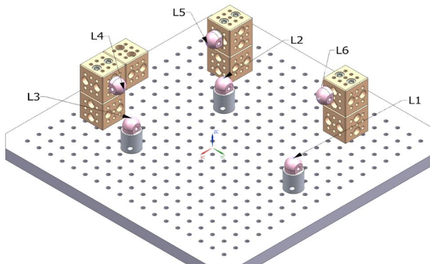
Figure 5.26. Locator Configuration – without Part 5
