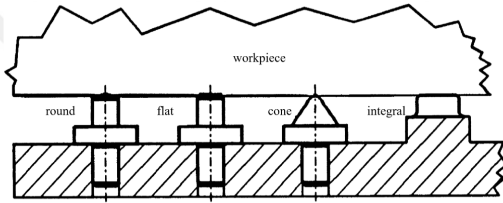
Figure 2.9. Examples for Locators Contacting with Workpiece [42]
