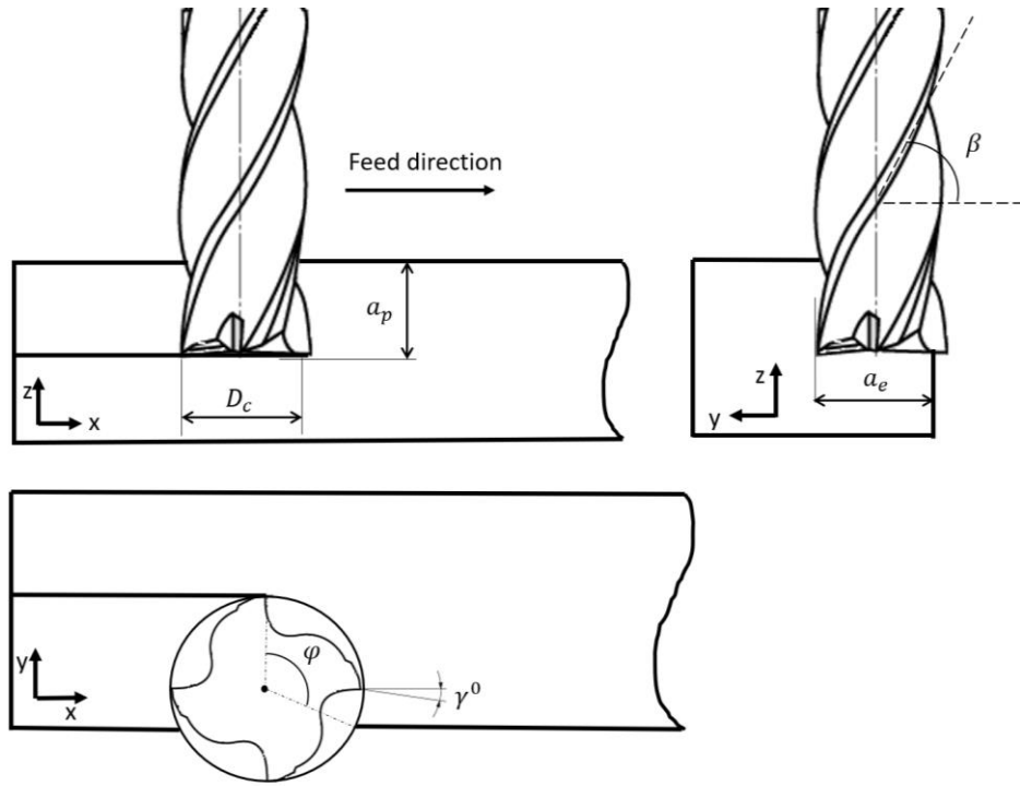
Figure A.1. Basic Parameters of a Generic End-milling Process.
