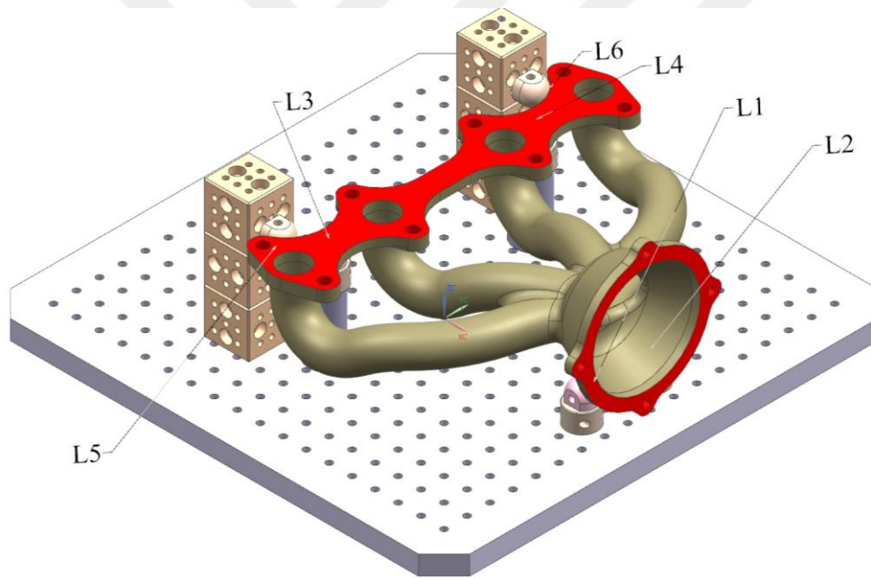
Figure 5.3. Locator configuration for Part 1
