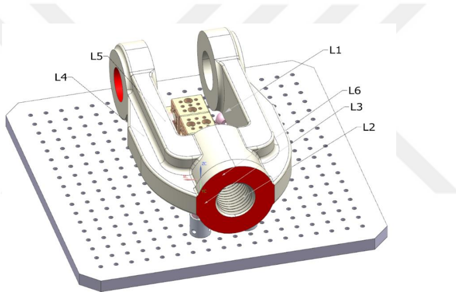
Figure 5.15. Locator Configuration for Part 3
