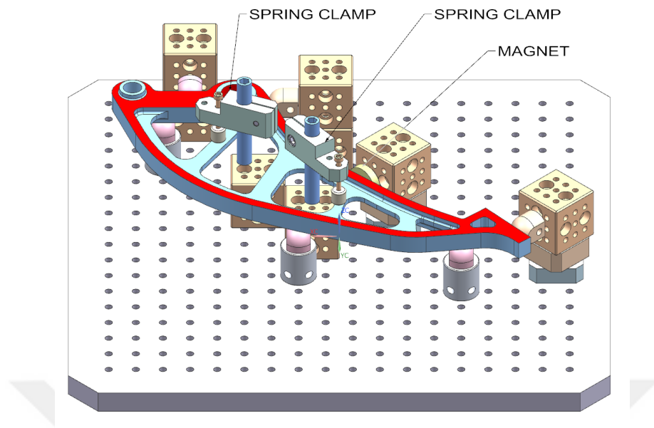
Figure 5.10. Full fixture configuration – Part 2
