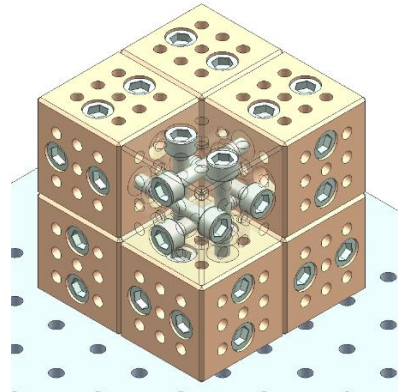
Figure 3.11. Fastening with 6 bolts
