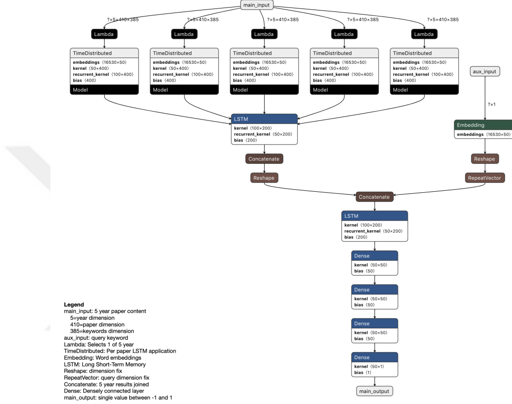
Figure 4.6: Model 4: The model includes Paper LSTM module to generate paper embeddings, LSTM module to generate one-year summary embeddings, and another LSTM module to generate representation over the observation window.
