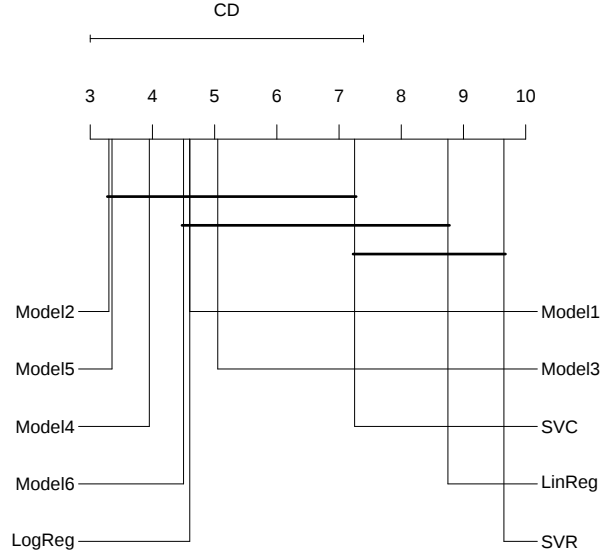
Figure 4.10: Nemenyi post-hoc test result for Label Increase F1 score
