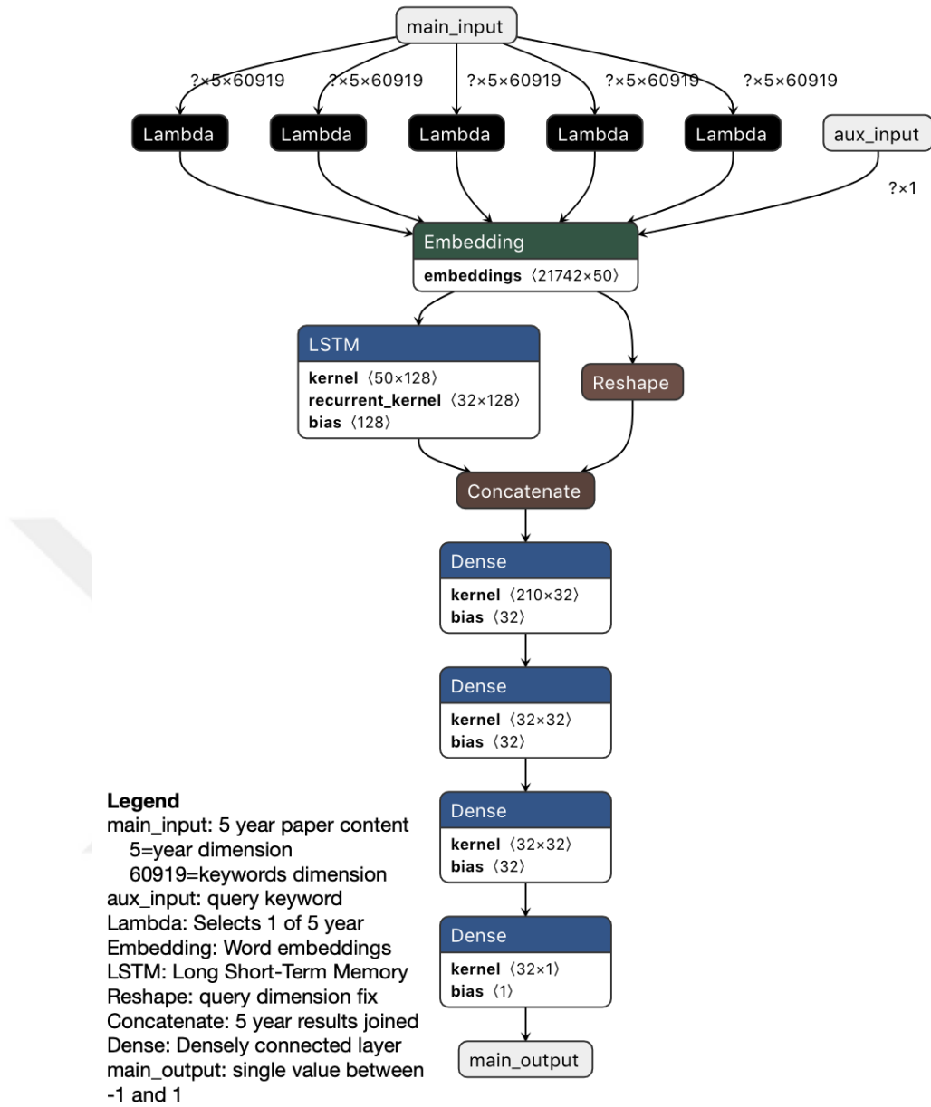
Figure 4.2: Model 1: The architecture includes a shared LSTM module to process paper collections per year, yearly embeddings are concatenated
