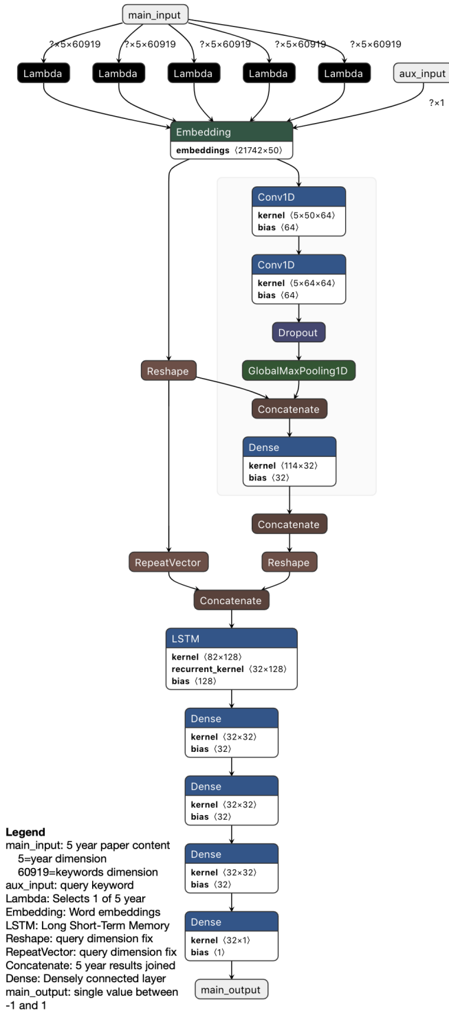
Figure 4.4: Model 3: The architecture includes a Convolution module for each year, it has an LSTM module to process all year results
