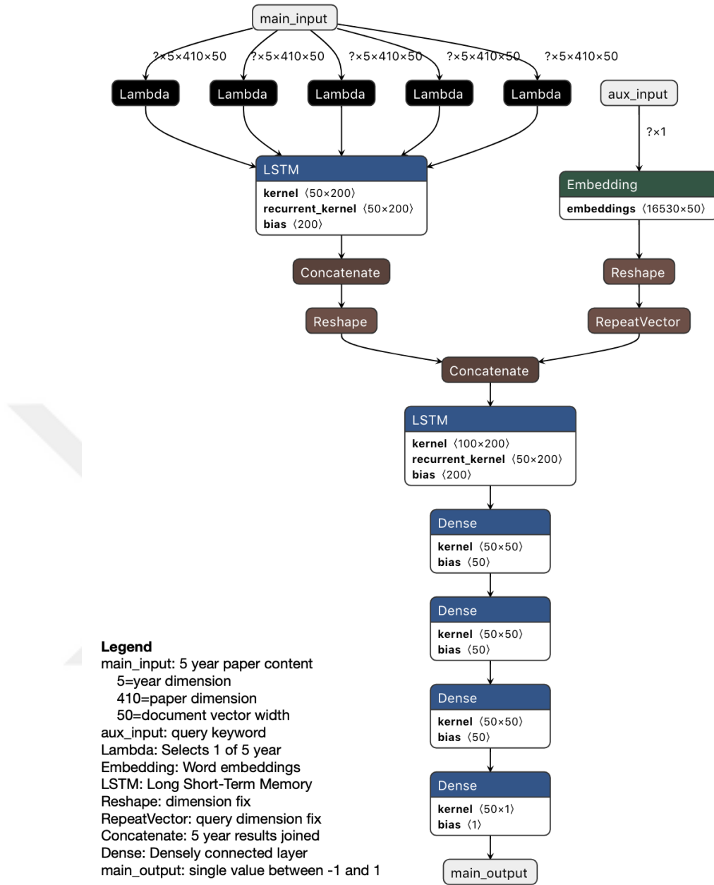
Figure 4.7: Model 5 & 6: The model includes Doc2Vec (in Model 5) or Specter (in Model 6) for each paper, an LSTM module to generate one-year summary representation, an another LSTM module to generate representation over the observation window.
