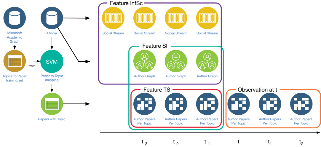
Figure 3.2: Data flow of the features
