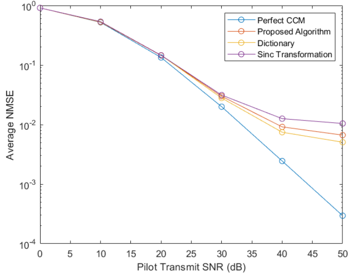
Figure 5.5: Average NMSE values of the MMSE channel estimator for different pilot transmit SNR values
