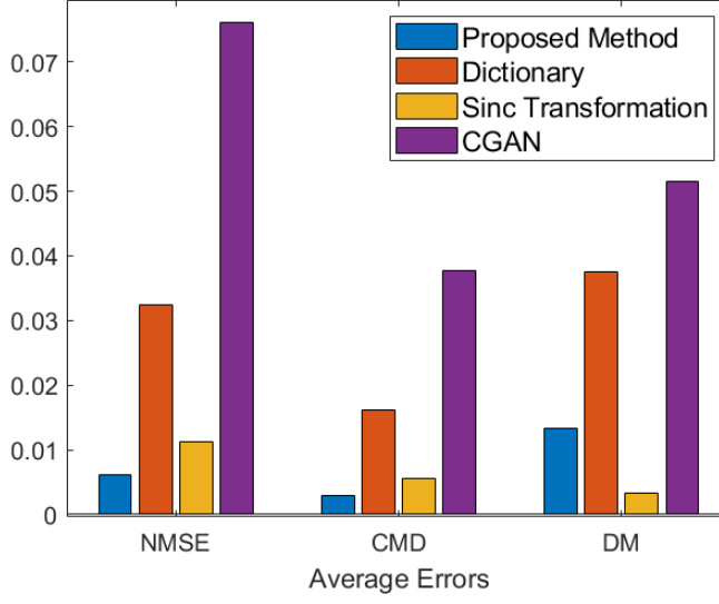
Figure 5.2: Average error values for our method and the benchmark methods for a perfect dataset with CCMs of a M = 256 base station antenna system
