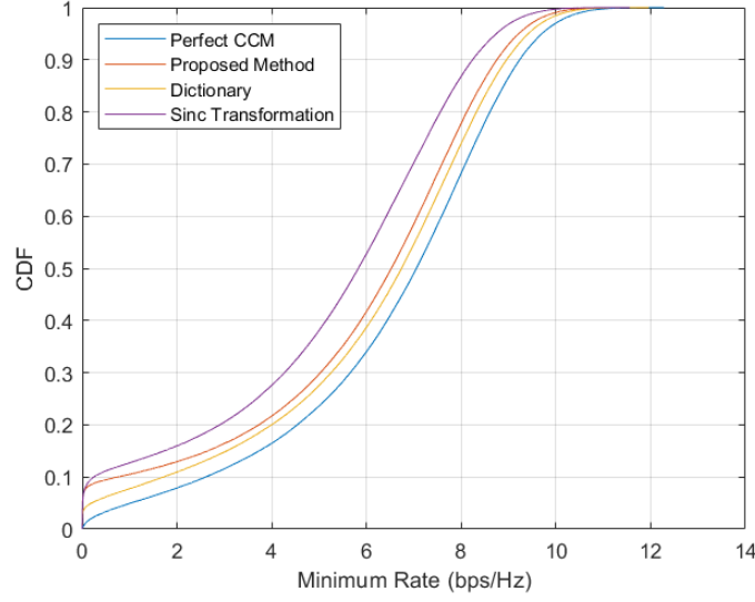
Figure 5.9: Empirical CDF of minimum rate achieved by the SLNR-based beamformer for K = 3 users using \rho = 20 dB transmit SNR value
