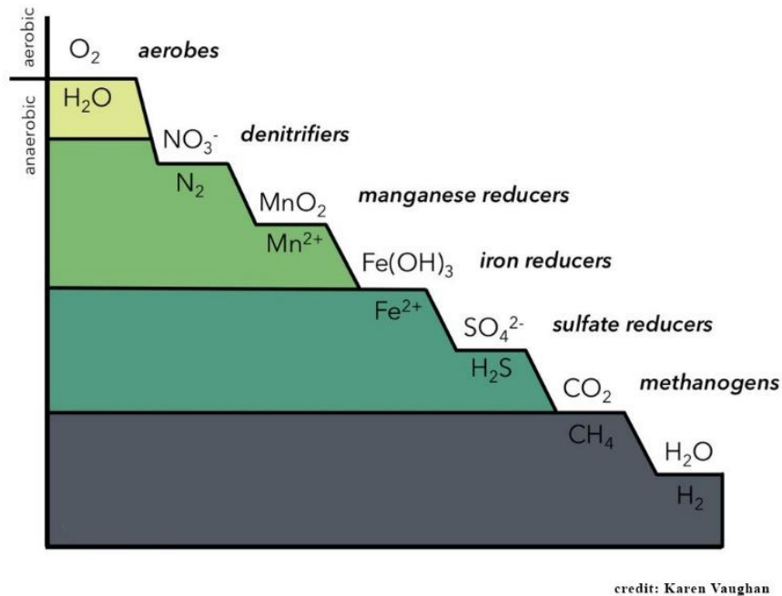
Figure 6. Description of common reduction reactions conducted by microorganisms in marine sediments. The most energetically favorable molecules and reactions are at the top, and the least favorable is at the bottom. Reproduced with permission (Karen Vaughan, personal communication, 2022).
