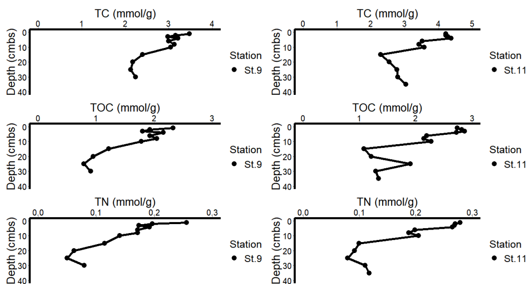
Figure 11. Carbon and Nitrogen measurements from Station 9 and Station 11 according to depth
