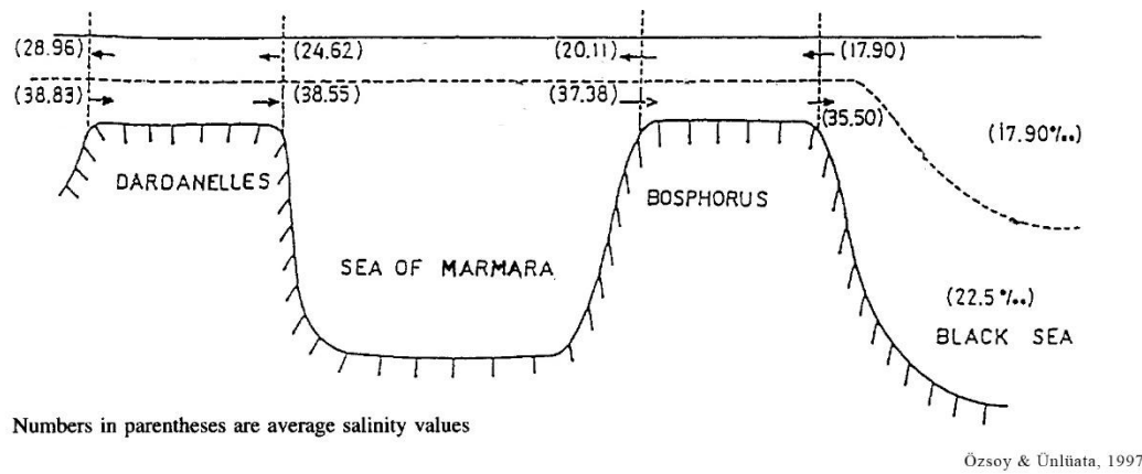
Figure 4. Water fluxes through Bosphorus Strait by Özsoy & Ünlüata, 1997.
