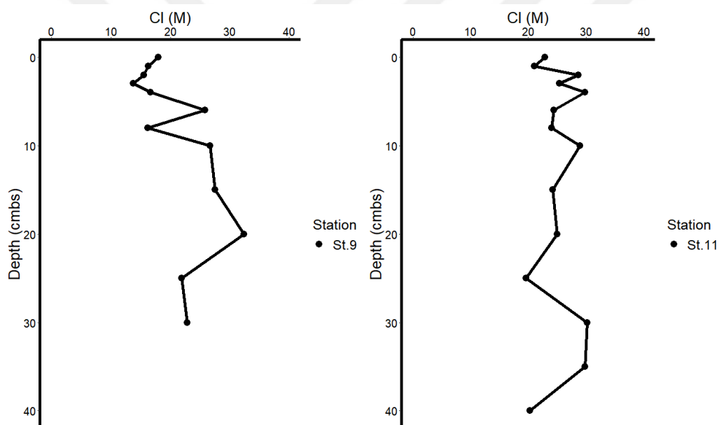
Figure 15. \text{Cl}^- concentrations measured in Station 9 and Station 11 according to depth
