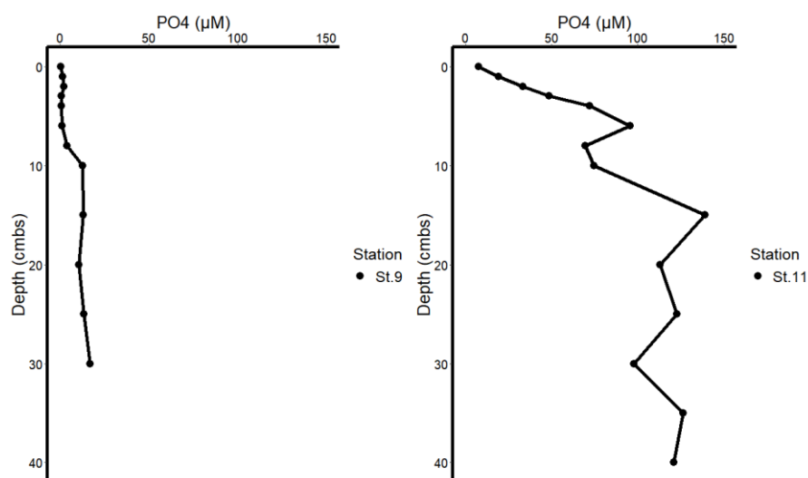
Figure 13. \text{PO}_4^{3-} measurements in Station 9 and Station 11 according to depth
