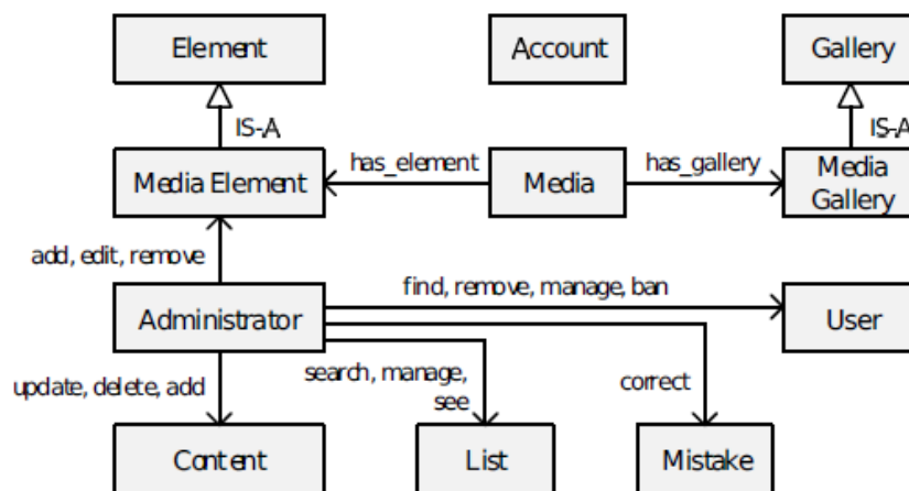
Figure 2.2 Example Conceptual Model created by Visual Narrator (Robeer et al., 2016)
