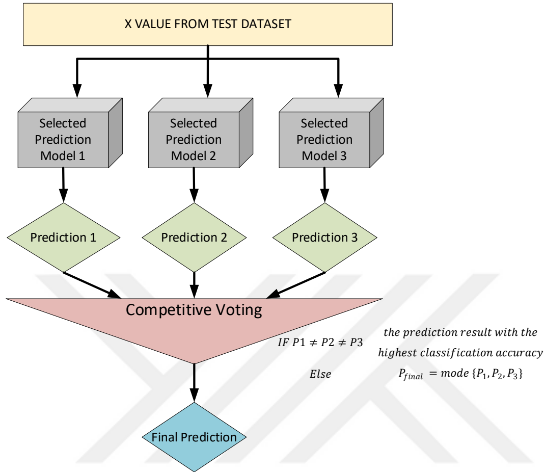
Figure 5.10. Competitive Voting
