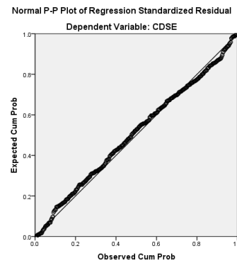
Figure 4.2 Normal P-P plot showing normality of residuals
