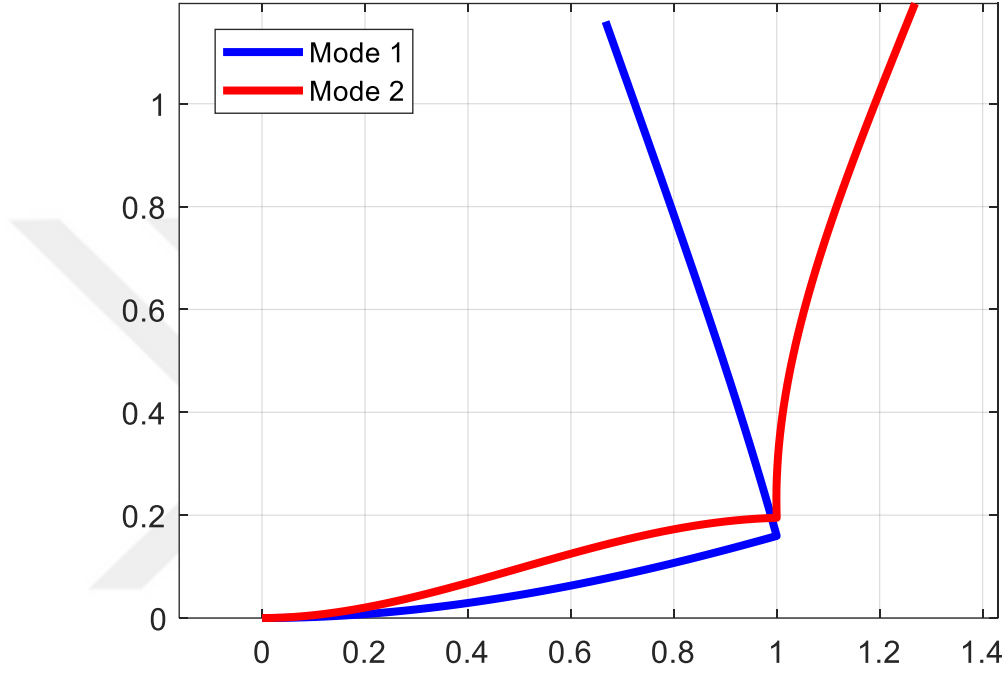
Figure 4.5. Mode Shapes of the Fixed L-Shaped Beam for Case 1
