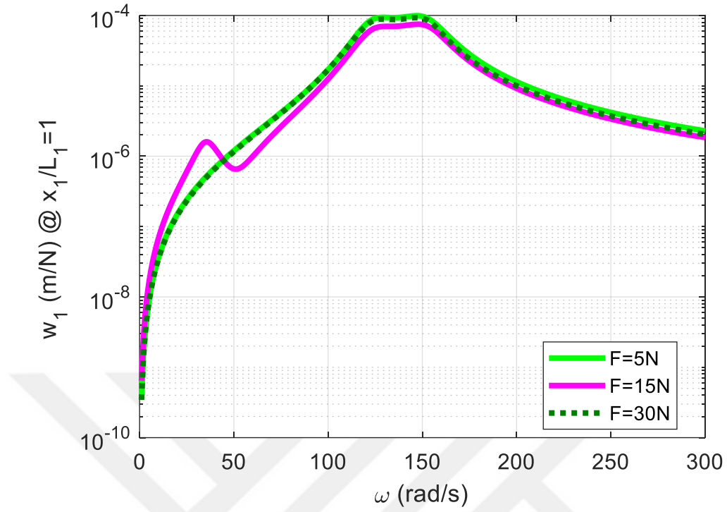
Figure 5.10. Frequency Response for Case 3 at x_1/L_1=1
