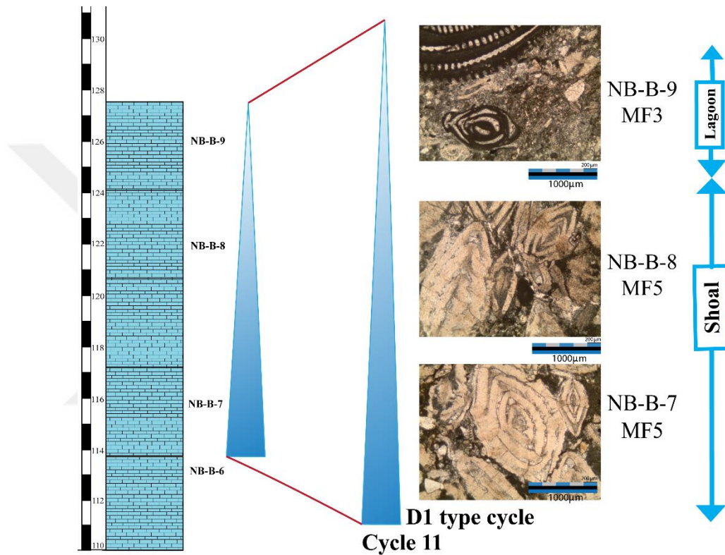
Figure 73: D1 type cycle (Cycle 11) of the measured section and photomicrographs of microfacies deposited within this cycle.
