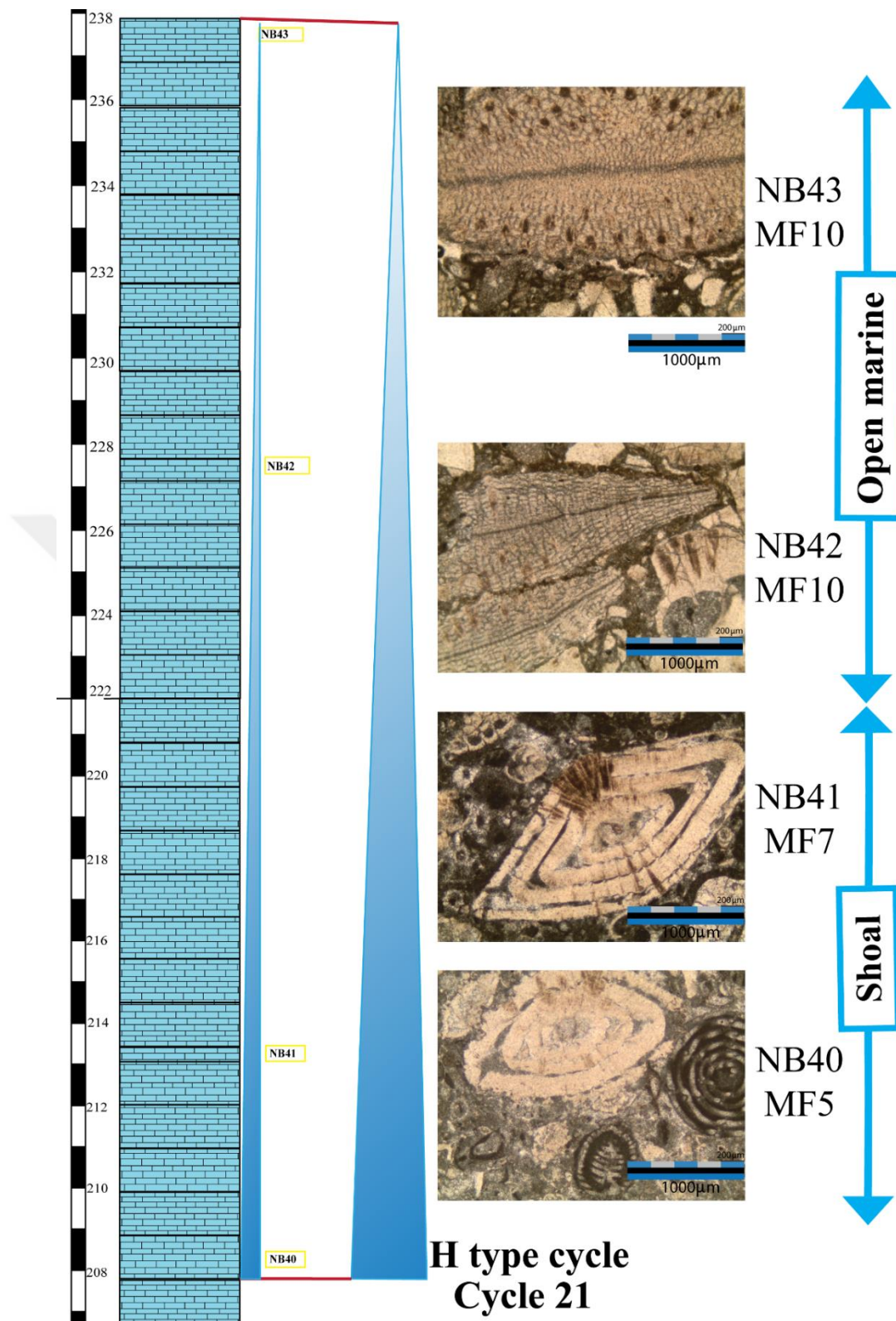
Figure 83: H type cycle (Cycle 21) of the measured section and photomicrographs of microfacies deposited within this cycle.
