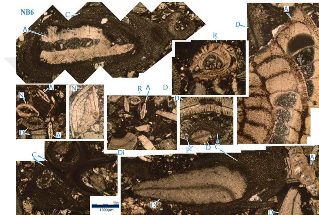
Figure 47: Photomicrograph of the MF8 (the sample NB6. A: Assilina sp., C: LCRA, CRA. D: Discocyclus sp., N: Nummulites sp., pf: Planktonic Foraminifera, R: Rotaliniid. At upper right: Assilina sp. surrounded by CRA, At lower left : D surrounded by CRA).
