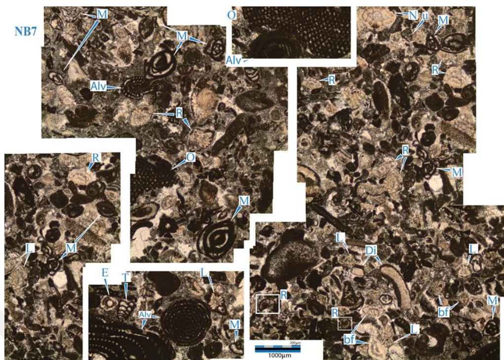
Figure 38: Photomicrograph of MF1 (sample NB7).
