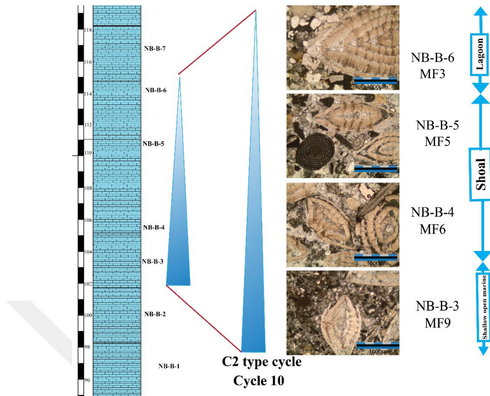
Figure 72: C2 type cycle (Cycle 10) of the measured section and photomicrographs of microfacies deposited within this cycle.
