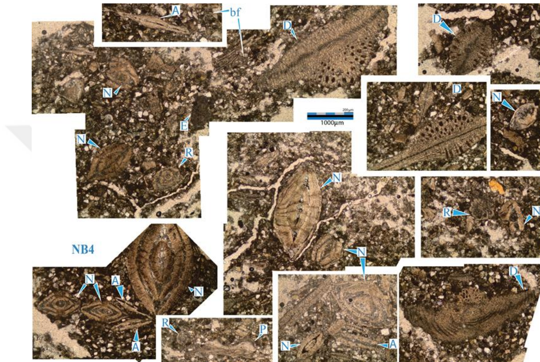
Figure 49: Photomicrograph of the MF9 (the sample NB4, MF11, A: Assilina sp., B: Benthic foraminifera C: Rotaliniid,, D: Discocyclina sp., E: echinoid fragment, pf: planktonic foraminifera, N: Nummulites sp., P: pelecypods).
