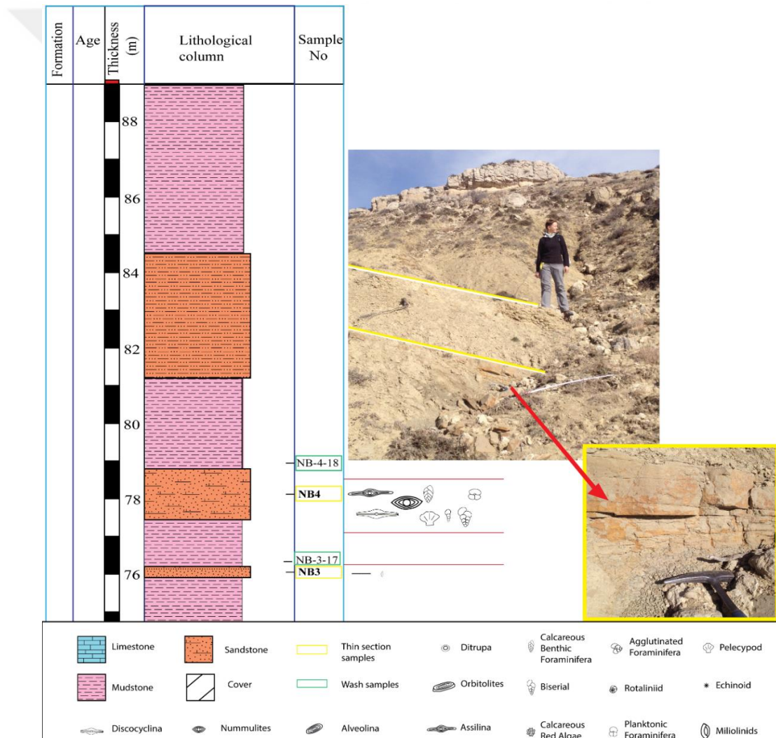
Figure 25: Detailed columnar section showing the taken samples NB3, NB4 location from the measured section.
