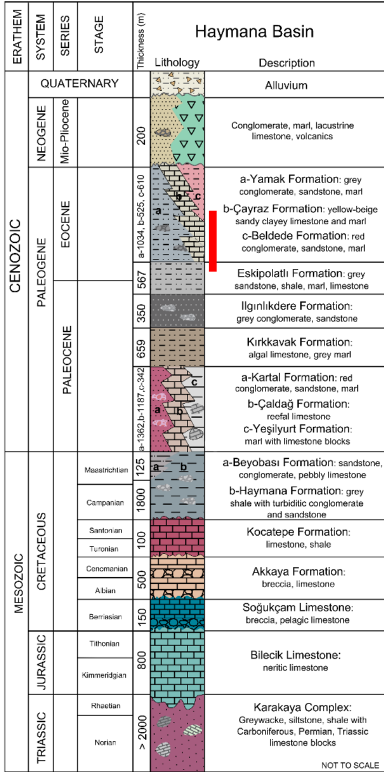
Figure 18: Generalized columnar section of the Haymana Basin modified from Ünalın et al. (1976) and Okay and Altınır (2016). (red line indicate the approximate location of the measured section covering the Çayraz Formation)
