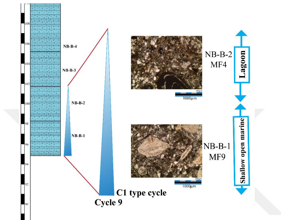
Figure 71: C1 type cycle (Cycle 9) of the measured section and photomicrographs of microfacies deposited within this cycle.
