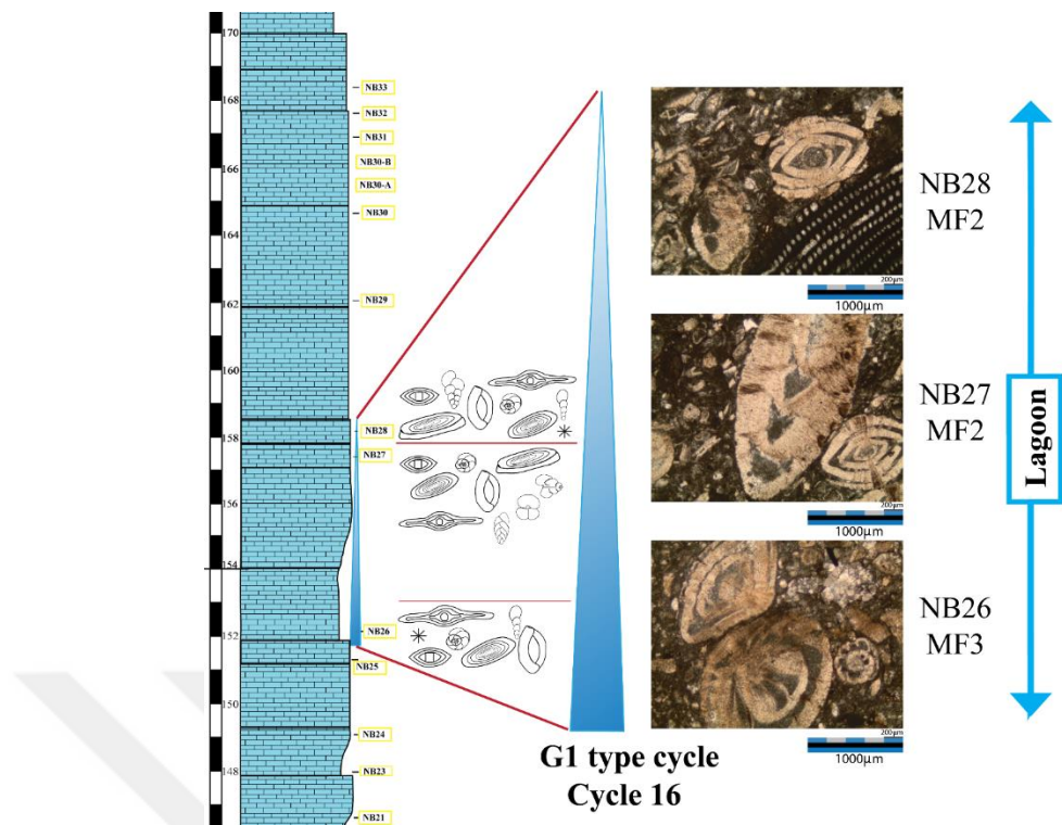
Figure 81: G1 type cycle (Cycle 16) of the measured section and photomicrographs of microfacies deposited within this cycle.
