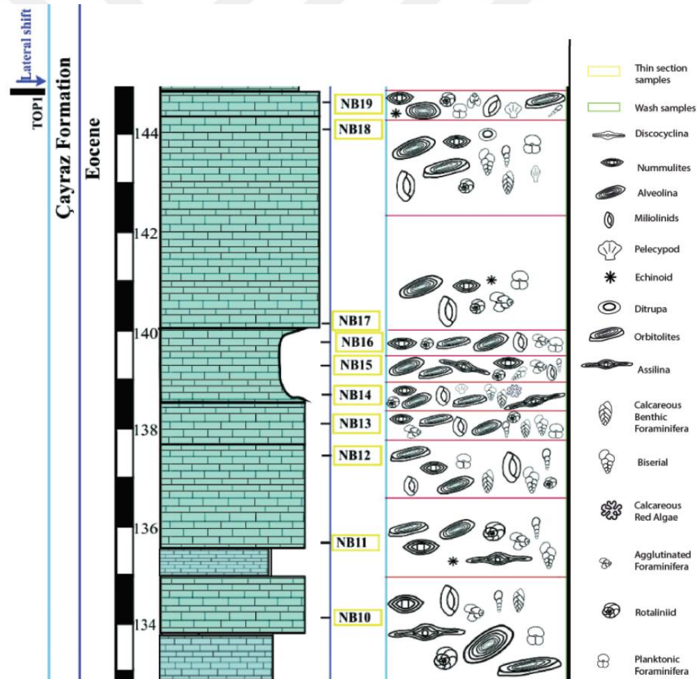
Figure 28: Detailed columnar section showing the taken samples NB10, NB11, NB12, NB13, NB14, NB15, NB16, NB17, NB18 and NB19 location from the measured section.
