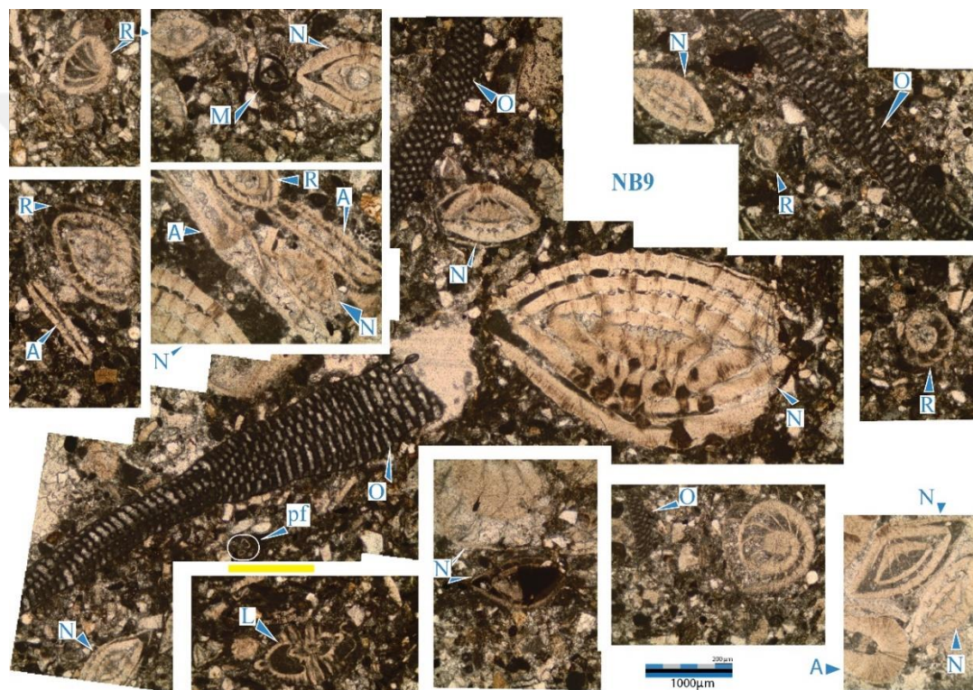
Figure 43: Photomicrograph of the microfacies MF4. (sample NB9. A: Assilina sp., bf: benthic foraminifera, D: Discocyclus sp., pf: planktonic foraminifera, N: Nummulites sp., O: Orbitolites sp., R: Rotaliniid .sp., L: Lockhartia sp.)
