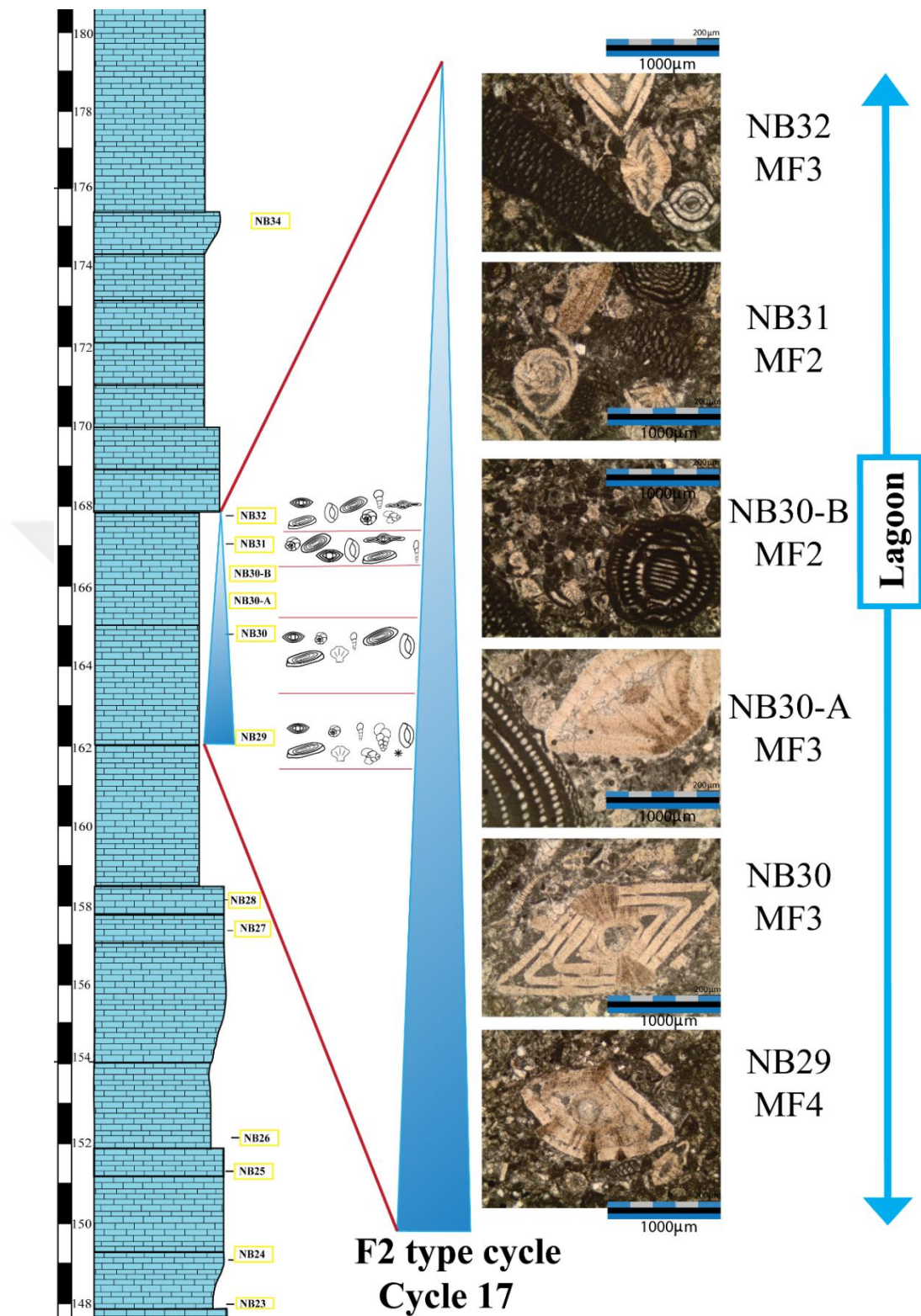
Figure 80: F2 type cycle (Cycle 17) of the measured section and photomicrographs of microfacies deposited within this cycle.
