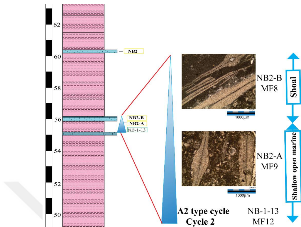
Figure 64: A2 type cycle (Cycle 2) of the measured section and photomicrographs of microfacies deposited within this cycle.
