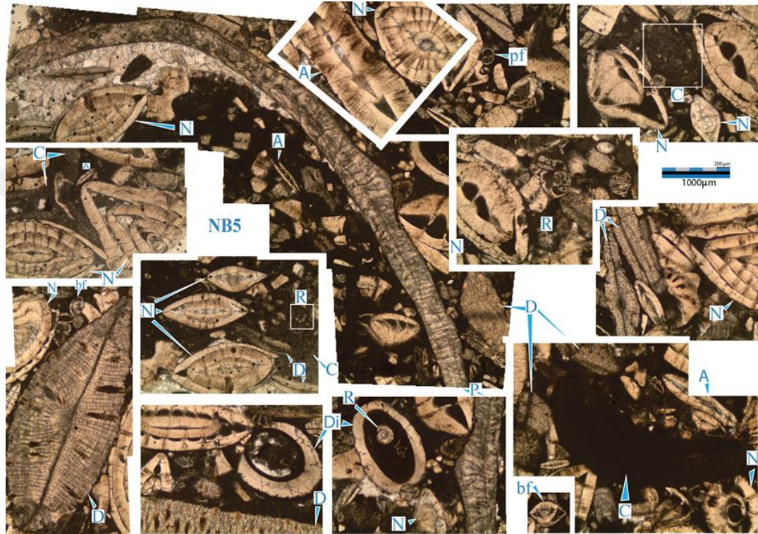
Figure 45: Photomicrograph of the MF6 (the sample NB5. P: pelecypoda surrounded with calcite crystal, C:LCRA and CRA. N: Nummulites , A: Assilina sp., R: Rotaliiniid , pf: Planktonic foraminifera, Di: Ditrupa sp., D: Discocyclina , C: Coralline Red Algae (CRA)).
