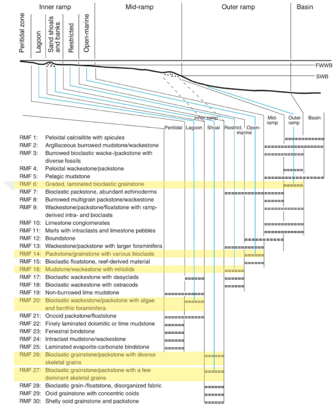
Figure 36: Generalized distribution of microfacies types in different parts of a homoclinal carbonate ramp (Flügel, 2010). The ones that were observed in the study have been indicated by yellow highlights.
