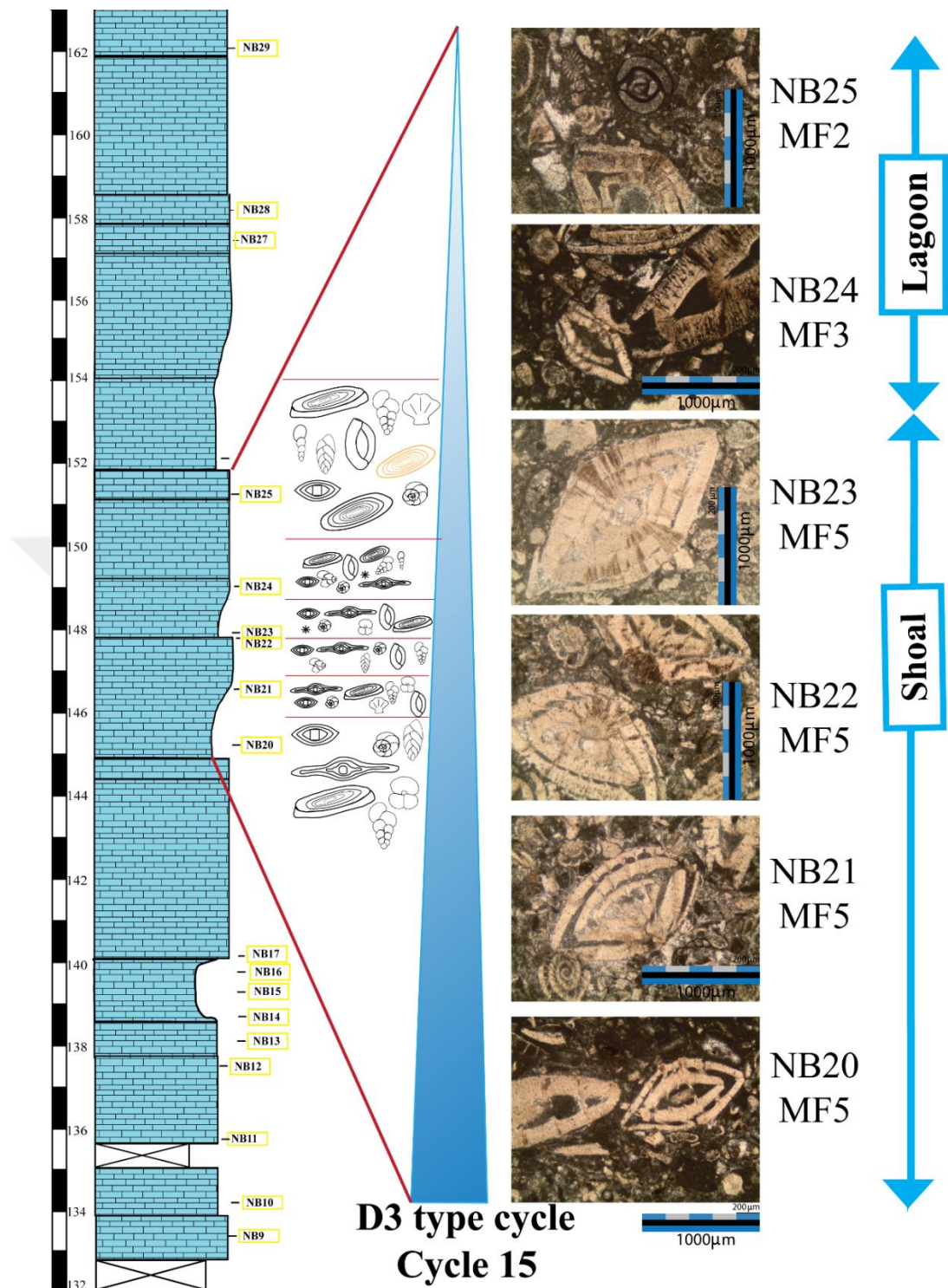
Figure 75: D3 type cycle (Cycle 15) of the measured section and photomicrographs of microfacies deposited within this cycle.
