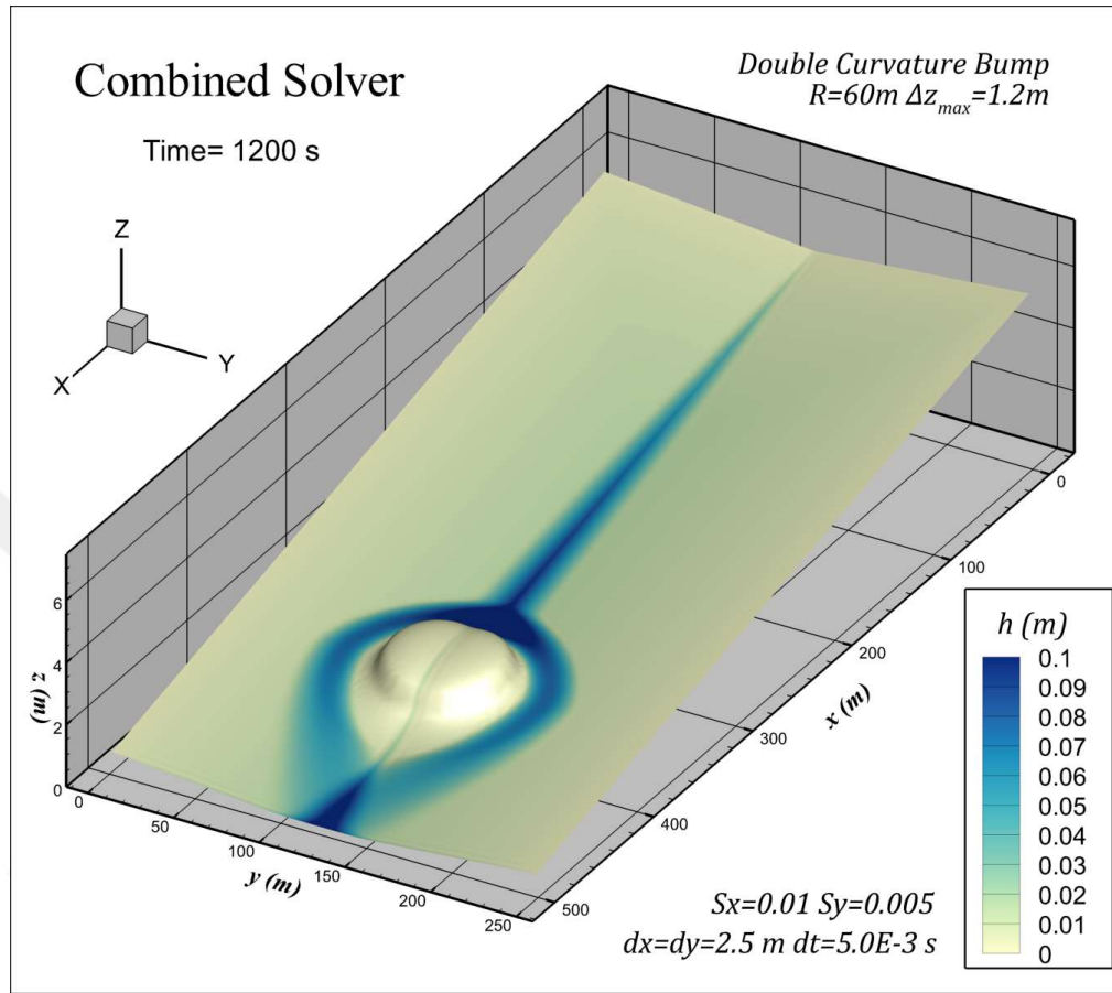
Figure 3.24 3D Water depth plot from combined solver for Test Case-2 at t = 1200\text{ s} .
