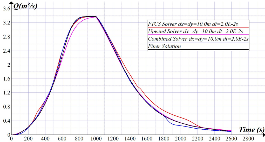
Figure 3.22 Comparison with finer mesh solution. Finer mesh solution obtained from the combined solver for dx = dy = 2.5\text{m} and dt = 5.0E - 3\text{s} .
