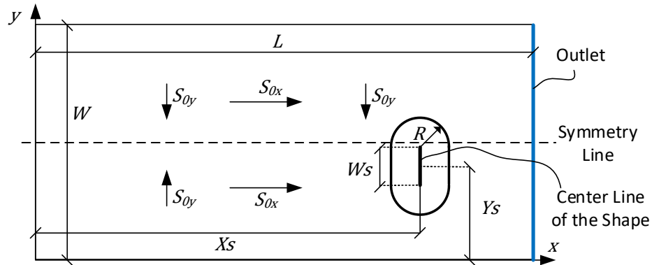
Figure 3.12 Geometry and important distances in test cases
