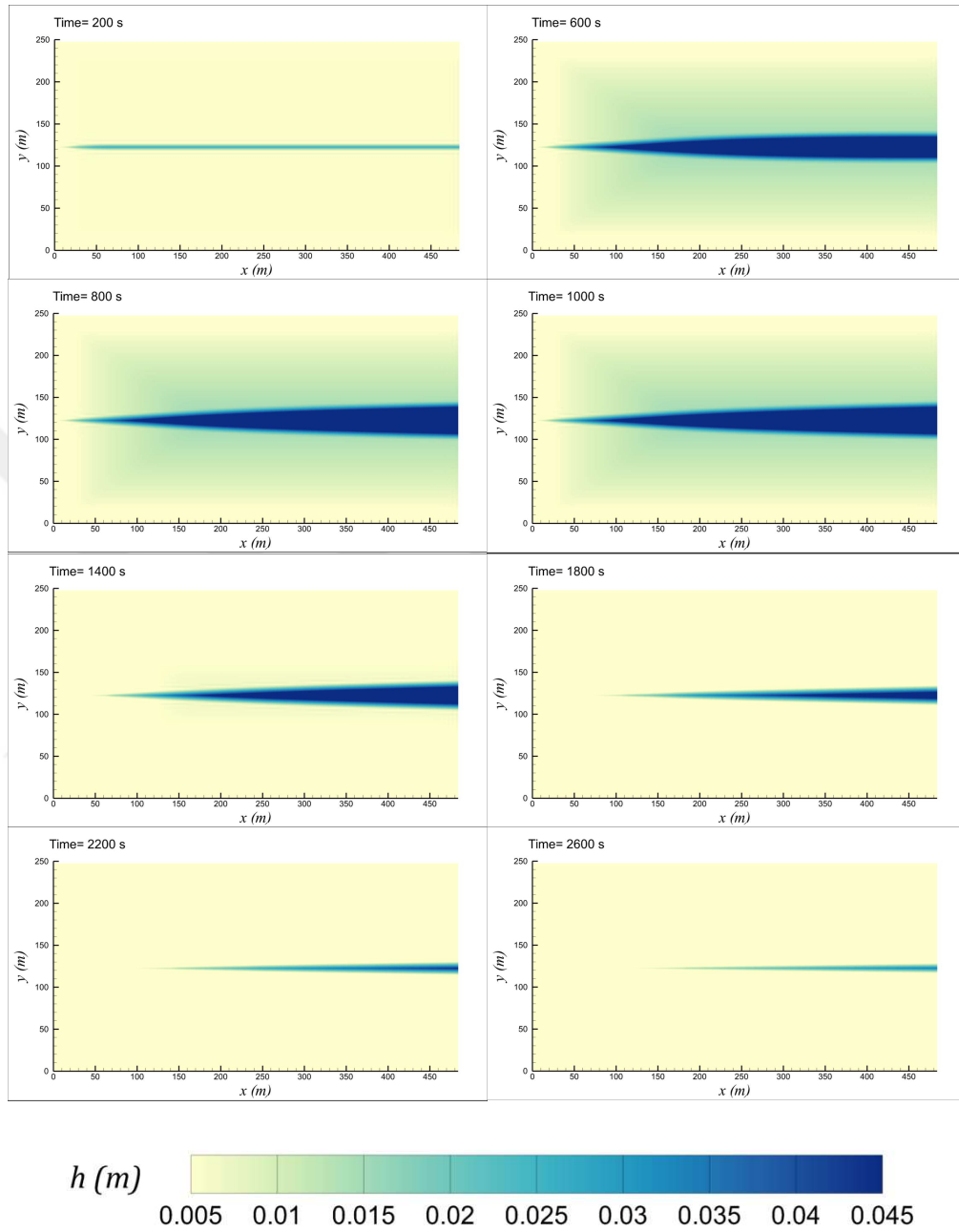
Figure 3.17 2D Water depth contour plot at different times for Test Case-1 from combined solver.
