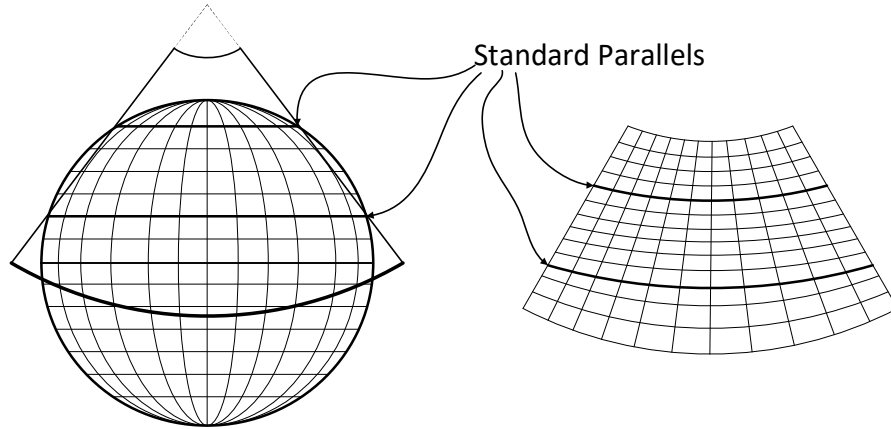
Figure 5.8 Conic Projection
