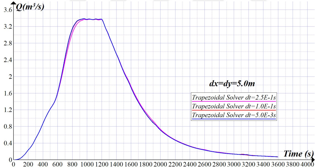
Figure 3.29 Outlet hydrograph for Test Case-2 obtained from trapezoidal central space solver for different time-step sizes.
