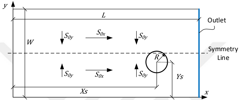
Figure 3.13 Test case geometry with W_s = 0 m.
