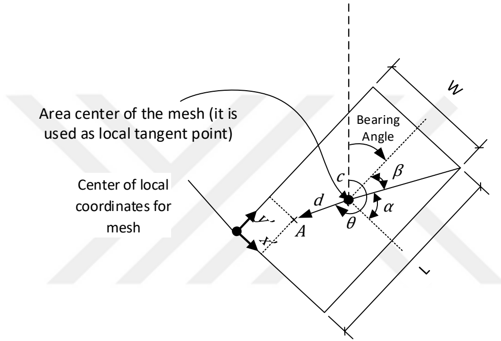
Figure 6.9 Mesh on the local tangent plane
