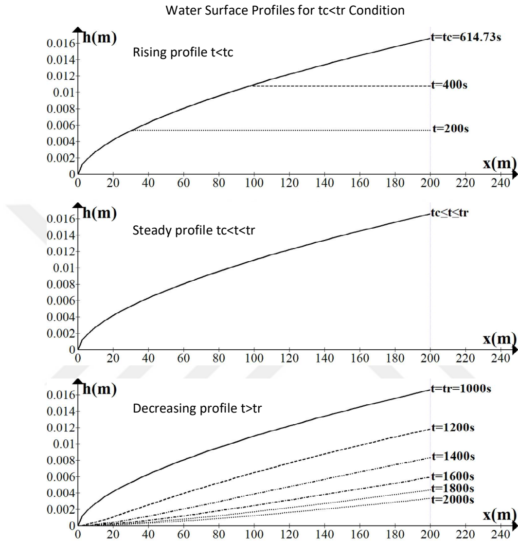
Figure 2.4 Water surface profiles for t_c < t_r condition
