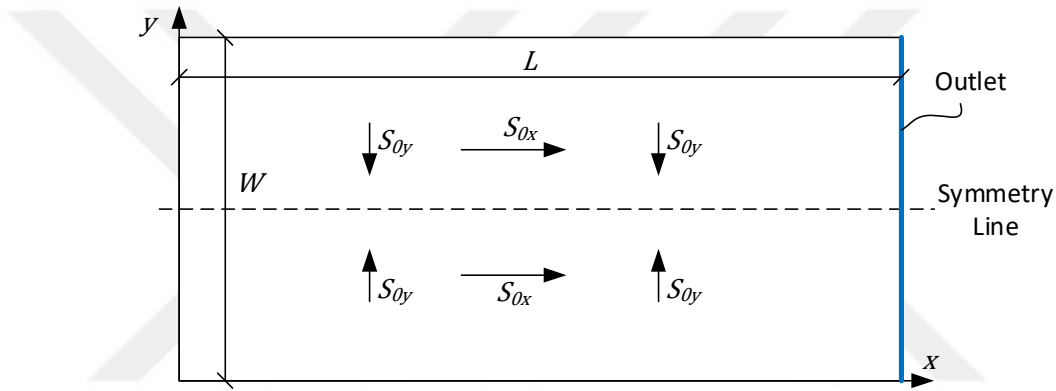
Figure 3.11 Main bed surface geometry.
