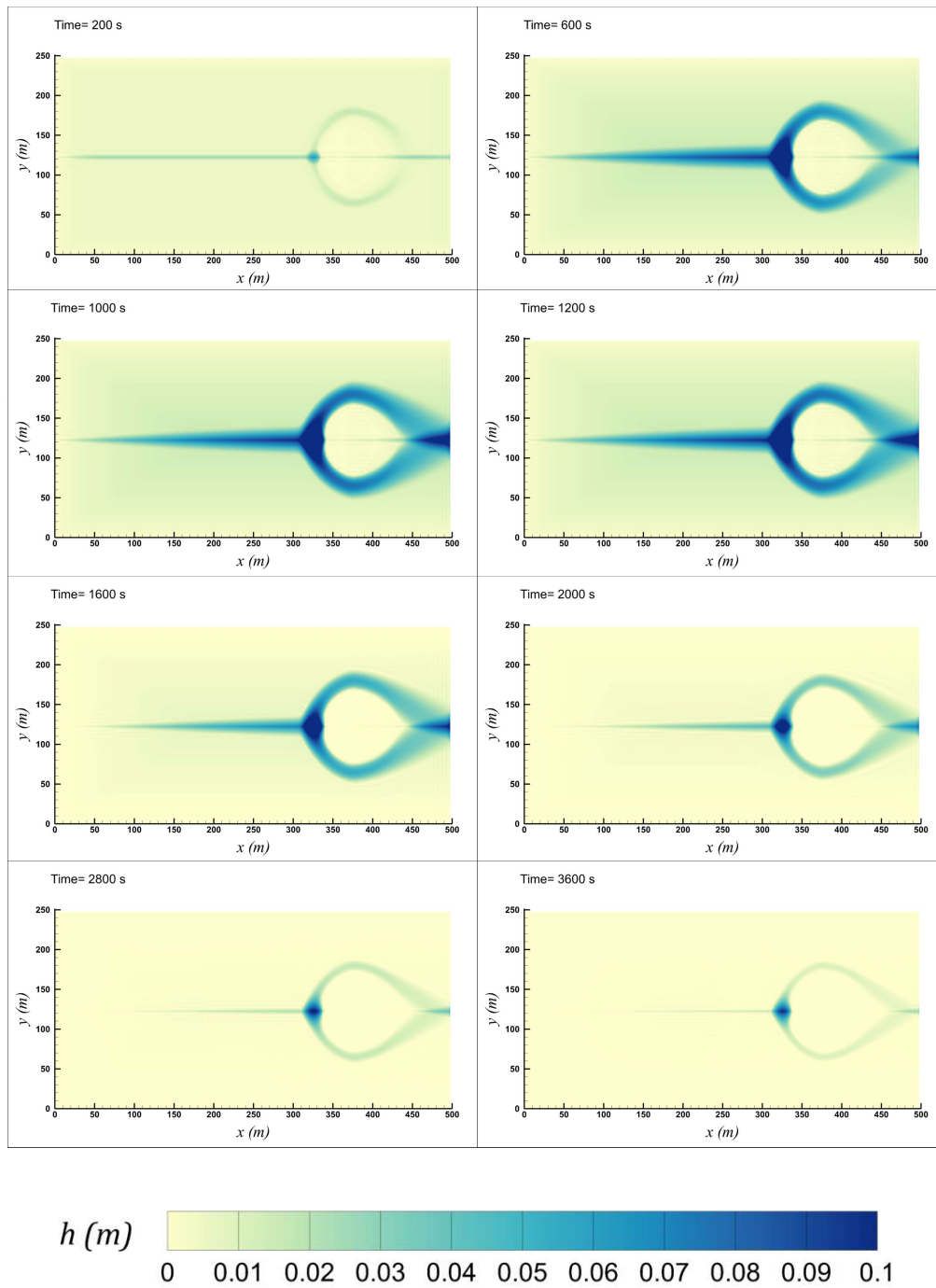
Figure 3.25 2D Water depth contour plot at different times for Test Case-2 from combined solver.
