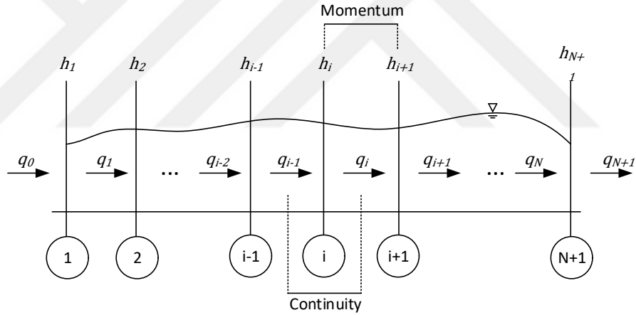
Figure 3.1 Grid structure for the one-dimensional model.
