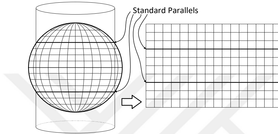
Figure 5.7 Cylindrical Projection
