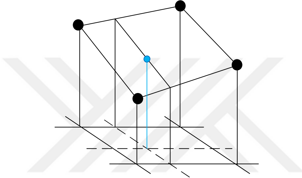
Figure 6.11 Bilinear interpolation
