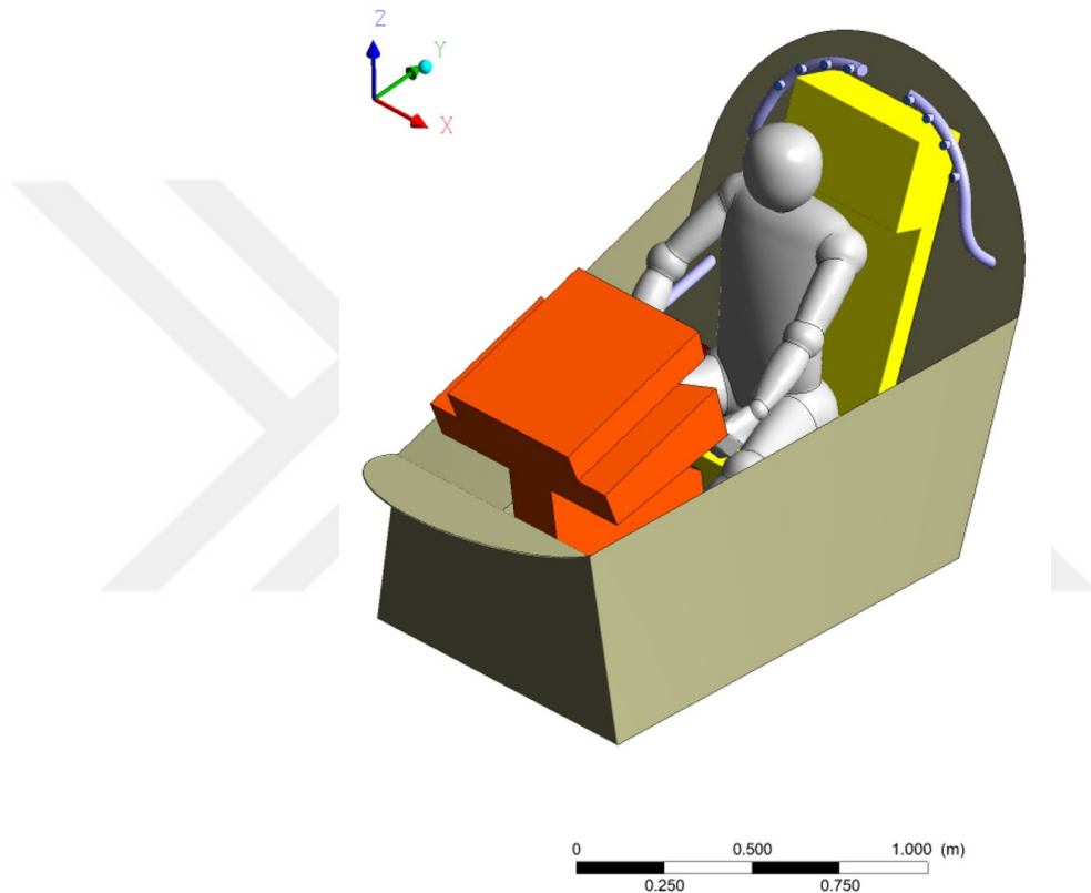
Figure 3.3-1- Geometry of Problem Domain
