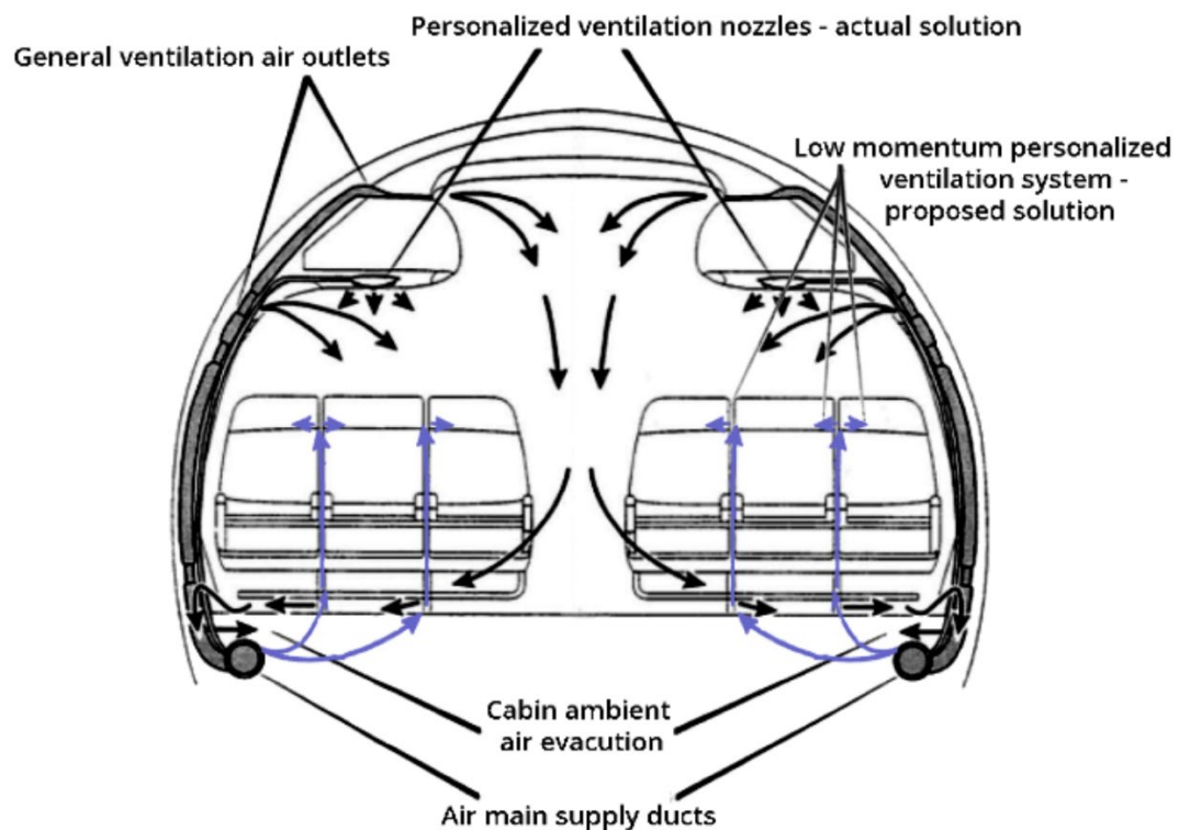
Figure 2.2-1- Personalized Ventilation [28]
