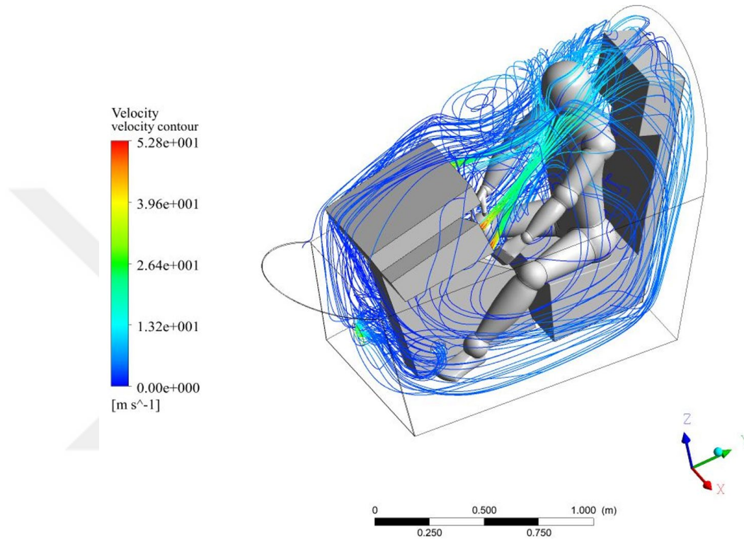
Figure 3.3-6 3D velocity magnitude streamline contour around the cockpit with gasper inlets
