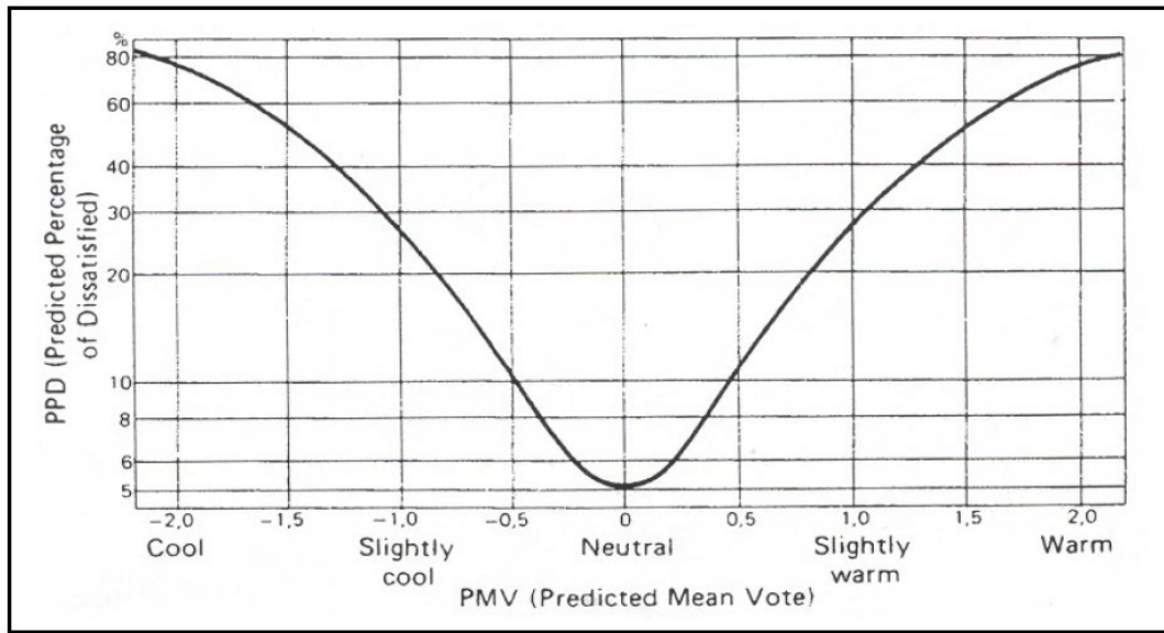
Figure 1.4-6- PMV-PPD Diagram [16]
