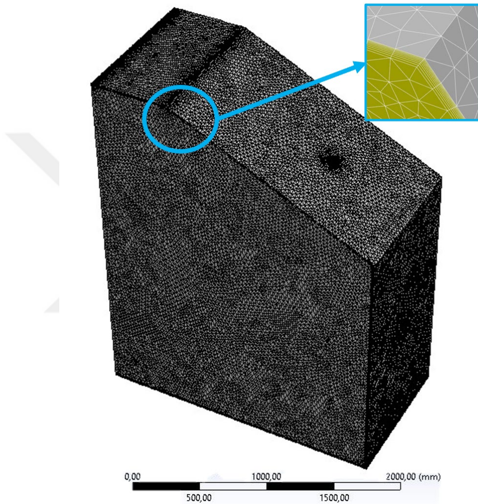
Figure 2.2-8- Tetrahedral Meshing of Sample Case
