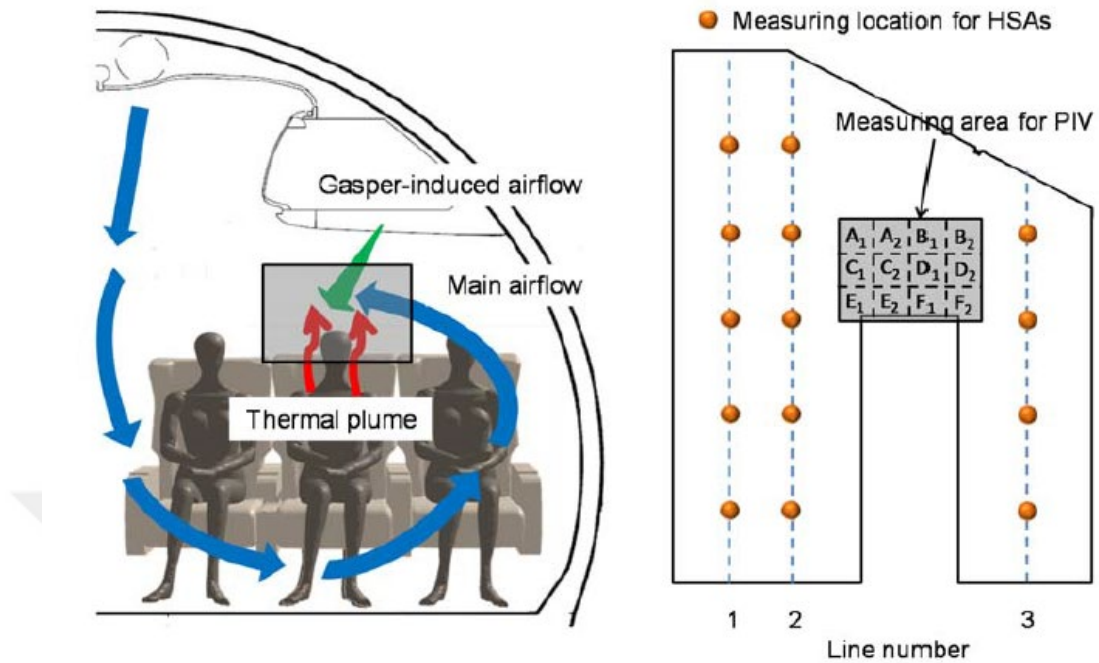
Figure 2.2-3- Experimental set-up measurement points of the study [27]
