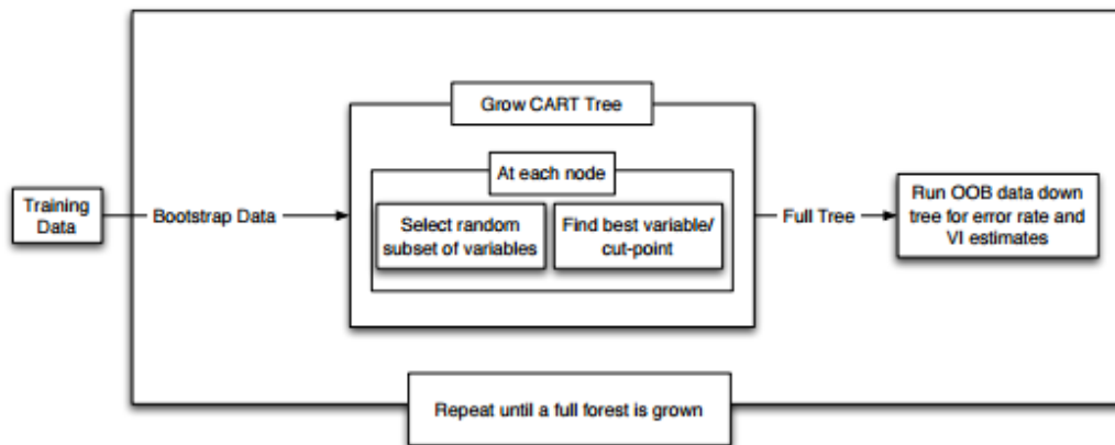
Figure 3: Construction [28] of Random Forest
