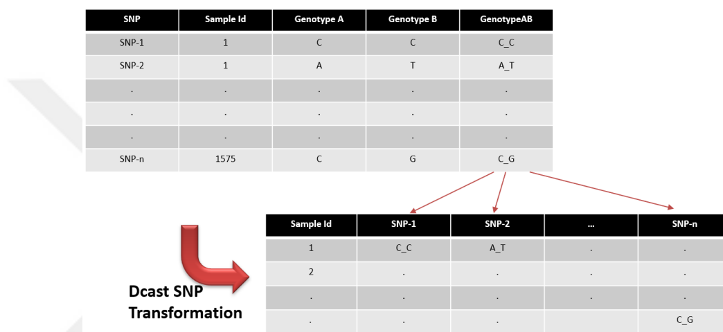
Figure 8: Reshape2 package: Dcast function Implementation
