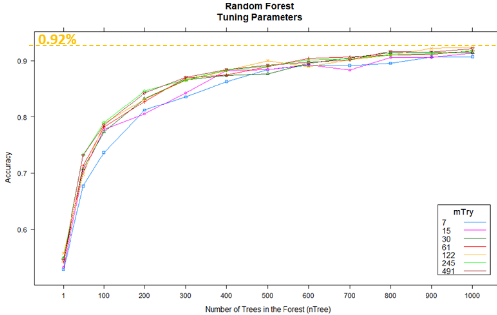
Figure 15: GenADA RF Tuning Parameters
