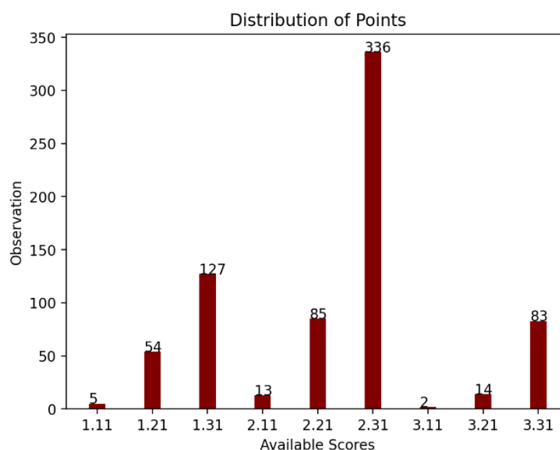
Figure 23: Ensemble Scoring Results
