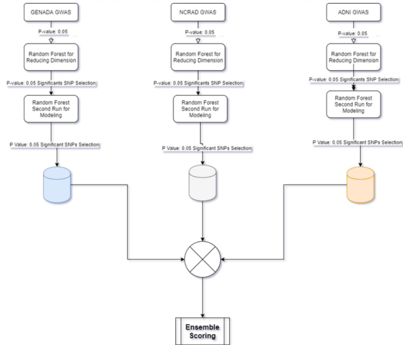
Figure 5: Overview of the Modeling Methodology
