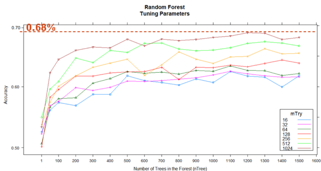
Figure 17: NCRAD RF Tuning Parameters
