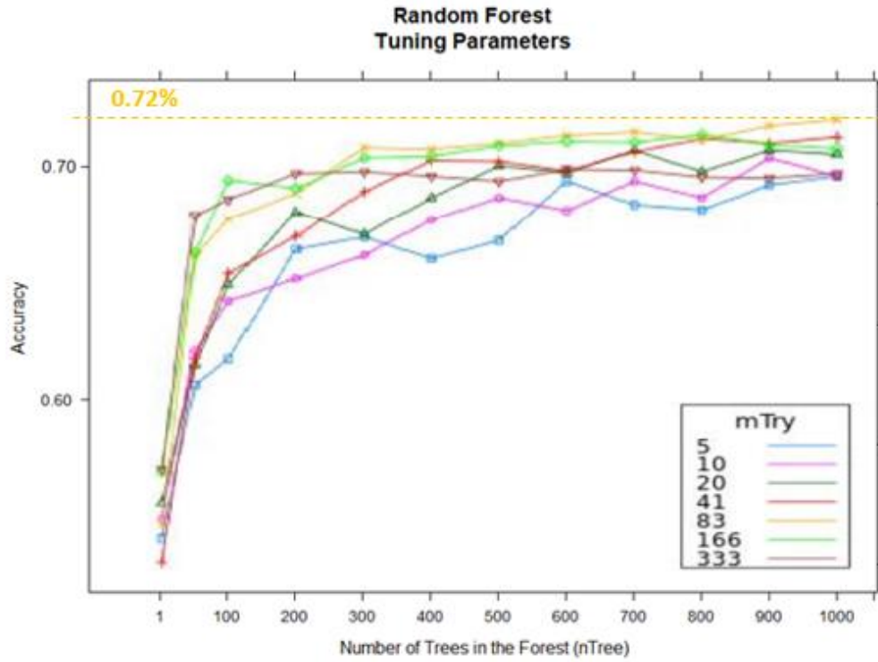
Figure 18: NCRAD RF-RF Tuning Parameters
