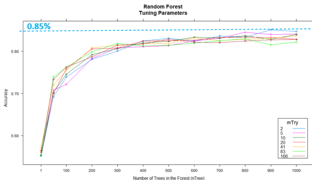
Figure 16: GenADA RF-RF Tuning Parameters
