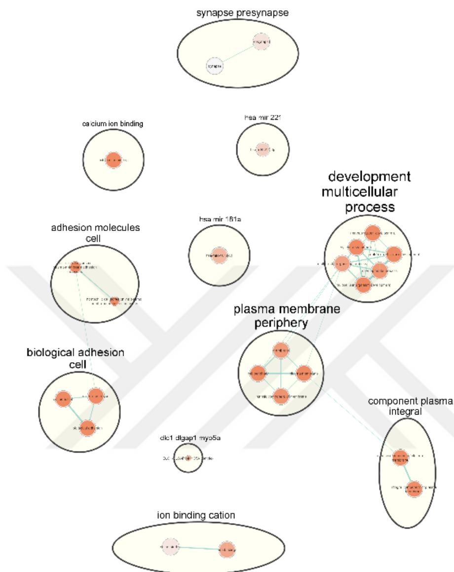
Figure 26: Functional Enrichment Analysis of Union of Variants with EnSCAN Class Score 2.31 or 3.31
