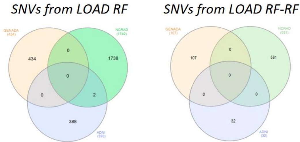
Figure 22: Number of Common SNVs from Three Individual Models
