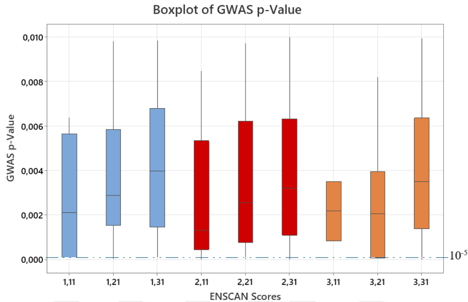
Figure 7: Comparison of GWAS p-values Relative to EnSCAN Scores
