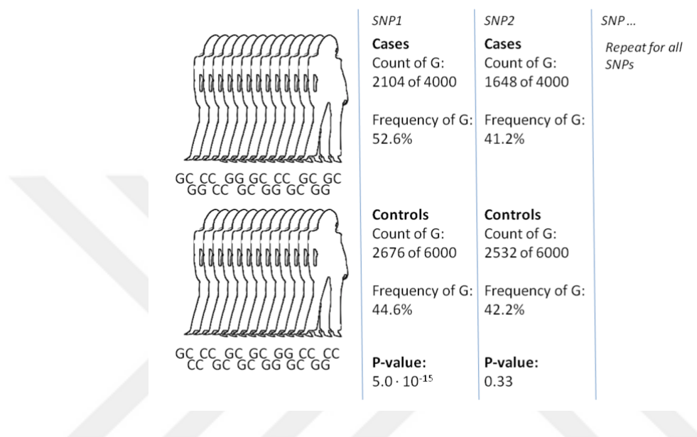
Figure 2: Genome-Wide Association Study
