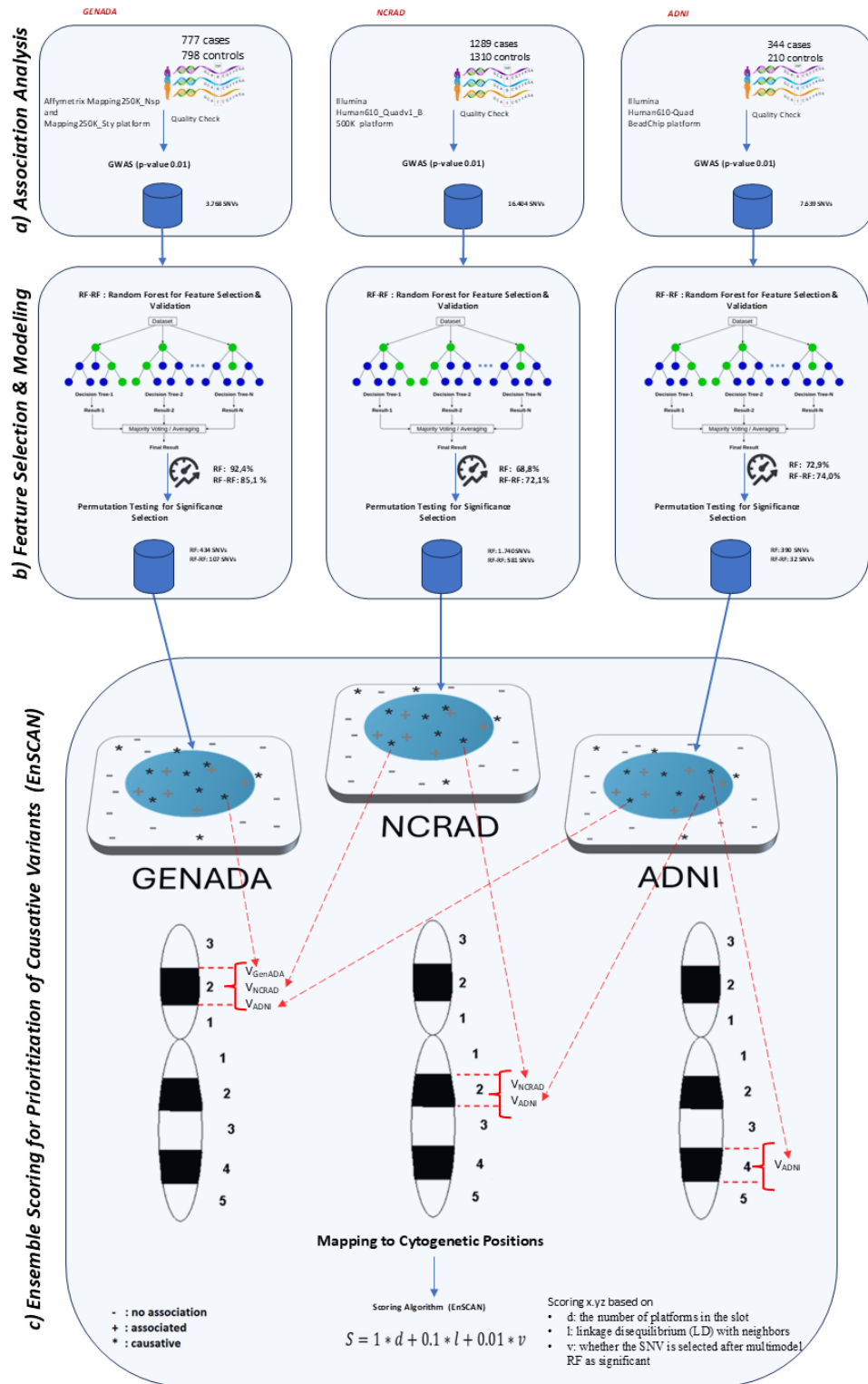
Figure 6: Design for Model Building and EnSCAN
