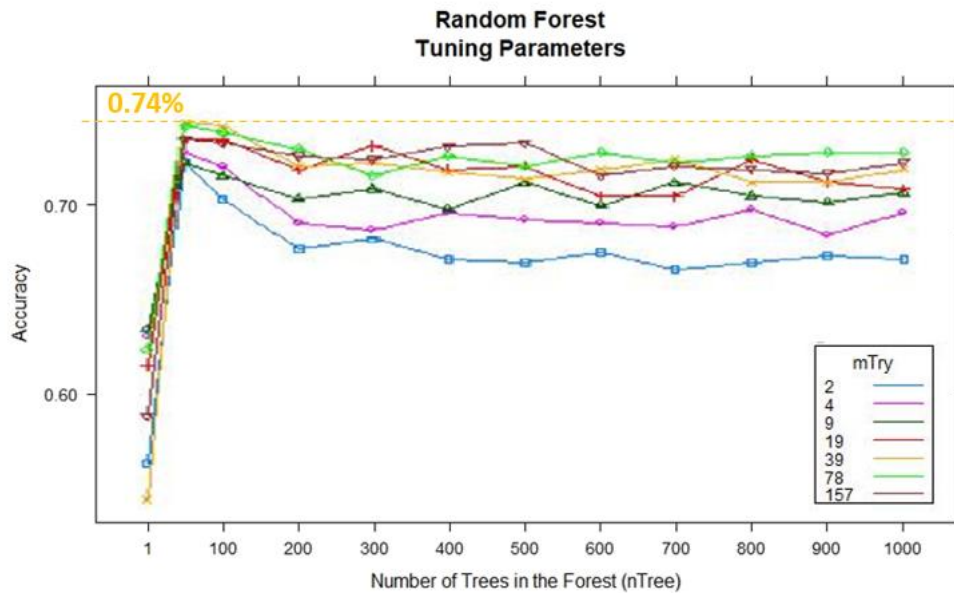
Figure 20: ADNI RF-RF Tuning Parameters
