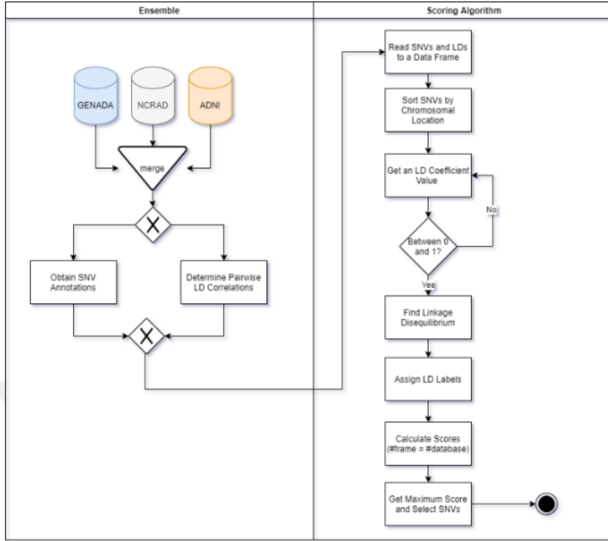
Figure 11: Flowchart of Ensemble Scoring Algorithm (EnSCAN)
