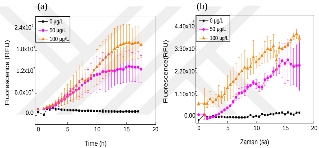
Figure 3.15 Fluorescence emission kinetics of immobilized arsenic bioreporter induced with varying As (V) concentrations (uninduced (0 \mu\text{g/L} )), 50 \mu\text{g/L} and 100 \mu\text{g/L} ). a) 12.5% CA and b) 10% PCL were used as the fibrous support materials, MOPS – supplemented medium was used as the growth and immobilization media; cells were grown till mid – exponential growth phase, OD_{600} was set as 0.5 n=4 .
