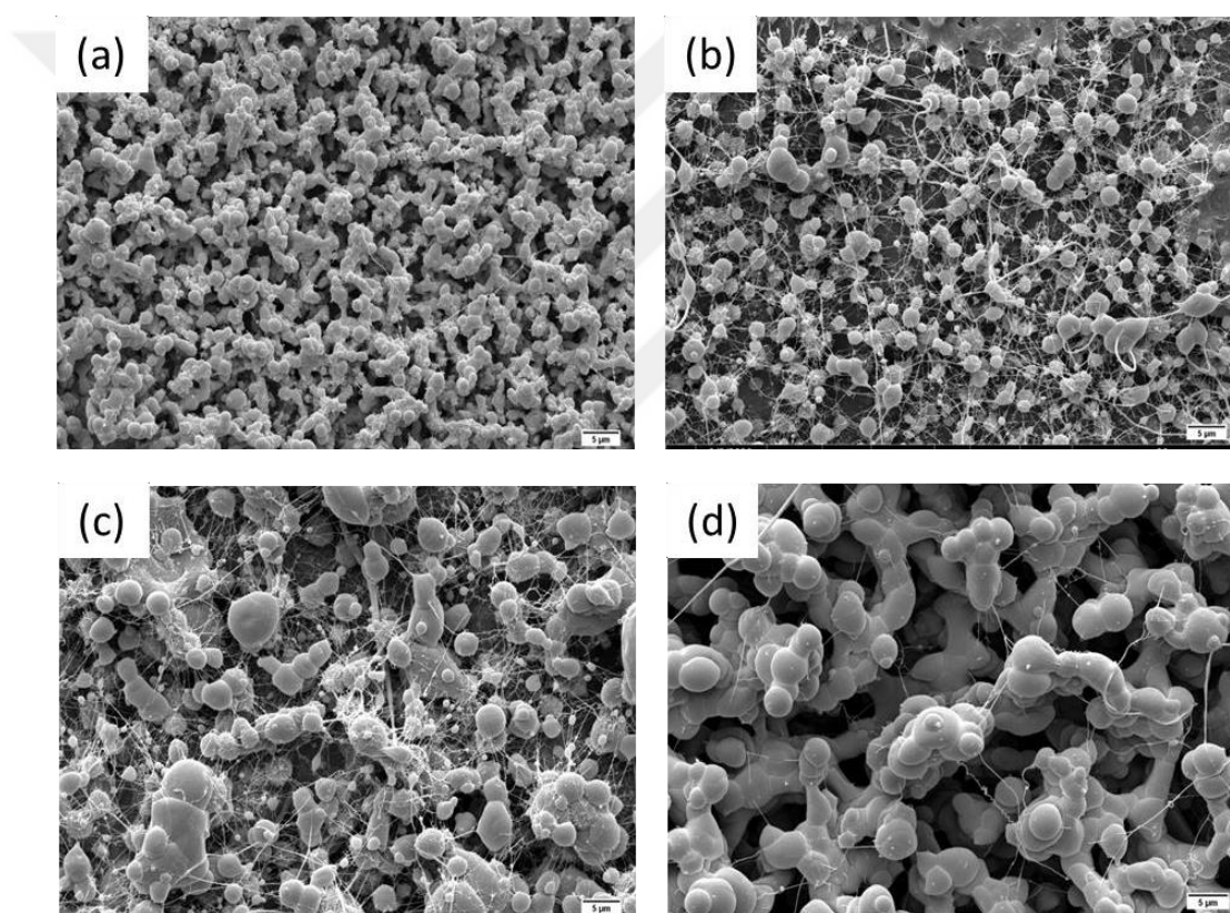
Figure 3.2 Typical SEM micrograph of (a) 10% PCL, (b) 15% PCL, (c) 20% PCL and (d) 25% PCL electrospun support material (Solvent system: DCM/DMF (1/1 v/v), Voltage: 25 kV, Flow rate: 0.5 mL/h, End to tip distance: 15 cm).
