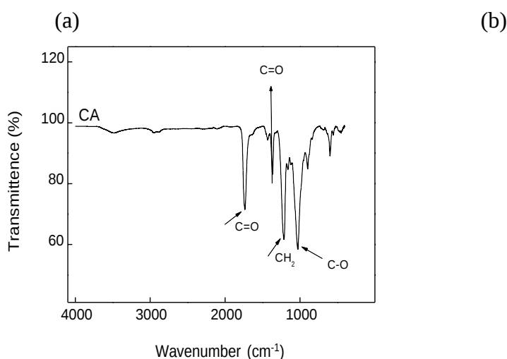
Figure 3.5 FTIR spectra of (a) 10 wt% CA and (b) 10 wt% PCL electrospun fibers.
