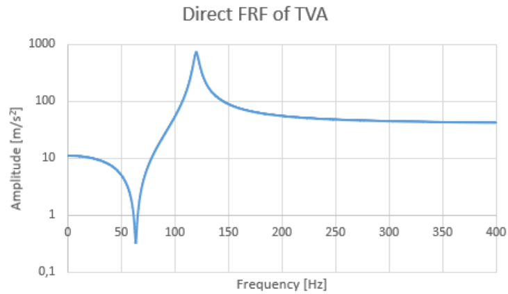
Figure 4.31: Direct FRF of the TVA
