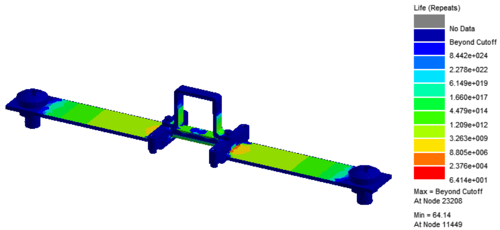
Figure 5.25: Fatigue Life Estimation Analysis Result for the TVA
