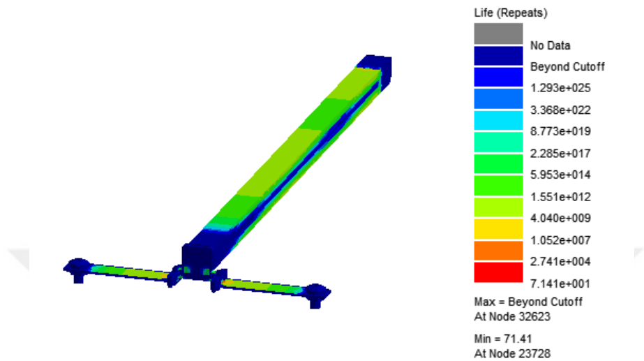
Figure 5.27: Fatigue Life Estimation Analysis Result for Full Body
