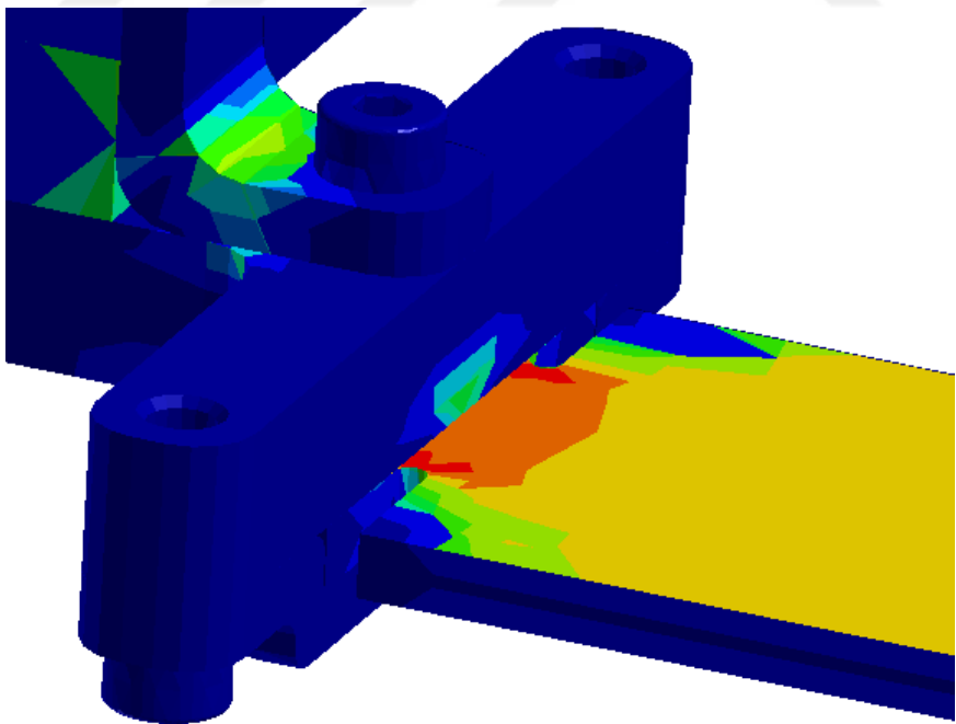
Figure 5.19: Detailed View of Fatigue Life Estimation Result of Notched Area
