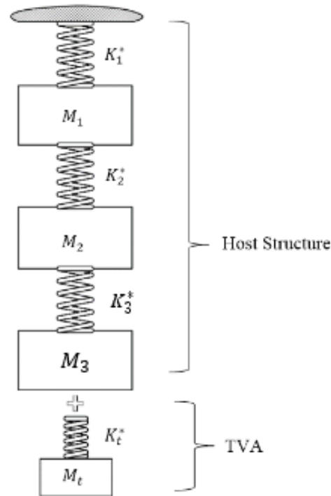
Figure 4.47: 4 DOF Structure.
