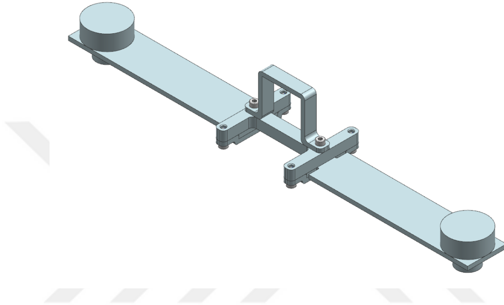
Figure 3.3: Cantilever Beam Type TVA
