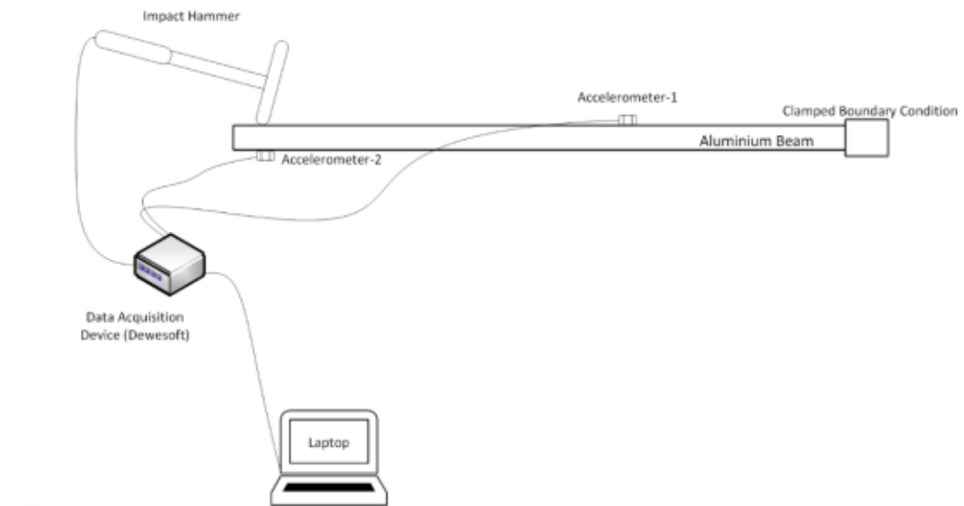
Figure 5.2: Test Setup for Tip Point Direct FRF Measurement of the Base Structure
