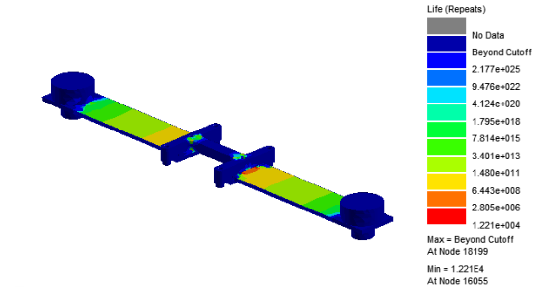
Figure 5.16: Fatigue Life Estimation Analysis Result for the TVA
