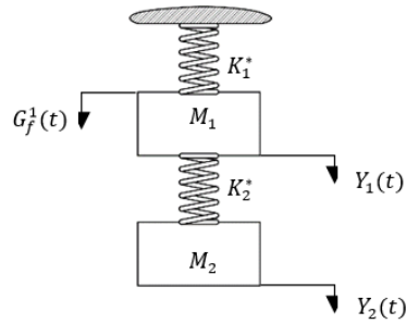
Figure 4.2: 2 DOF Structure.
