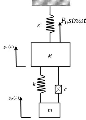
Figure 2.2: A Structure Modified with a TVA
