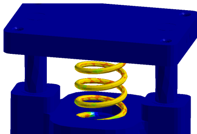
Figure 4.44: Detailed View of Fatigue Life Estimation Result of Most Critical Area
