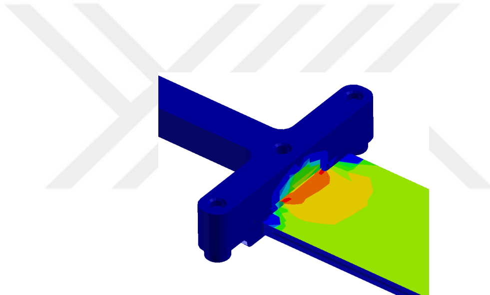
Figure 4.25: Detailed View of Fatigue Life Estimation Result of Notched Area
