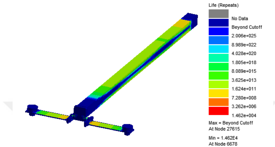
Figure 5.18: Fatigue Life Estimation Analysis Result for Full Body
