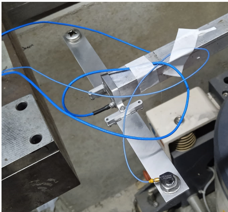
Figure 5.31: Detail View of Redesigned TVA During Transmissibility Measurement
