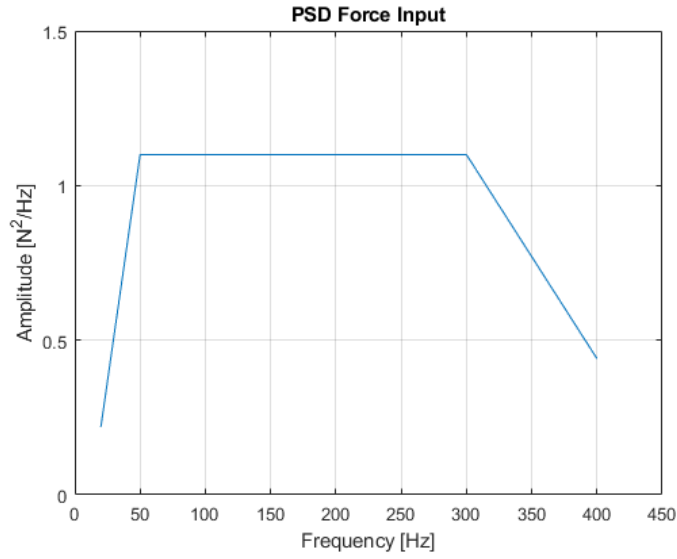
Figure 5.24: Changed PSD Force Input
