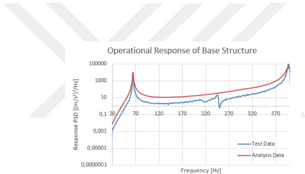
Figure 5.29: Operational Response with New PSD Force Input
