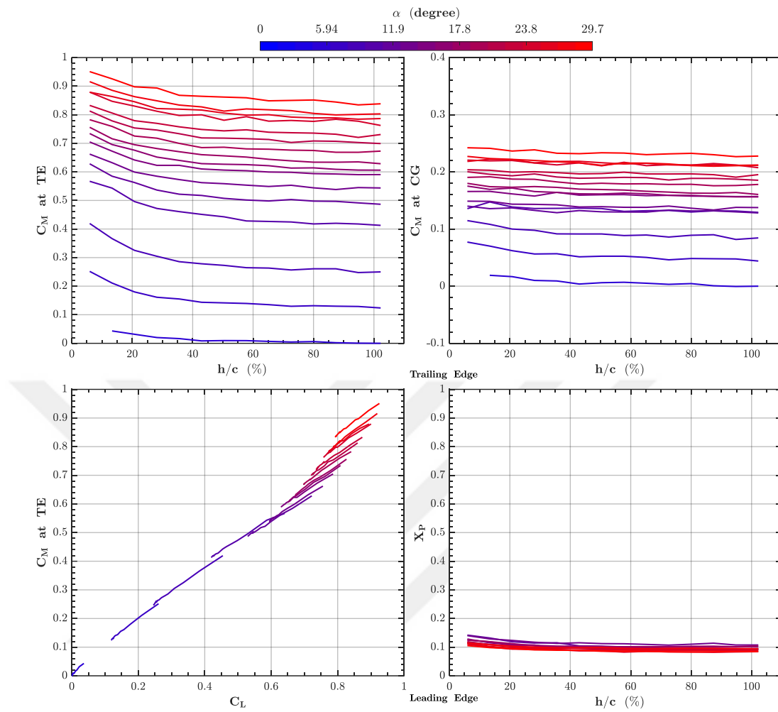
Figure C - 8 Variation of Moment coefficient C_M at trailing-edge (TE) and center of gravity (CG) as a function of function of non-dimensional height values and Lift coefficient C_L , and Non-Dimensional Pressure Center coordinate X_P as a function of non-dimensional height values for the reverse delta wing 2b
