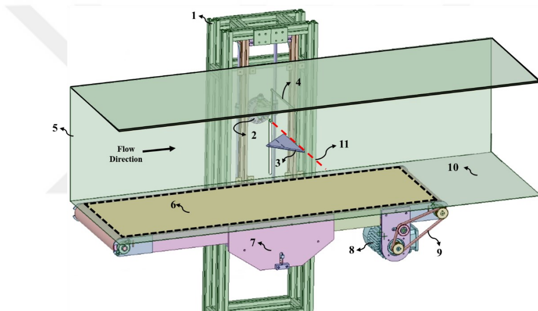
Figure 3-16 The ground effect test rig with moving belt mechanism and model positioning system, 1) model positioning system tower, 2) angle setter disks, 3) wing, 4) struts, 5) wind tunnel test section, 6) moving belt, 7) belt tension roller, 8) motor, 9) trigger belt, 10) wind tunnel floor, 11) rotation axis of angle of attack change
