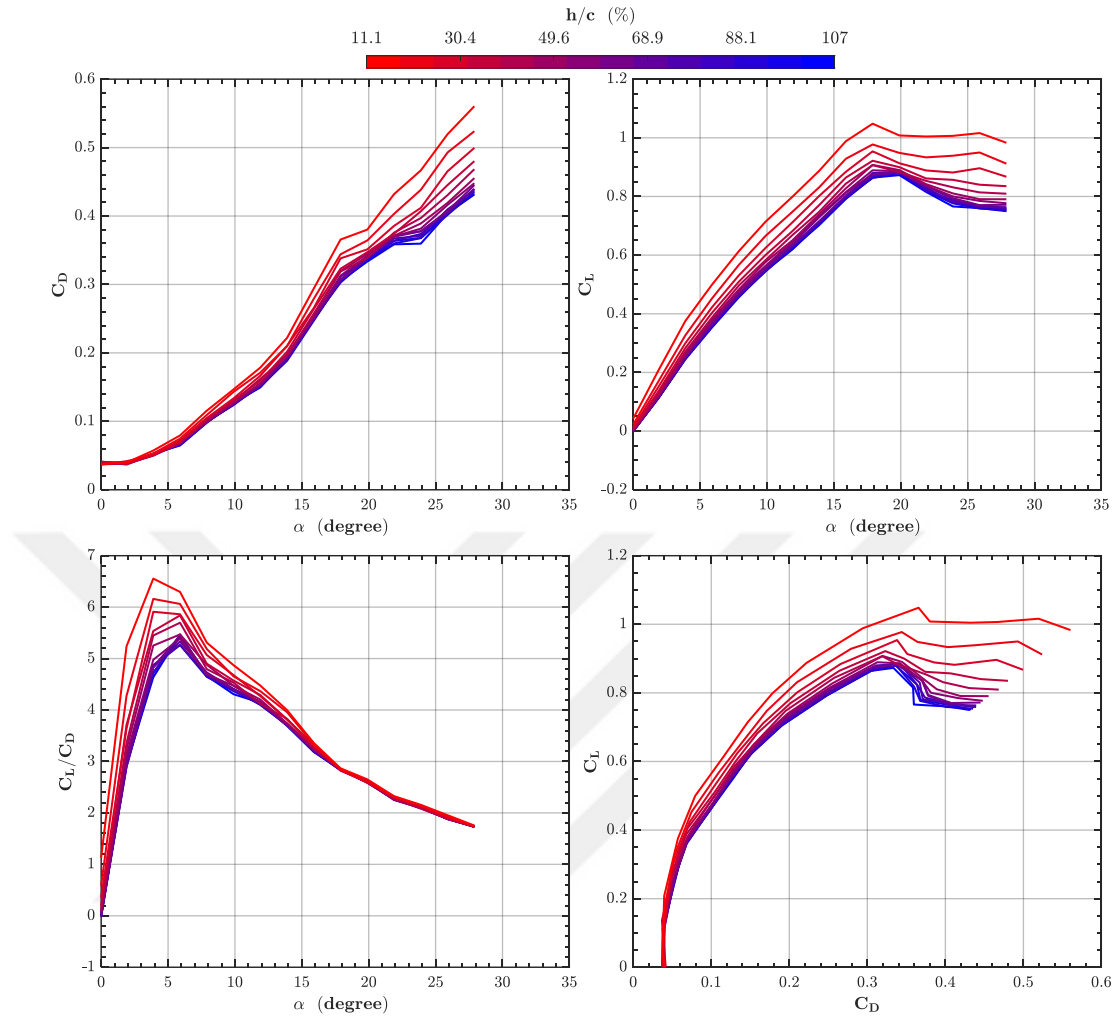
Figure 4-10 Variation of Drag coefficient C_D , Lift-to-Drag ratio C_L/C_D , Lift coefficient C_L as a function of angle of attack and Drag Polar for the delta wing 1b
