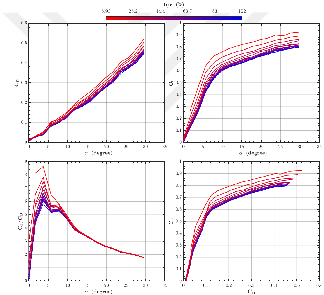
Figure 4-14 Variation of Drag coefficient C_D , Lift-to-Drag ratio C_L/C_D , Lift coefficient C_L as a function of angle of attack and Drag Polar for the reverse delta wing 2b
