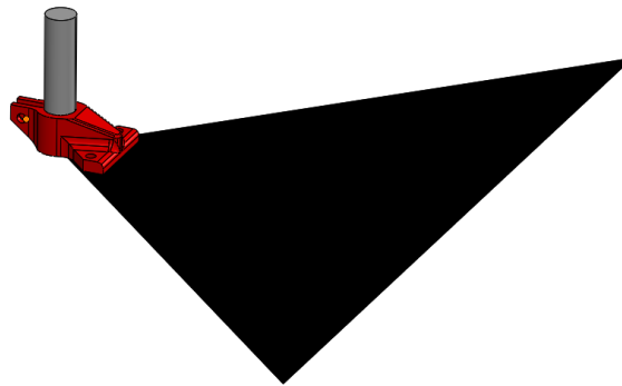
Figure B - 2 The reverse delta wing 2b, ( \Lambda = 45^\circ , t/c = 1.1\% , \delta = 0^\circ , Cr = 0\% )
