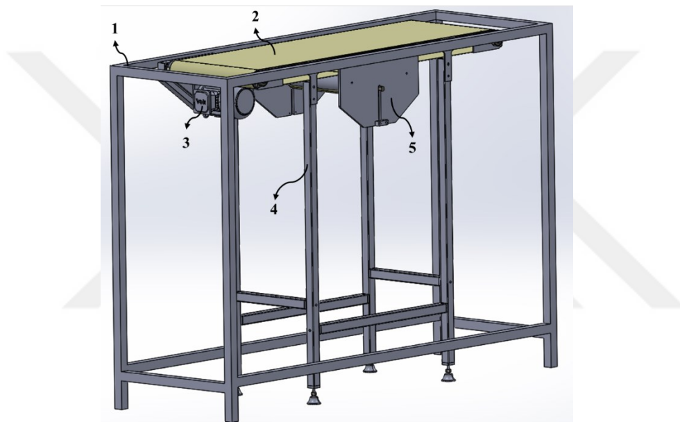
Figure 3-14 Schematic representation of the moving belt mechanism, 1) wind tunnel bottom floor, 2) moving belt, 3) motor, 4) moving ground plane height adjustment legs, 5) belt tension adjustment tool
