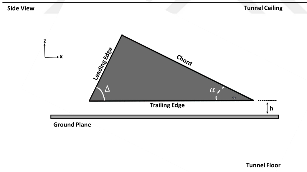
Figure A - 3 Side view of the anhedral reverse delta wing at effective angle of attack value
