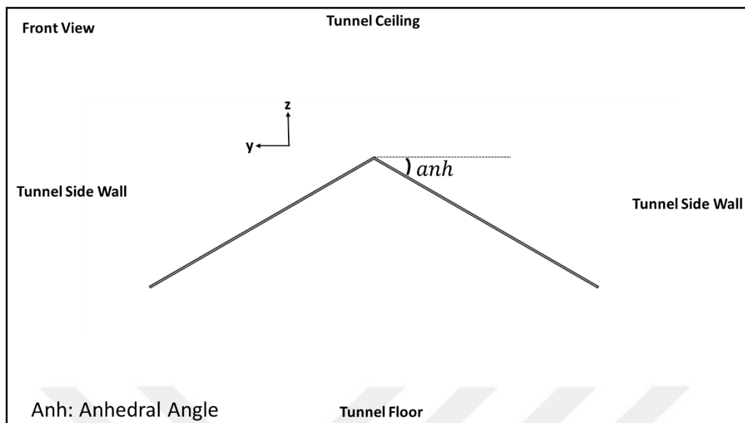
Figure A - 2 The front view of the anhedral reverse delta wing
