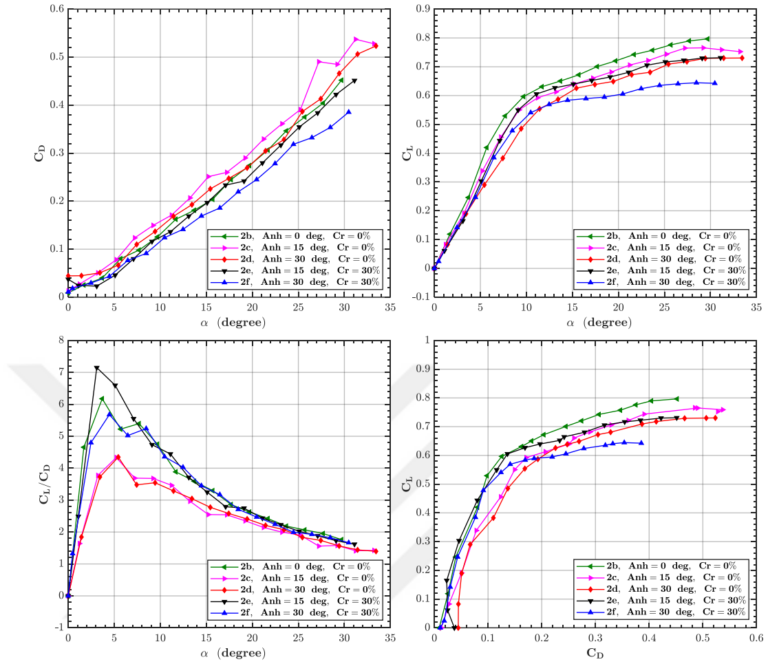
Figure 4-5 Distributions of drag coefficient C_D , lift-to-drag ratio C_L/C_D , lift coefficient C_L as a function of angle of attack and drag polar for different reverse delta wing configurations (2b), (2c), (2d), (2e), (2f)
