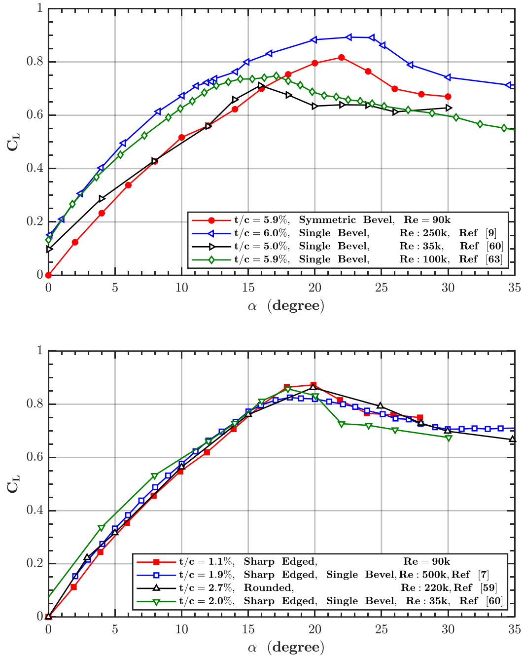
Figure 3-27 The comparison of lift coefficient of thick (1a) and thin (1b) delta wings with the results of [7], [9], [59], [60], and [63].
