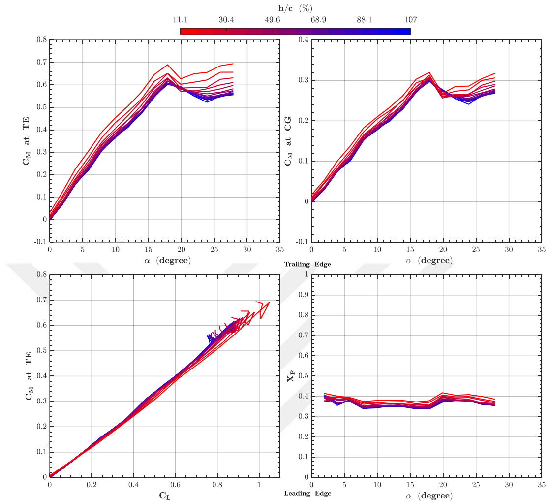
Figure 4-11 Variation of Moment coefficient C_M at trailing-edge (TE) and center of gravity (CG) as a function of angle of attack and Lift coefficient C_L , and Non-Dimensional Pressure Center coordinate X_P as a function of angle of attack for the delta wing 1b
