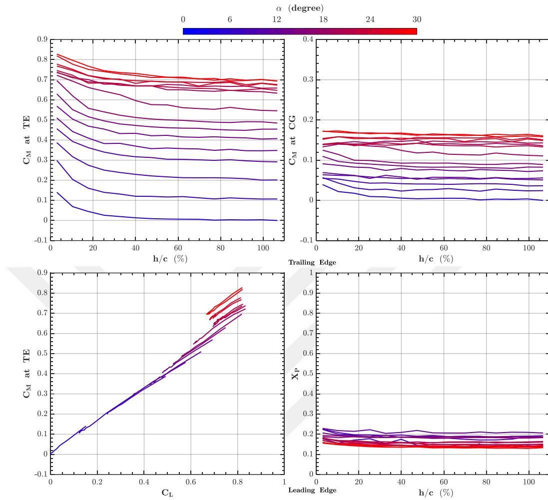
Figure C - 6 Variation of Moment coefficient C_M at trailing-edge (TE) and center of gravity (CG) as a function of function of non-dimensional height values and Lift coefficient C_L , and Non-Dimensional Pressure Center coordinate X_P as a function of non-dimensional height values for the reverse delta wing 2a
