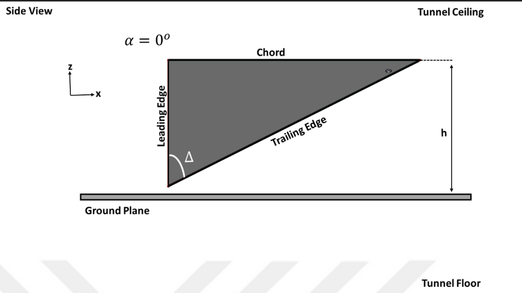
Figure A - 4 Side view of the anhedral reverse delta wing at zero angle of attack value
