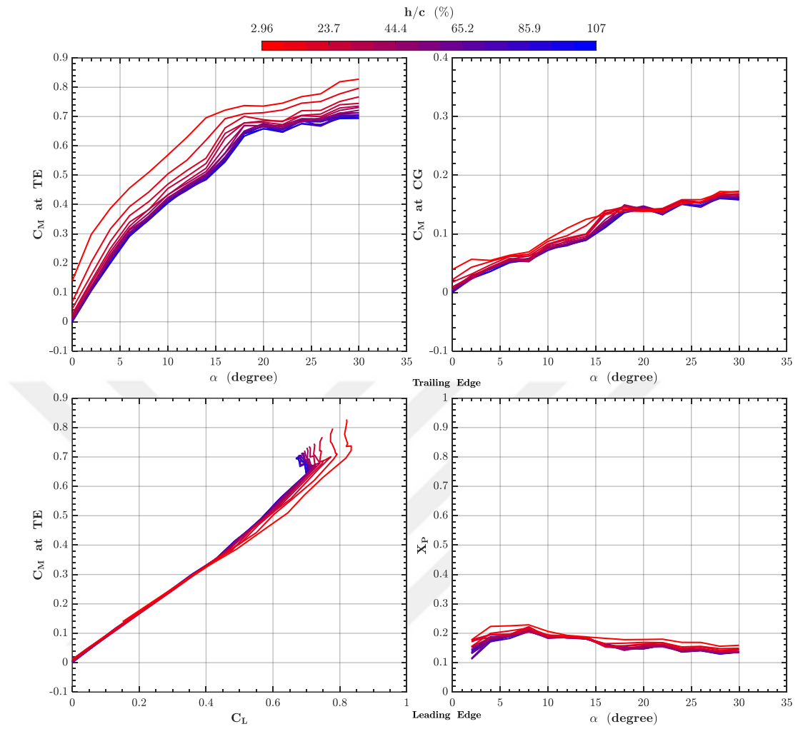
Figure 4-13 Variation of Moment coefficient C_M at trailing-edge (TE) and center of gravity (CG) as a function of angle of attack and Lift coefficient C_L , and Non-Dimensional Pressure Center coordinate X_P as a function of angle of attack for the reverse delta wing 2a
