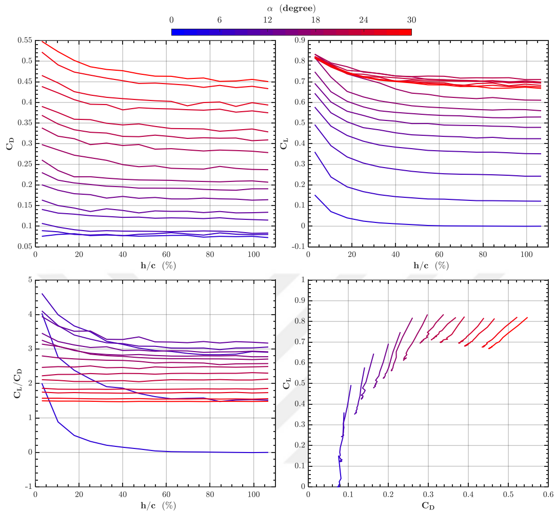
Figure C - 5 Variation of Drag coefficient C_D , Lift-to-Drag ratio C_L/C_D , Lift coefficient C_L as a function of non-dimensional height values and Drag Polar for the reverse delta wing 2a
