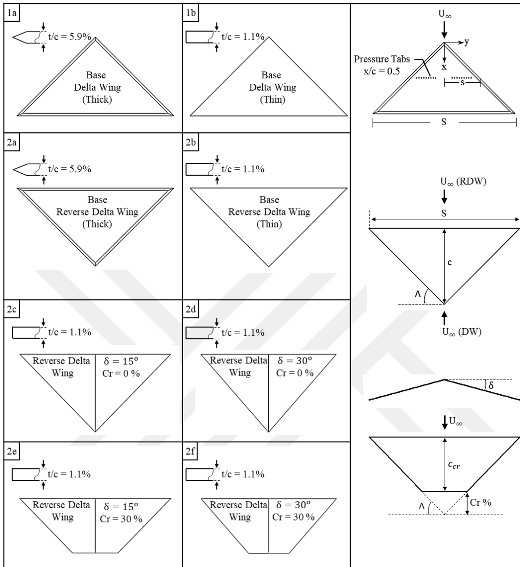
Figure 4-1 Schematic representations of the wings including delta wing, reverse delta wing, anhedral and cropped
