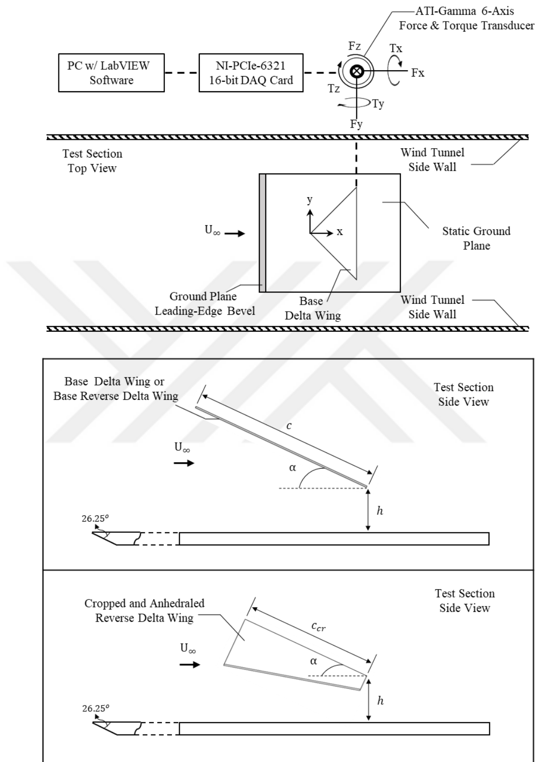
Figure 3-19 Schematic representations of the top and side views for the force measurement set-up
