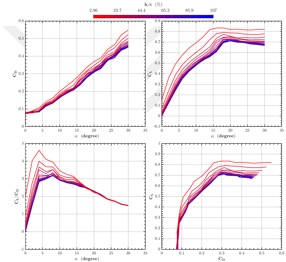
Figure 4-12 Variation of Drag coefficient C_D , Lift-to-Drag ratio C_L/C_D , Lift coefficient C_L as a function of angle of attack and Drag Polar for the reverse delta wing 2a
