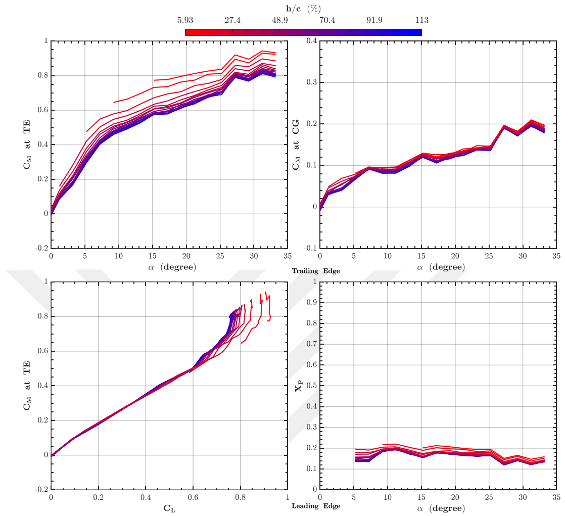
Figure 4-17 Variation of Moment coefficient C_M at trailing-edge (TE) and center of gravity (CG) as a function of angle of attack and Lift coefficient C_L , and Non-Dimensional Pressure Center coordinate X_P as a function of angle of attack for the reverse delta wing 2c
