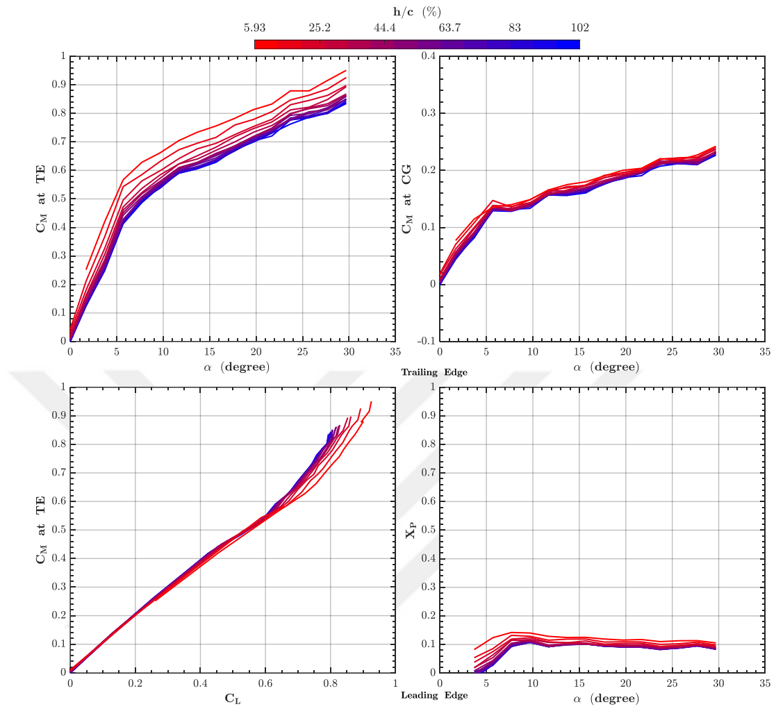
Figure 4-15 Variation of Moment coefficient C_M at trailing-edge (TE) and center of gravity (CG) as a function of angle of attack and Lift coefficient C_L , and Non-Dimensional Pressure Center coordinate X_P as a function of angle of attack for the reverse delta wing 2b
