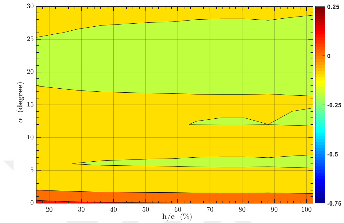
Figure 4-26 Height stability H.S. with respect to angle of attack and non-dimensional height for the delta wing 1a
