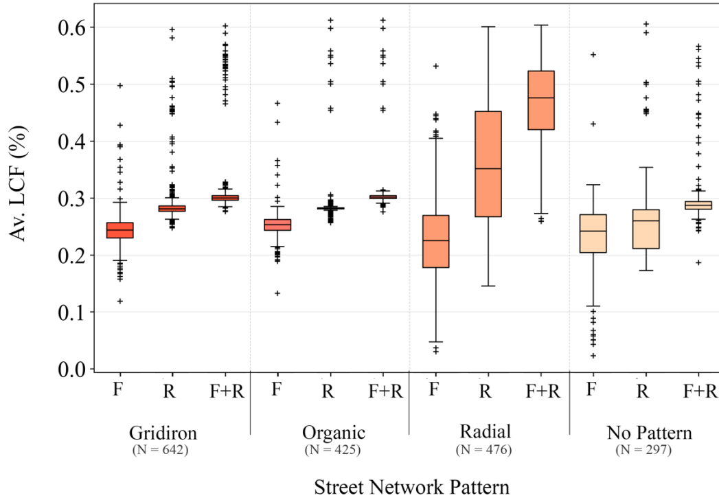
Figure 5.13 Building LCF for three BIPV applications, roof (R), façade (F) and roof and façade (R+F).
