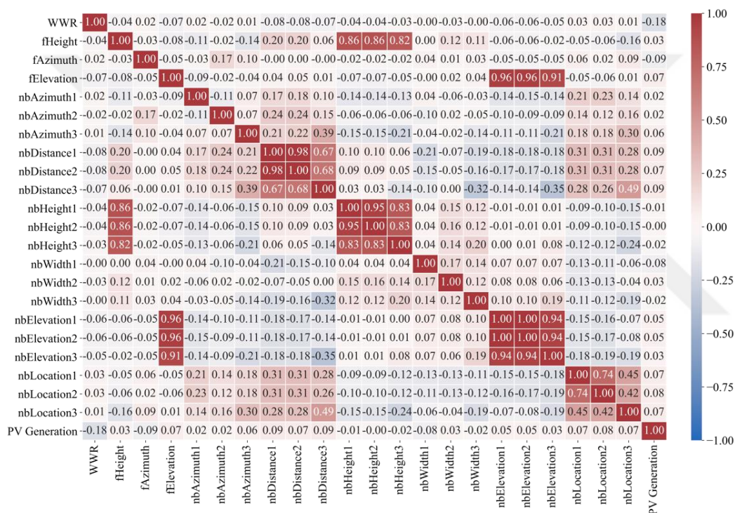
Figure 5.15 Correlations between the basic and output features for facades.
