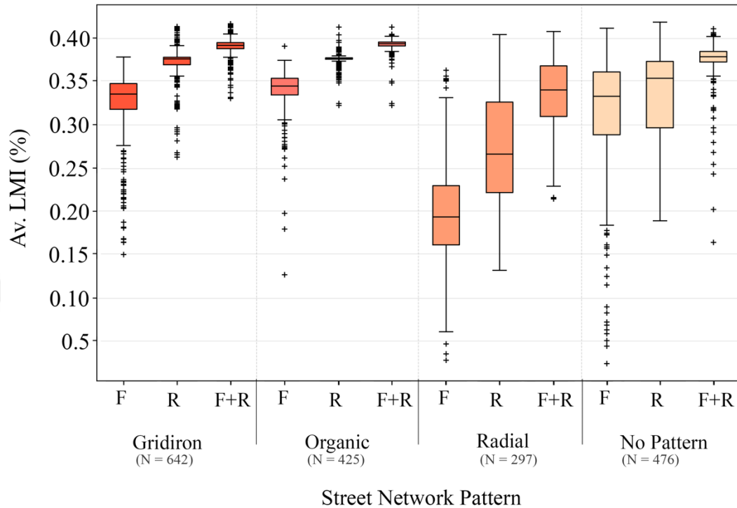
Figure 5.12 Building LMI for three BIPV applications, roof (R), façade (F) and roof and façade (R+F).
