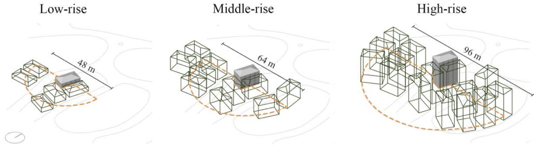
Figure 4.1 Context geometries included in shading analysis.
