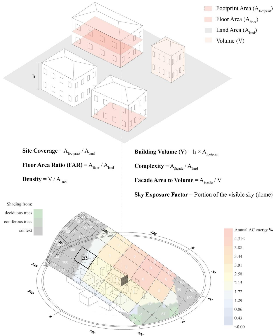
Figure 5.8 Studied urban morphology indicators.
