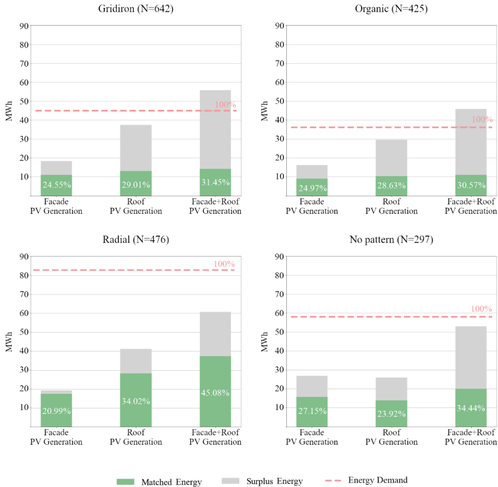
Figure 5.11 Matched and surplus energy for a year.
