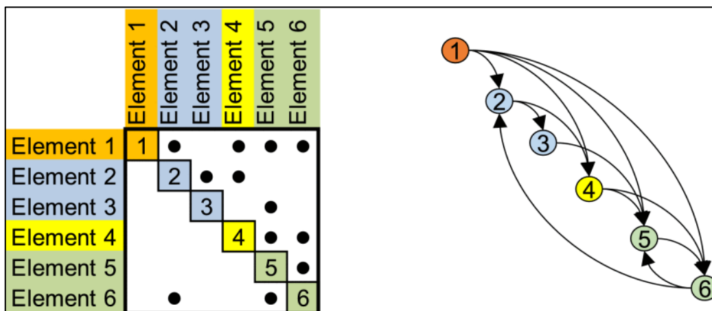
Figure 3.10. DSM matrix and its equivalent node-link diagram (Tyson R. Browning, 2016)
