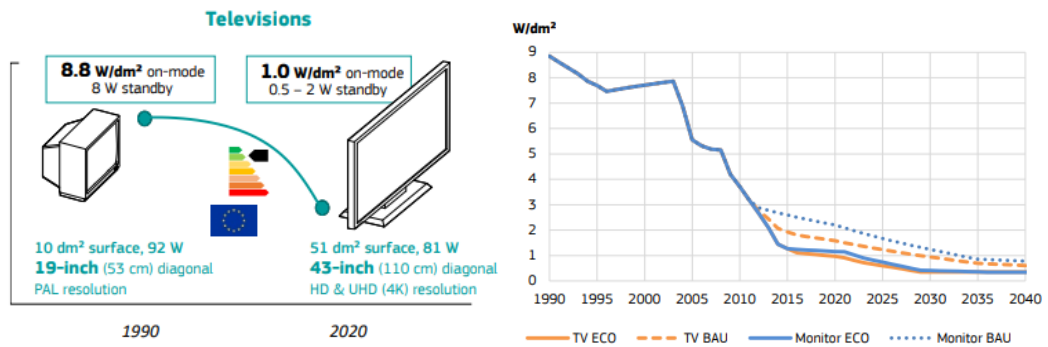
Figure 24. Energy consumptions in on-mode and standby
