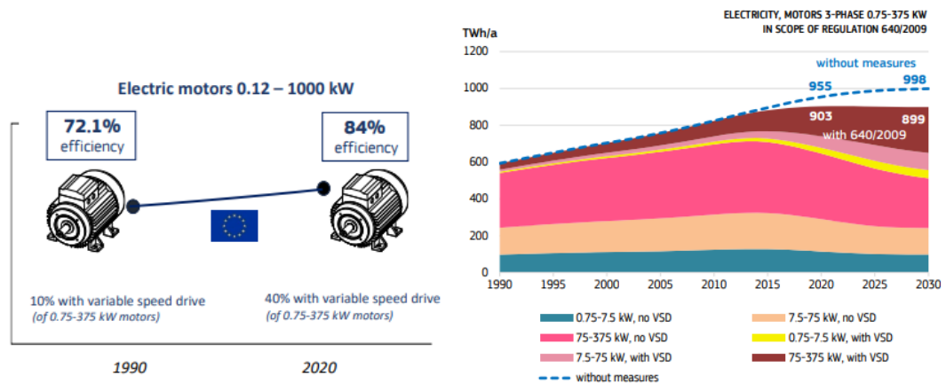
Figure 29. Efficiency of Motors
