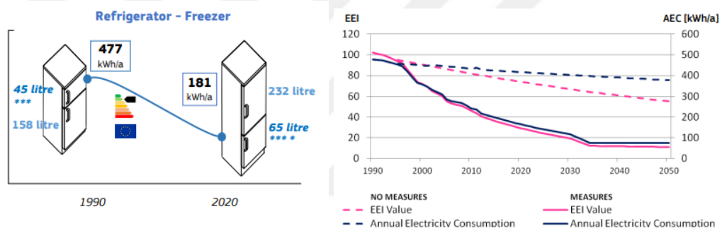
Figure 25. Energy consumptions and EEI value
