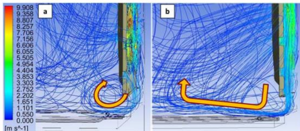
Figure 63. Airflows before (a) and after (b)
