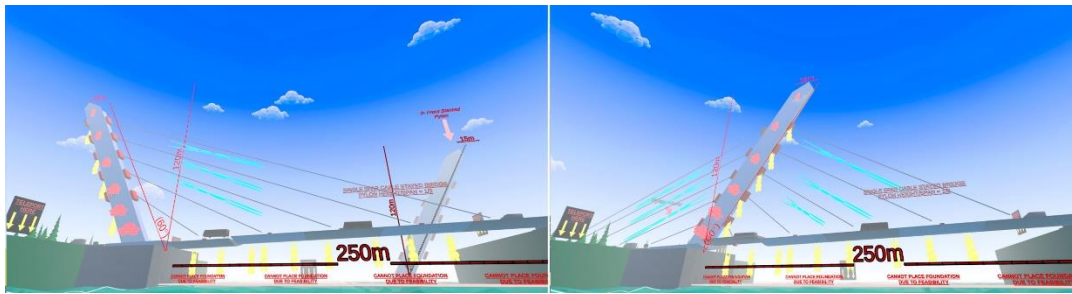
Figure 3.19. Back and front leaning single spar bridges under loading
