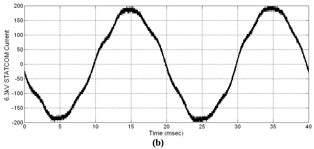
Figure 4.30 STATCOM Voltages and Currents at 6.3 kV a: Line-to-Line Voltage ; b : Line Current
