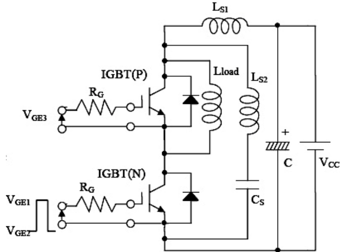
Figure 3.13 Switching Test Circuitry
