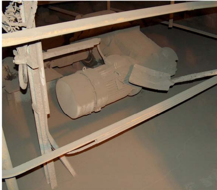
Figure 3.4 Belt Conveyor Motors with Excessive Coal Dust
