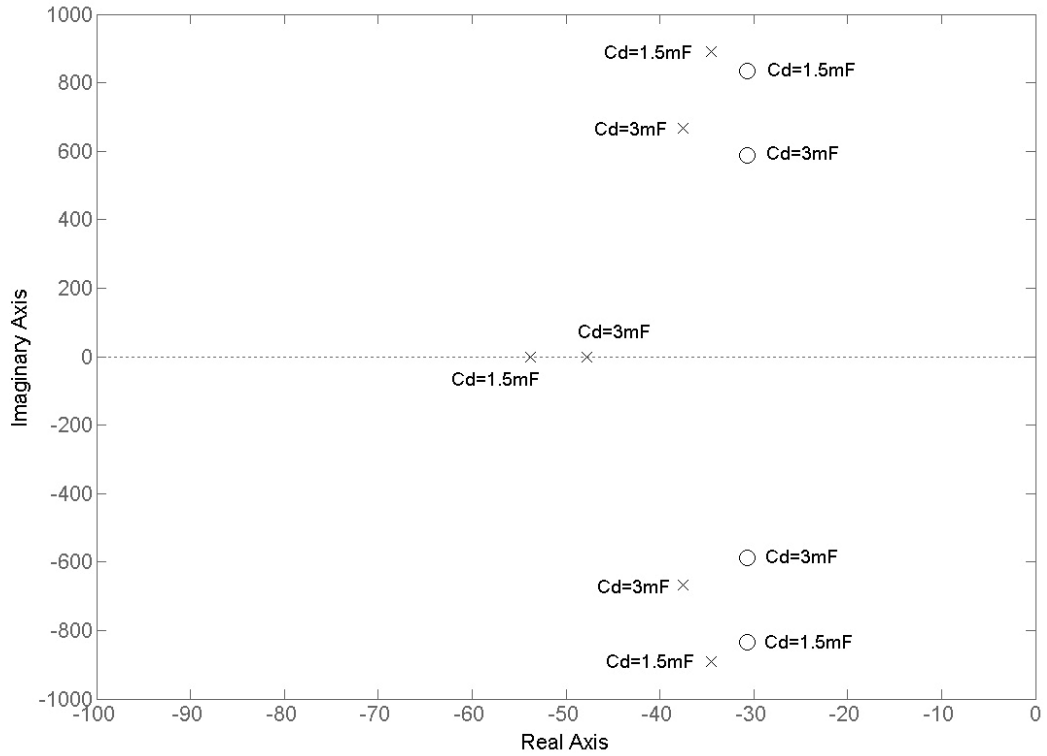
Figure 3.47 Effect of DC Link Capacitor on the Root Locus of Open Loop Transfer Function of STATCOM
