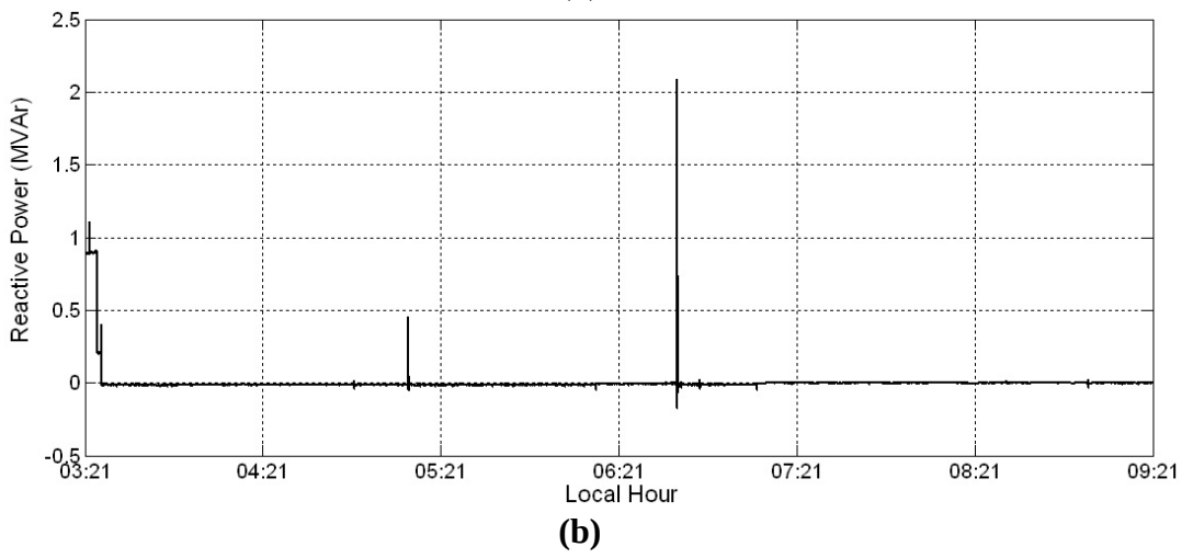
Figure 4.31 Measured Reactive Powers A : Load and STATCOM Reactive Power ; b : 31.5kV Source Reactive Power
