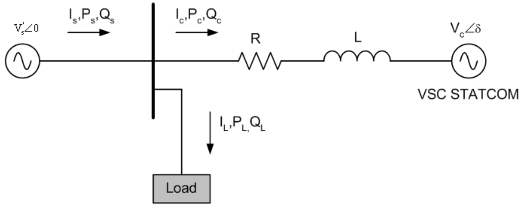
Figure 2.3 Simplified Model of STATCOM
