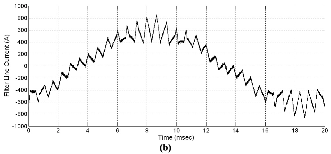
Figure 4.22 Input Filter Capacitor Line Current a : Capacitive Operation Mode ; b: Inductive Operation Mode
