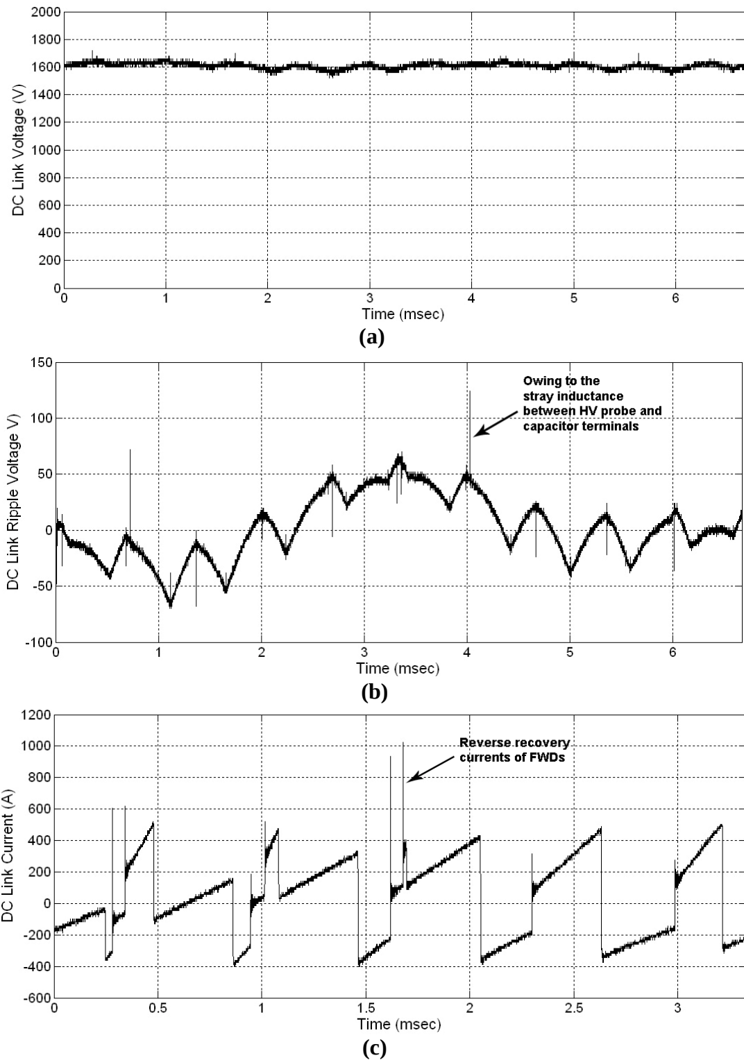
Figure 4.17 DC Link Voltage and Current Waveforms in Capacitive Operation Mode a : DC Link Voltage ; b: DC Link Ripple Voltage c : DC Link Current
