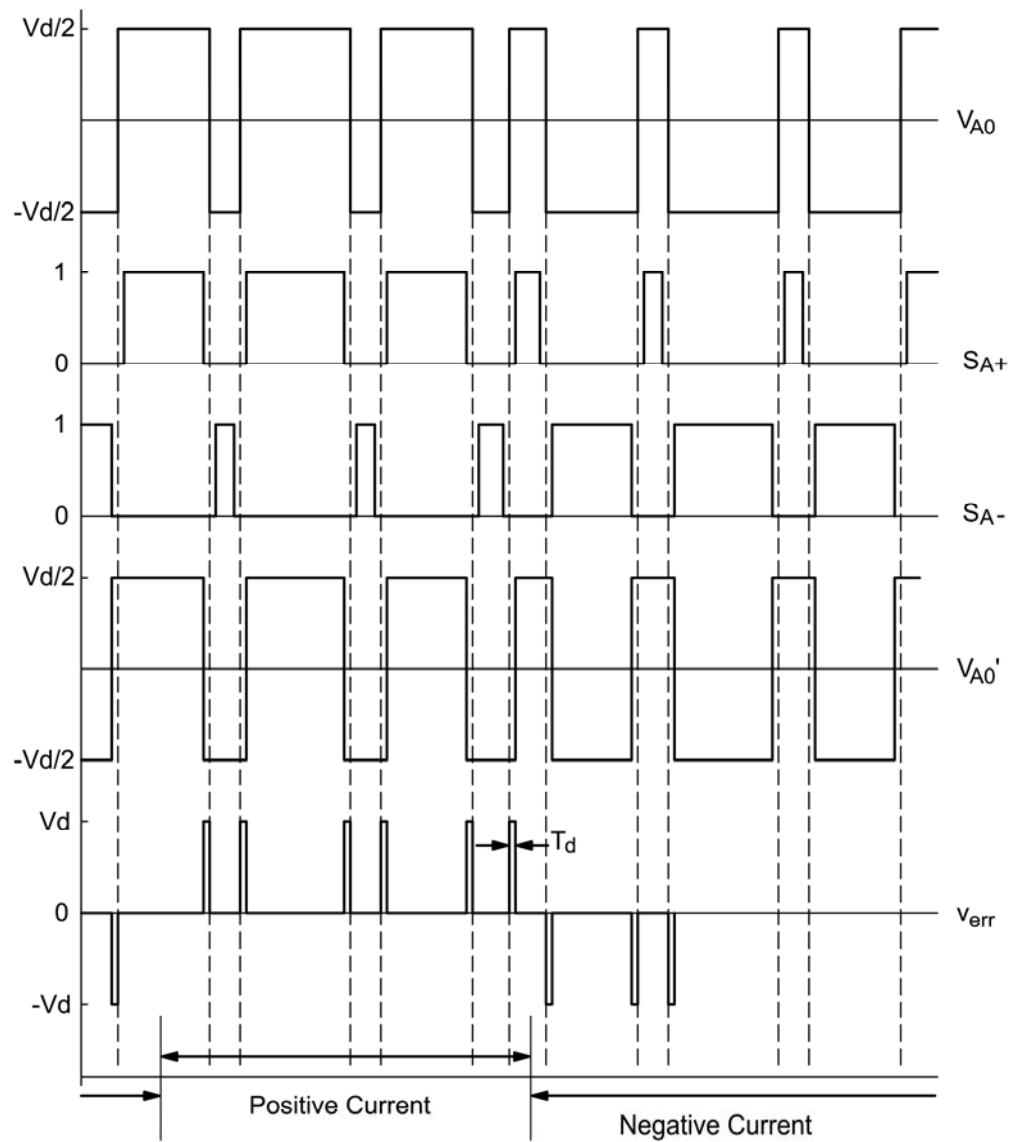
Figure 3.63 Practical Waveforms With Dead Time
