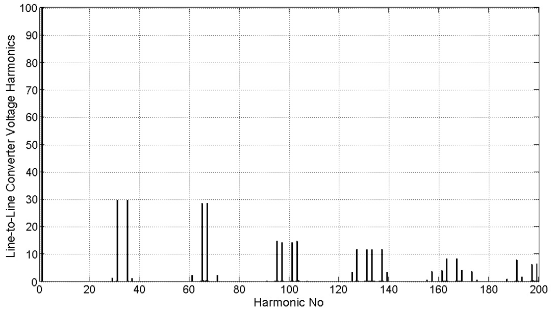
Figure 2.16 Converter Output Voltage Harmonics as a Percentage of Fundamental Component (SPWM with m_a=0.9 and m_f=33 )
