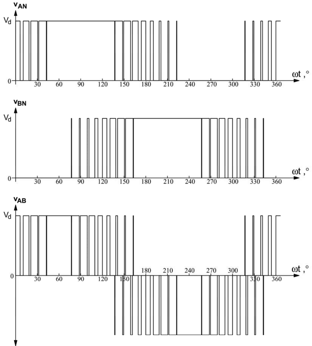
Figure 2.33 Converter Voltages for 8-Angle SHEM
