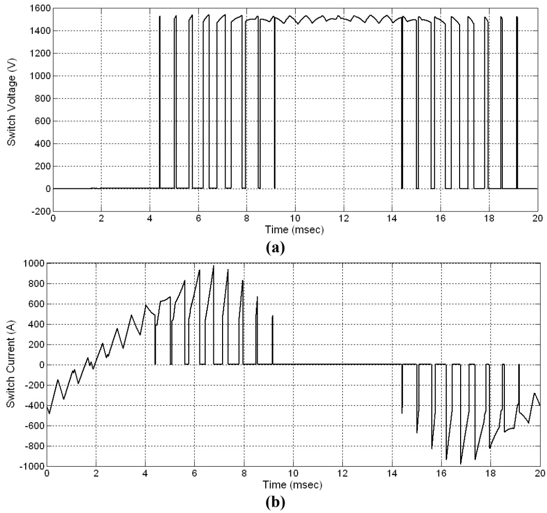
Figure 3.10 Switching Waveforms of Power Semiconductor a : Switch Voltage ; b : Switch Current (PSCAD/EMTDC)
