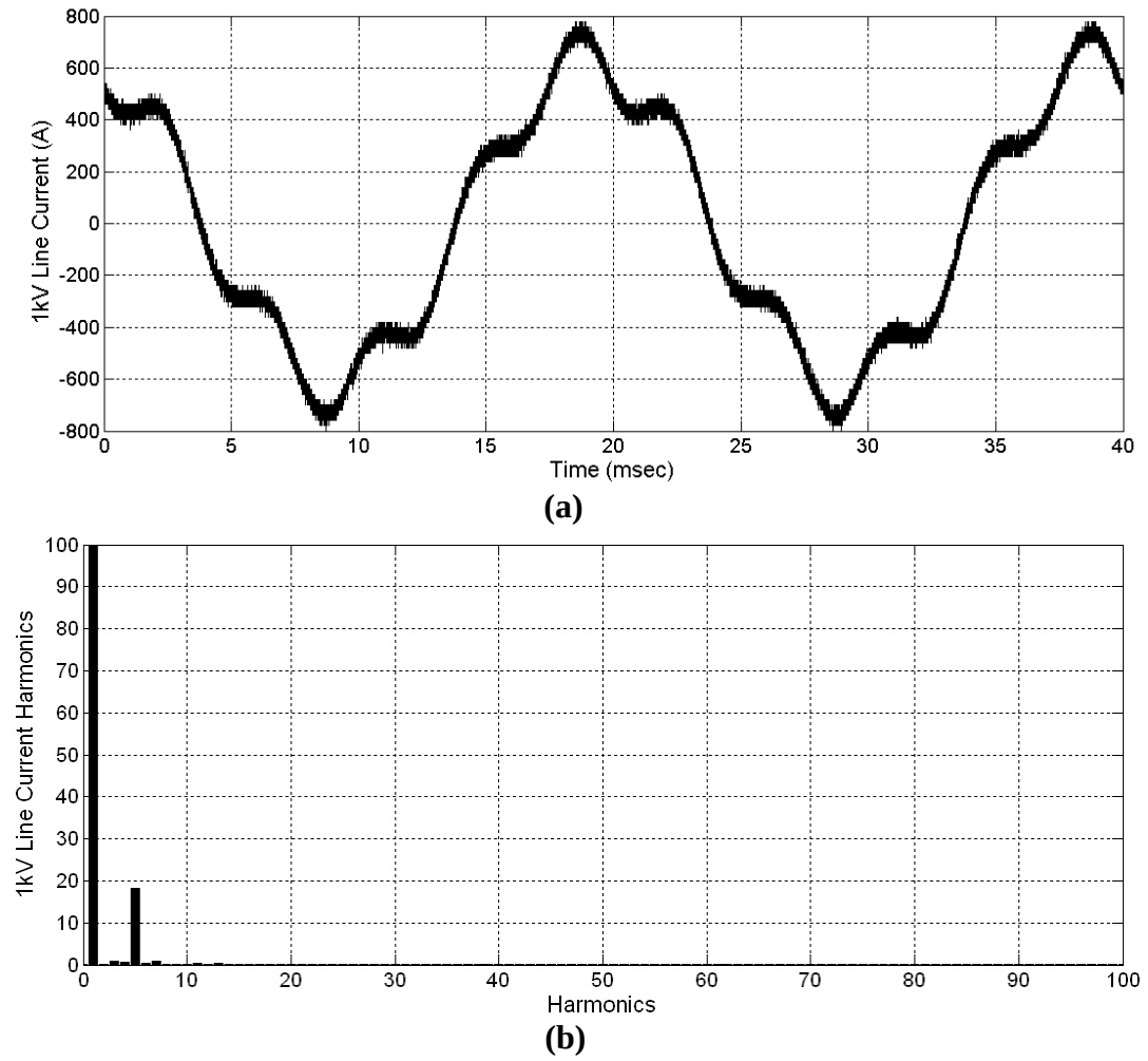
Figure 4.26 1kV Line Current when VSC is disconnected from 1kV bus a: Waveform ; b : Harmonic Spectra
