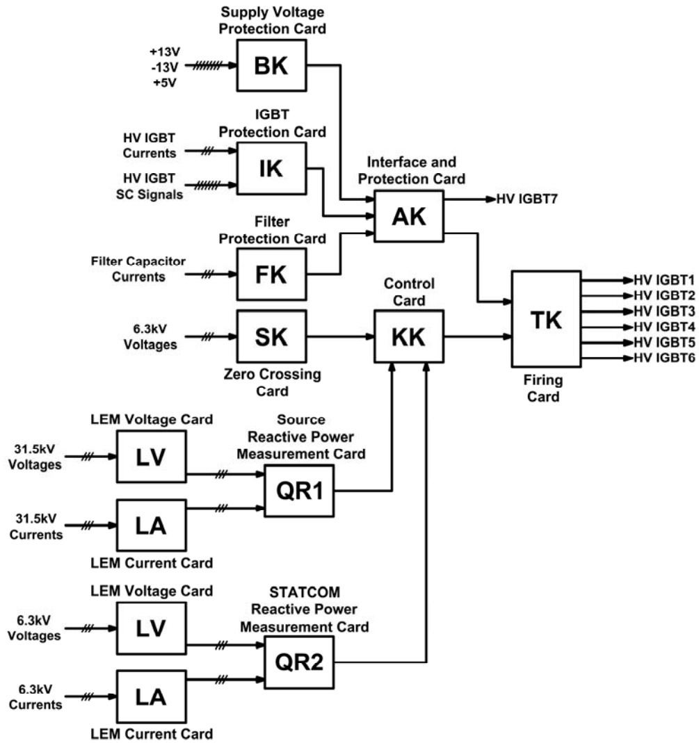
Figure 3.59 Block Diagram of Control System
