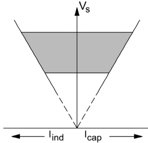
Figure 1.2 V-I Characteristic of SVCs
