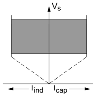
Figure 3.8 Current-Voltage Characteristic of STATCOM
