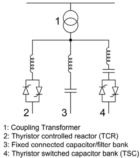
Figure 1.1 SVC Examples
