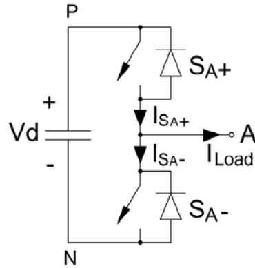
Figure 2.22 One-Leg Converter
