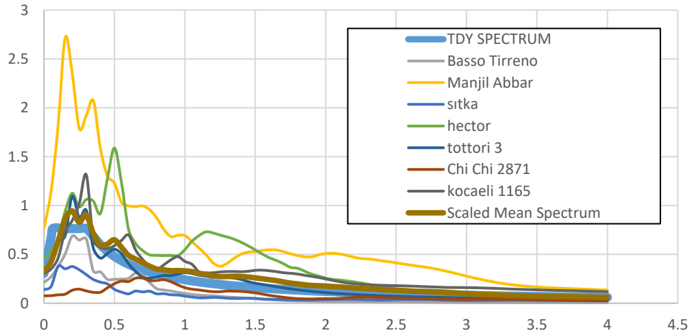
Figure B.6. TDY 2020 design spectrum and response spectrum of scaled time histories for ground motion SET-1 and scaling method M1 of V03 Bridge
