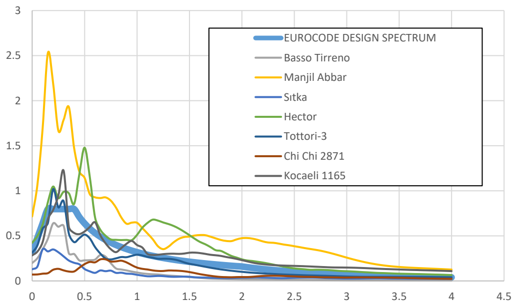
Figure B.4711. EN-8 design spectrum and response spectrum of unscaled time histories for ground motion SET-1 and scaling method M1 of V14 Bridge
