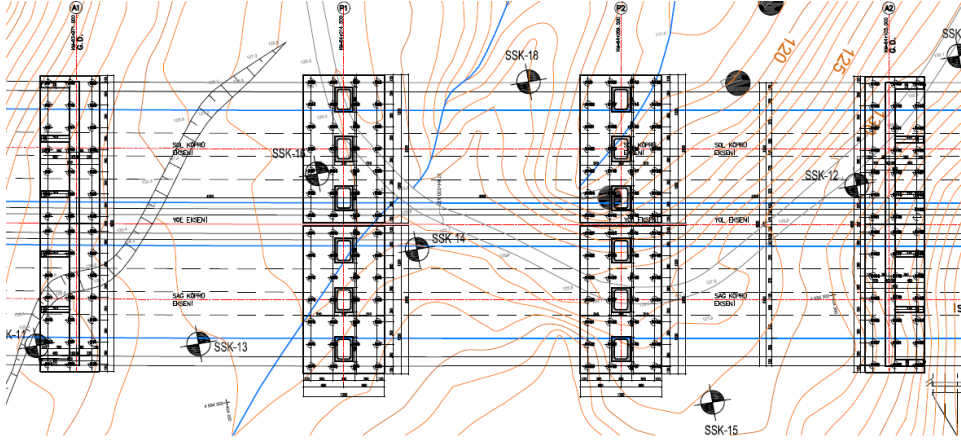
Figure 3.13. Plan view of V14 Bridge
