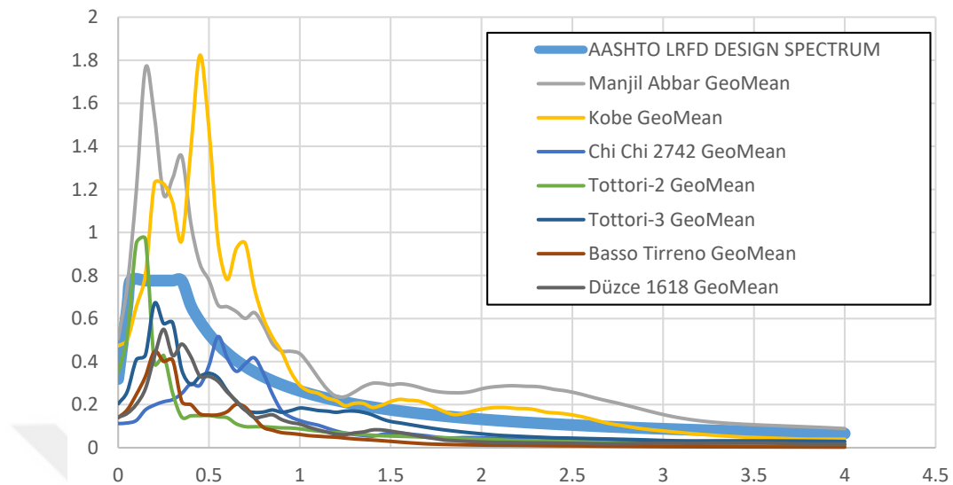
Figure B.5521. AASHTO LRFD design spectrum and response spectrum of unscaled time histories for ground motion SET-3 and scaling method M1 of V14 Bridge
