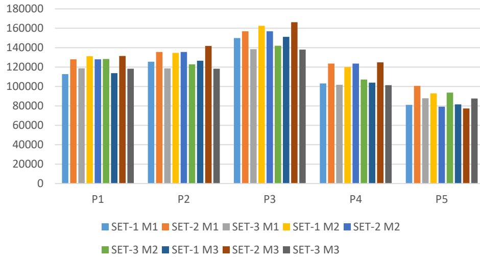
Figure 4.31. M_x values of all of the pier columns for three scaling methods applied according to EN-8 (kN.m)
