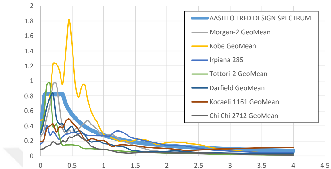
Figure B.61. AASHTO LRFD design spectrum and response spectrum of unscaled time histories for ground motion SET-2 and scaling method M1 of V08 Bridge
