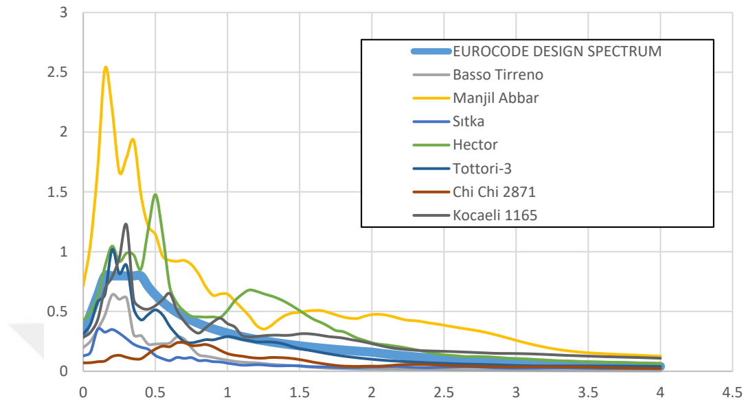
Figure B.129. EN-8 design spectrum and response spectrum of unscaled time histories for ground motion SET-1 and scaling method M2 of V14 Bridge
