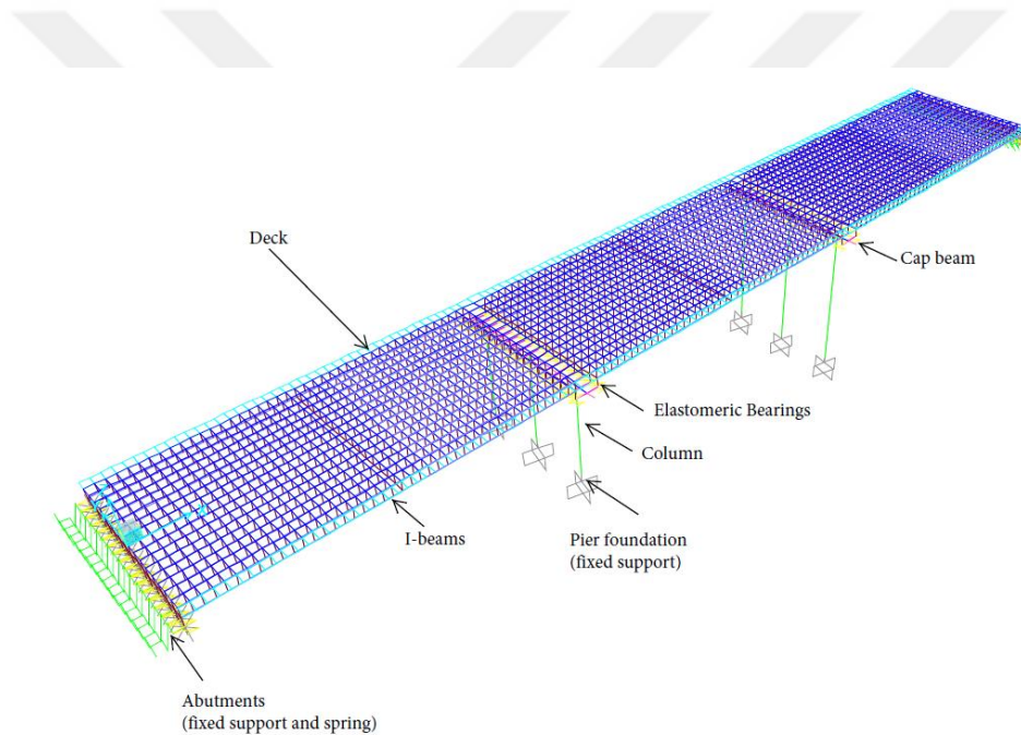
Figure 3.20. Representation of bridge elements
