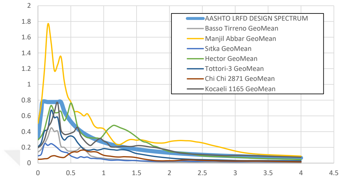
Figure B.4509. AASHTO LRFD design spectrum and response spectrum of unscaled time histories for ground motion SET-1 and scaling method M1 of V14 Bridge
