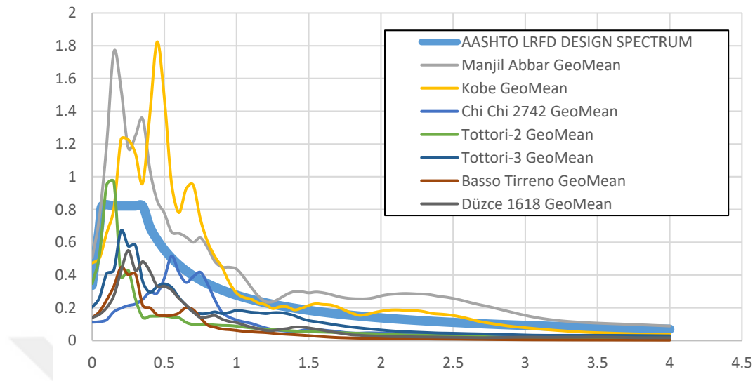
Figure B.85. AASHTO LRFD design spectrum and response spectrum of unscaled time histories for ground motion SET-3 and scaling method M2 of V08 Bridge
