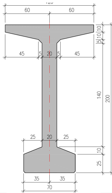
Figure 3.17. Cross section of the beam
