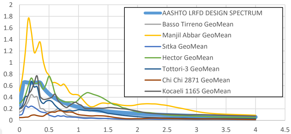
Figure B.1. AASHTO LRFD design spectrum and response spectrum of unscaled time histories for ground motion SET-1 and scaling method M1 of V03 Bridge
