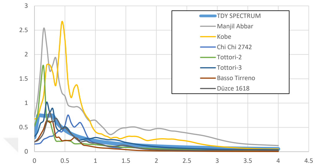
Figure B.89. TDY 2020 design spectrum and response spectrum of unscaled time histories for ground motion SET-3 and scaling method M2 of V08 Bridge
