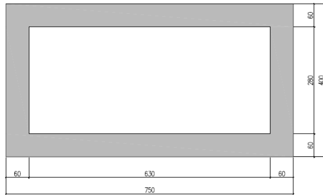
Figure 3.12. Cross section of the column
