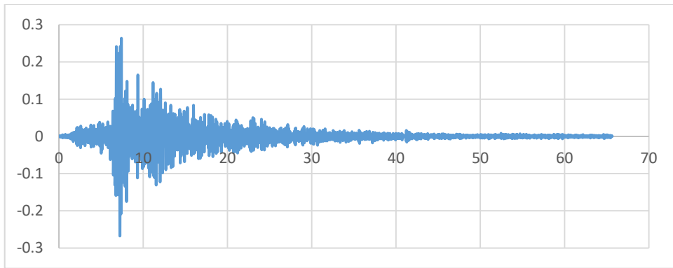
Figure A.40. Accelerogram of Tottori-2 earthquake in y-direction (SET-3)
