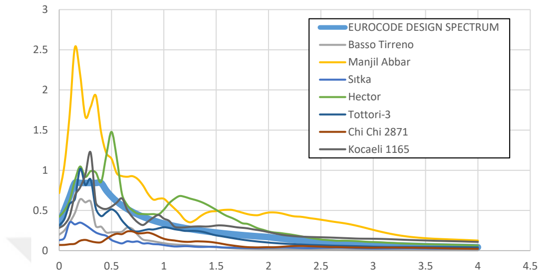
Figure B.93. EN-8 design spectrum and response spectrum of unscaled time histories for ground motion SET-1 and scaling method M3 of V08 Bridge
