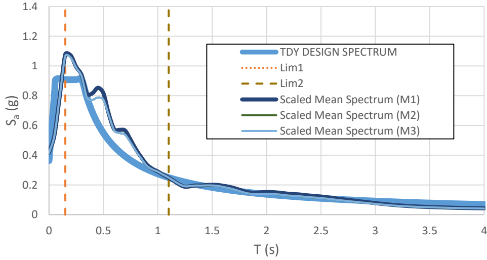
Figure 4.42. Scaled mean spectra for M1,M2 and M3 and TDY design response spectrum for SET-3
