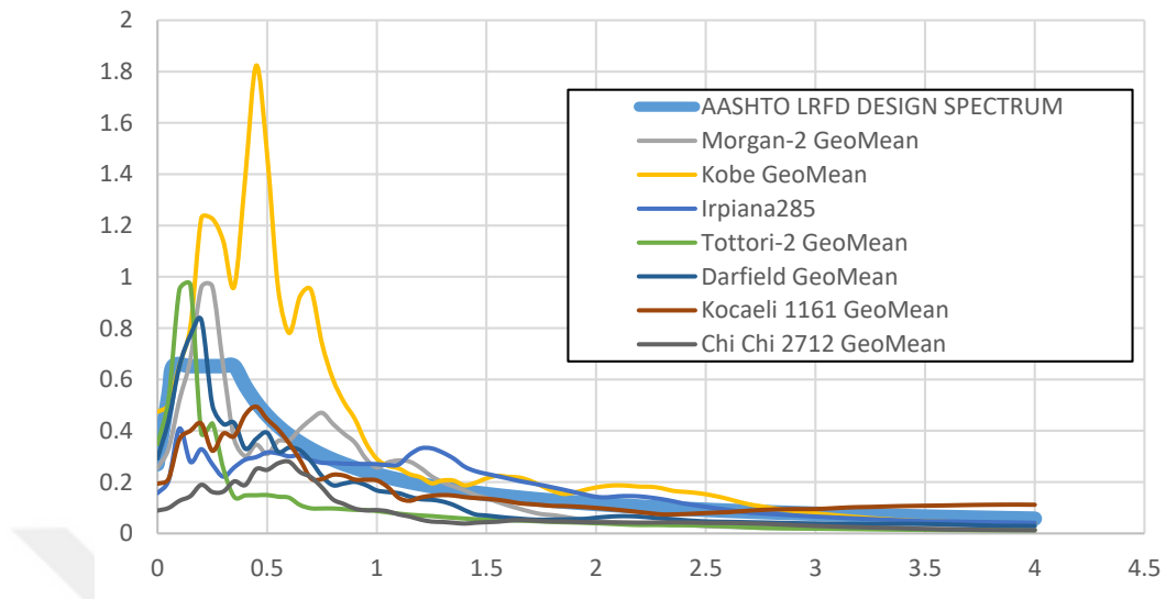
Figure B.25. AASHTO LRFD design spectrum and response spectrum of unscaled time histories for ground motion SET-2 and scaling method M2 of V03 Bridge
