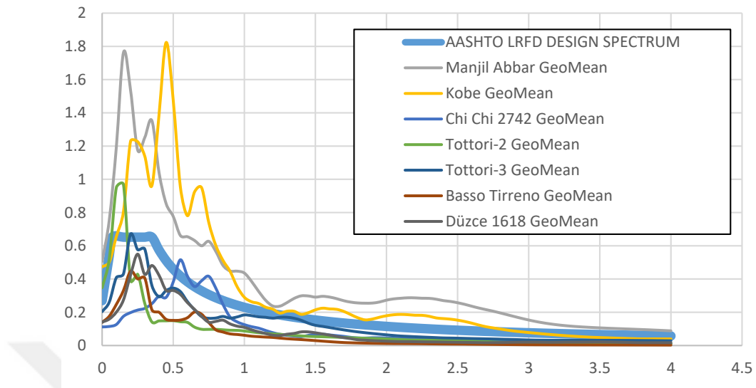
Figure B.49. AASHTO LRFD design spectrum and response spectrum of unscaled time histories for ground motion SET-3 and scaling method M3 of V03 Bridge
