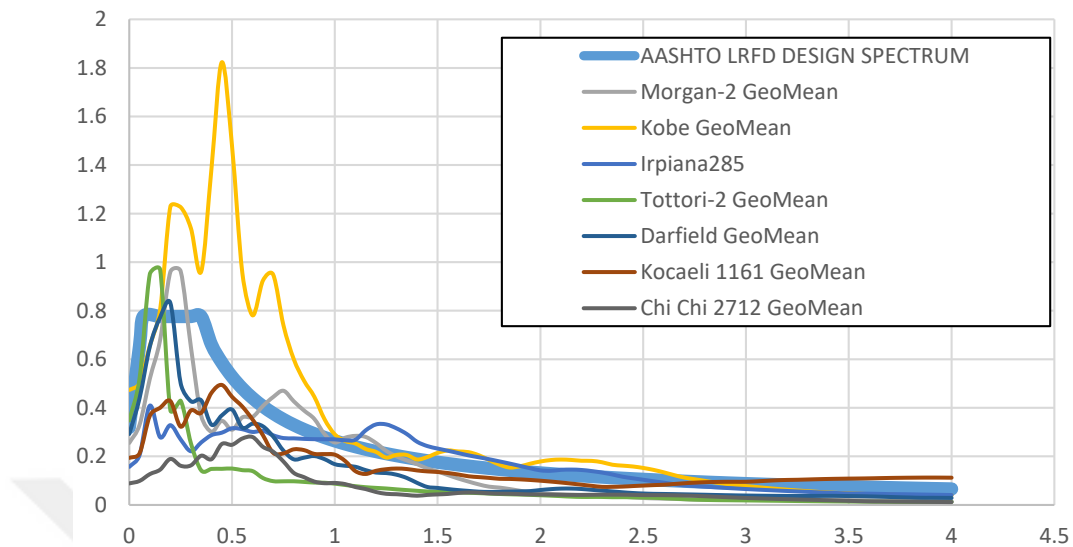
Figure B.6433. AASHTO LRFD design spectrum and response spectrum of unscaled time histories for ground motion SET-2 and scaling method M2 of V14 Bridge
