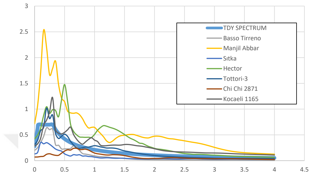
Figure B.7949. TDY 2020 design spectrum and response spectrum of unscaled time histories for ground motion SET-1 and scaling method M3 of V14 Bridge
