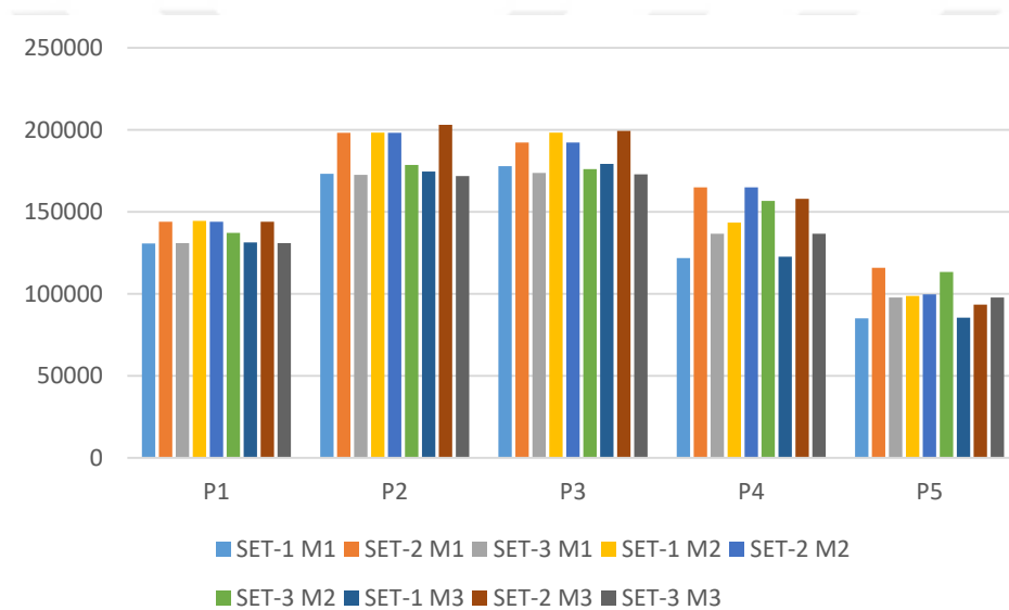
Figure 4.30. M_y values of all of the pier columns for three scaling methods applied according to EN-8 (kN.m)
