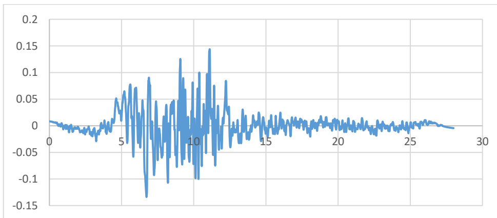
Figure A.24. Accelerogram of Kocaeli_1161 earthquake in y-direction (SET-2)
