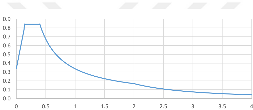
Figure 3.40. Eurocode-8 design spectrum for V08 Bridge ( S_a(g) - T(s) )
