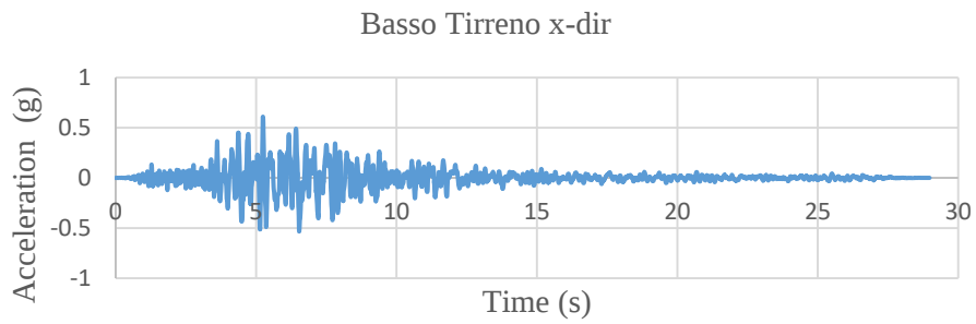
Figure 4.1 Unscaled accelerogram for Basso Tirreno earthquake
