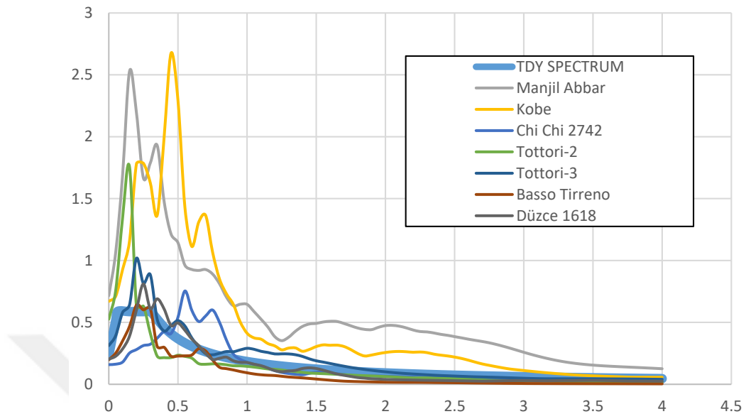
Figure B.53. TDY 2020 design spectrum and response spectrum of unscaled time histories for ground motion SET-3 and scaling method M3 of V03 Bridge
