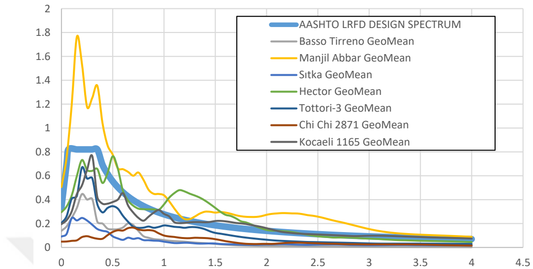
Figure B.73. AASHTO LRFD design spectrum and response spectrum of unscaled time histories for ground motion SET-1 and scaling method M2 of V08 Bridge
