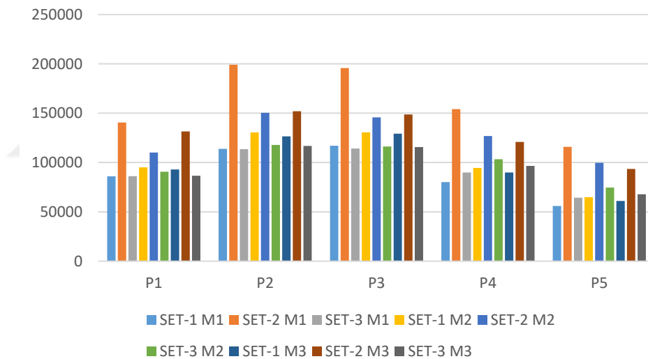
Figure 4.32. M_y values of all of the pier columns for three scaling methods applied according to TDY 2020 (kN.m)
