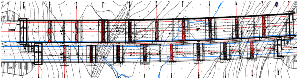
Figure 3.1. Plan view of V03 Bridge
