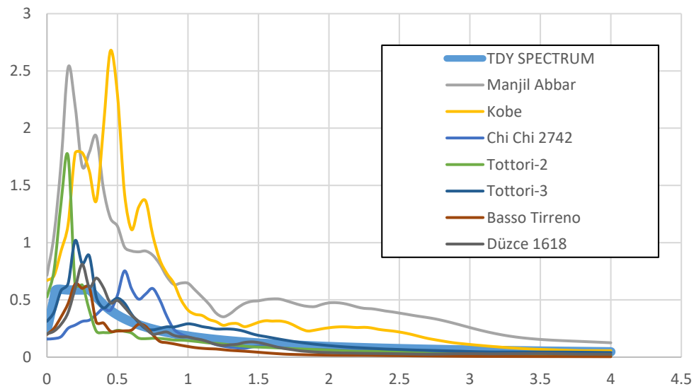
Figure B.35. TDY 2020 design spectrum and response spectrum of unscaled time histories for ground motion SET-3 and scaling method M2 of V03 Bridge
