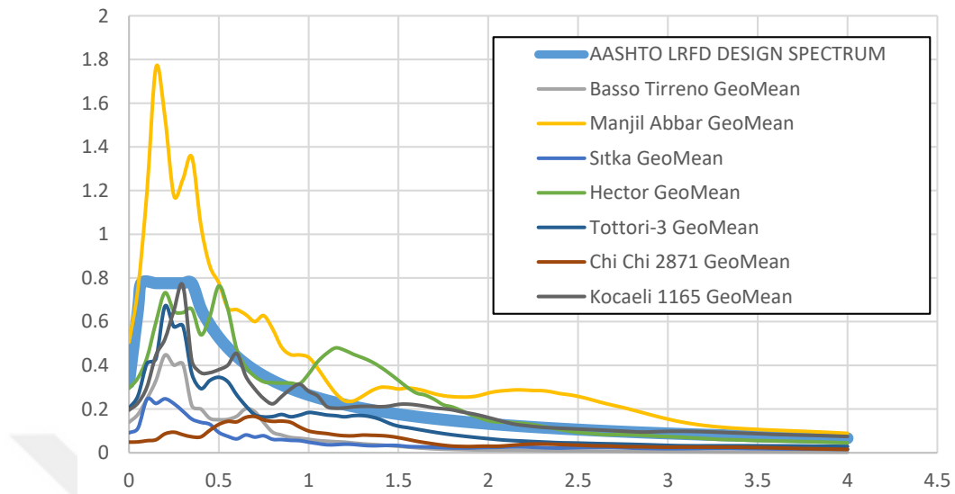
Figure B.7545. AASHTO LRFD design spectrum and response spectrum of unscaled time histories for ground motion SET-1 and scaling method M3 of V14 Bridge
