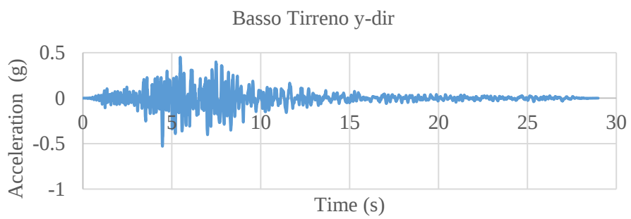
Figure 4.2. Scaled accelerogram for Basso Tirreno earthquake
