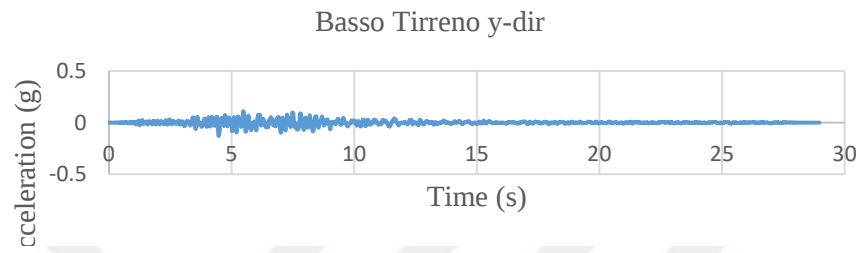
Figure 4.1 Unscaled accelerogram for Basso Tirreno earthquake
