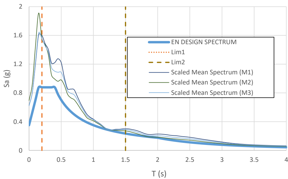
Figure 4.11. Scaled mean spectra for M1,M2 and M3 and EN 8 design response spectrum for SET-3
