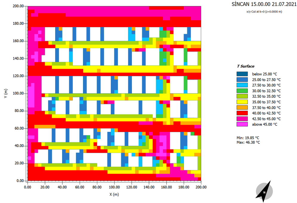
Figure D.14. T Surface Temperature (°C) of Urban Block 14 - Sincan
