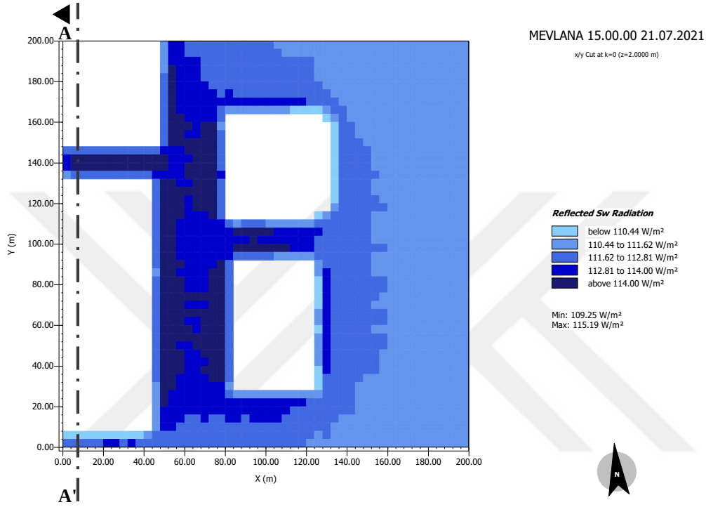
Figure 5.35. Reflected Shortwave Radiation ( \text{W/m}^2 ) in Mevlana Bulvarı Block at 21.07.2021, 15.00.00, plan view, 2 meters above the ground
