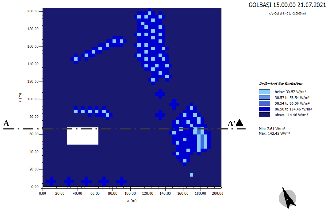
Figure 5.56. Reflected Shortwave Radiation ( \text{W/m}^2 ) in Gölbaşı at 21.07.2021, 15.00.00, plan view, z=2 meters
