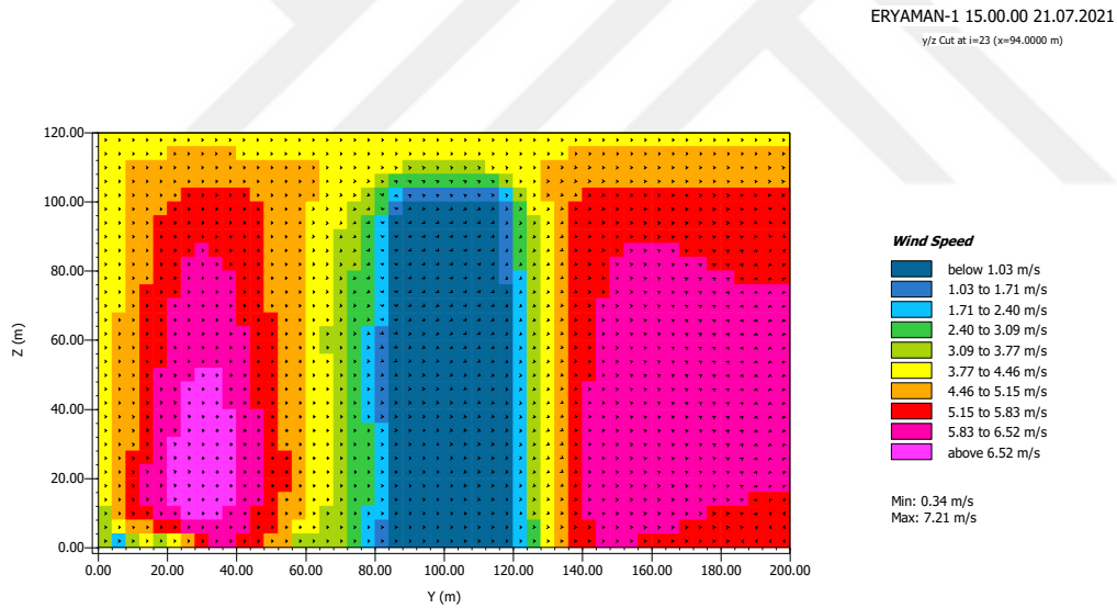
Figure 5.8. Wind speed values (m/s) for Eryaman-1 at 21.07.2021, 15.00.00, Section BB', cut at x=94 meters
