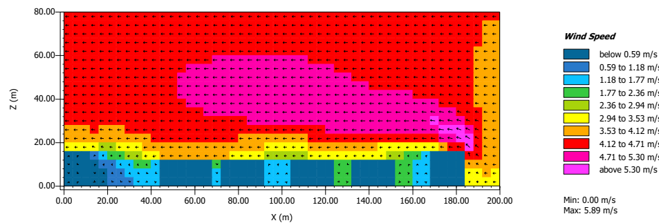
Figure 5.45. Wind speed values (m/s) for İvedik at 21.07.2021, 15.00.00, Section BB', cut at y=82 meters
