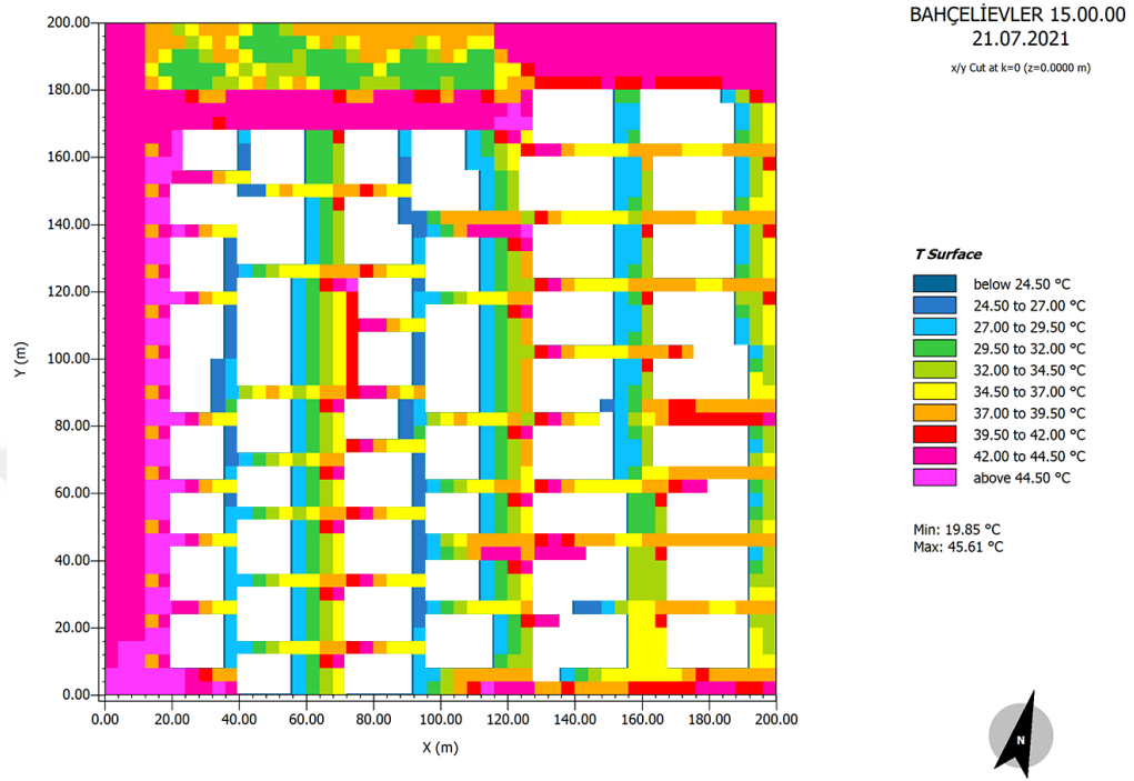
Figure 5.12. T surface values for Bahçelievler (°C) at 21.07.2021, 15.00.00, plan view, z=0 meters
