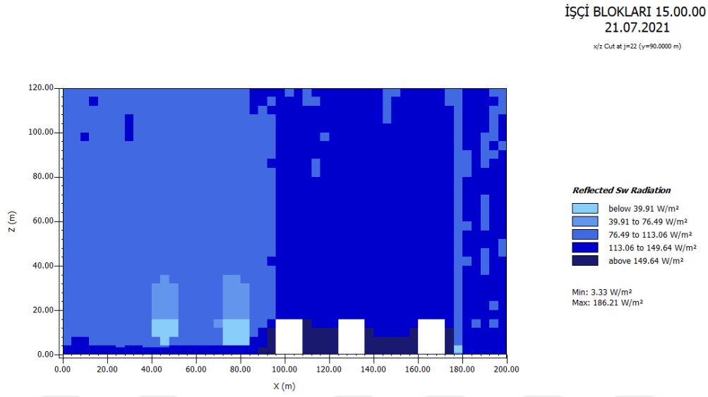
Figure 5.24. Reflected Shortwave Radiation (W/m 2 ) in İşçi Blokları at 21.07.2021, 15.00.00, Section AA', cut at y=90 meters
