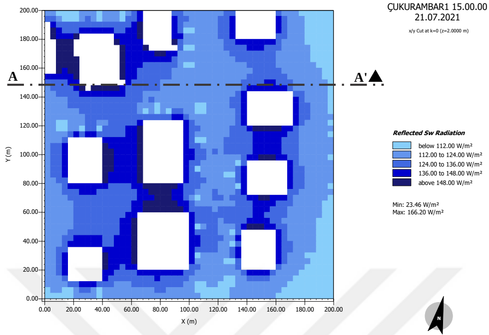
Figure 5.28. Reflected Shortwave Radiation (W/m 2 ) in Çukrambar 1 at 21.07.2021, 15.00.00, plan view, 2 meters above the ground
