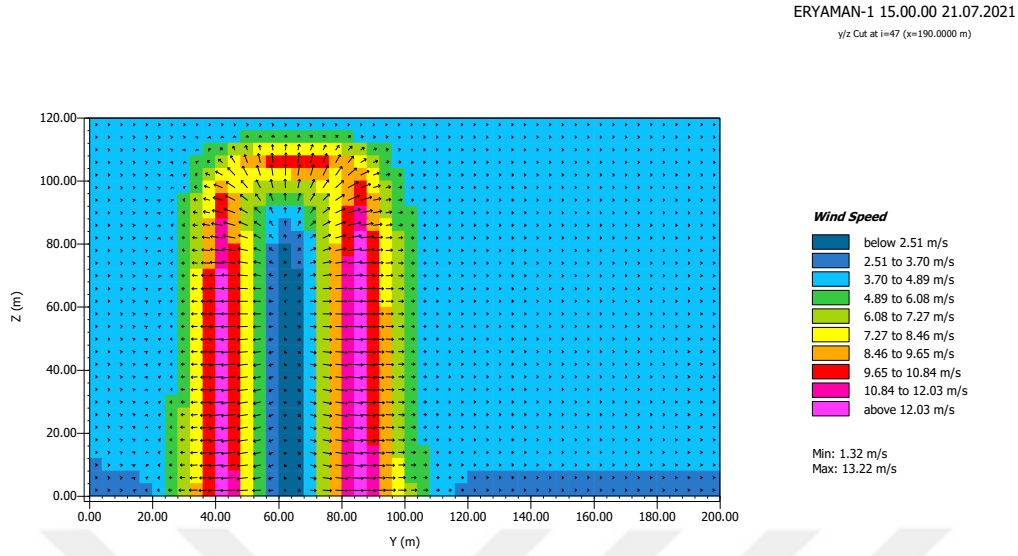
Figure 5.7. Wind speed values (m/s) for Eryaman-1 at 21.07.2021, 15.00.00, Section AA', cut at x=190 meters
