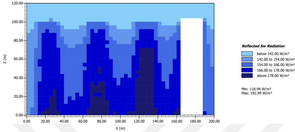
Figure 5.10. Section view of Reflected Shortwave Radiation ( \text{W/m}^2 ) in Eryaman-1 at 21.07.2021, 15.00.00, Section AA', cut at y=82 meters
