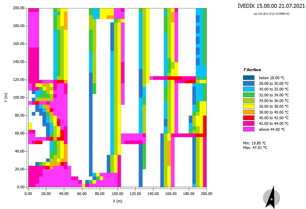
Figure D.11. T Surface Temperature (°C) of Urban Block 11 - İvedik
