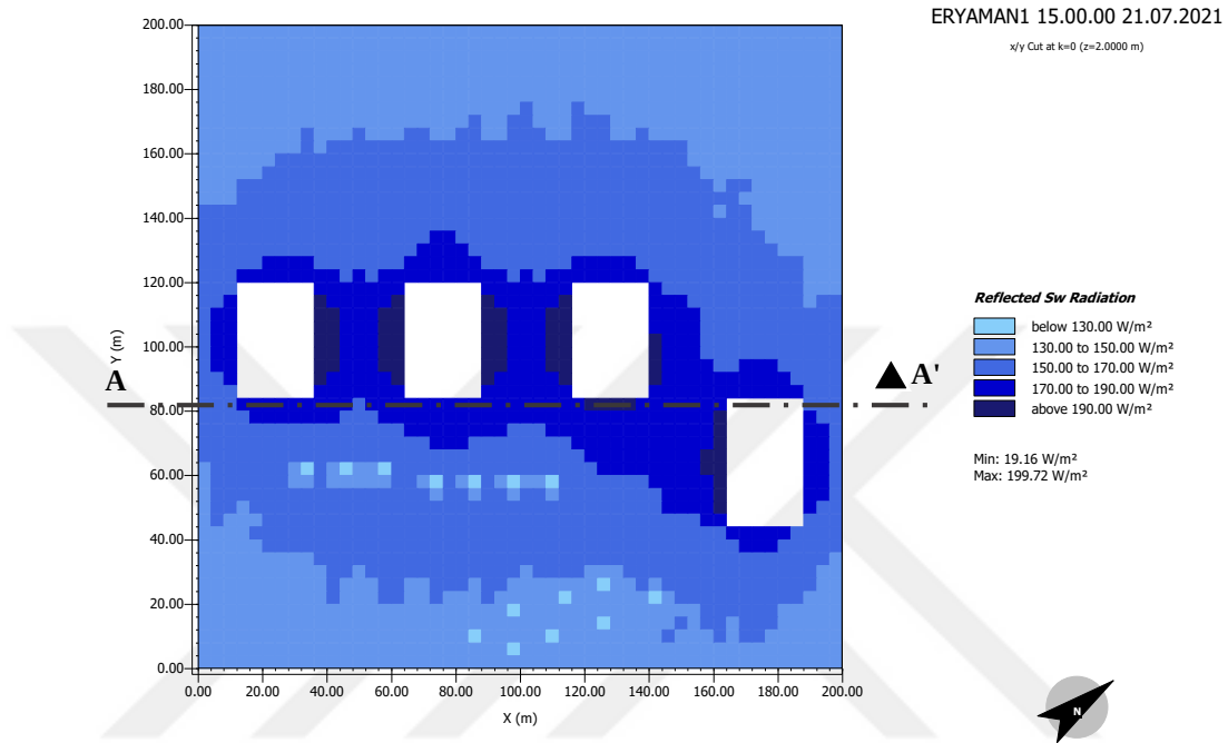
Figure 5.9. Plan view of Reflected Shortwave Radiation ( \text{W/m}^2 ) in Eryaman-1 at 21.07.2021, 15.00.00, plan view, 2 meters above the ground
