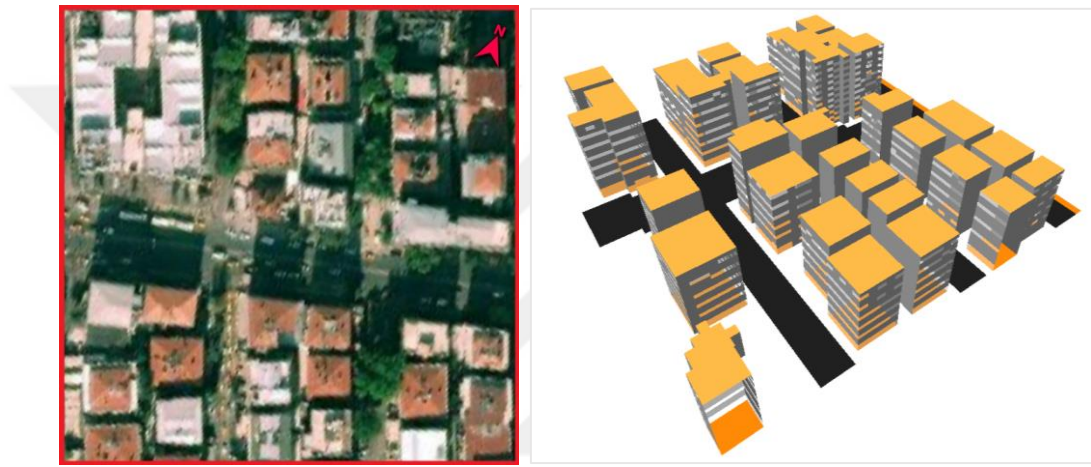
Figure 3.17. Satellite Image (left) and 3D Model (right) of the selected Urban Block 12 - Kızılay
