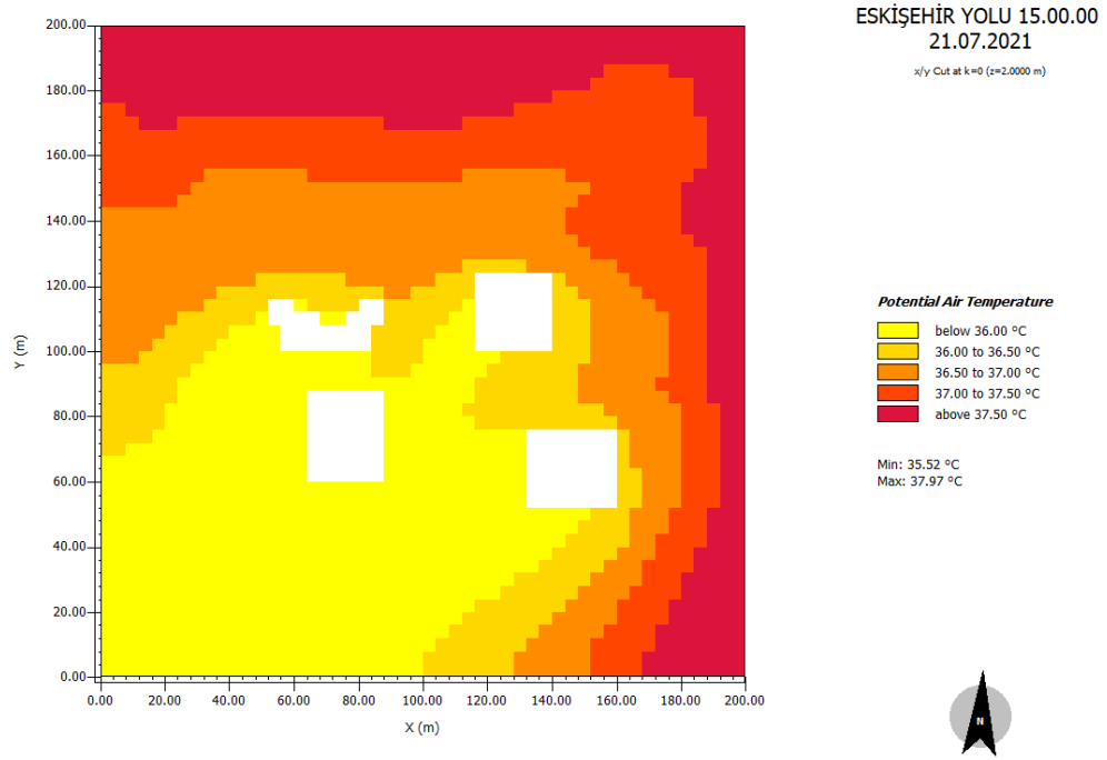
Figure D.23. Potential Air Temperature (°C) of Urban Block 7 - Eskişehir Yolu
