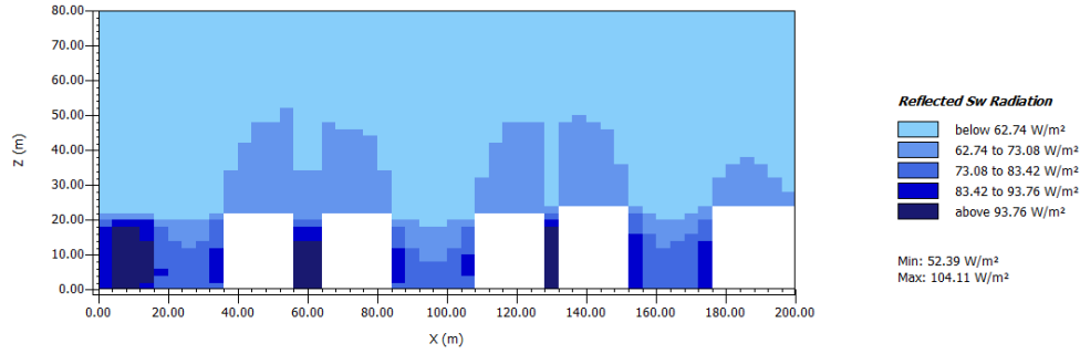
Figure 5.31. Reflected Shortwave Radiation ( \text{W/m}^2 ) in Demetevler Block at 21.07.2021, 15.00.00, Section BB', cut at y=86 meters
