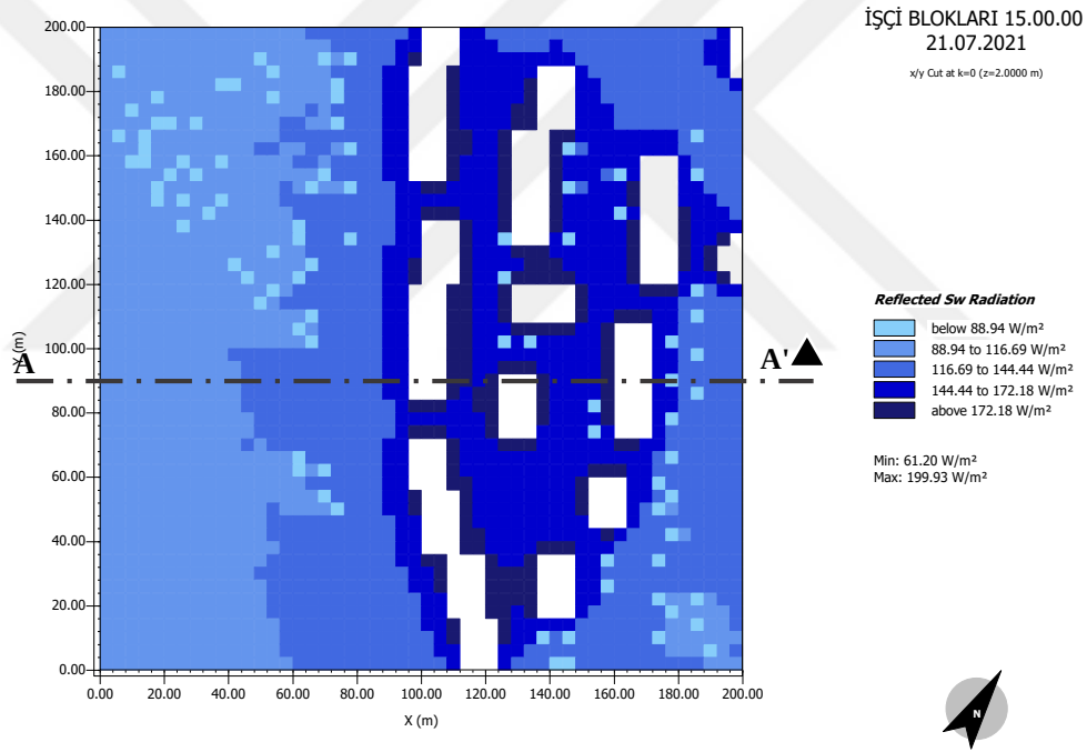
Figure 5.23. Reflected Shortwave Radiation ( \text{W/m}^2 ) in İşçi Blokları at 21.07.2021, 15.00.00, plan view, 2 meters above the ground
