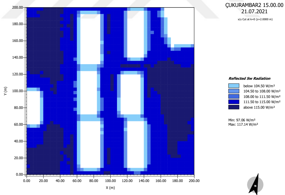
Figure D.51. Reflected Shortwave Radiation (W/m 2 ) of Urban Block 3 – Çukurambar 2
