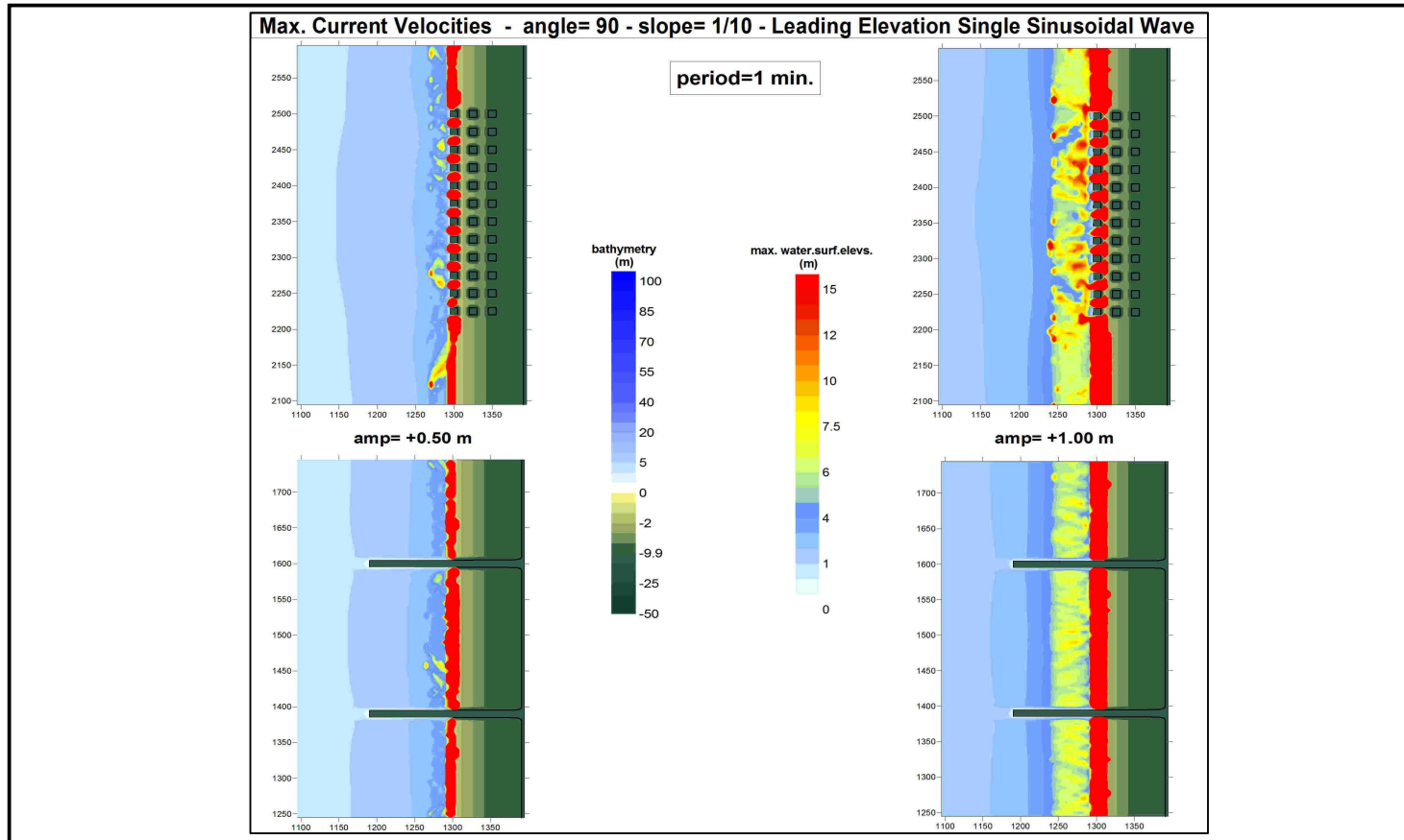
Figure 4.34: Distribution of Maximum Current Velocities for Perpendicular Approach of the Wave (angle=90°) with Period of 1 min. for LEW with the Bottom Slope of 1/10 (Incoming Wave Amplitudes= +0.5m, +1.0m at the toe)
