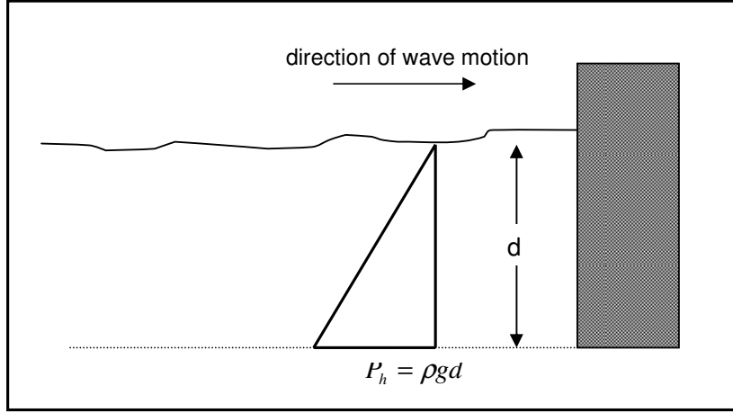
Figure 3.6: Sectional View of Hydrostatic Pressure on a Coastal Structure
