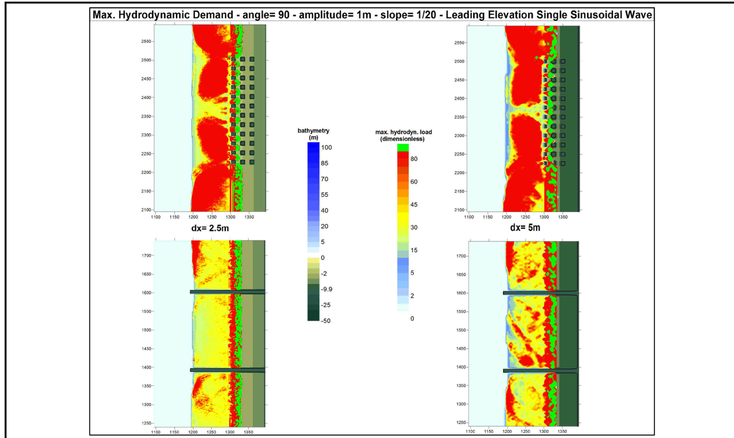
Figure 5.10: Comparison of Distribution of Maximum Hydrodynamic Demands for the Grid Sizes of 2.5m and 5m , with Perpendicular Approach of the Wave (angle= 90^\circ ), Period of 3min. and Bottom Slope of 1/20 for LEW (Incoming Wave Amplitude= +1.0m at the toe)
