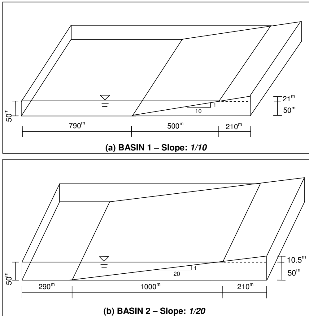
Figure 4.2: Three-Dimensional View of (a) Basin 1 with slope of 1/10 and (b) Basin 2 with slope of 1/20 .
