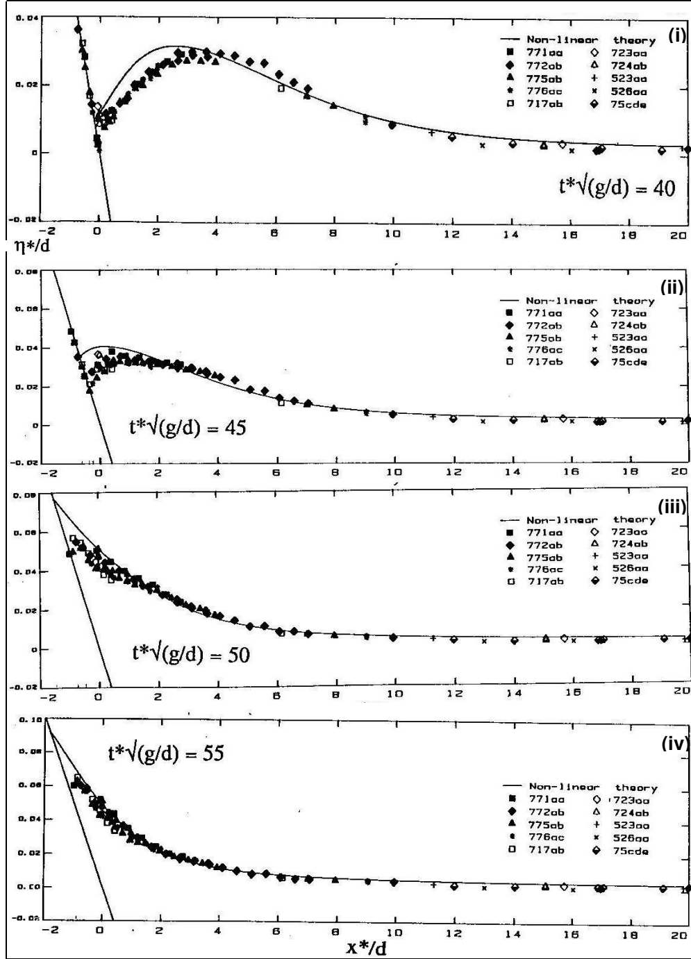
Figure 4.5 (a): Comparison between laboratory data and the nonlinear model for a 0.0185 solitary wave up on a 1/19.85 beach. Profiles are shown as functions of x at t = 40 (i), 45(ii), 50(iii) and 55 (iv). Different symbols indicate different realizations of the same experiment (Synolakis, 1987).
