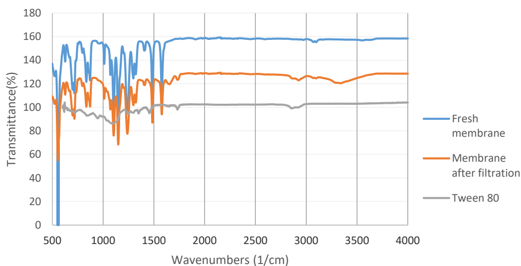
Figure 4.7 FTIR analysis on fresh membrane, membrane after 0,1 g/l Tween 80 solution and Tween 80 droplet.
