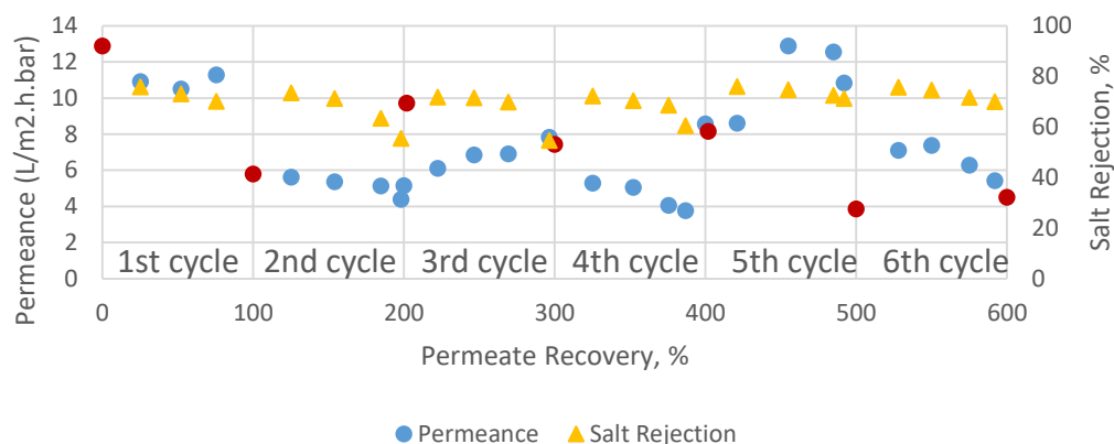
Figure 4.24 6 Sequential filtrations of stream 2 \text{NaHCO}_3 -EG solutions on DESAL DL membrane in concentration mode for 6 cycles
