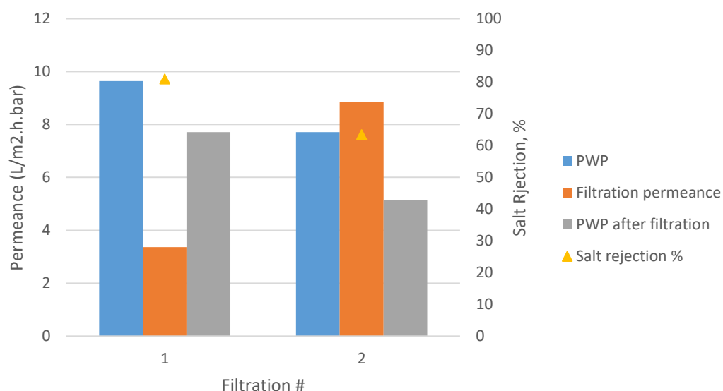
Figure 4.21 Filtration of 0,15% \text{NaHCO}_3 and 26% EG (filtration # 1) and 2,2% \text{NaHCO}_3 and 2,5% EG (filtration # 2) solutions on DESAL DL membrane in total recycle mode
