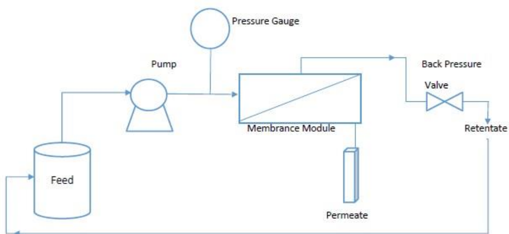
Figure 3.1 Schematic of the cross-flow system
