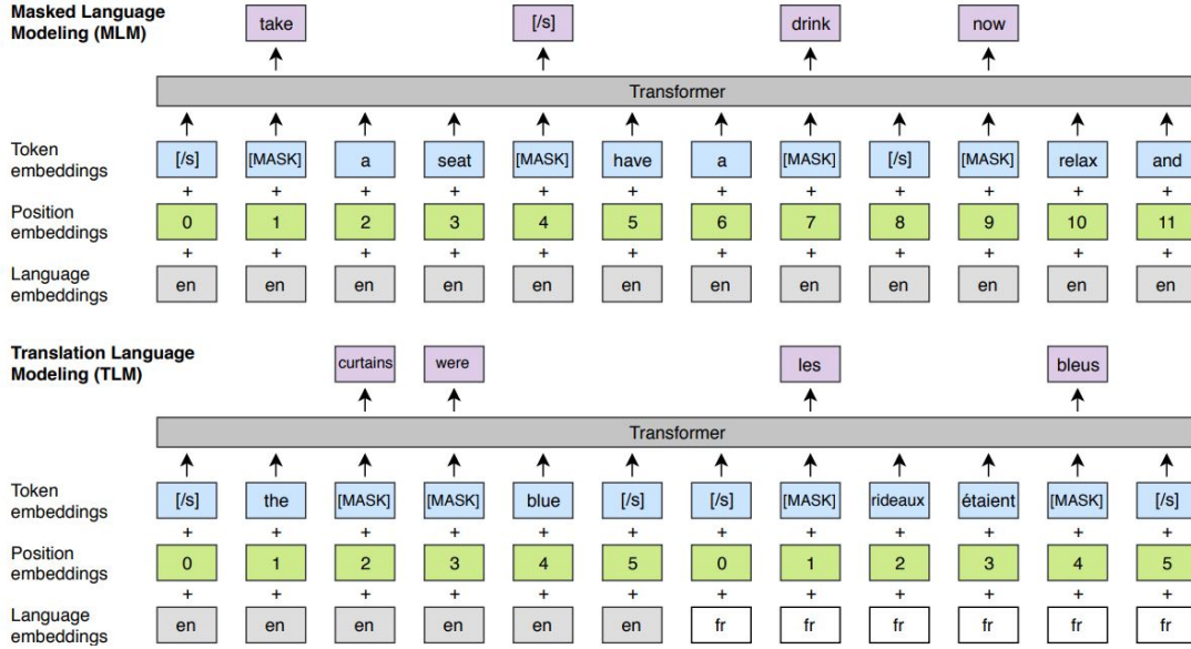
Figure 3.4: Cross-lingual language model pre-training [4]
