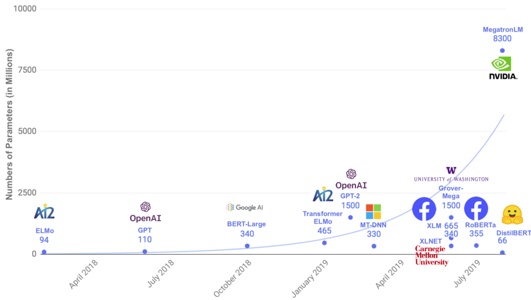
Figure 3.3: Parameter counts of several pre-trained language models [3]
