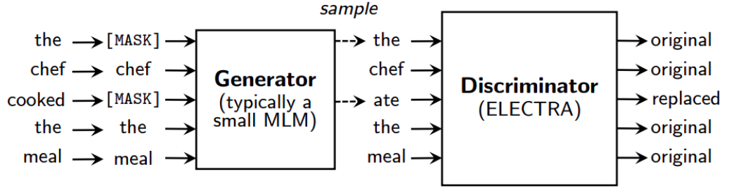
Figure 3.5: ELECTRA model Replaced Token Detection Mechanism Illustration [5]
