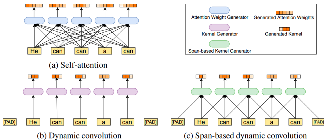
Figure 3.6: Self attention, dynamic convolution and span-based dynamic convolution [6]
