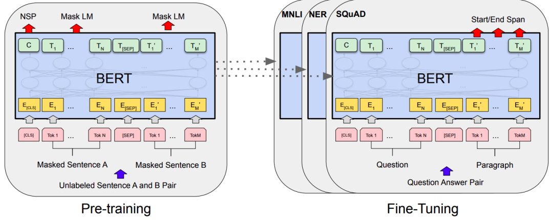
Figure 3.2: BERT Pre-training and Fine-tuning [2]
