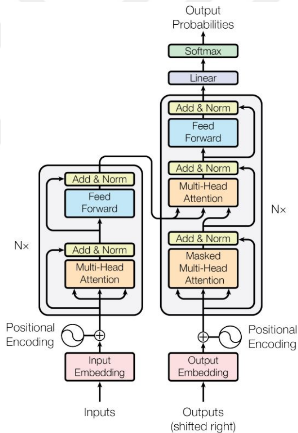
Figure 3.1: Transformer model architecture [1]
