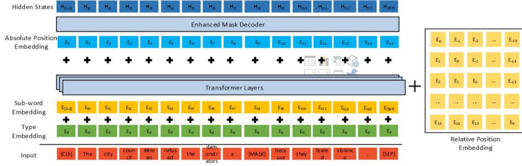
Figure 3.7: DeBERTa Architecture [7]
