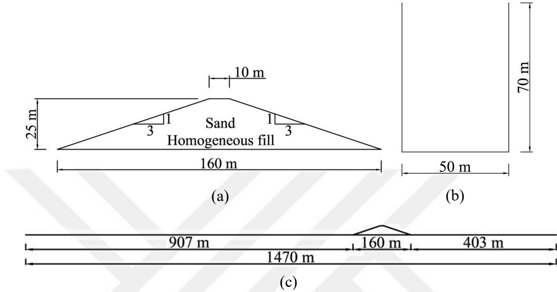
Figure 3.2. Views of the deterministic model a) dam cross-section b) channel cross-section c) channel longitudinal view
