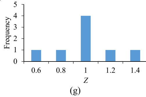
Figure 3.4. Frequency histograms of dam breach parameters for final breach bottom elevation of a) uniform PDF and b) triangular PDF; left column shows histogram of parameters based on E_b = uniform PDF and right column shows histogram of parameters based on E_b = triangular PDF: c-d) t_f , e-f) W_b , g) Z
