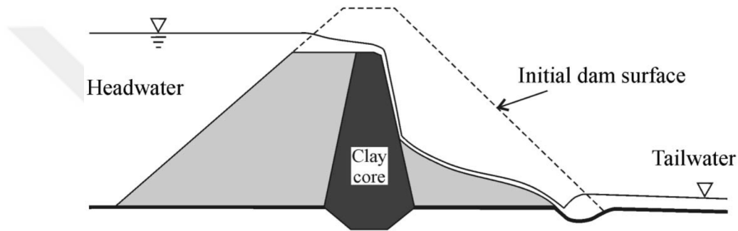
Figure 1.3. Breaching mechanism for composite dam (After Wu et al., 2011)
