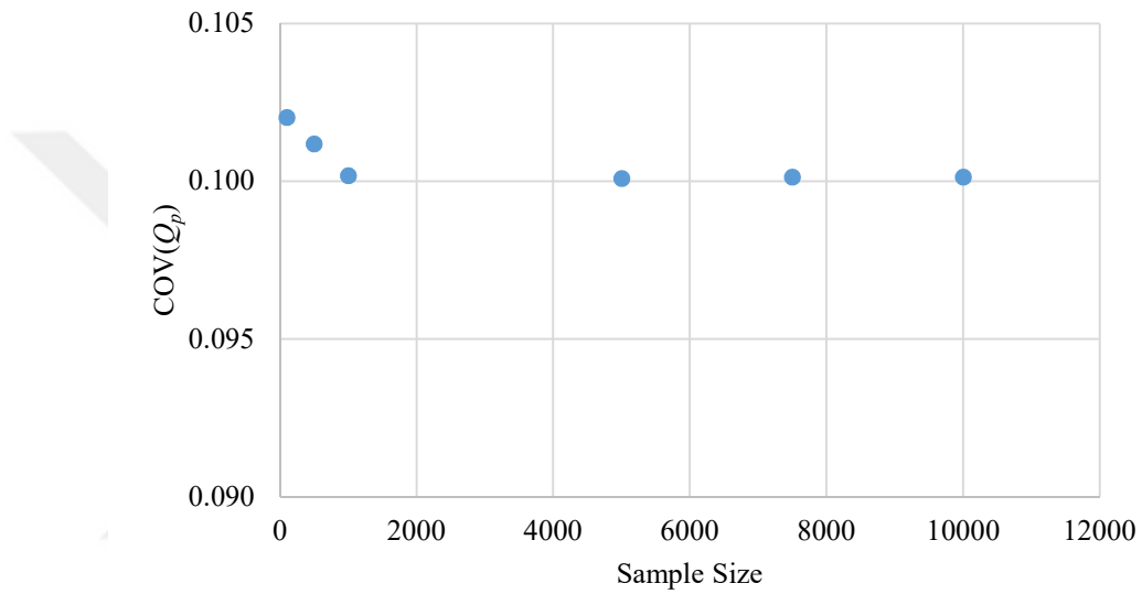
Figure 3.5. Sample size vs COV(Q_p) graph
