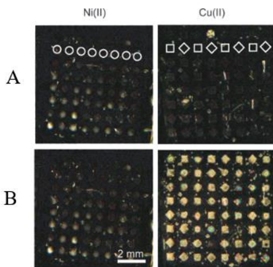
Figure 2.1 Optical images of 5CB on nickel(II) or copper(II) perchlorate salt-treated surface (A) before, (B) after the exposure of 10 ppm DMMP in nitrogen 43 .
