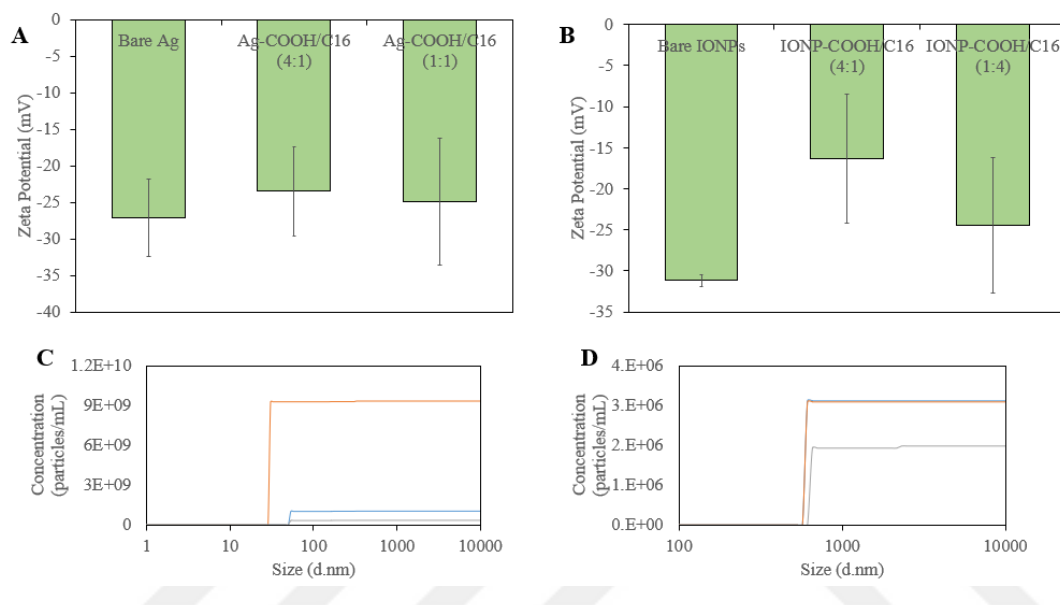
Figure 4.10 Characterizations of mixed monolayer of 11-mercaptoundecanoic acid (-COOH) and 1-hexadecanethiol (-C16) terminated thiols groups (-COOH/C16 monolayer) functionalized silver and IONPs. (A) zeta potential measurements of bare, -COOH/C16 mixed monolayer terminated silver nanoparticles for ratios of -COOH:C16 is 4:1 or 1:1, (B) zeta potential measurements of bare, -COOH/C16 mixed monolayer terminated IONPs for ratios of -COOH:C16 is 4:1 or 1:4, (C-E) particle concentration measurements of -COOH/C16 mixed monolayer terminated silver and IONPs.
