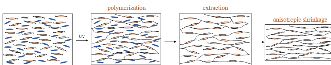
Figure 1.5 Schematic illustration of the polymerization of reactive mesogen (orange) and non-reactive mesogen (blue) mixture.
