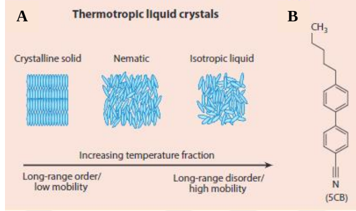
Figure 1.1 (A) Schematic illustration of the temperature-dependent phase behavior of thermotropic LCs, (B) the molecular structure of the 5CB, nematogenic LC 15 .
