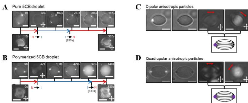
Figure 2.8 (A) Particles on the surfaces of the pure (5CB) droplets diffused toward one another after heating (isotropic phase), whereas (B) particles positioned were preserved for polymerized droplets. Typical (C) dipolar and (D) quadrupolar anisotropic particles 13 .
