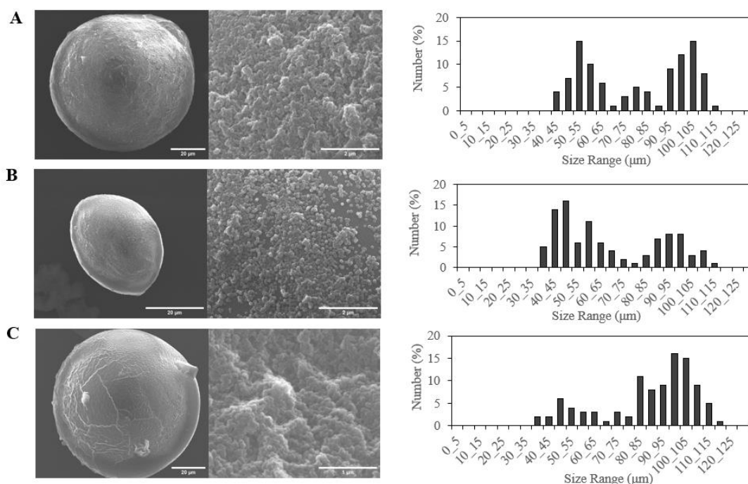
Figure 4.32 SEM micrographs of polymerized LC droplets and size distribution analysis of nanoparticles. Before polymerization LC droplets were exposed to the -NH 2 terminated 87.5 nm \pm 7.2 nm-average-sized-silica nanoparticles and -COOH terminated 51.2 nm \pm 9.0 nm-average-sized-silica nanoparticles with the concentrations of (A) 1.0 \times 10 9 particles/mL for both nanoparticles, (B) 1.0 \times 10 8 particles/mL and 1.0 \times 10 9 particles/mL, (C) 1.0 \times 10 9 particles/mL and 1.0 \times 10 8 particles/mL, respectively.
