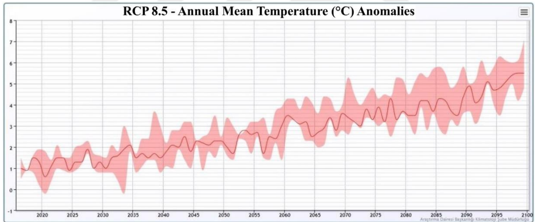
Figure A.16. RCP 8.5 - Temperature Anomaly Change Projection (MGM, 2015)
