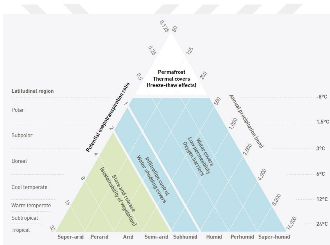
Figure 2.1. Cover system design according to climate types (ICMM, 2019)
