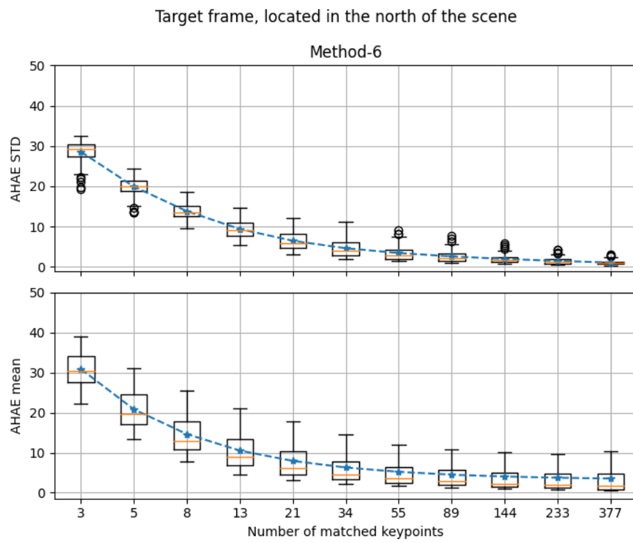
Figure 3.30: Method-6 AHAЕ Mean and Standard Deviations Box Plot
