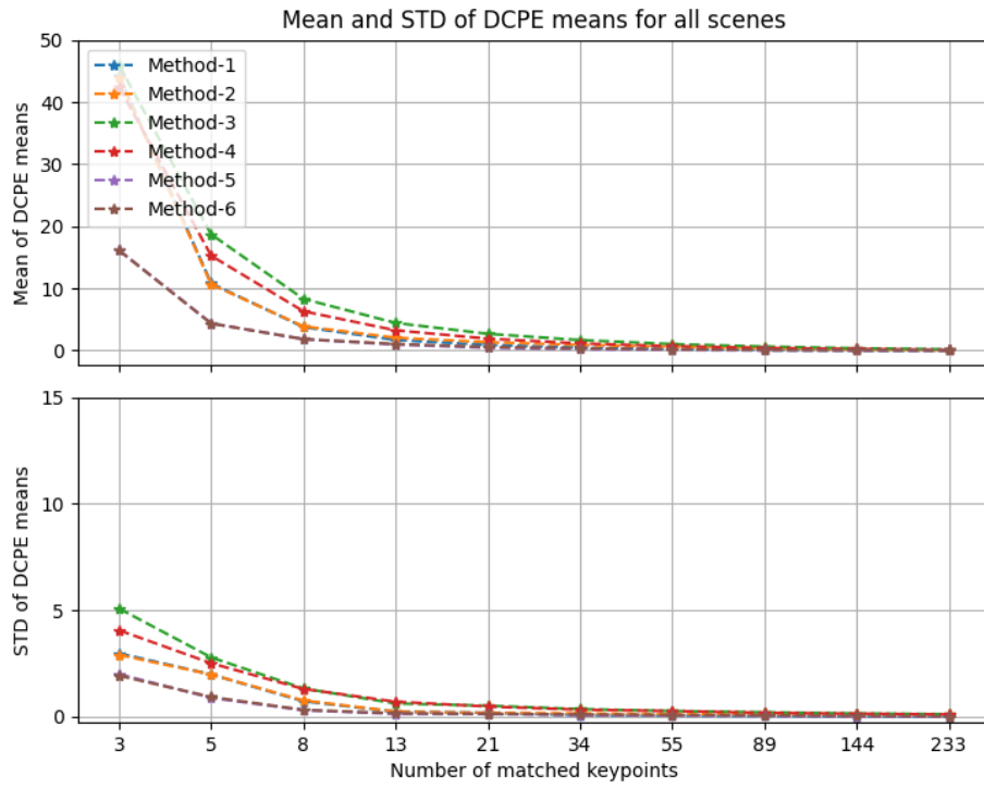
Figure 3.49: Mean and Standard Deviation of DCPE Means Comparison
