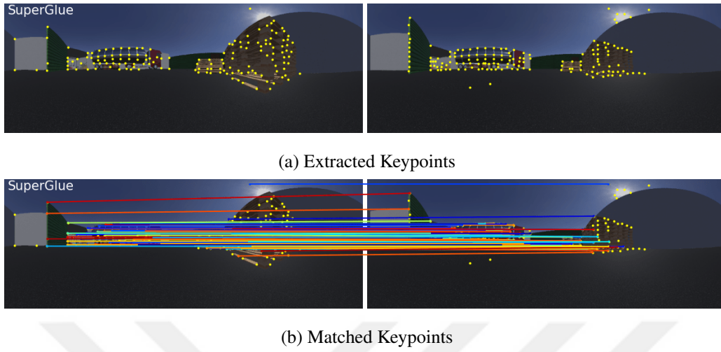
Figure 6.43: False Movement End and Node-49 Local Feature Matching Results
