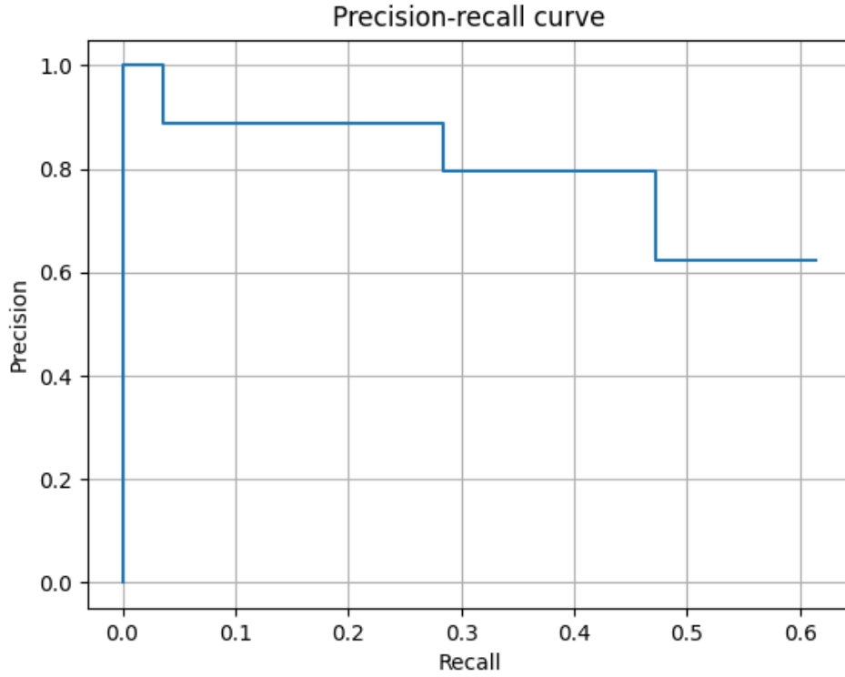
Figure 3.11: Sample Precision-recall curve
