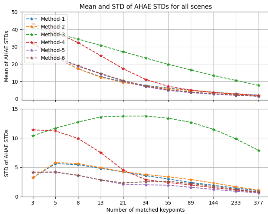
Figure 3.39: Mean and Standard Deviation of AHAE Standard Deviations Comparison
