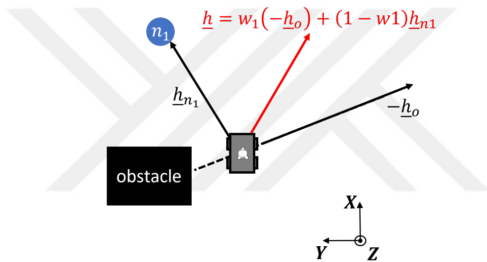
Figure 4.9: Obstacle Avoidance Strategy
