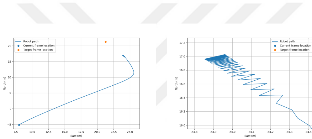
Figure 3.68: Path Change For Sample Failure Case of Method-1
