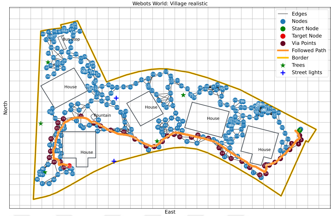
Figure 6.19: Village Realistic Followed Path for the First Round
