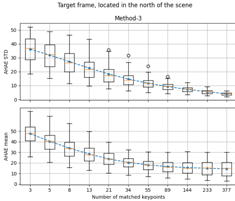
Figure 3.27: Method-3 AHAЕ Mean and Standard Deviations Box Plot
