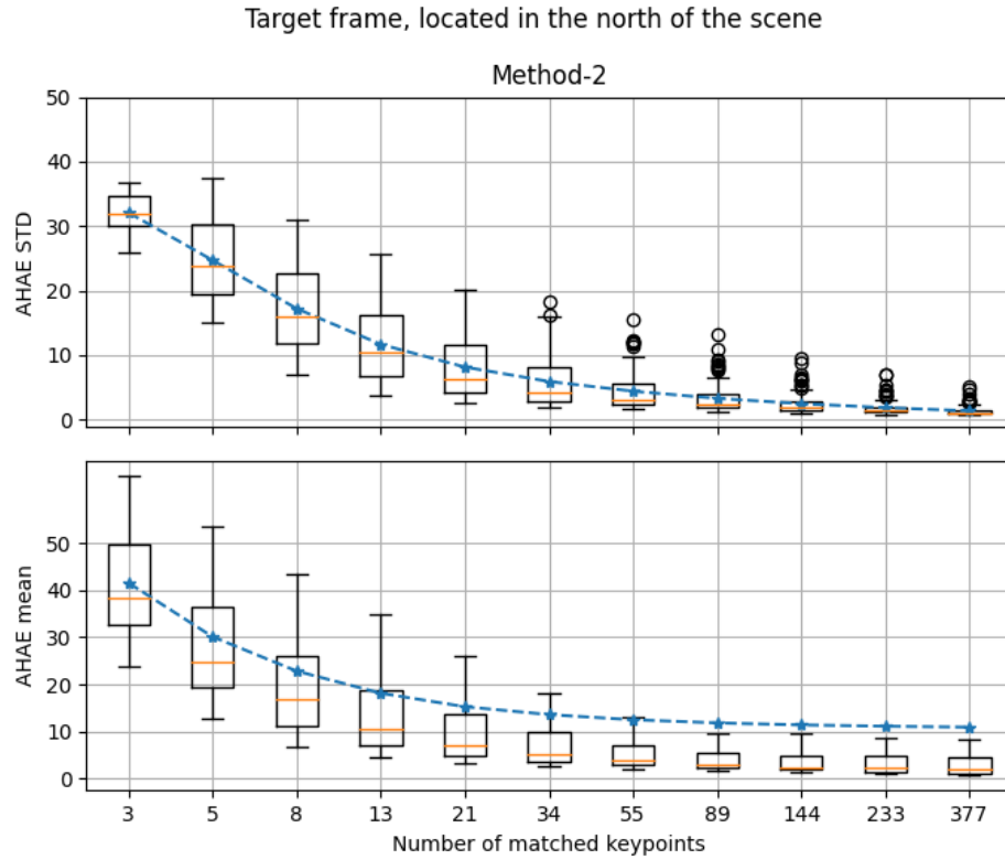
Figure 3.26: Method-2 AHAЕ Mean and Standard Deviations Box Plot
