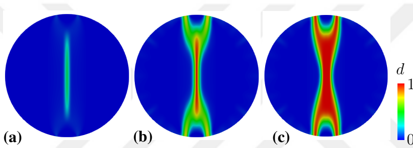
Figure 2.31: Prediction of crack pattern in concrete specimen under Brazilian tensile test at (a) u = 0.102 mm, (b) u = 0.212 mm and (c) u = 0.24 mm.
