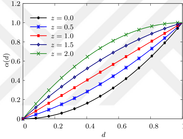
Figure 2.2: The geometric crack function \alpha(d) versus the crack phase-field for different values of the parameter z .
