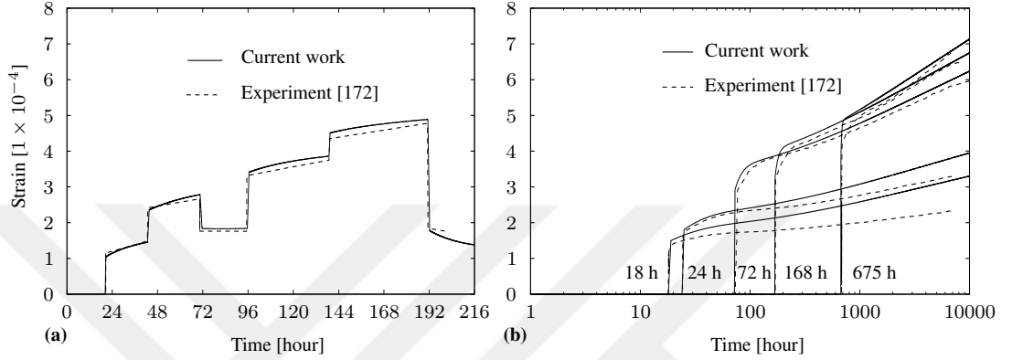
Figure 4.6: Basic creep tests: (a) cyclic test on the cylindrical concrete specimen, and (b) monotonic test on the cylindrical concrete specimen
