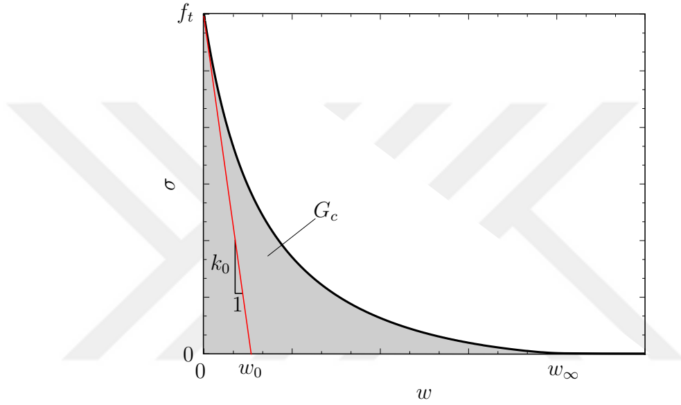
Figure 2.6: A generic traction-separation \sigma - w curve with the critical fracture energy release rate G_c , and the initial slope of k_0 = -\frac{f_t}{w_0} .
