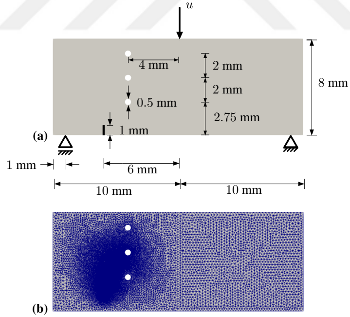
Figure 2.18: Asymmetric notched three-point bending beam. (a) geometry, dimensions, loading and boundary conditions, and (a) finite element mesh with the effective element size h = 0.01 mm in the damage critical zone.
