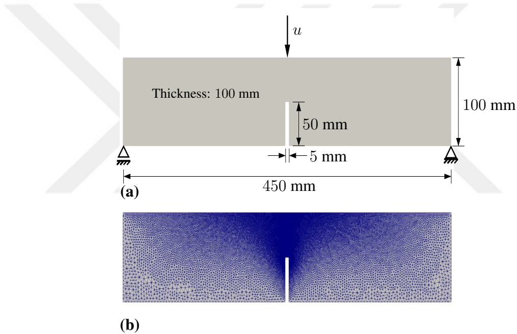
Figure 2.24: Three-point bending test. (a) Geometry, loading and boundary conditions of a notched concrete beam (b) Finite element discretization with the effective element size h = 0.25 mm.
