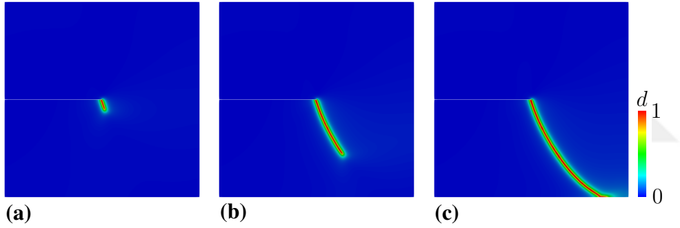
Figure 2.16: Single edge notched pure shear test. Crack propagation path for \eta = 0 kNs/mm 2 at a displacement of (a) u = 6.02 \times 10^{-3} mm, (b) u = 6.52 \times 10^{-3} mm, and (c) u = 7.04 \times 10^{-3} mm.
