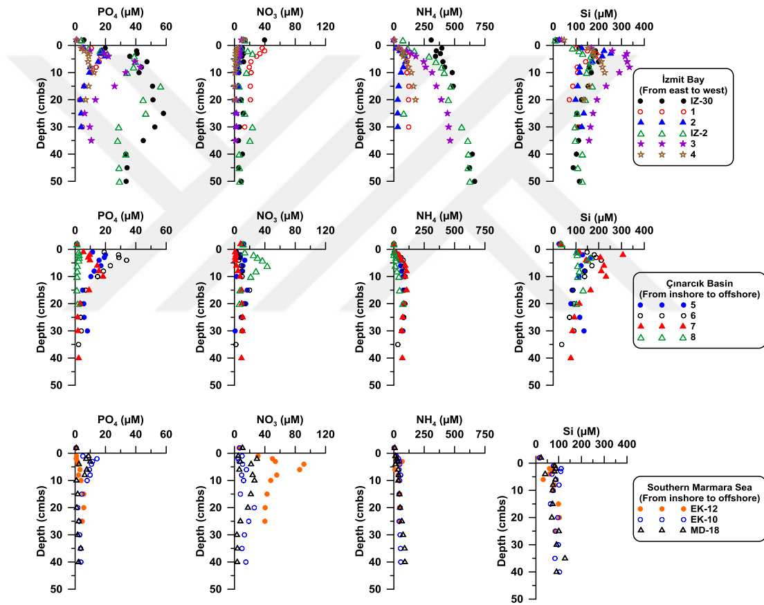
Figure 3.6. Porewater nutrient concentrations in the sediment cores from the Marmara Sea.
