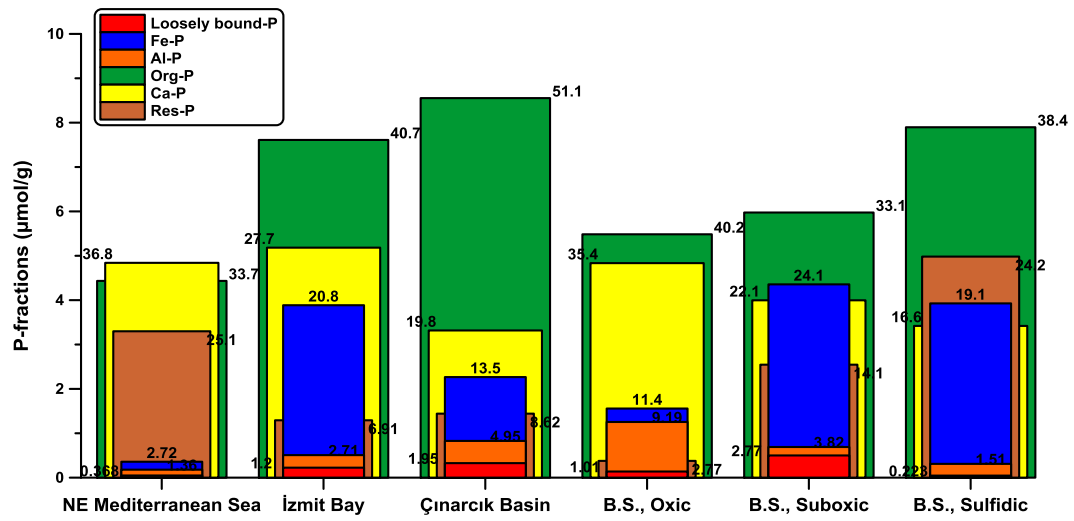
Figure 4.6. Concentration of P-fractions and their contribution to the TP pool (%) in surface (0-2 cm) sediments of the NE Mediterranean, Marmara and Black Seas.
