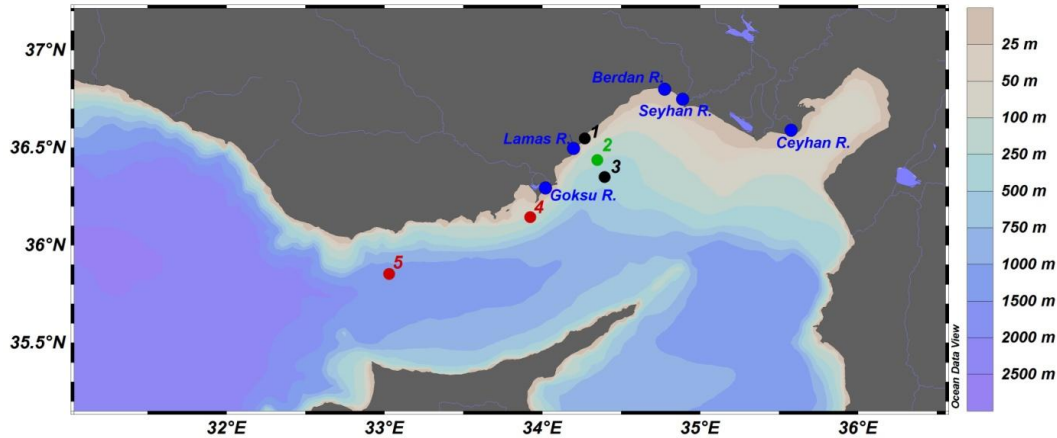
Figure 2.2. Locations of sediment core and river stations (black dots represent March 2018, red dots represent April 2018, one green dot represents both March and April 2018 and blue dots represent river stations).
