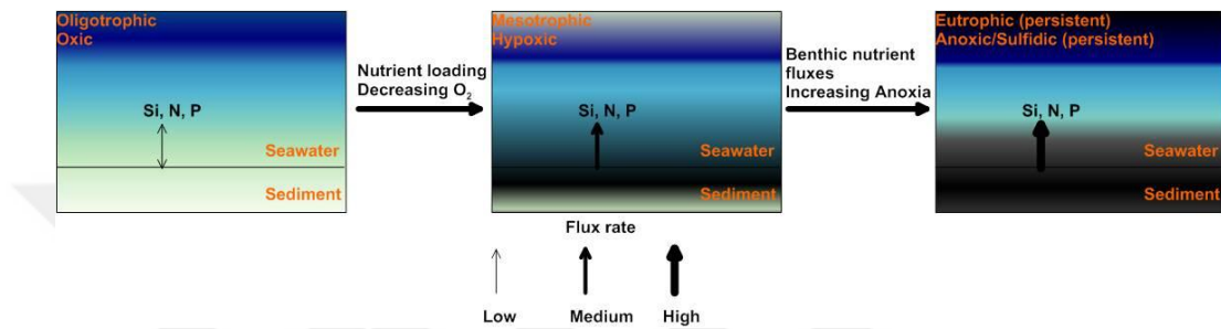
Figure 5.4. Changes in porewater diffusive nutrient fluxes during exposure to eutrophication and deoxygenation.
