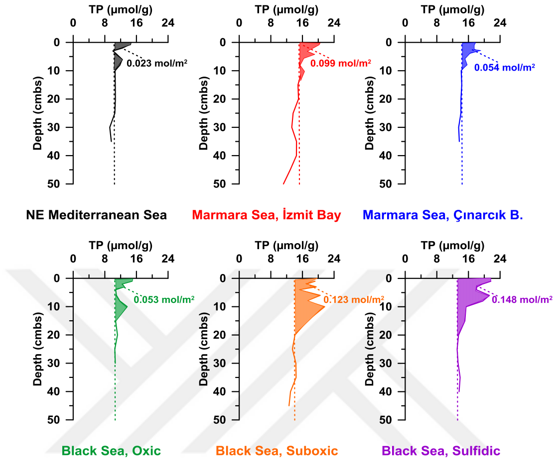
Figure 4.7. Amount of mobile phosphorus in the NE Mediterranean, Marmara and Black Seas. Dashed lines indicated the burial concentration of sedimentary P.
