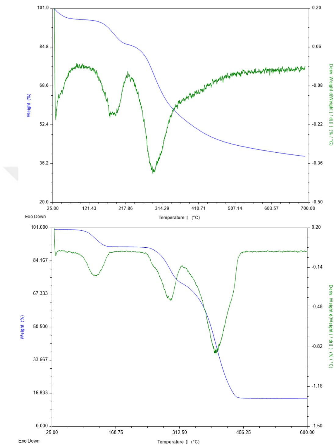
Figure 3.42 TGA curves of neat SF (top) and neat PMMA (bottom) electrospun meshes.
