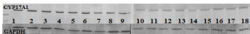
Figure 3.7 Immunoreactive protein bands of LNCaP cells representing the expression of CYP17A1 (57 kDa) and GAPDH (37 kDa).
