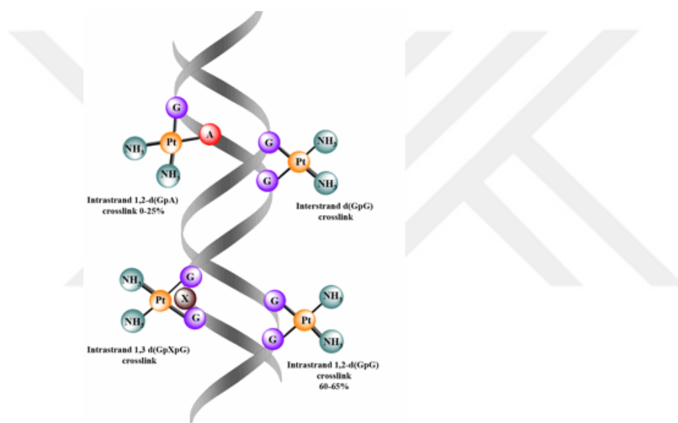
Figure 1.2. Cisplatin-DNA adducts (Boulikas T., et. al., 2007).
