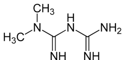
Figure 1.3. Chemical Formula of Metformin.
