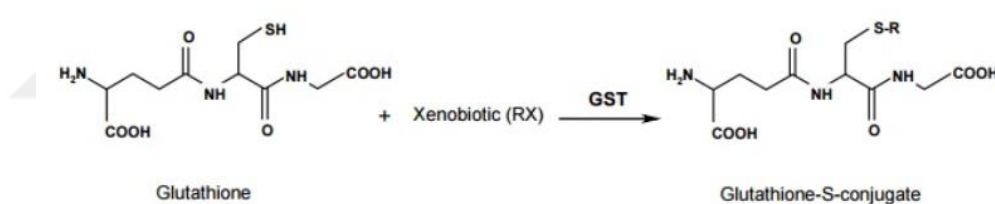
Figure 1.7 Glutathione conjugation to a xenobiotic by GSTs.
