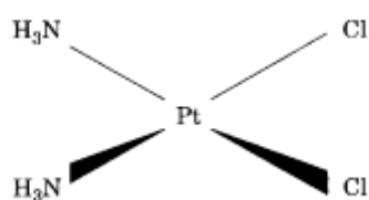
Figure 1.1. Structure of cisplatin (The chemical book database, 2014).
