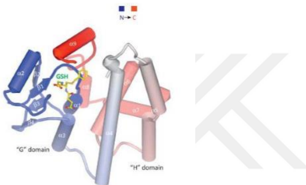
Figure 1.8 3-D structure of GST enzyme (Wu and Dong, 2012).
