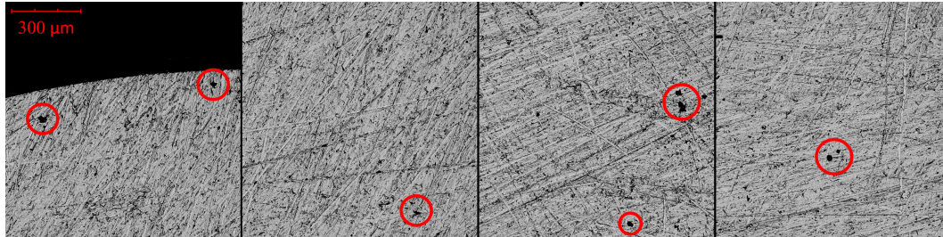
Figure 3.17: Some SEM images of the cylinder test parts, red circles indicate example larger pore areas.
