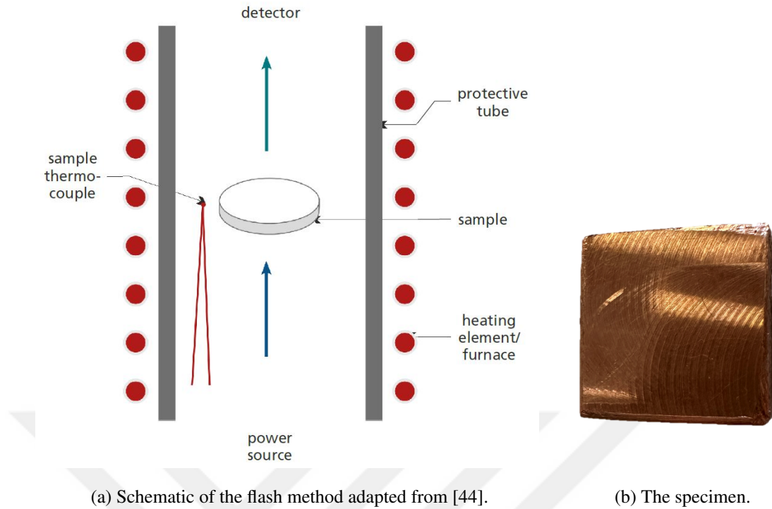
Figure 3.19: Thermal conductivity measurements.
