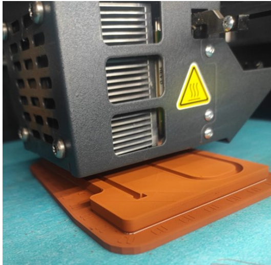
(a) Printing process of a cold plate on the Metal X 3D printer.
