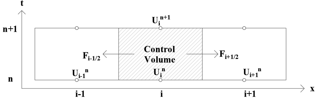
Figure 4.1: Discretization of i^{\text{th}} cell
