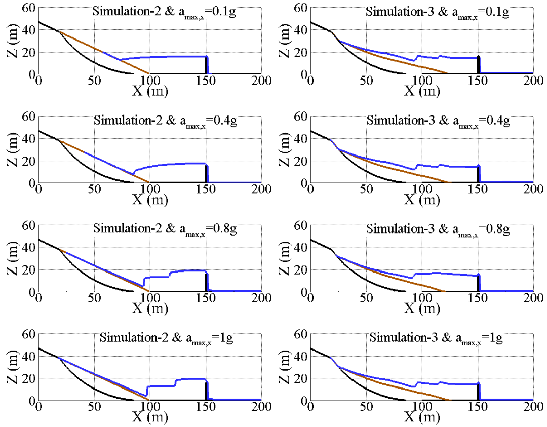
Figure 5.42: For Case-E4, screenshots of Simulation-2 and -3 at Time = 20.0 Seconds
