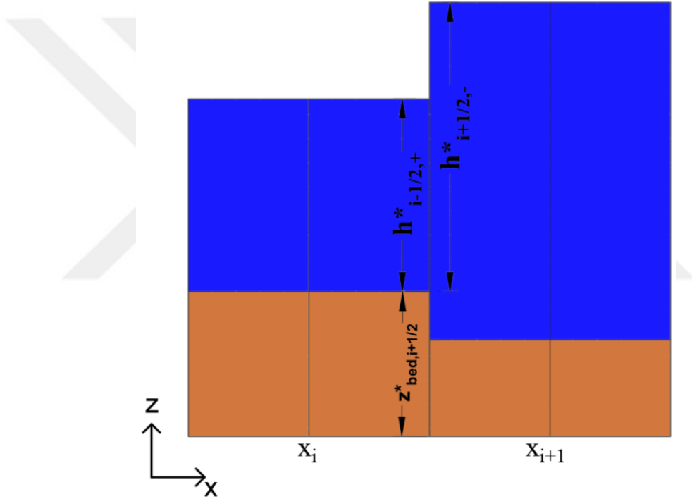
Figure 4.2: Hydrostatic Reconstructed Variables
