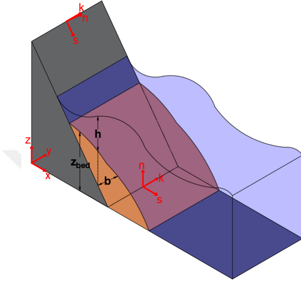
Figure 3.1. Coordinates and geometric description of landslide parameters
