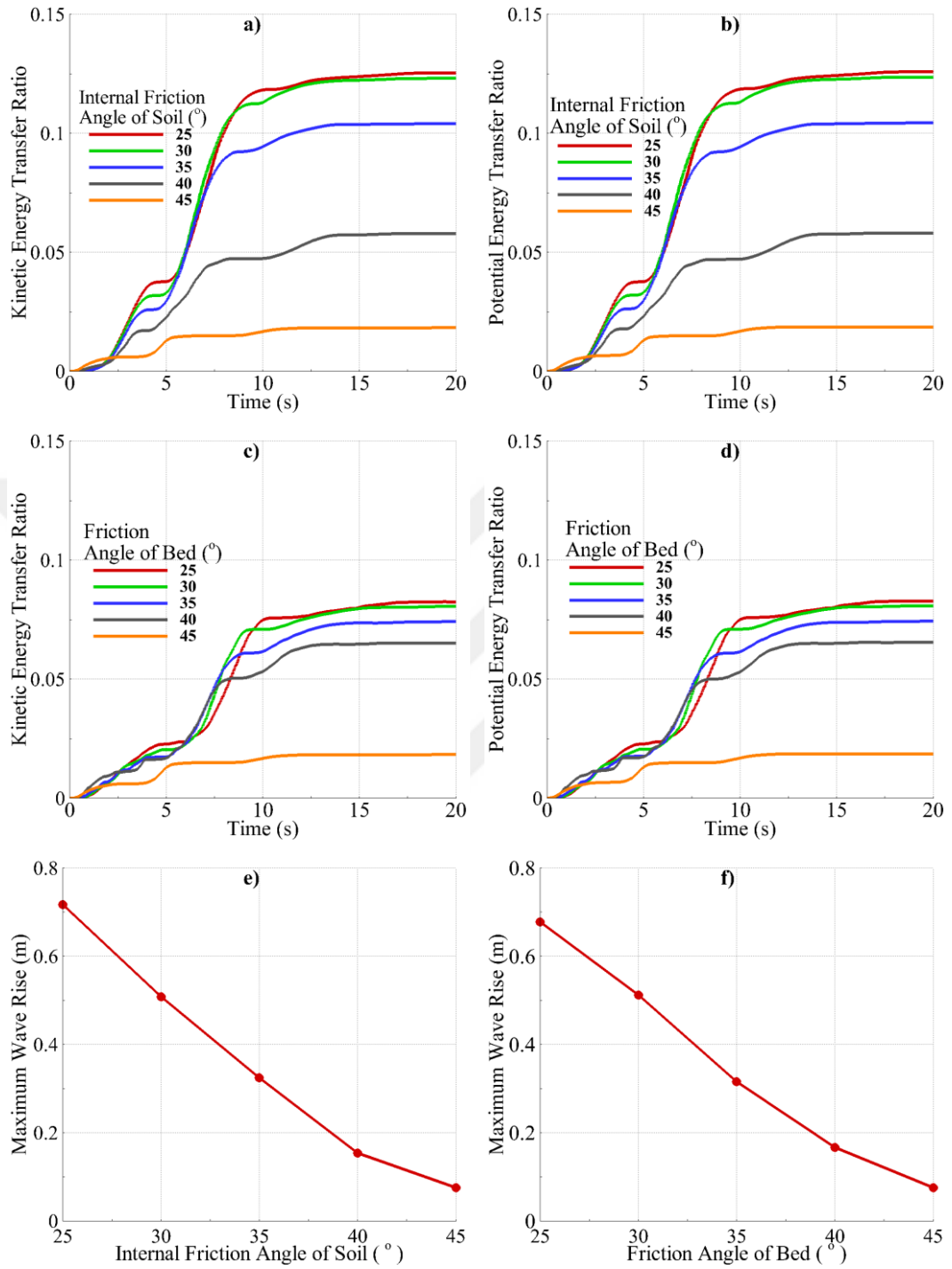
Figure 5.32: a) KETR vs. Time for Case-D16, b) PETR vs. Time for Case-D16, c) KETR vs. Time for Case-D17, d) PETR vs. Time for Case-D17, e) Maximum Wave Rise vs. Internal Friction Angle of Soil for Case-D16 and f) Maximum Wave Rise vs. Friction Angle of Bed for Case-D17
