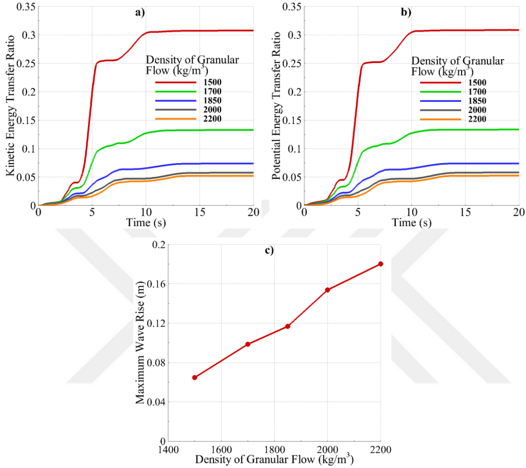
Figure 5.34: For Case-D19; a) KETR vs. Time, b) PETR vs. Time and c) Maximum Wave Rise vs. Density of Granular Flow
