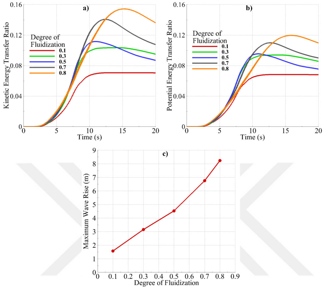
Figure 5.15: For Case-C7; a) KETR vs. Time, b) PETR vs. Time and c) Maximum Wave Rise vs. Degree of Fluidization
