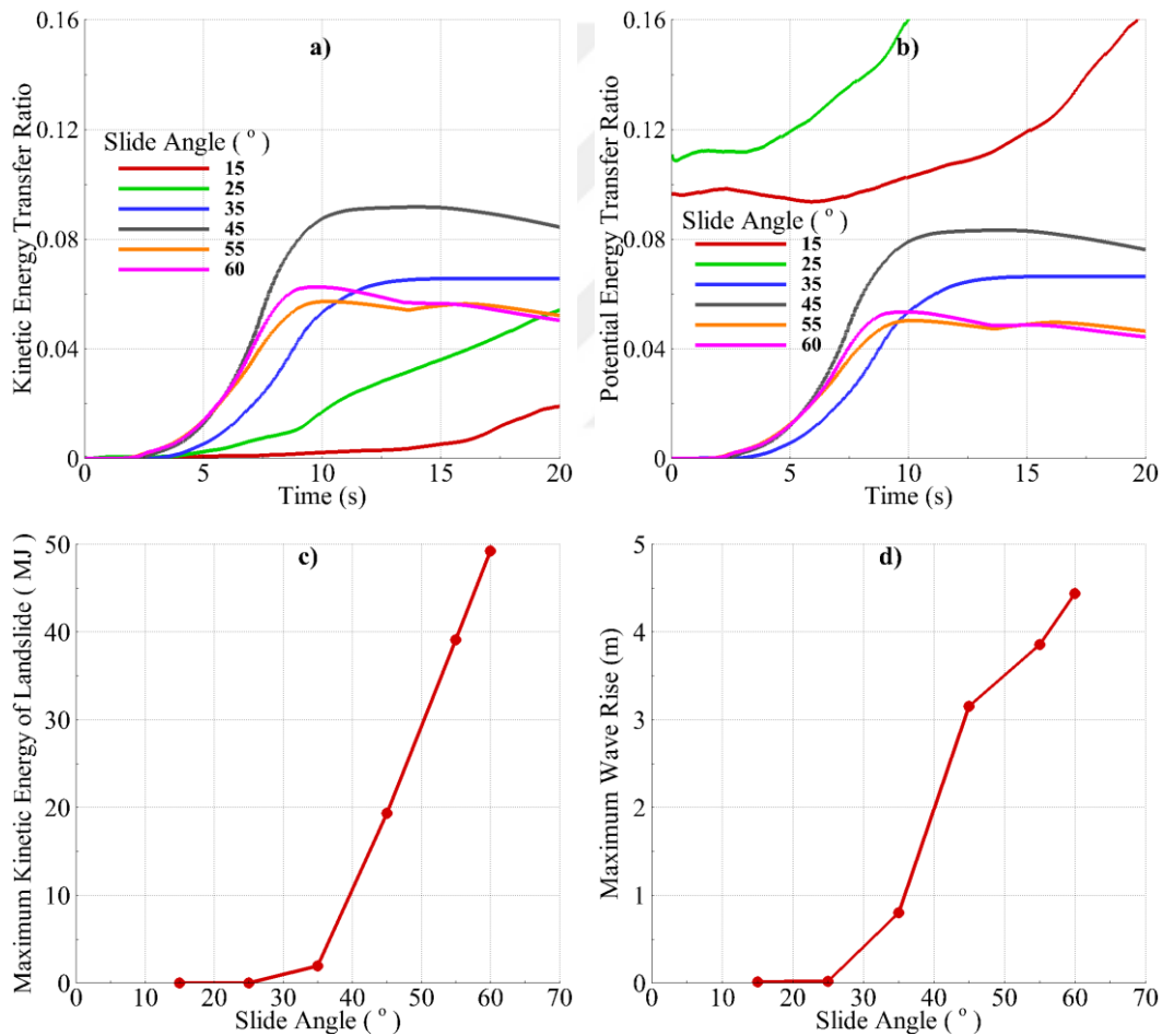
Figure 5.12: For Case-C3; a) KETR vs. Time, b) PETR vs. Time, c) Maximum Kinetic Energy of Landslide vs. Slide Angle and d) Maximum Wave Rise vs. Slide Angle
