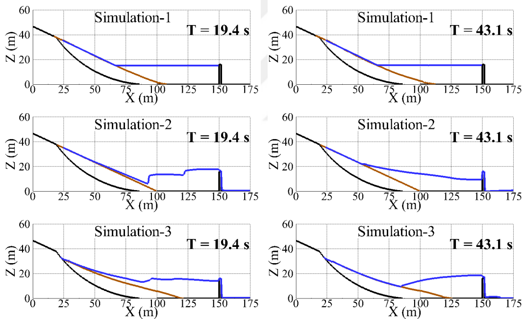
Figure 5.38: Screenshots of simulations-1, -2 and -3
