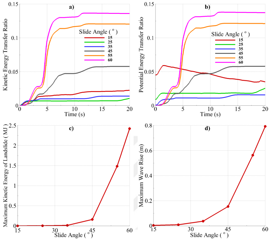
Figure 5.30: For Case-D14; a) KETR vs. Time, b) PETR vs. Time, c) Maximum Kinetic Energy of the Landslide vs. Slide Angle and d) Maximum Wave Rise vs. Slide Angle
