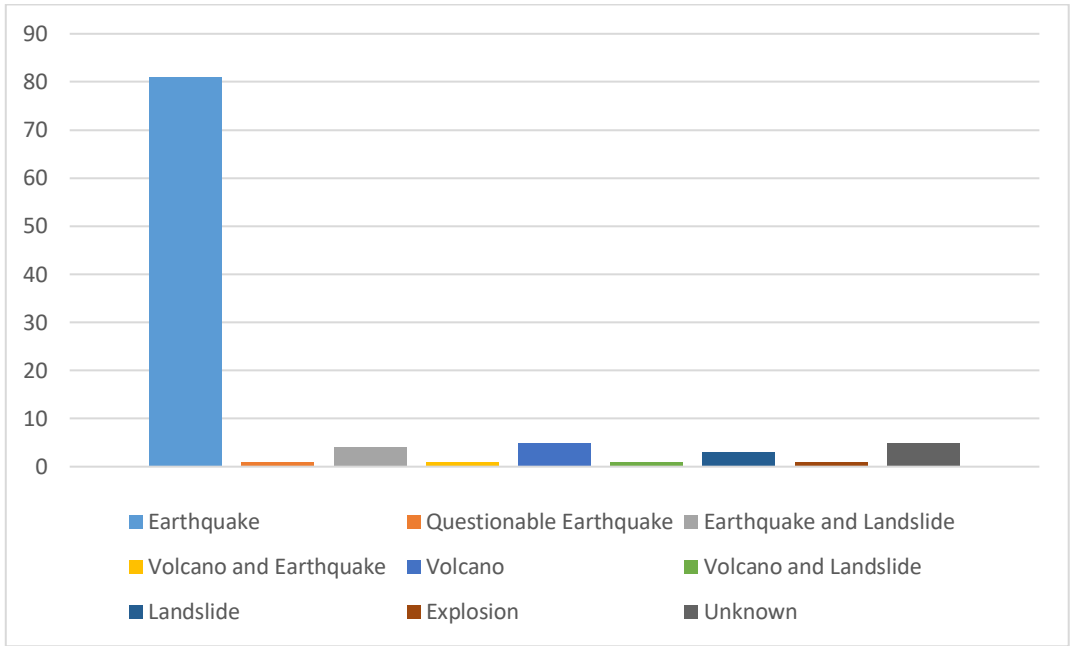
Figure 1.1. Relative Occurrence of Various Historical Tsunami Sources Based on the NOAA/NGDC tsunami database (NGDC 2013)
