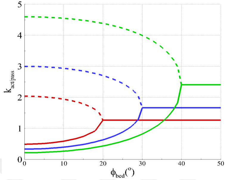
Figure 3.2. Motion states of the Granular Flow
