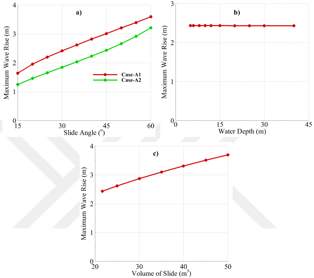
Figure 5.3: a) Maximum Wave Rise vs. Slide Angle for Cases-A1 & A2; b) Maximum Wave Rise vs. Water Depth for Case-A3 and c) Maximum Wave Rise vs. Volume of Slide for Case-A4
