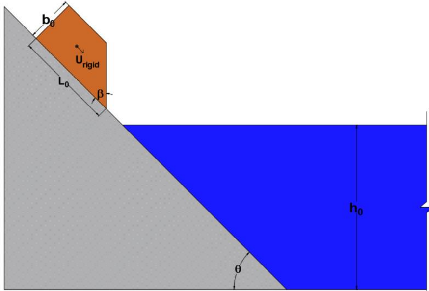
Figure 5.4: Assumed Test Geometry for the Rigid Block Model
