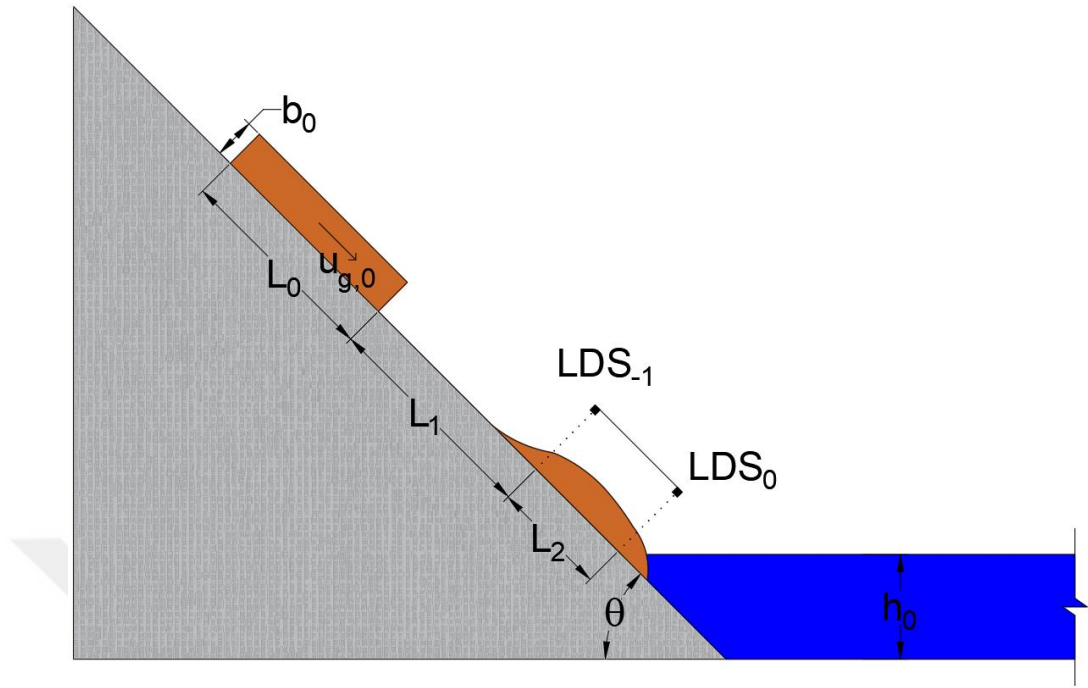
Figure 4.3: Experimental Geometry Conducted in Heller & Hager, 2010
