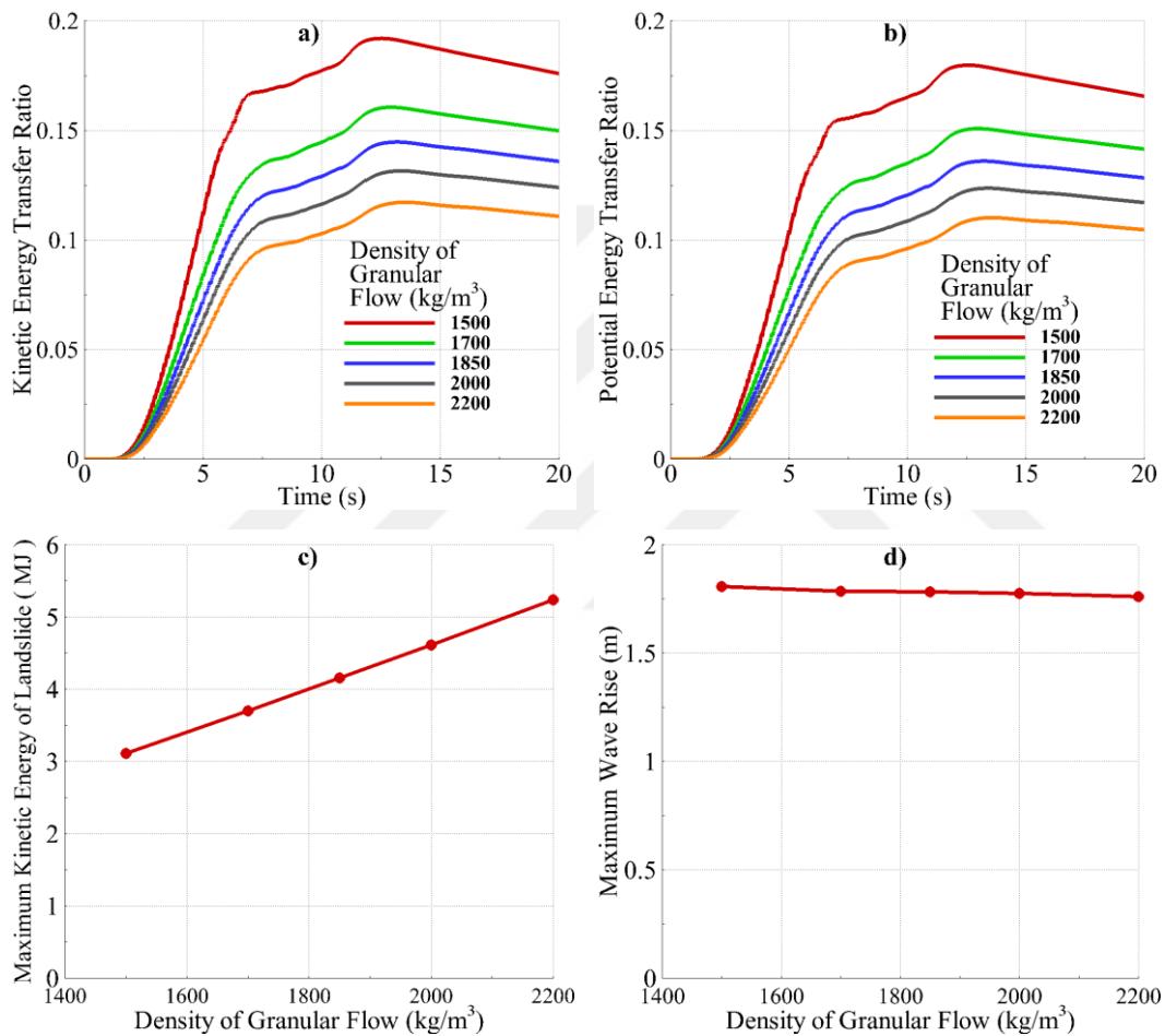
Figure 5.26: For Case-D9; a) KETR vs. Time, b) PETR vs. Time, c) Maximum Kinetic Energy of the Landslide vs. Density of Granular Flow and d) Maximum Wave Rise vs. Density of Granular Flow
