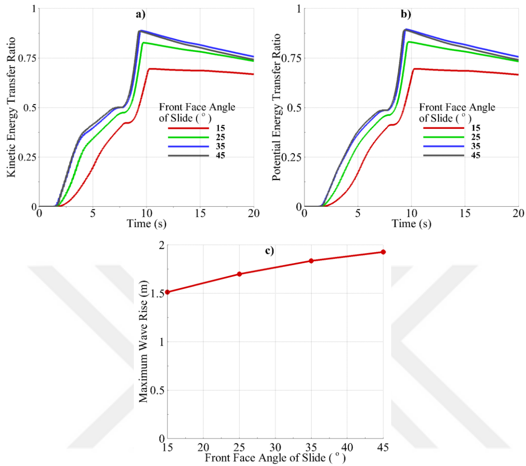
Figure 5.6: For Case-B3; a) KETR vs. Time, b) PETR vs. Time, c) Maximum Wave Rise vs. Front Face Angle of Slide
