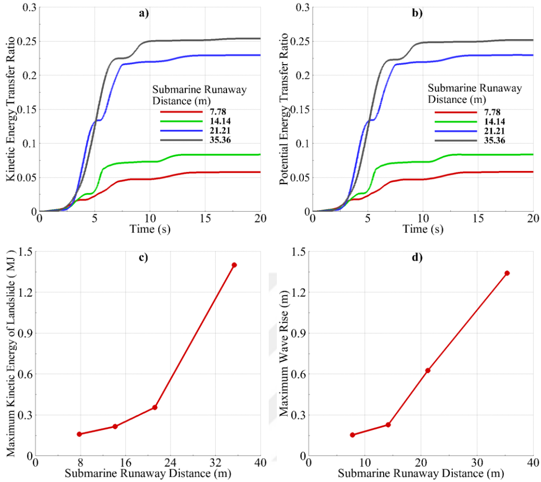
Figure 5.29: For Case-D13; a) KETR vs. Time, b) PETR vs. Time, c) Maximum Kinetic Energy of the Landslide vs. Submarine Runaway Distance and d) Maximum Wave Rise vs. Submarine Runaway Distance
