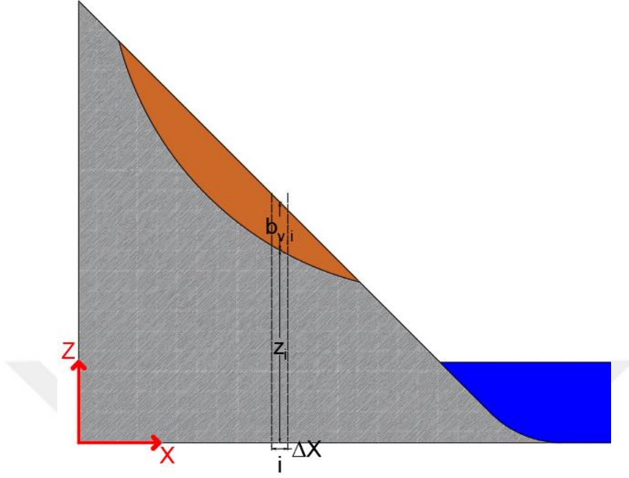
Figure 3.3. Initial position of the landslide-generated waves
