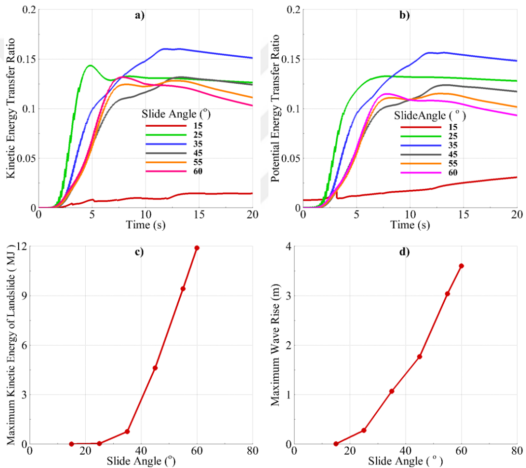
Figure 5.22: For Case-D4; a) KETR vs. Time, b) PETR vs. Time, c) Maximum Kinetic Energy of the Landslide vs. Slide Angle and d) Maximum Wave Rise vs. Slide Angle
