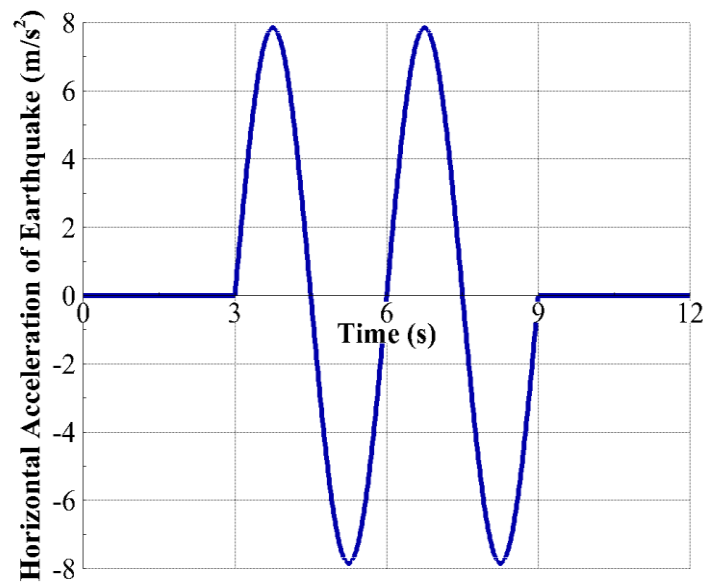
Figure 5.37: Description of Sinusoidal Earthquake Acceleration
