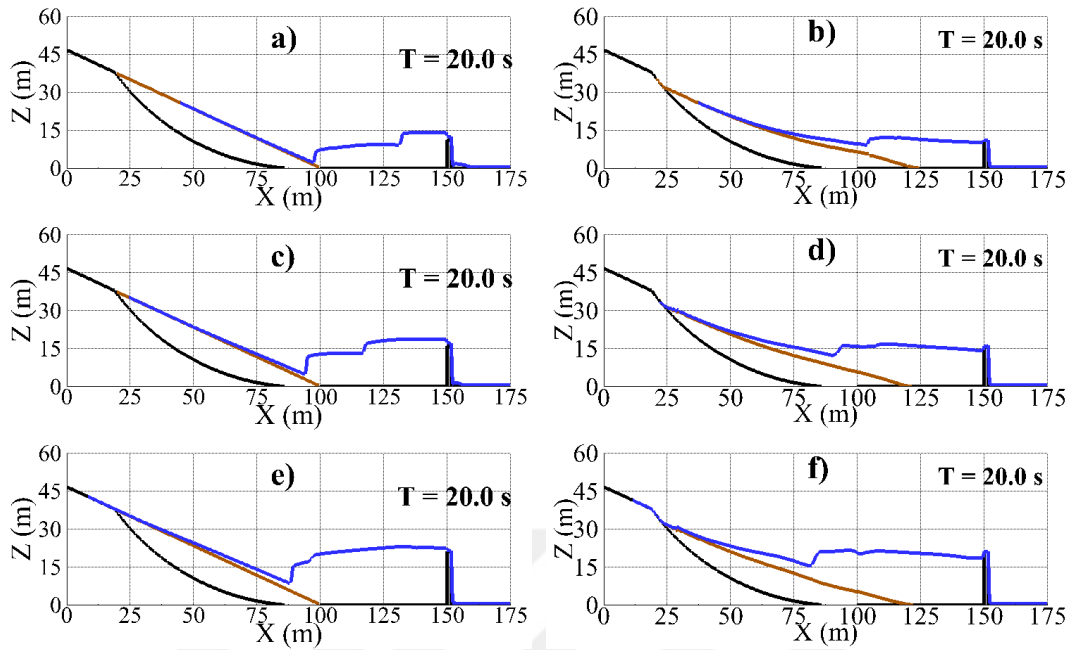
Figure 5.40: Screenshots of Simulation-2 when Initial Water Depth is; a) 10 meters; c) 15 meters and e) 20 meters and of Simulation-3 when Initial Water Depth is; b) 10 meters; d) 15 meters and f) 20 meters at Time = 20.0 Seconds
