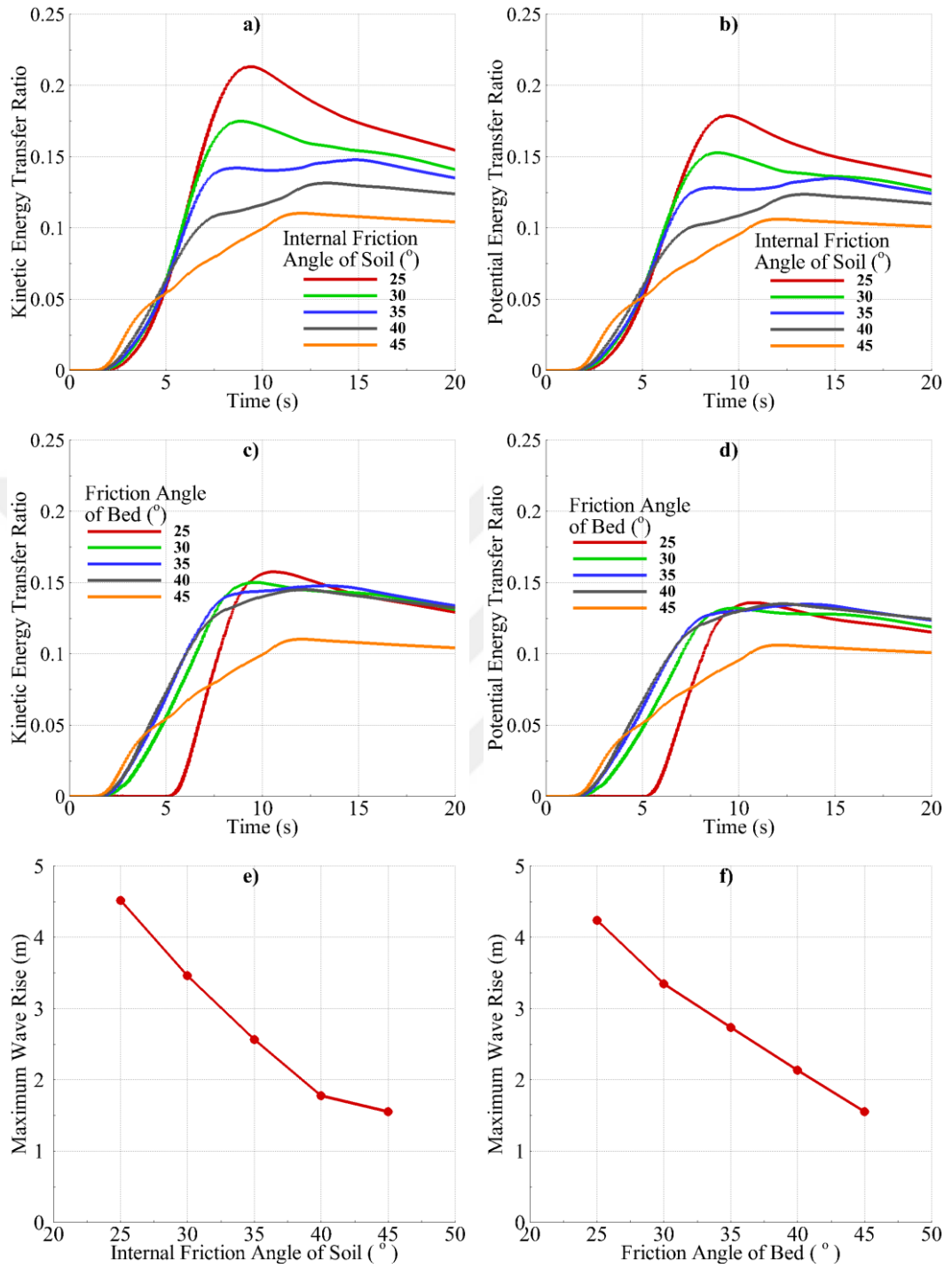
Figure 5.24: a) KETR vs. Time for Case-D6, b) PETR vs. Time for Case-D6, c) KETR vs. Time for Case-D7, d) PETR vs. Time for Case-D7, e) Maximum Wave Rise vs. Internal Friction Angle of Soil for Case-D6 and f) Maximum Wave Rise vs. Friction Angle of Bed for Case-D7
