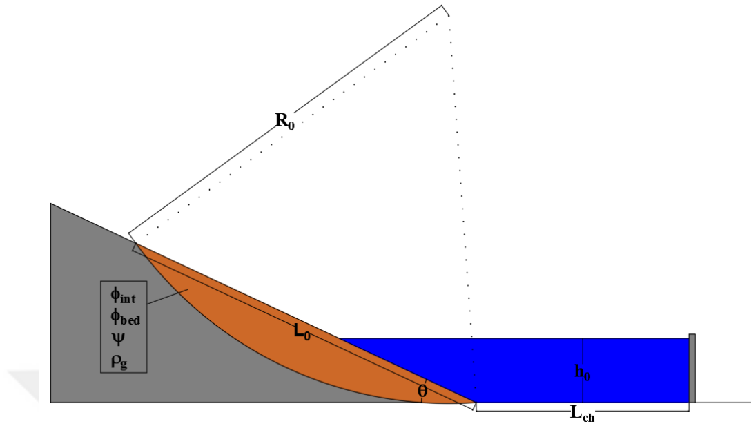
Figure 5.36: Assumed Test Geometry for the Two-Layer Circular Landslide and Earthquake Model
