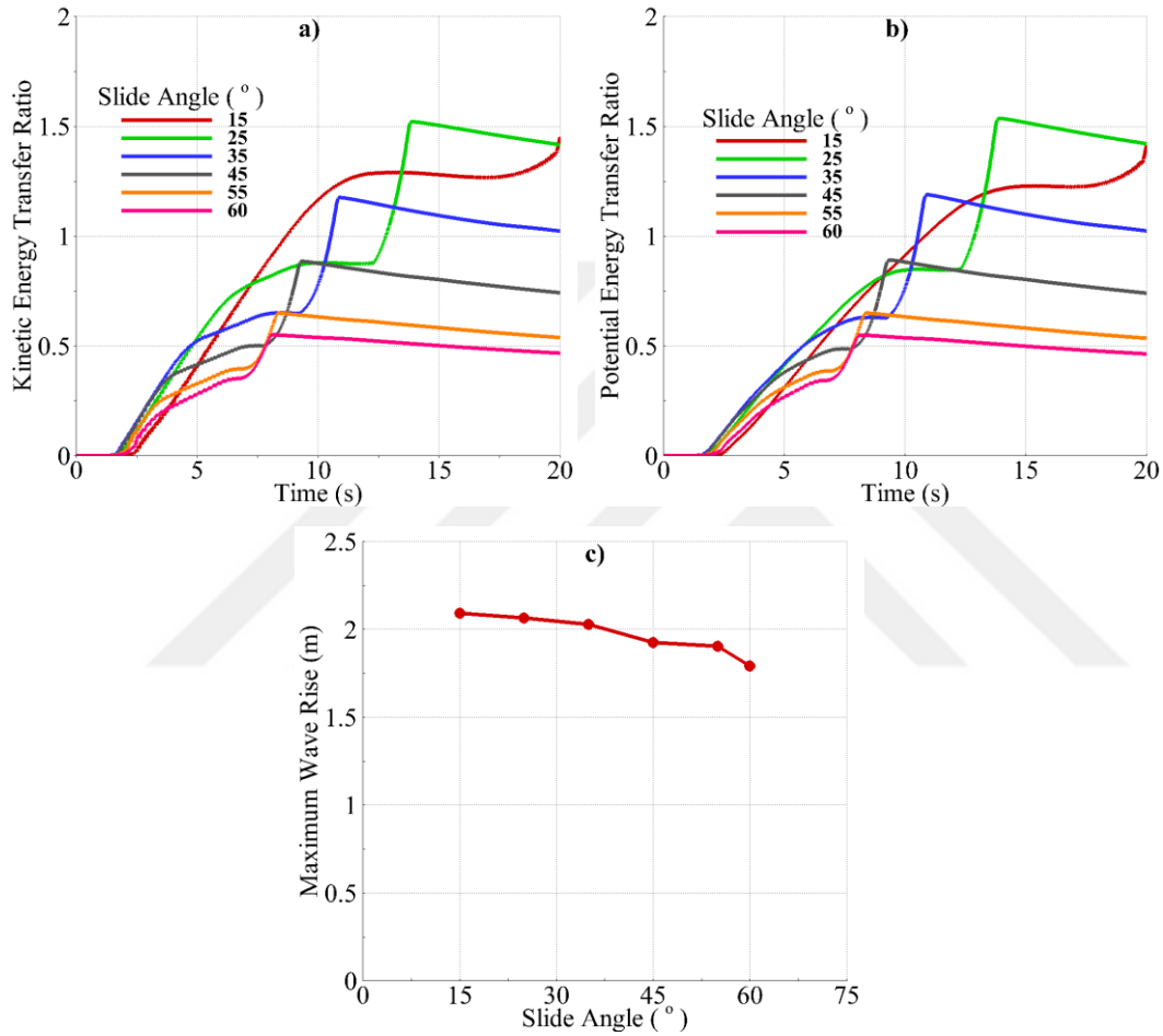
Figure 5.9: For Case-B6; a) KETR vs. Time, b) PETR vs. Time, c) Maximum Wave Rise vs. Slide Angle
