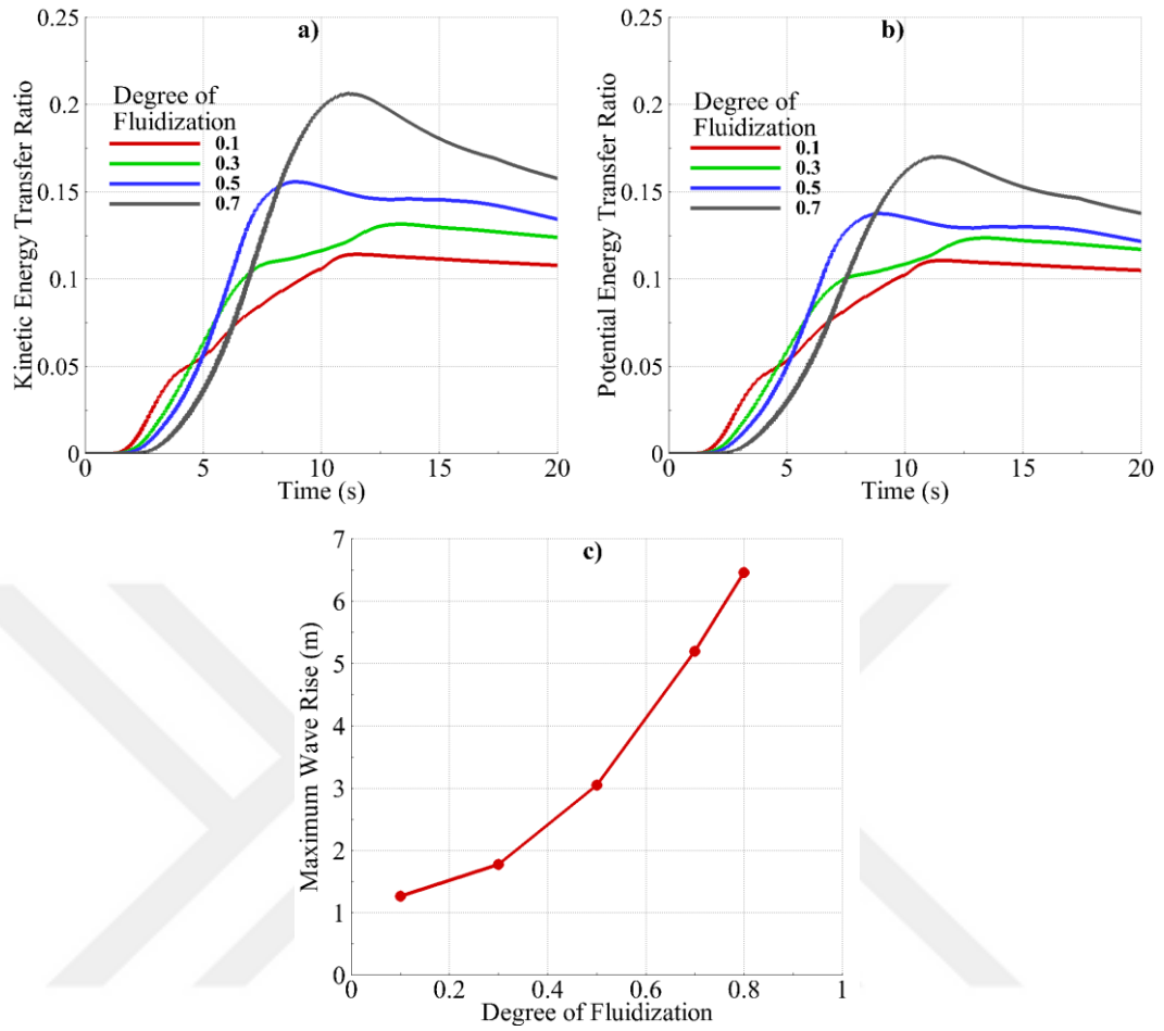
Figure 5.25: For Case-D8; a) KETR vs. Time, b) PETR vs. Time and c) Maximum Wave Rise vs. Degree of Fluidization
