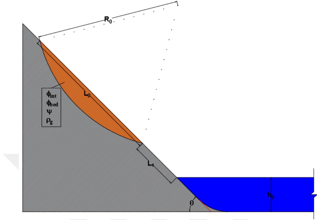
Figure 5.18: Assumed Test Geometry for the Two-Layer Subaerial Circular Landslide Model
