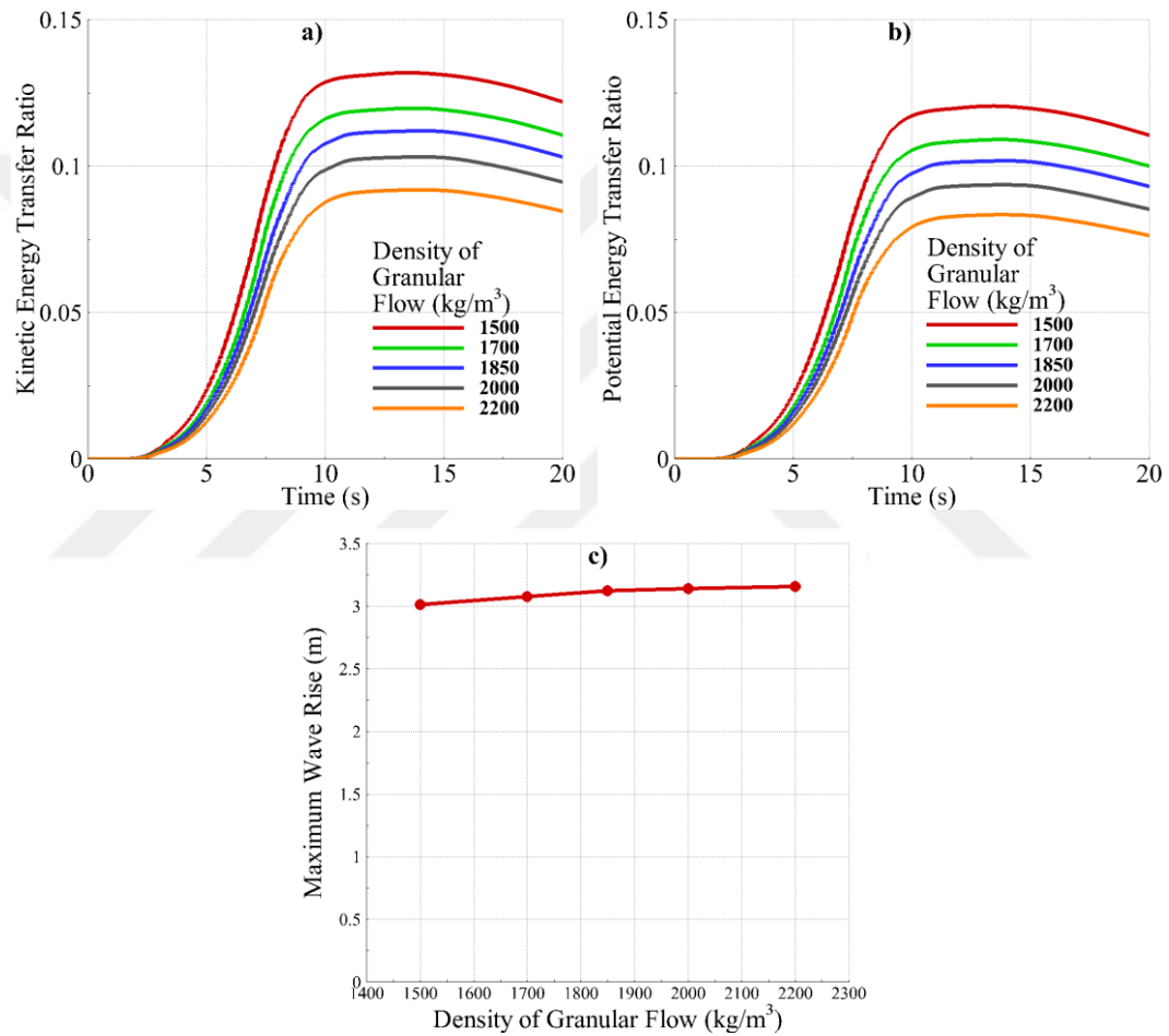
Figure 5.16: For Case-C8; a) KETR vs. Time, b) PETR vs. Time and c) Maximum Wave Rise vs. Density of Granular Flow
