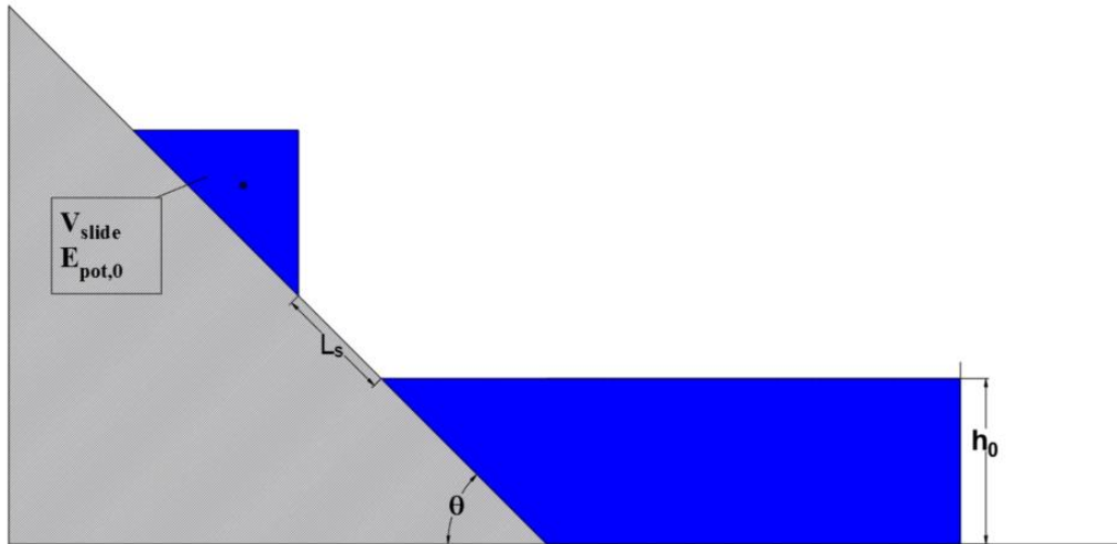
Figure 5.1: Assumed Test Geometry for the One-Layer Model
