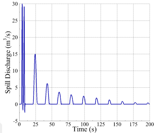
Figure 5.39: Spill discharge for Simulation-3 of Case-E1
