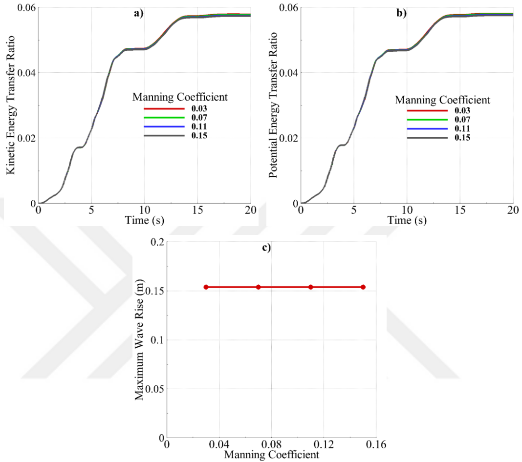
Figure 5.35: For Case-D20; a) KETR vs. Time, b) PETR vs. Time and c) Maximum Wave Rise vs. Manning Coefficient
