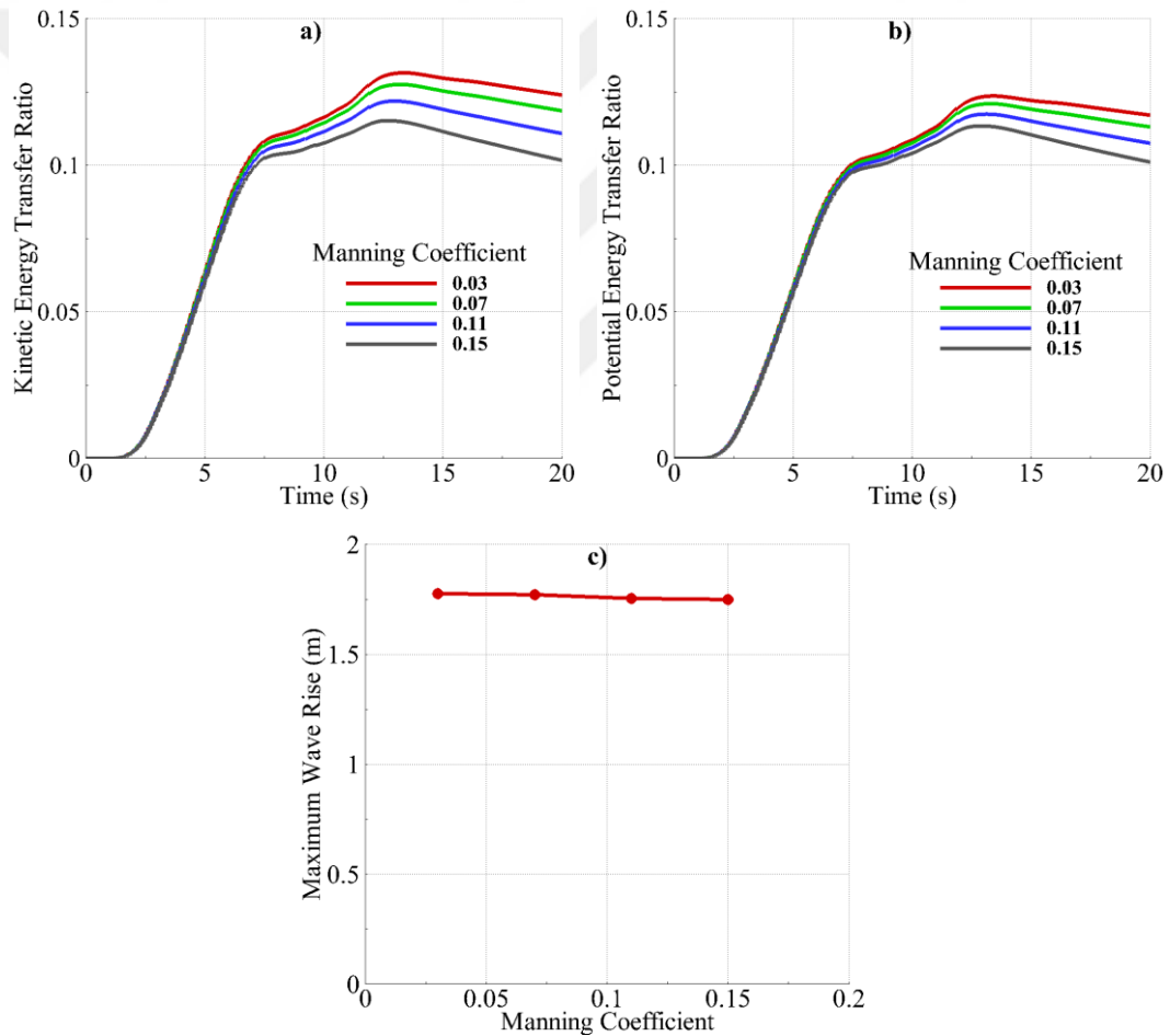
Figure 5.27: For Case-D10; a) KETR vs. Time, b) PETR vs. Time and c) Maximum Wave Rise vs. Manning Coefficient
