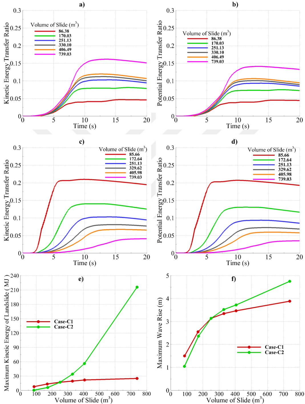
Figure 5.11: a) KETR vs. Time for Case-C1; b) PETR vs. Time for Case-C1; c) KETR vs. Time for Case-C2; d) PETR vs. Time for Case-C2; e) Maximum Kinetic
