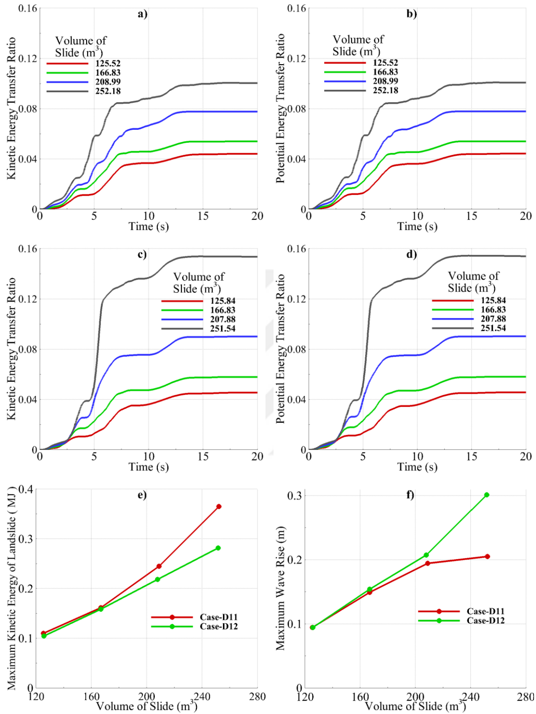
Figure 5.28: a) KETR vs. Time for Case-D11, b) PETR vs. Time for Case-D11, c) KETR vs. Time for Case-D12, d) PETR vs. Time for Case-D12, e) Maximum Kinetic Energy of the Landslide vs. Volume of Slide for Cases-D11 & D12 and f) Maximum Wave Rise vs. Volume of Slide for Cases-D11 & D12
