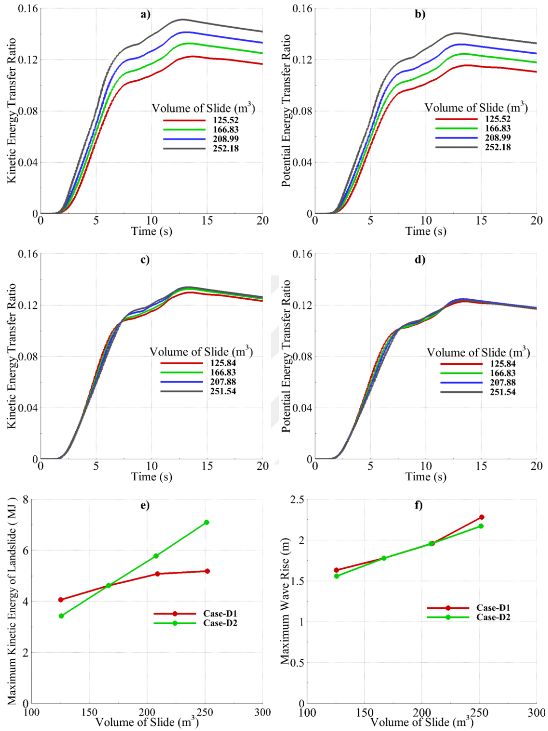
Figure 5.20: a) KETR vs. Time for Case-D1; b) PETR vs. Time for Case-D1; c) KETR vs. Time for Case-D2; d) PETR vs. Time for Case-D2; e) Maximum Kinetic Energy of Landslide vs. Volume of Slide for Cases-D1 & D2 and f) Maximum Wave Rise vs. Volume of Slide for Cases-D1 & D2
