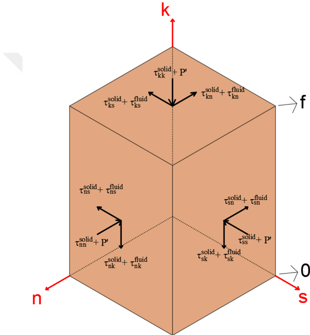
C. 1. Applied Stresses on a Single Mesh of The Granular Flow
