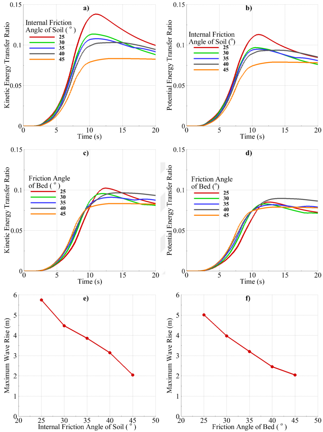
Figure 5.14: a) KETR vs. Time for Case-C5, b) PETR vs. Time for Case-C5, c) KETR vs. Time for Case-C6, d) PETR vs. Time for Case-C6, e) Maximum Wave Rise vs. Internal Friction Angle of Soil for Case-C5 and f) Maximum Wave Rise vs. Friction Angle of Bed for Case-C6
