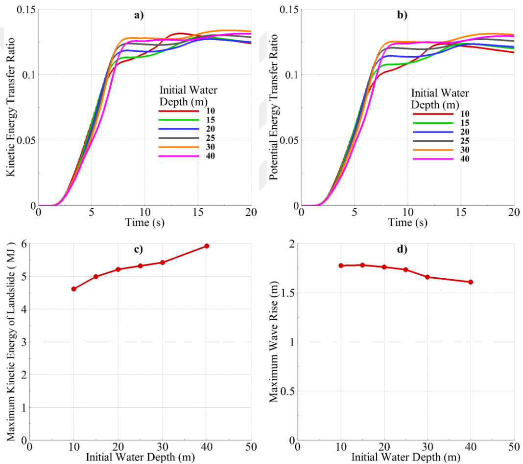
Figure 5.23: For Case-D5; a) KETR vs. Time, b) PETR vs. Time, c) Maximum Kinetic Energy of the Landslide vs. Initial Water Depth and d) Maximum Wave Rise vs. Initial Water Depth
