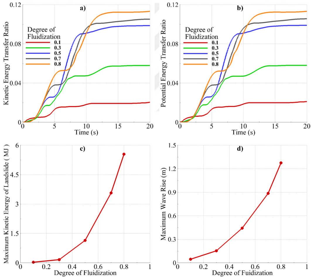
Figure 5.33: For Case-D18; a) KETR vs. Time, b) PETR vs. Time, c) Maximum Kinetic Energy of the Landslide vs. Degree of Fluidization and d) Maximum Wave Rise vs. Degree of Fluidization
