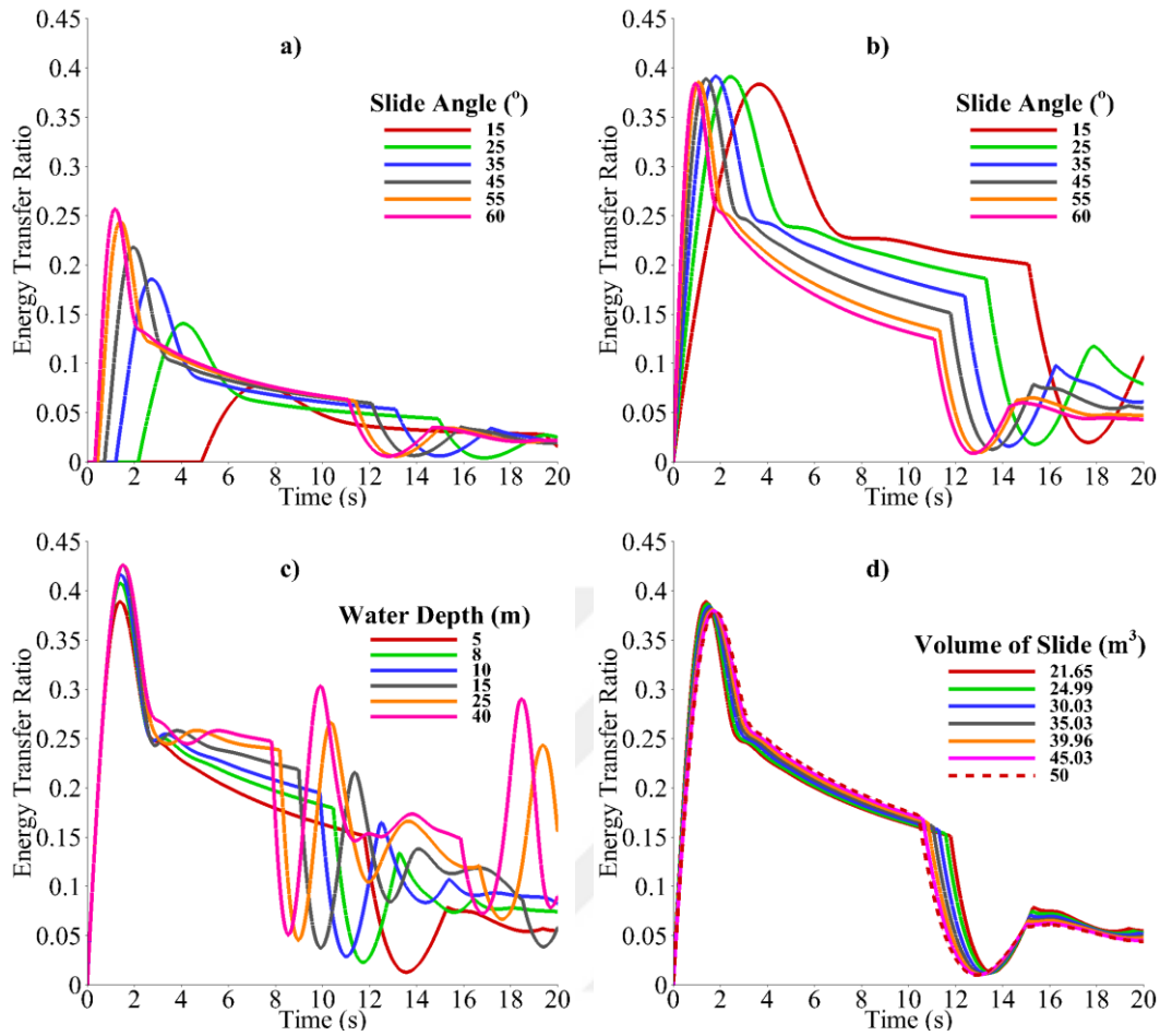
Figure 5.2: Energy Transfer Ratio vs. Time a) for Case-A1; b) for Case-A2; c) for Case-A3; d) for Case-A4
