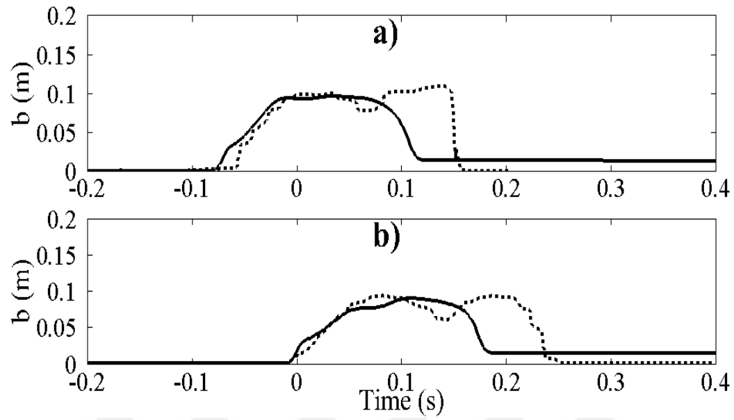
Figure 4.4: Laboratory (dashed line) and Numerical (Solid line) Experiments measured at a) LDS-1 and b) LDS0
