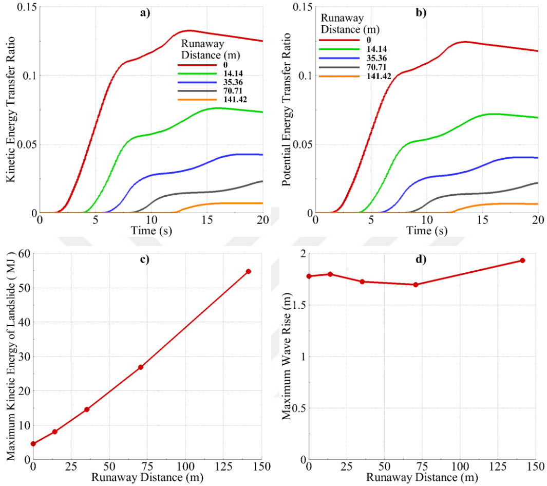
Figure 5.21: For Case-D3; a) KETR vs. Time, b) PETR vs. Time, c) Maximum Kinetic Energy of the Landslide vs. Runaway Distance and d) Maximum Wave Rise vs. Runaway Distance
