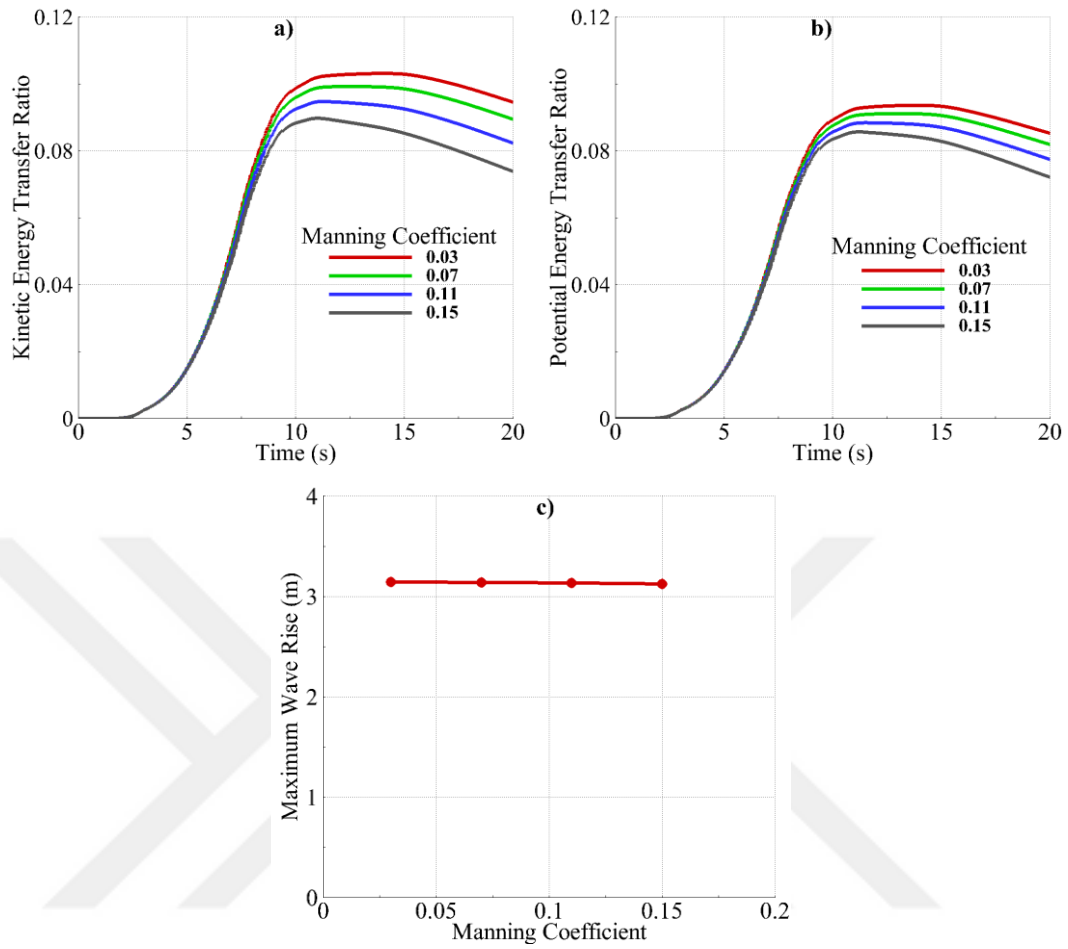
Figure 5.17: For Case-C9; a) KETR vs. Time, b) PETR vs. Time and c) Maximum Wave Rise vs. Manning Coefficient
