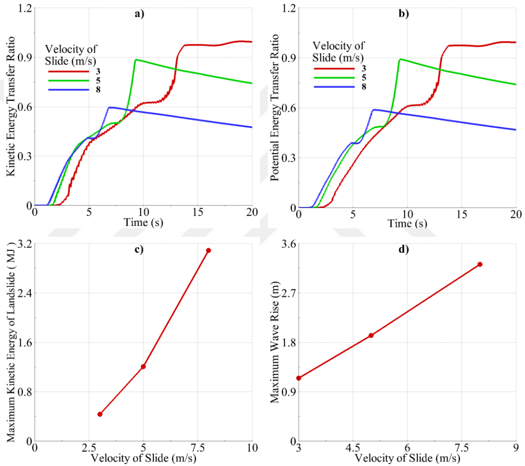
Figure 5.7: For Case-B4; a) KETR vs. Time, b) PETR vs. Time, c) Maximum Kinetic Energy of Landslide vs. Velocity of Slide and d) Maximum Wave Rise vs. Velocity of Slide
