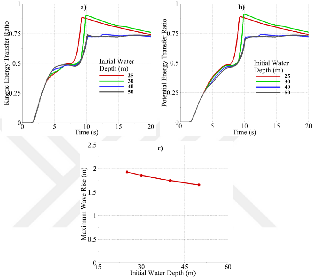
Figure 5.8: For Case-B5; a) KETR vs. Time, b) PETR vs. Time, c) Maximum Wave Rise vs. Initial Water Depth
