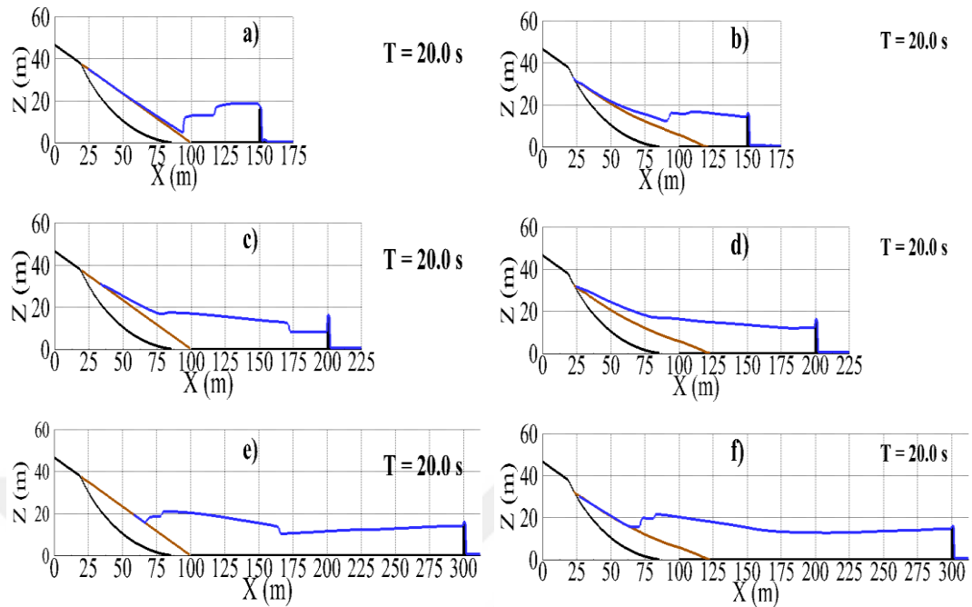
Figure 5.41: Screenshots of Simulation-2 when Channel Length is; a) 50 meters; c) 100 meters and e) 200 meters and of Simulation-3 when Channel Length is; b) 50 meters; d) 100 meters and f) 200 meters at Time = 20.0 Seconds
