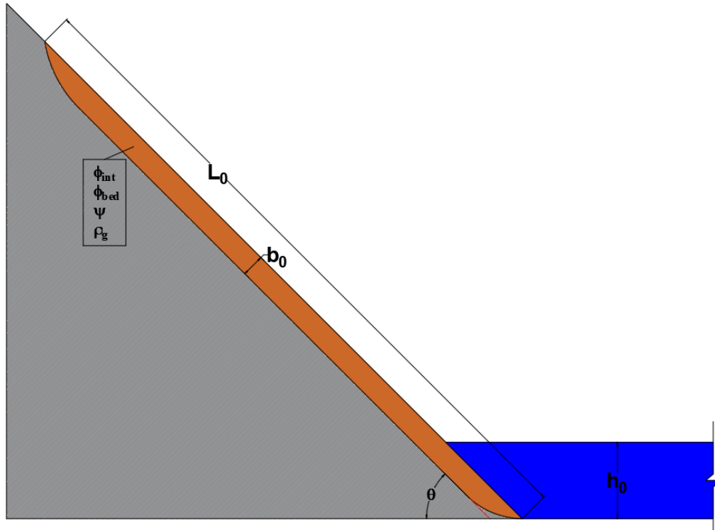
Figure 5.10: Assumed Test Geometry for the Two-Layer Translational Landslide Model
