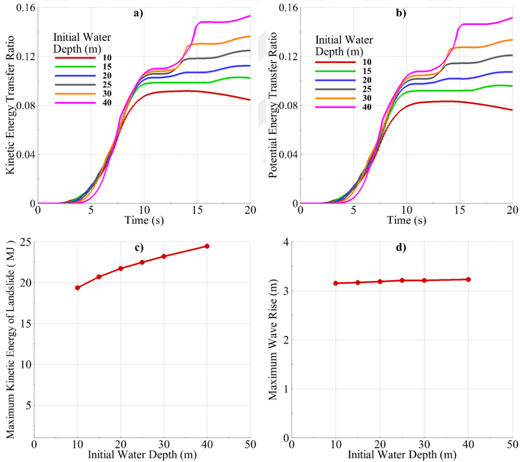
Figure 5.13: For Case-C4; a) KETR vs. Time, b) PETR vs. Time, c) Maximum Kinetic Energy of Landslide vs. Initial Water Depth and d) Maximum Wave Rise vs. Initial Water Depth
