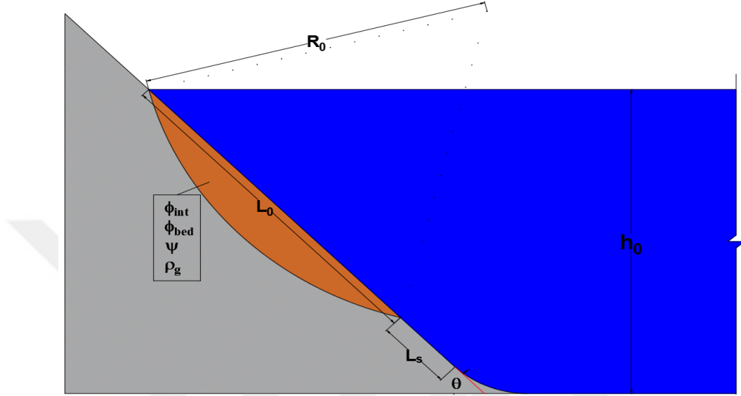
Figure 5.19: Assumed Test Geometry for the Two-Layer Submarine Circular Landslide Model
