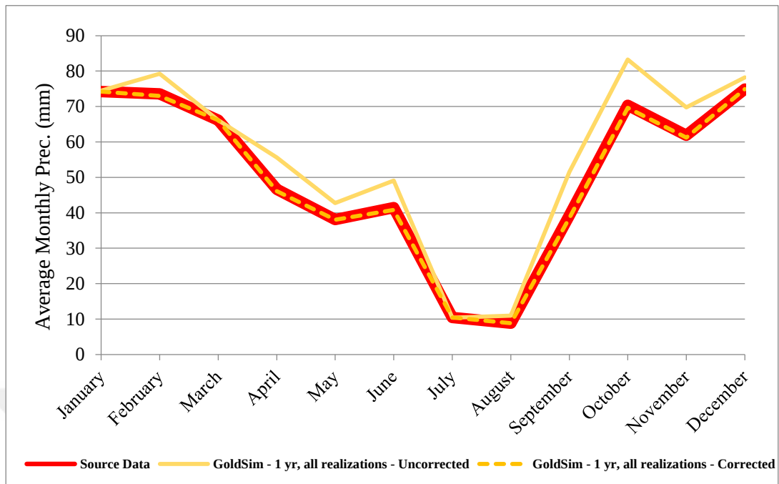
Figure 2.12. Comparison of Source (Project Site), Uncorrected and Corrected WGEN Generated Data for 1-year simulation
