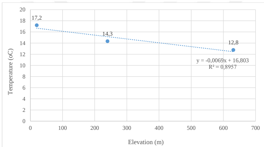
Figure 2.5. Elevation vs Annual Average Temperature Relationship
