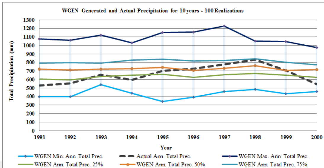
Figure 2.14. WGEN Generated and Actual Precipitation for 10 years – 100 realizations
