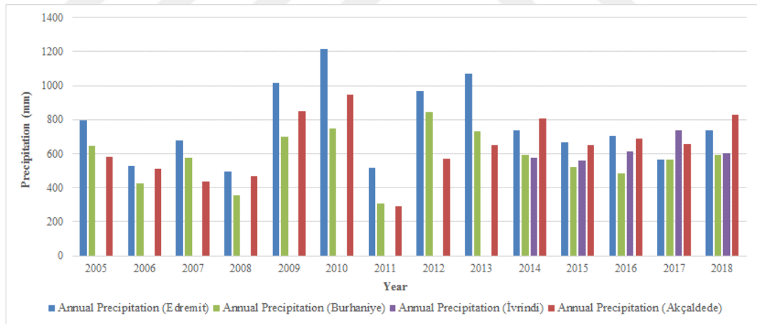
Figure 2.3. Annual Total Precipitation Amount for the Stations between 2005-2018 Period
