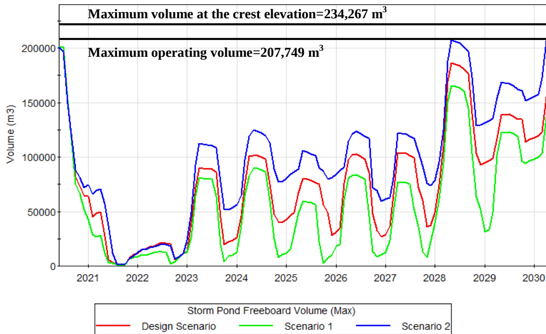
Figure 4.9. Storm Pond Operating Volumes for Different Scenarios
