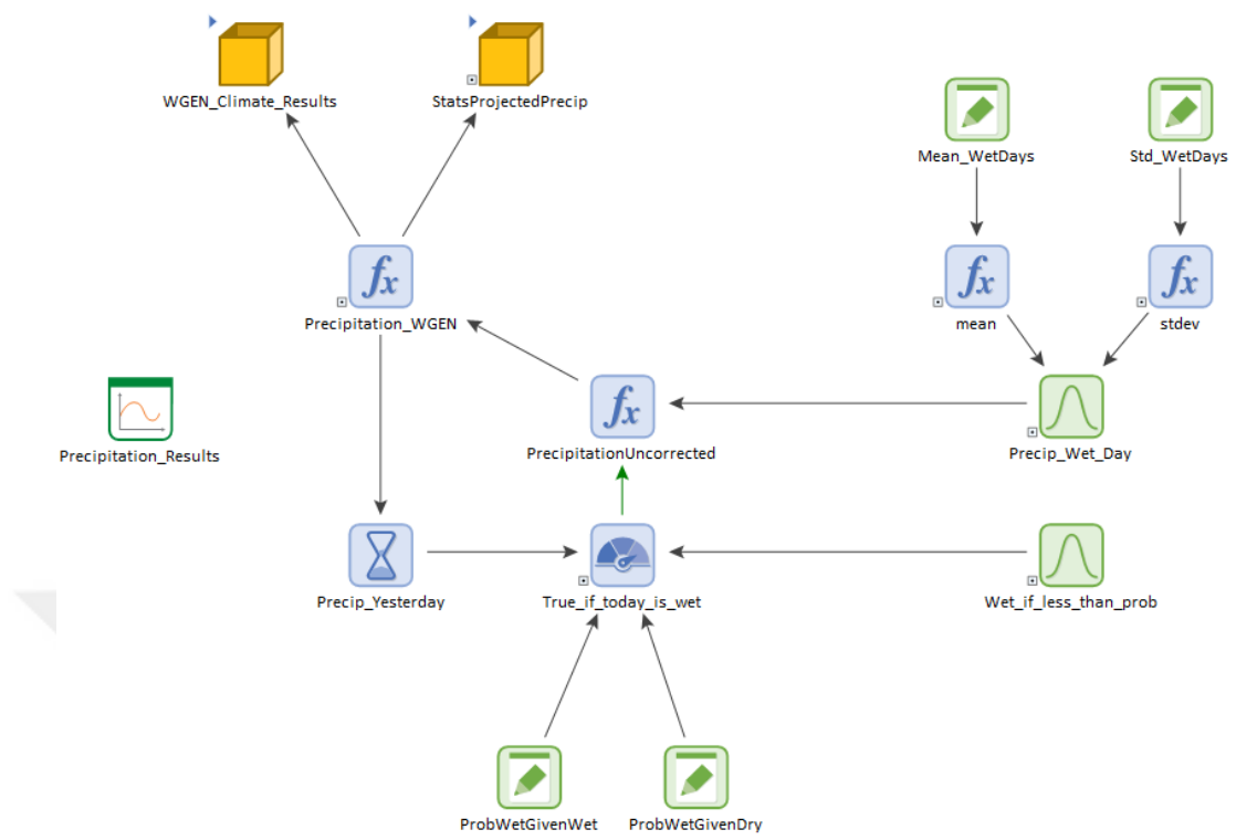
Figure 2.10. WGEN Container with Generated Model Inputs
