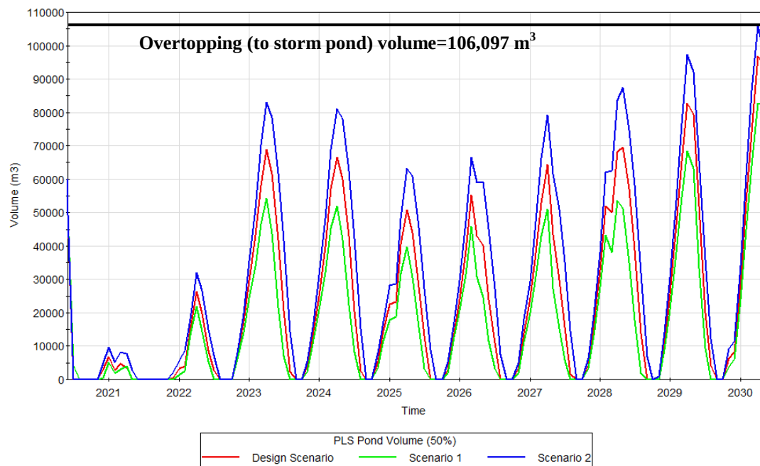
Figure 4.8. PLS Pond Operating Volumes for Different Scenarios
