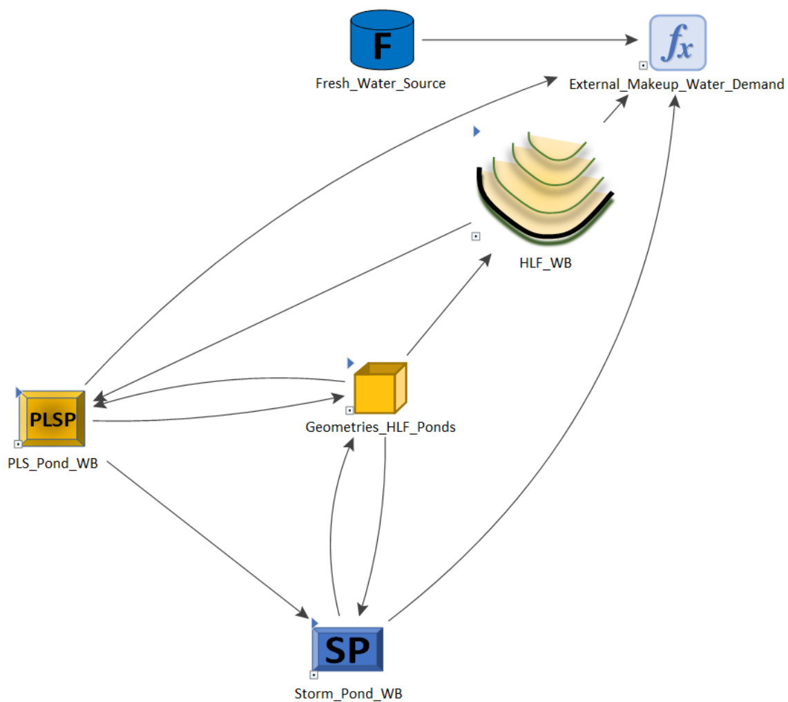
Figure 3.3. Operational Heap Leach Water Balance Containers, Elements, and Influences
