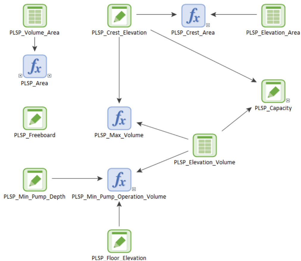
Figure 3.5. Elements and Influences Inside the PLS Pond Geometry Container
