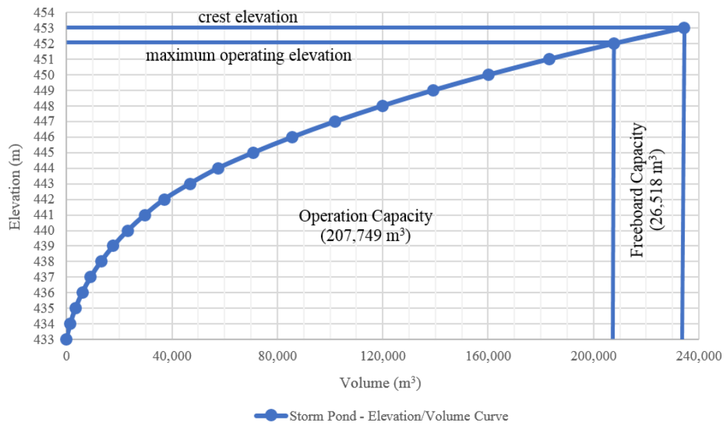
Figure 3.8. Stage-Storage Curve for the Storm Pond
