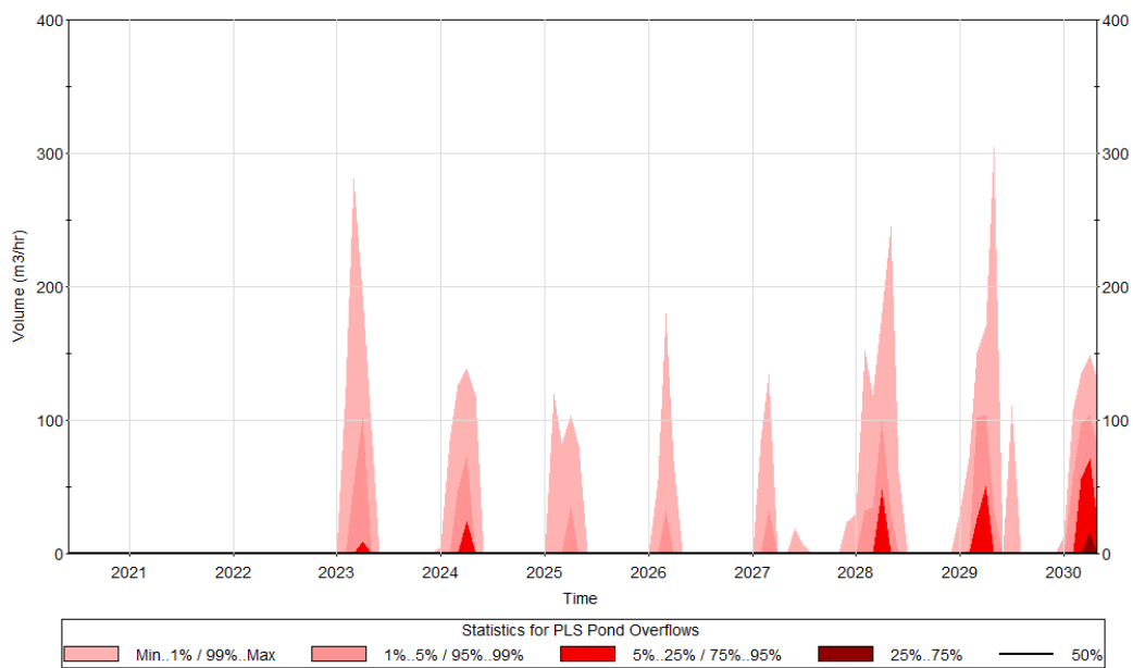
Figure 4.4. PLS Pond Probabilistic Overflows
