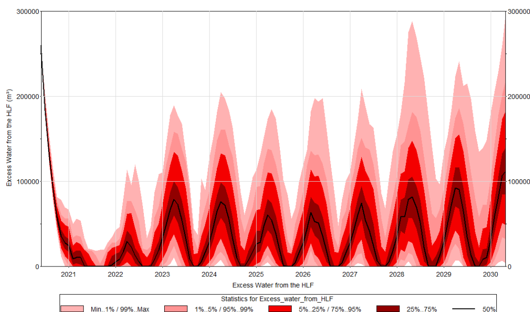
Figure 4.6. Probabilistic Excess Water Volumes (PLS Pond + Storm Pond) from the HLF
