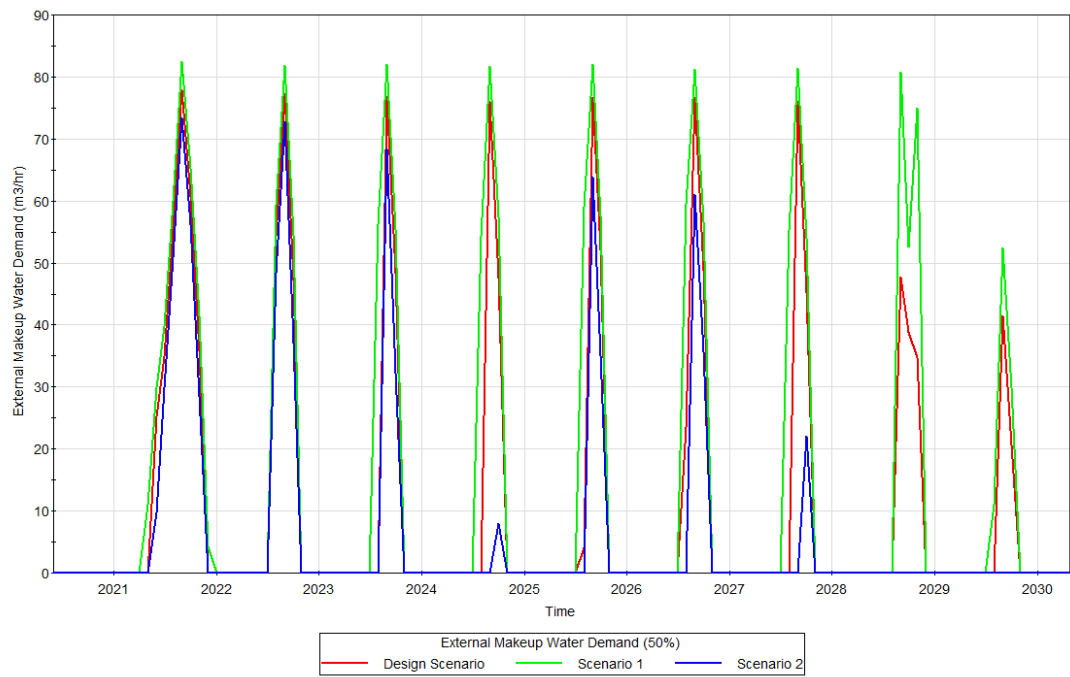
Figure 4.10. External Makeup Water Demand for Different Scenarios
