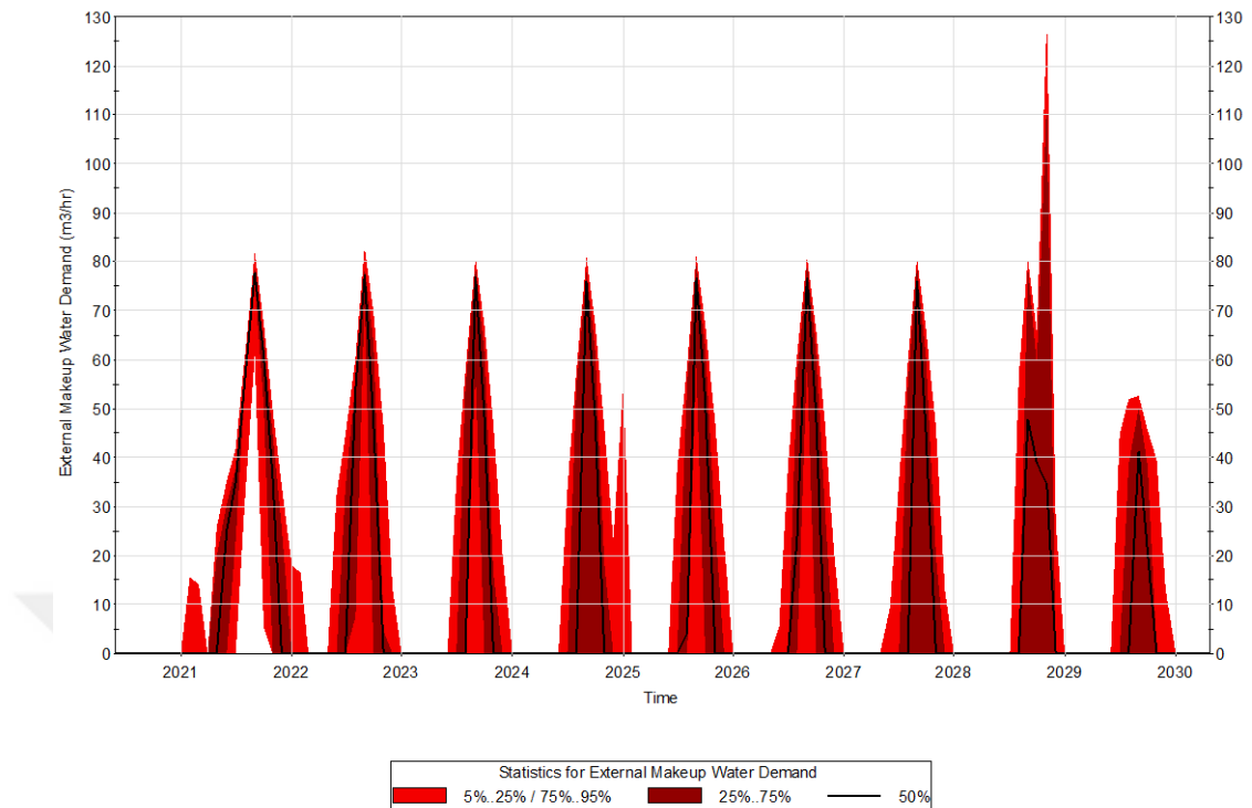
Figure 4.7. Probabilistic External Makeup (Raw) Water Demand
