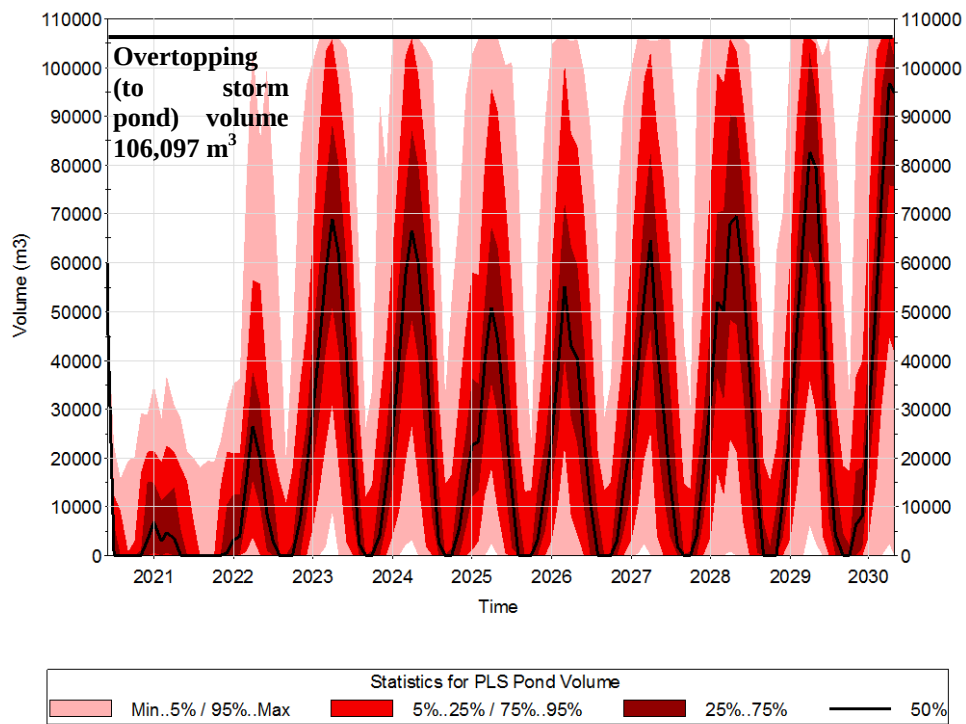
Figure 4.3. PLS Pond Probabilistic Operating Volumes
