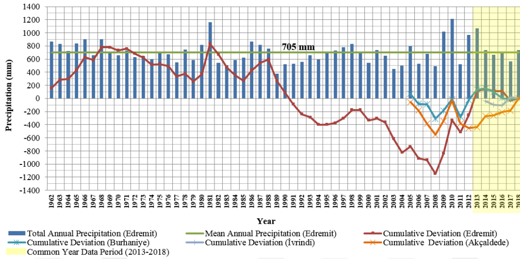
Figure 2.2. Total Annual Precipitation and Mean Annual Precipitation for the Edremit Station together the Cumulative Deviations from Mean Annual Precipitations of the Edremit, Burhaniye, İvrindi and Akçaldede Stations
