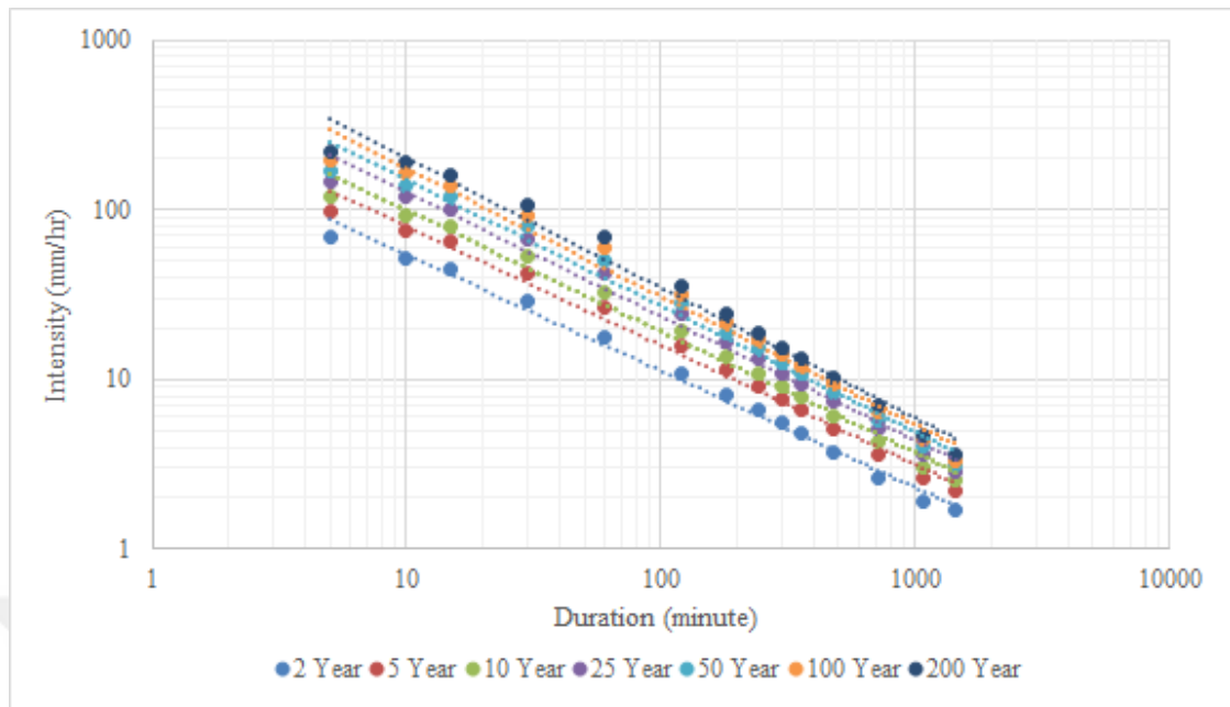
Figure 2.15. IDF Curve for the Project Site
