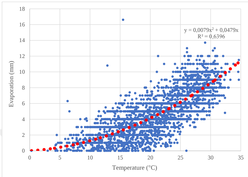
Figure 2.6. Temperature vs Evaporation for Edremit Station (1962-2018)
