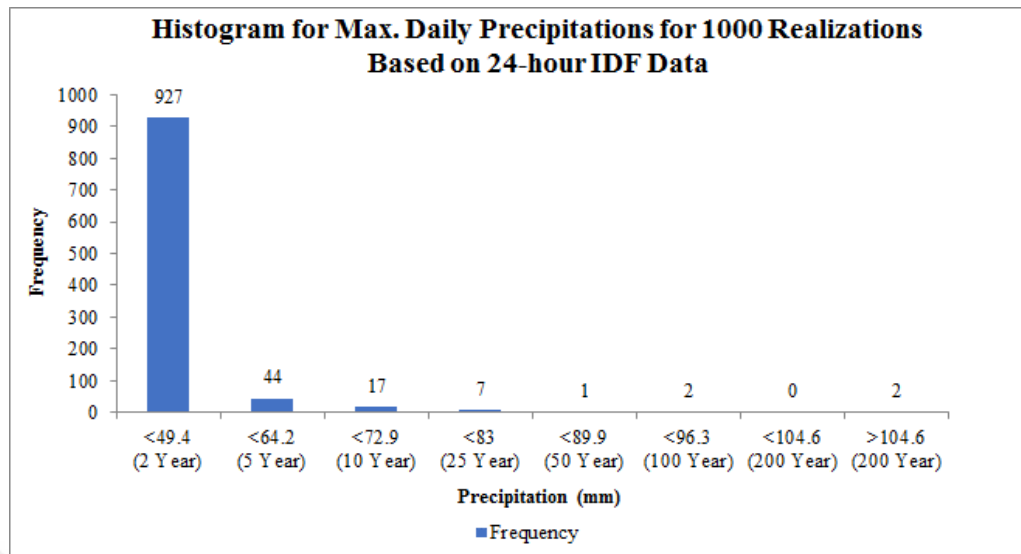
Figure 4.2. Histogram for Maximum Daily Precipitations for 1000 Realizations Based on the 24-Hour IDF Data
