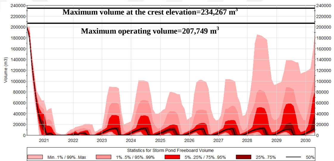
Figure 4.5. Storm Pond Probabilistic Operating Volumes
