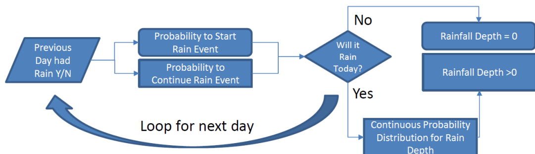
Figure 2.9. WGEN Synthetic Precipitation Generator Operation Logic (Hoekstra, 2015)
