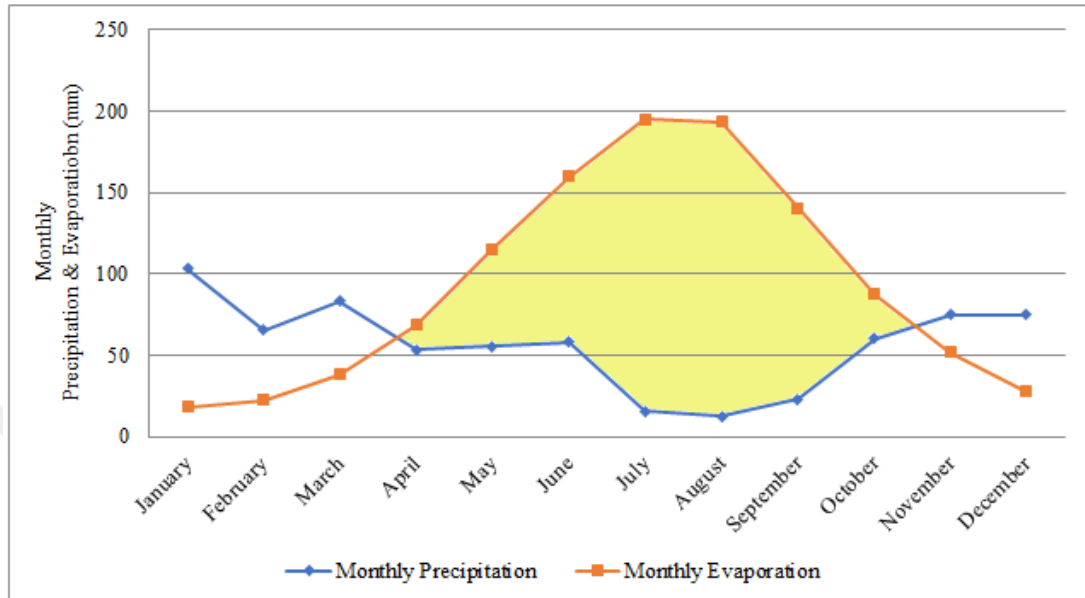
Figure 2.7. Monthly Precipitation and Evaporation (in mm) for the Proposed Heap Leach Site
