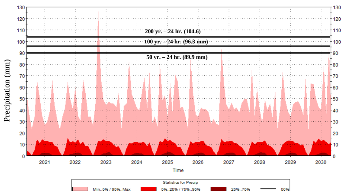
Figure 4.1. WGEN Generated Daily Precipitation Data for 10-years with 1000 Simulations
