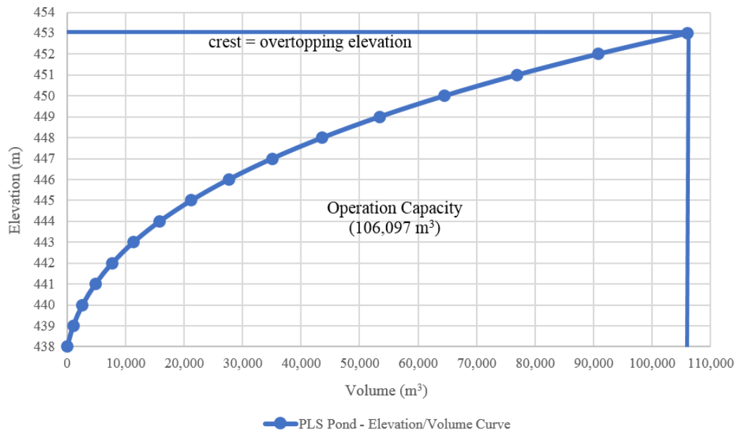
Figure 3.6. Stage-Storage Curve for the PLS Pond
