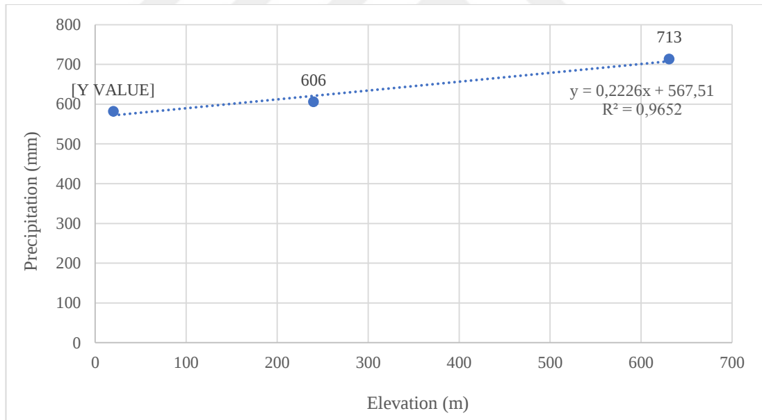
Figure 2.4. Elevation vs Total Annual Precipitation Relationship
