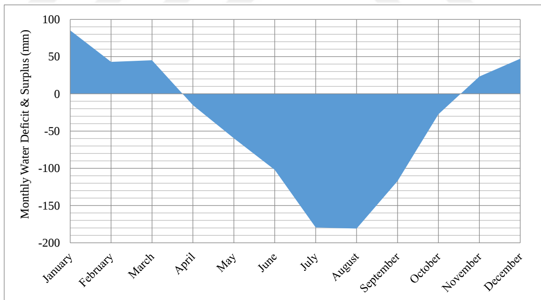
Figure 2.8. Monthly Water Deficit and Surplus (in mm) for the Proposed Heap Leach Site
