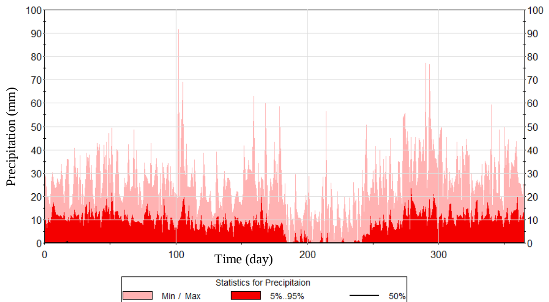
Figure 2.13. WGEN Generated Daily Precipitation Data for 1-year (365 days) with 100 Simulations (January 1 through December 31)
