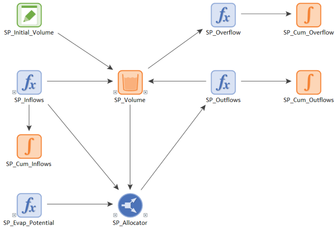
Figure 3.10. Elements and Influences Inside the Storm Pond Water Balance Container
