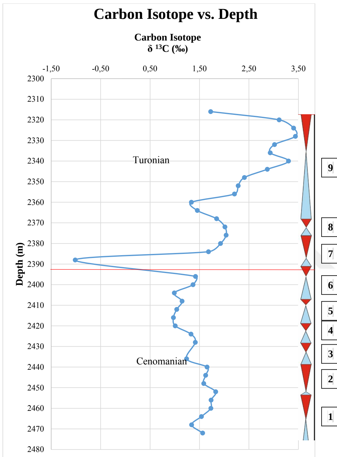
Figure 97. Carbon isotope data vs. depth (m) graph of K-2 well based on the data of Table 7 (Red line shows the C-T boundary)
