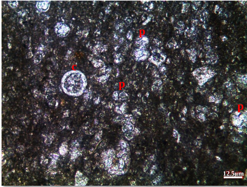
Figure 56. Skeletal calcisphaerulid-bearing planktonic foraminiferal wackestone to packstone microfacies from the thin section at 1695.03 m of the K-11 well (s: skeletal fragments; c: calcisphaerulid ( Pithonella spherica ); p: planktonic foraminifer)
