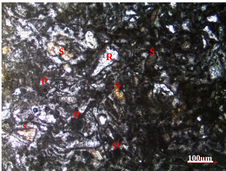
Figure 48. Skeletal peloidal packstone to grainstone microfacies from the thin section at 1772.17 m of the K-11 well (s: skeletal fragments; R: recrystallized skeletal fragment; p: peloid)
