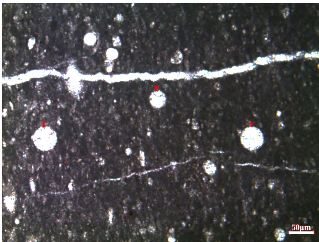
Figure 69. Radiolaria-bearing mudstone microfacies from the thin section at 1697.42 m of the K-11 well (r: calcified radiolaria)
