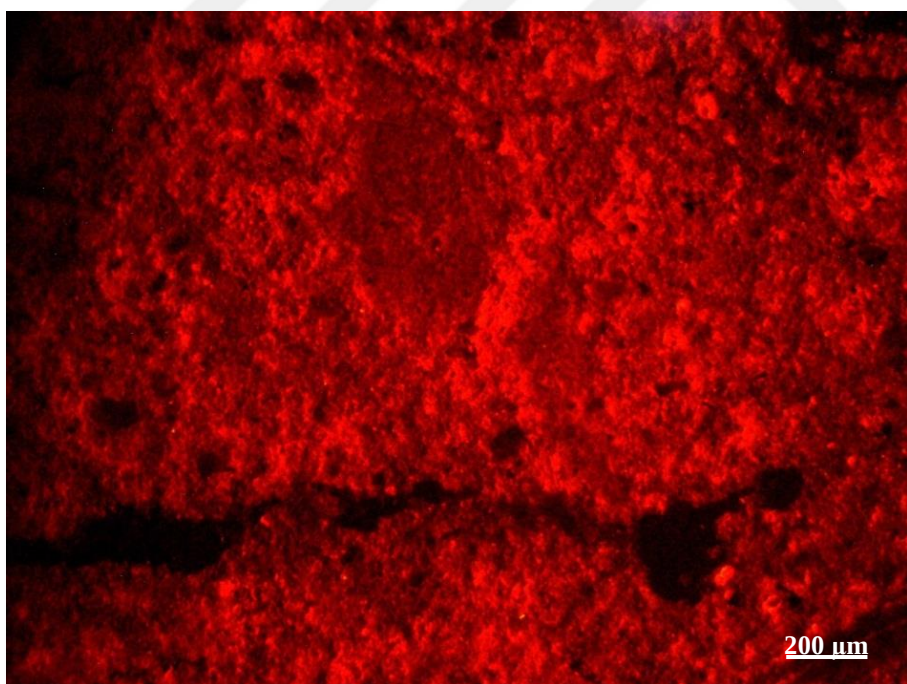
Figure 6. Light microscope based cathodoluminescence photomicrograph of peloidal facies and fracture of K-2 well
