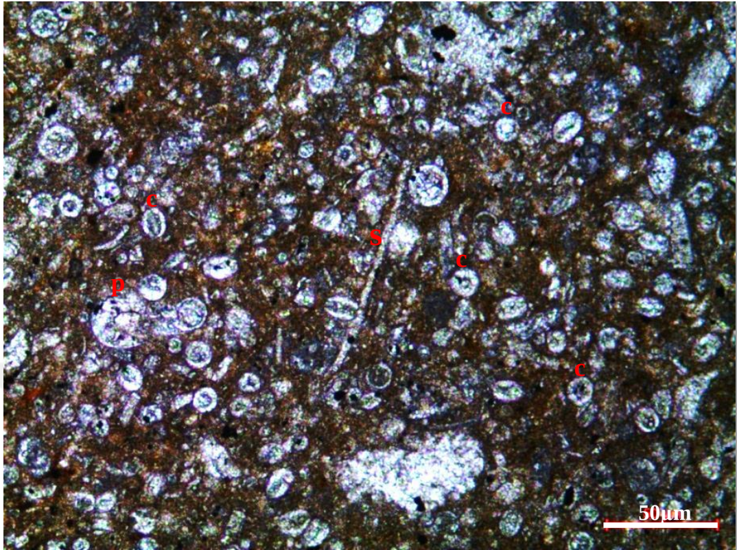
Figure 77. Planktonic foraminiferal skeletal calcisphaerulid-bearing wackestone to packstone microfacies from the thin section at 1722.82 m of the K-11 well (p: planktonic foraminifer; s: skeletal fragments (thin walled mollusk (pelecypod)); c: calcisphaerulid ( Pithonella spherica and Pithonella ovalis ))
