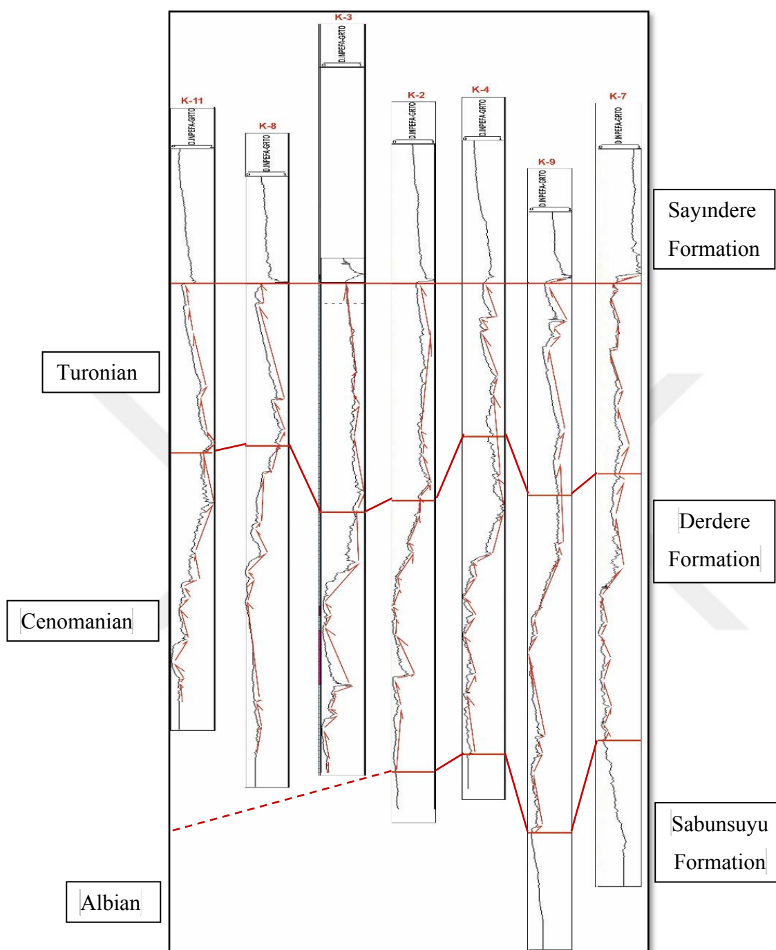
Figure 85. From west to east INPEFA log responses with interpretation (K-11, K-8, K-3, K-2, K-4, K-9, and K-7) (The direction of red arrows shows shoaling upward and deepening upward packages in the sequences. Going through right means deepening, going through left means shoaling. Red lines show timelines including Albian-Cenomanian and Cenomanian-Turonian boundaries.)
