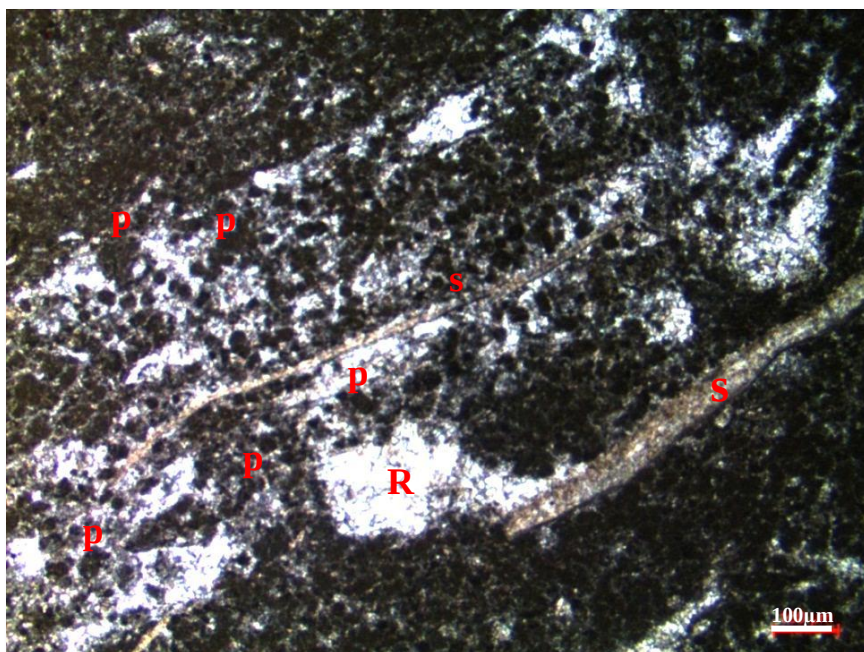
Figure 50. Peloidal skeletal packstone microfacies from the thin section at 1765.08 m of the K-11 well [p: peloid; s: skeletal fragments (possible brachiopod); R: Recrystallization]
