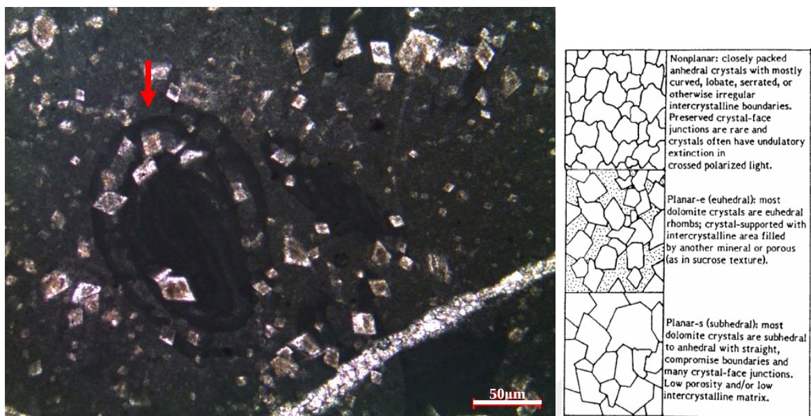
Figure 108. Planar-e dolomite with partly replaced benthic foraminifera and the micrite dominated matrix from thin section at 1800 m of the K-8 well (Dolomite rock texture classification of Gregg and Sibley (1984) is on the right.)
