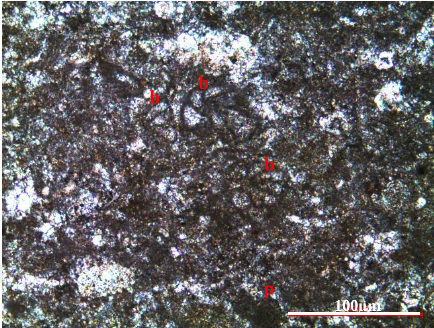
Figure 44. Benthic foraminiferal skeletal peloidal packstone/grainstone microfacies from the thin section at 1767.39 m of the K-11 well (b: benthic foraminifera; p: peloid)
