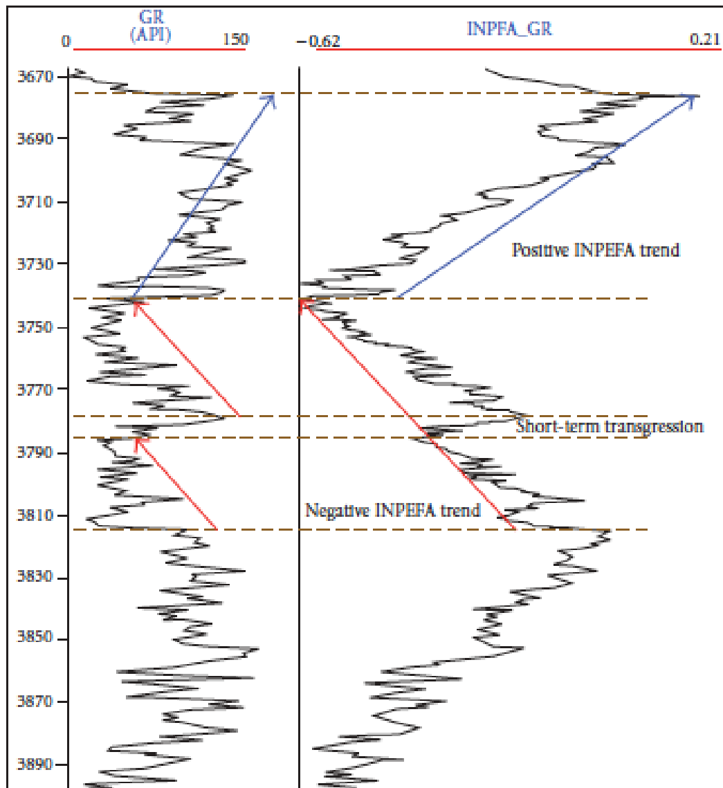
Figure 9. Presentation and correlation of the integrated predictive error filter (INPEFA) short-term curve (Nio et al. 2005; Souza, 2012) showing working principle depend on GR-log. Red arrows show negative INPEFA trend (decreasing upward values of GR and INPEFA-GR shoaling) while blue arrow shows positive INPEFA trend (increasing upward values of GR and INPEFA-GR and deepening). Trends are more visible on INPEFA-GR log compared to GR log.
