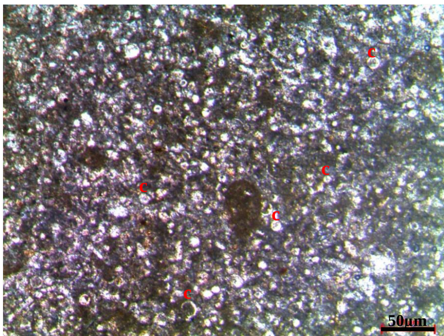
Figure 73. Calcisphaerulid-bearing packstone microfacies from the thin section at 1712 m of the K-11 well (c: calcisphaerulid ( Pithonella spherica ))
