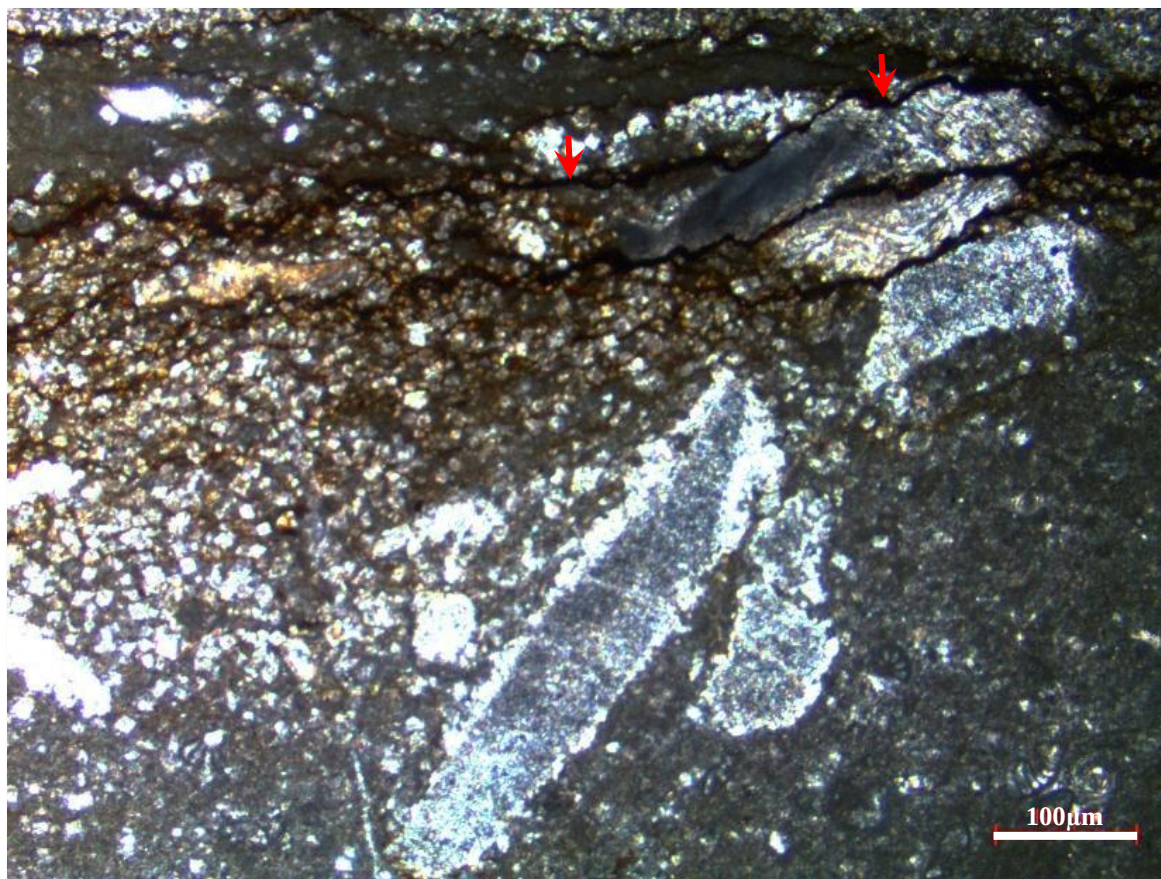
Figure 140. Stylolites associated with dolomitization and formed around the skeletal grains from the thin section at 1780.93 m of the K-11 well
