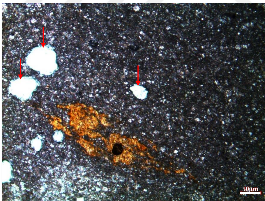
Figure 119. Porous dolomicrosparite microfacies from the thin section samples of 1649.62 m of K-11 well (Red arrows show vuggy porosity.)
