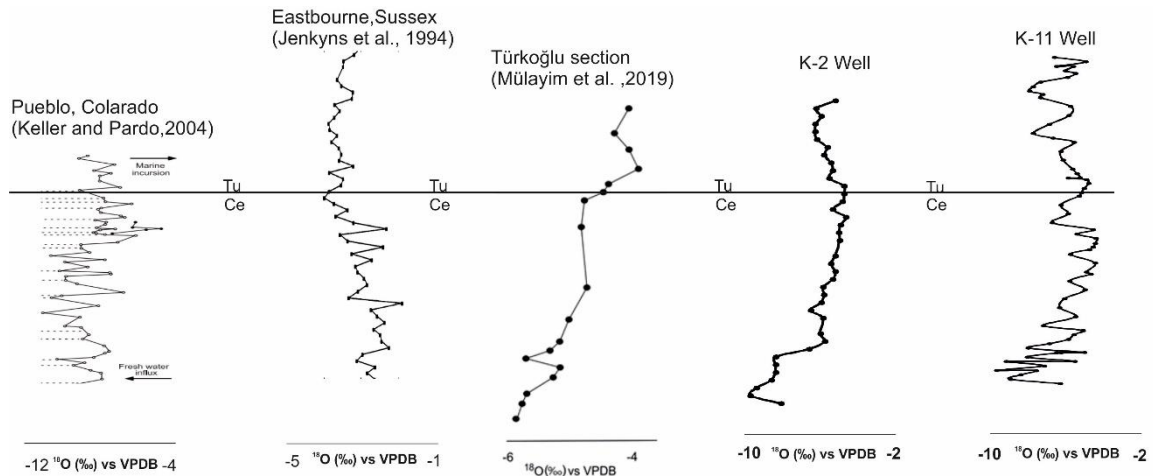
Figure 102. Correlation of O-isotope curve of K-2 and K-11 wells with the curves of Türkoğlu section, the Cenomanian-Turonian time of Eastbourne and Pueblo reference sections
