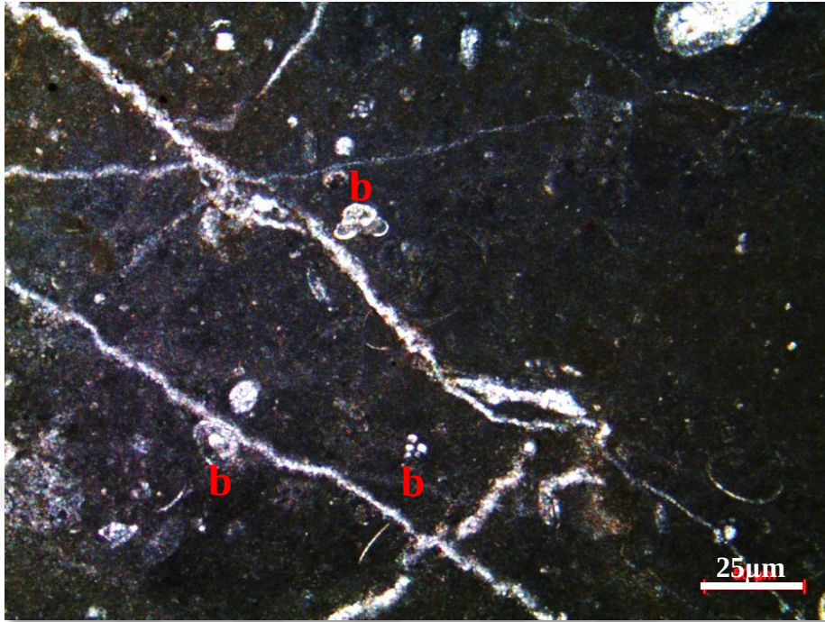
Figure 35. Benthic foraminiferal mudstone microfacies from the thin section at 1778.45m of the K-11 well (b: benthic foraminifera)
