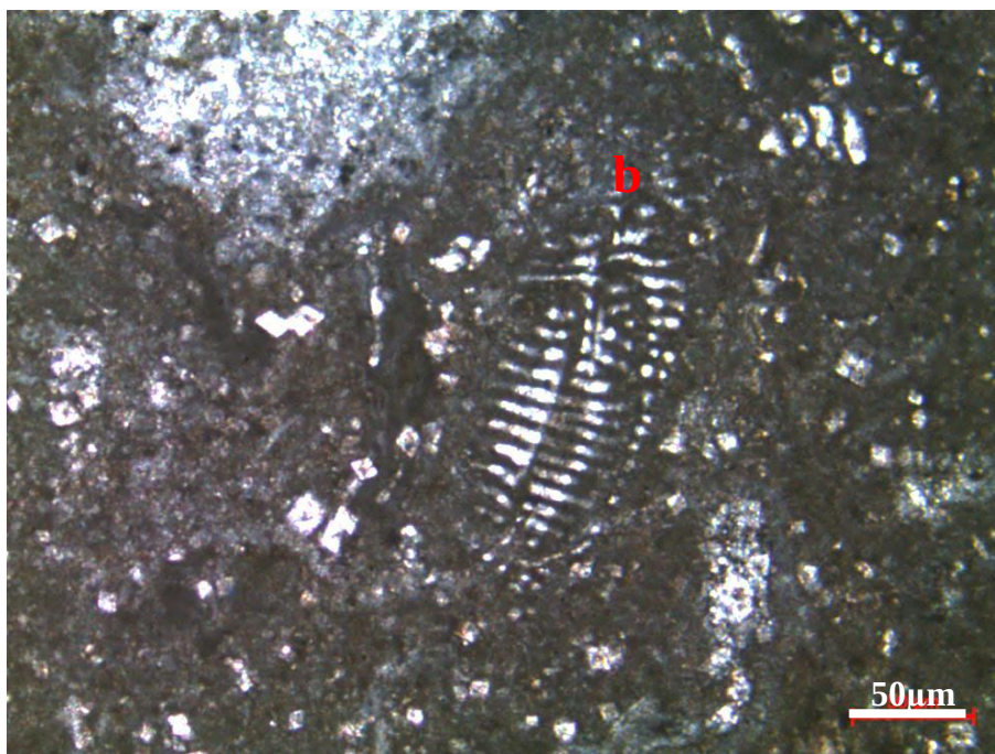
Figure 33. Benthic foraminiferal mudstone microfacies from the thin section at 1780.79 m of the K-11 well (b: benthic foraminifera)
