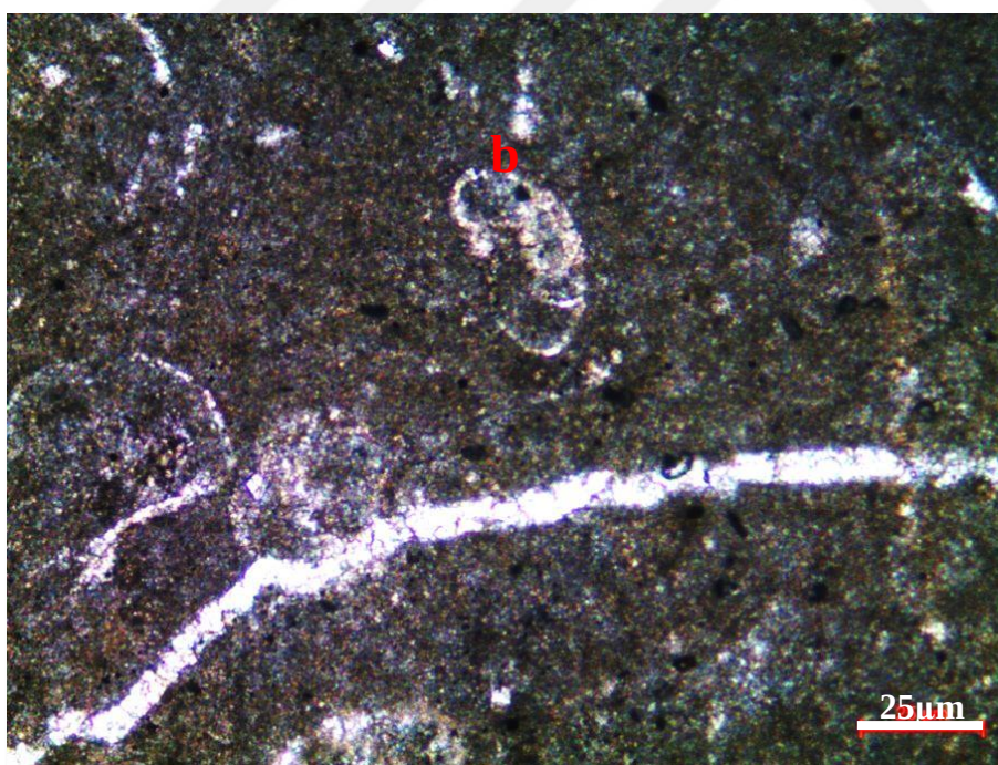
Figure 34. Benthic foraminiferal mudstone microfacies from the thin section at 1778.59 m of the K-11 well (b: benthic foraminifera)
