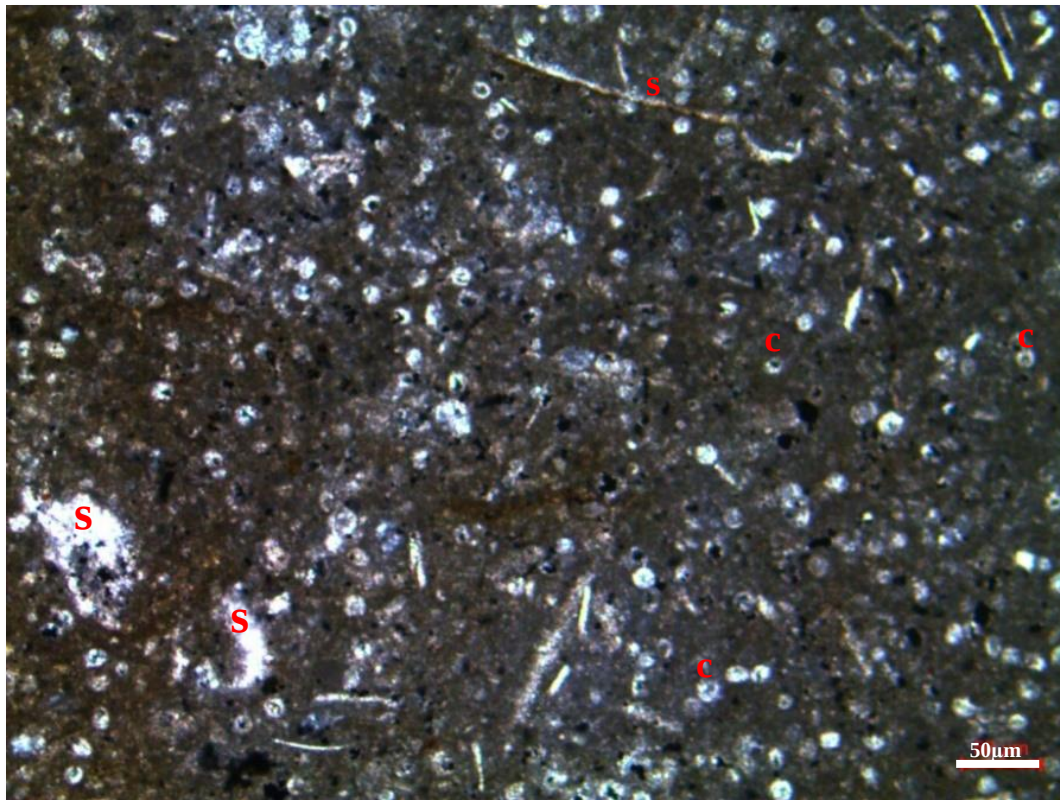
Figure 78. Skeletal calcisphaerulid-bearing wackestone to packstone microfacies from the thin section at 1719.06 m of the K-11 well [s: skeletal fragments (thin walled mollusk (pelecypod) and “ Saccocoma ”; c: calcisphaerulid ( Pithonella spherica )]
