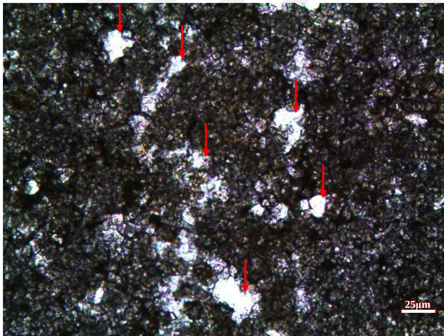
Figure 118. Porous dolomicrosparite microfacies from the thin section at 1649.83 m of the K-11 well (Red arrows show vuggy porosity.)
