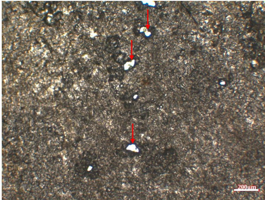
Figure 110. Dolomicrosparite and pore spaces of the K-11 well, plane polar light
