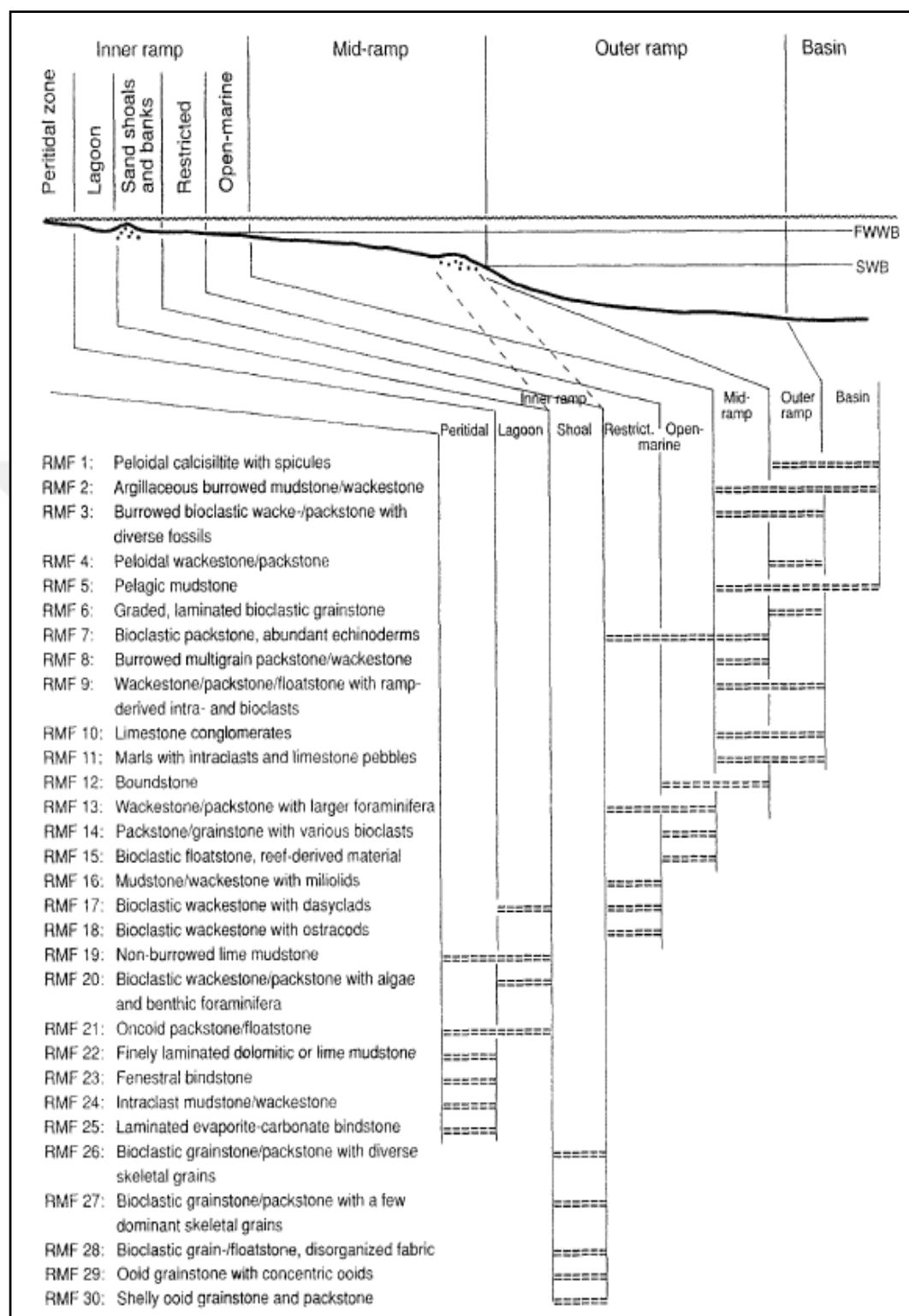
Figure 31. Generalized distribution of microfacies types in different parts of a homoclinal carbonate ramp (Flügel, 2004)
