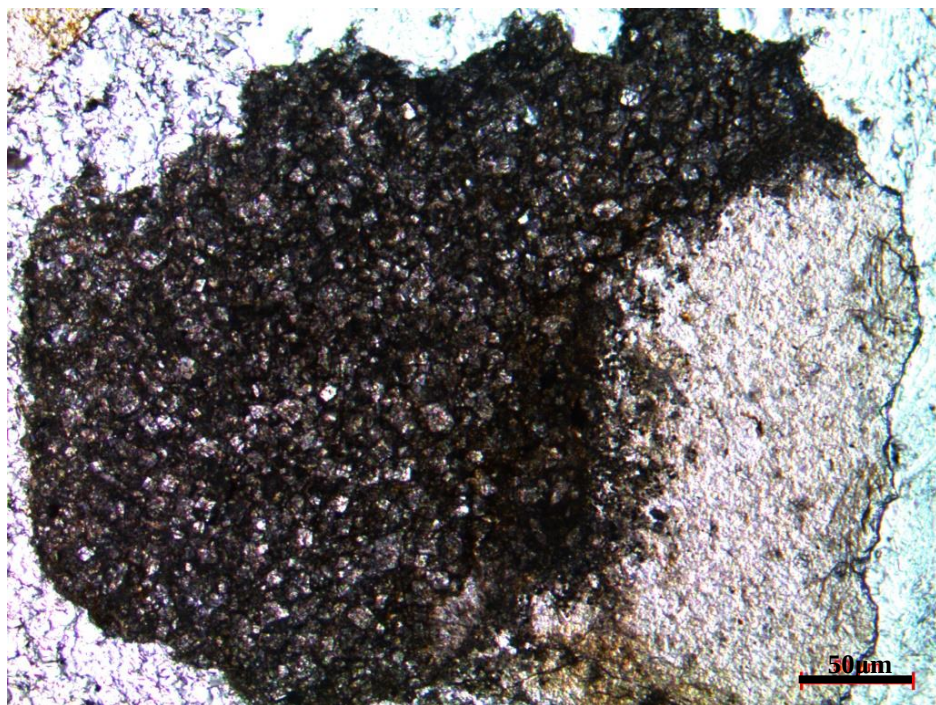
Figure 133. Silica replacement of dolosparite from the thin section at 1866 m of the K-8 well, plane polar light
