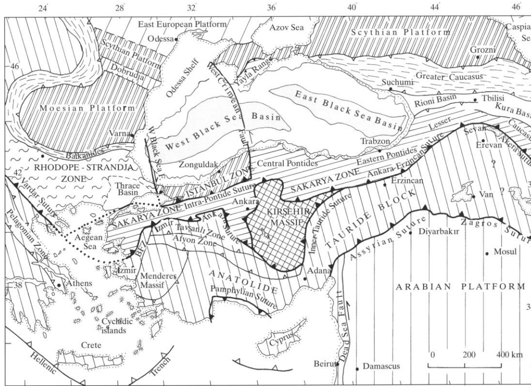
Figure 12. Tectonic map showing the major sutures and continental blocks. Sutures are shown by heavy lines with the polarity of former subduction zones indicated by filled triangles. Heavy lines with open triangles represent active subduction zones. The Late Cretaceous oceanic crust in the Black Sea is shown by grey tones. Small open triangles indicate the vergence of the major fold and thrust belts. BFZ denotes the Bornova Flysch Zone (Okay and Tüysüz (1999))
