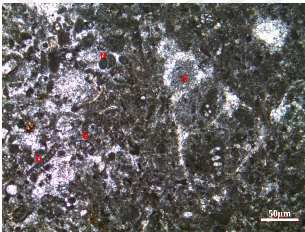
Figure 43. Benthic foraminiferal skeletal peloidal packstone/grainstone microfacies from the thin section at 1777.77 m of the K-11 well (b: benthic foraminifera; s: skeletal fragment (gastrod); p: peloid)
