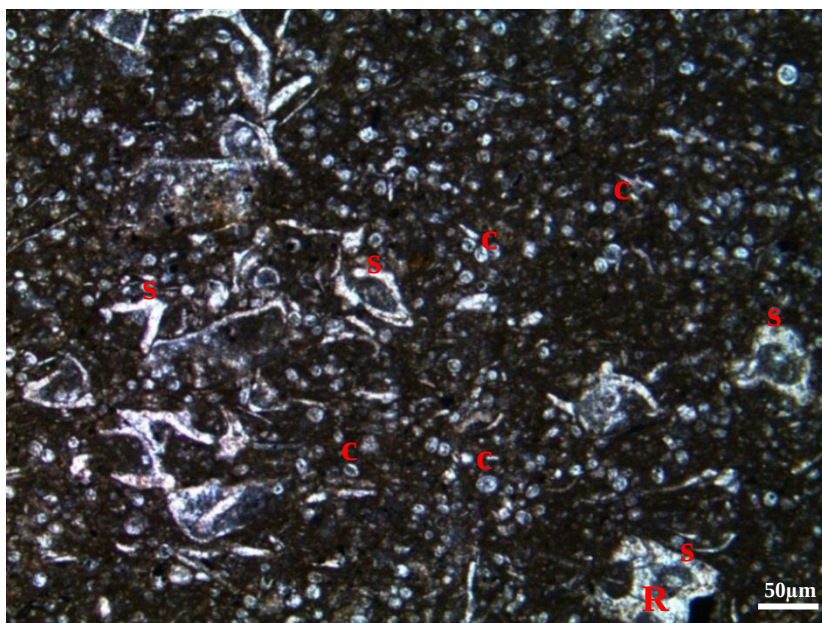
Figure 62. Calcisphaerulid-bearing skeletal wackestone/packstone microfacies from the thin section samples of 1720.21 m of K-11 well (c: calcisphaerulid ( Pithonella spherica ; s: skeletal fragments ( Saccocoma ); R: Recrystallization)
