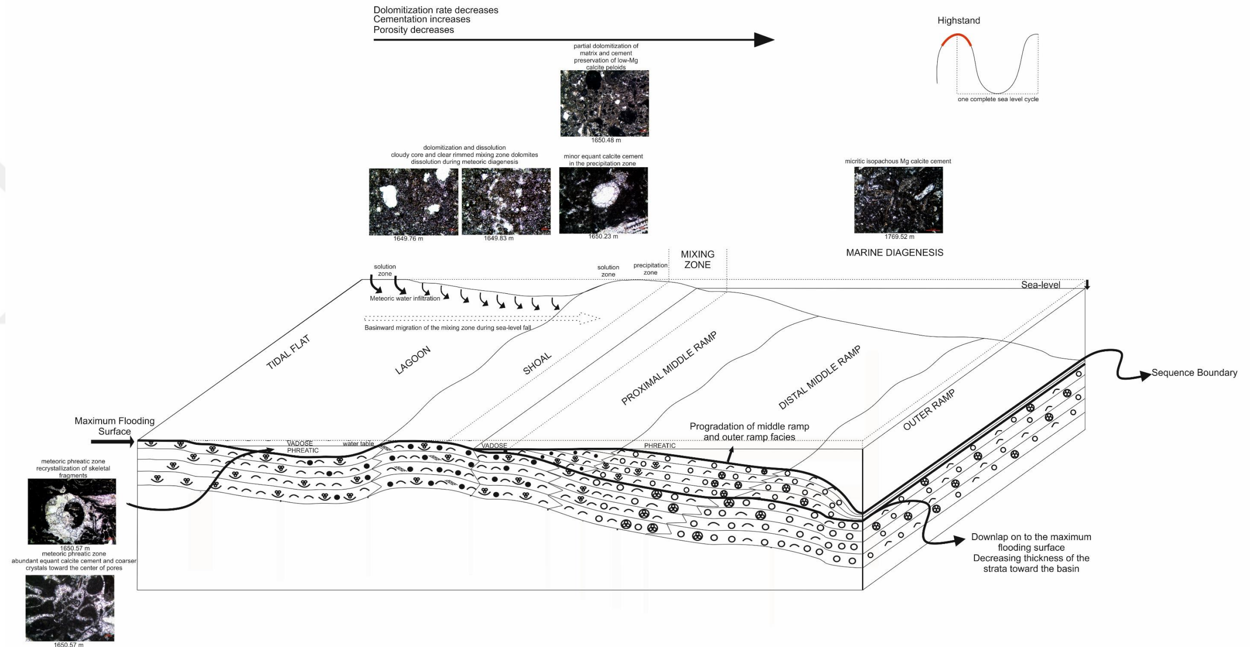
Figure 147. Depositional environments and diagenetic environments on the ramp model of the Derdere Formation during highstand systems tract and relative sea-level fall
