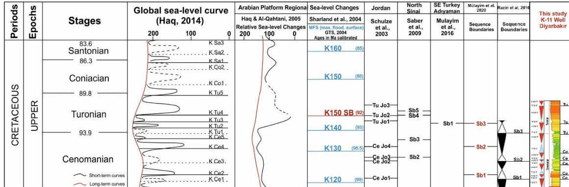
Figure 96. Comparison between the sequence boundaries of the present study with the other Cenomanian-Turonian carbonate platforms in neighbouring areas and with the global eustatic scheme of Haq (2014) (modified from Mülâyim et. al., 2020)
