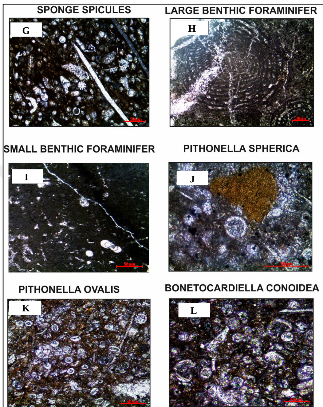
Figure 22. Photomicrographs, which show the primary constituents of the Derdere Formation, are from the samples of K-11 well with the scale of 50 \mu\text{m} .) [Depths of samples are 1721.84 m (G), 1778.04 m (H), 1778.34 m (I), 1721.84 m (J), 1722.82 m (K), and 1725.35 (L).]
