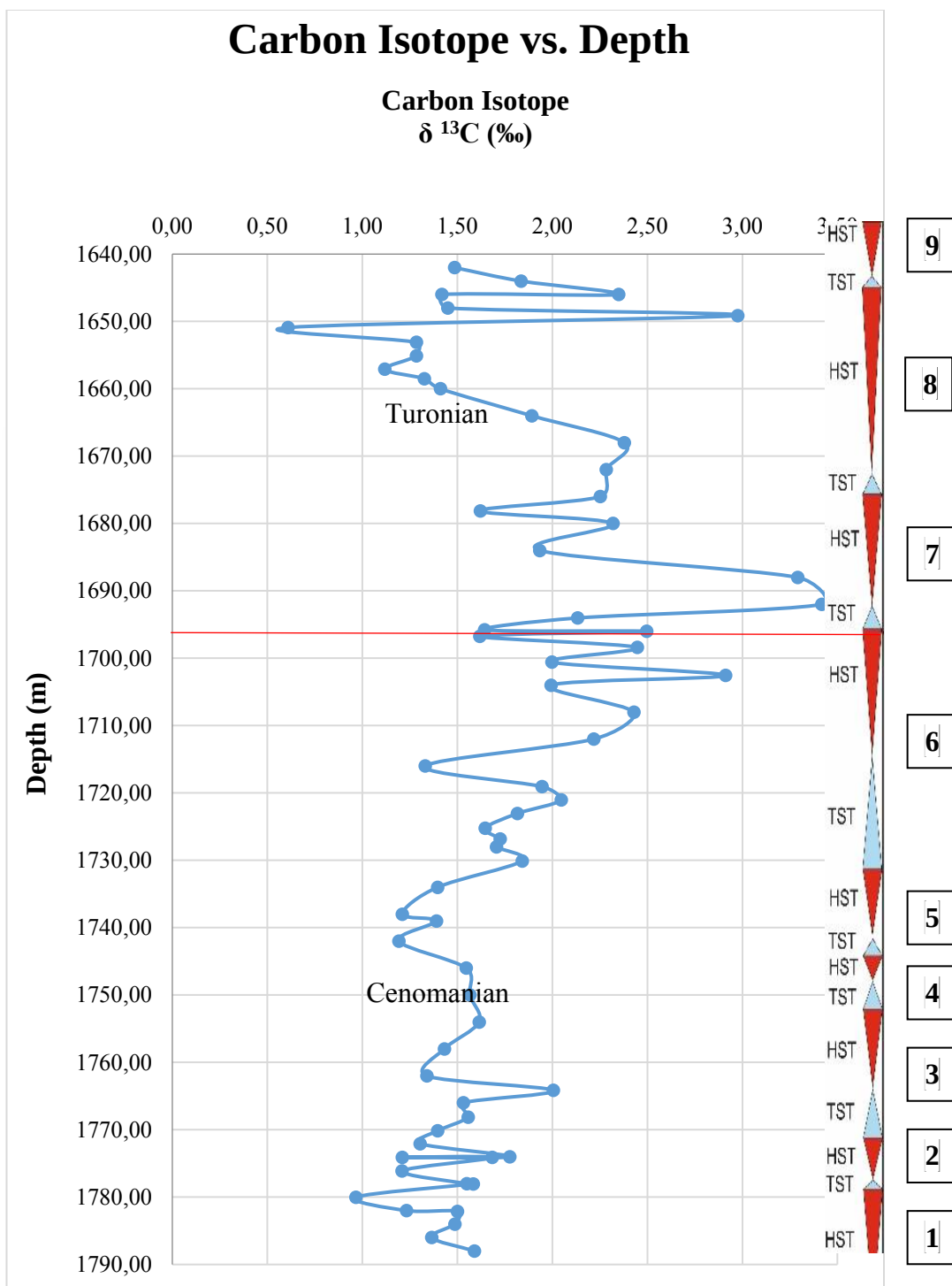
Figure 98. Carbon isotope data vs. depth (m) graph of K-11 well based on the data of Table 8 (Red line shows the C-T boundary)
