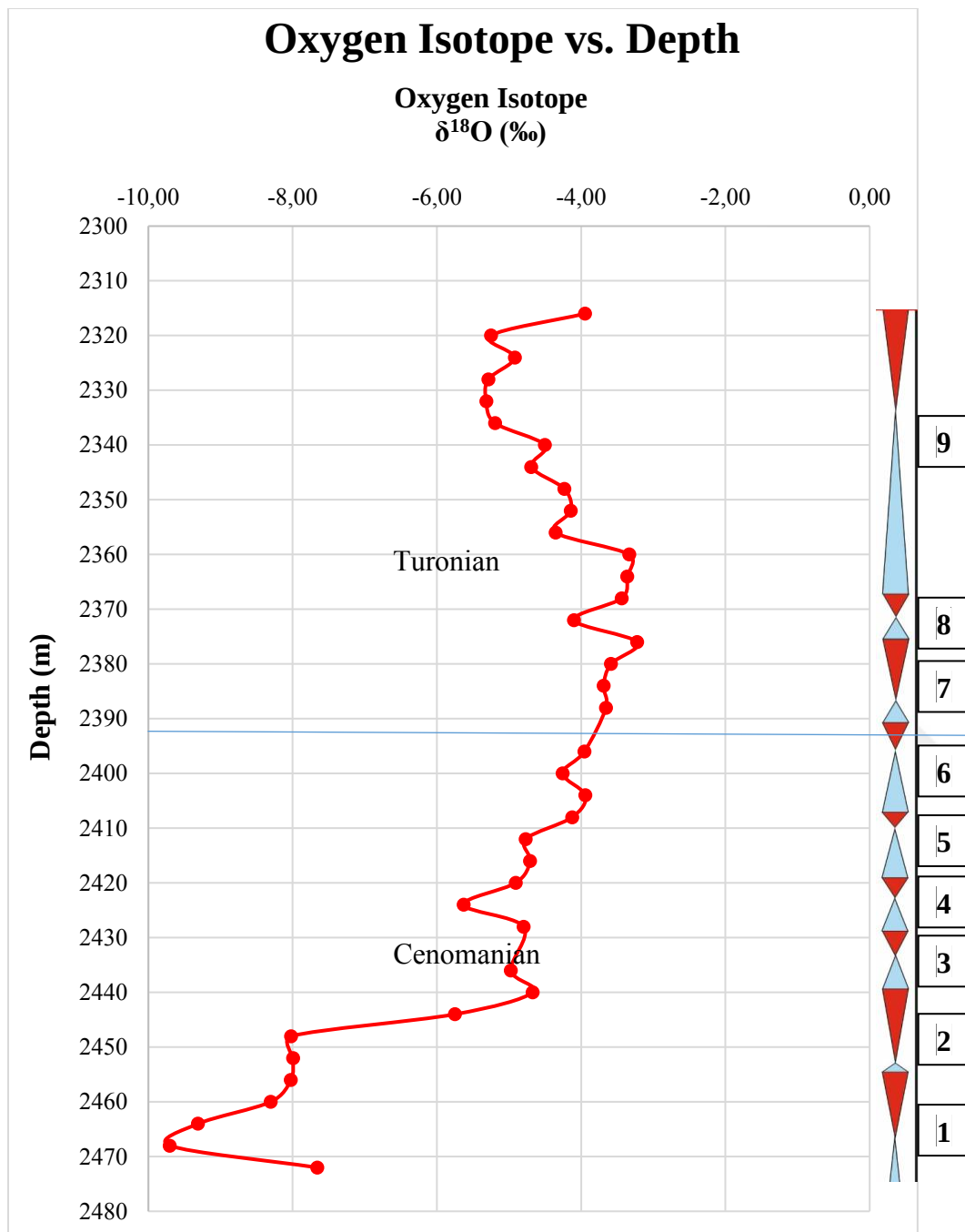
Figure 99. Oxygen isotope data vs. depth (m) graph of K-2 well based on the data of Table 7 (Blue line shows the C-T boundary)
