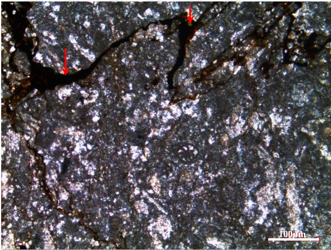
Figure 135. Stylolites filled with organic matter and clay from the thin section at 1769.03 m of the K-11 well
