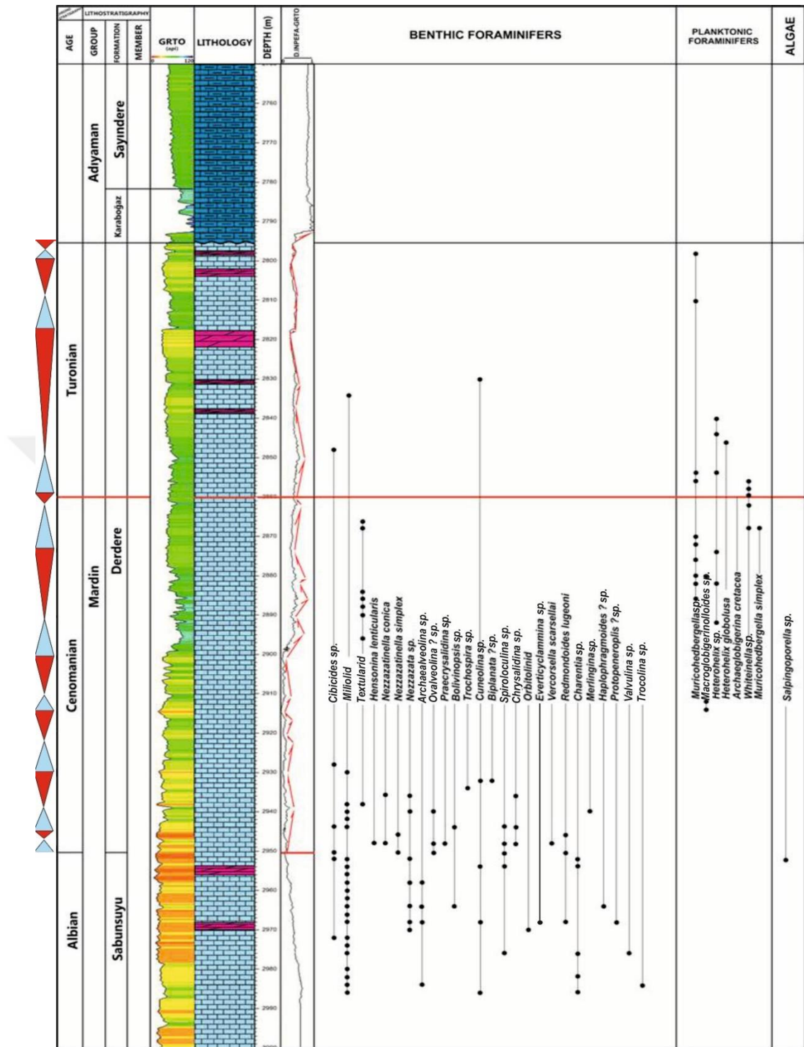
Figure 89. Benthic and planktonic foraminifer assemblage of the Derdere Formation observed in the K-7 well (Red line shows the Cenomanian-Turonian boundary.)
