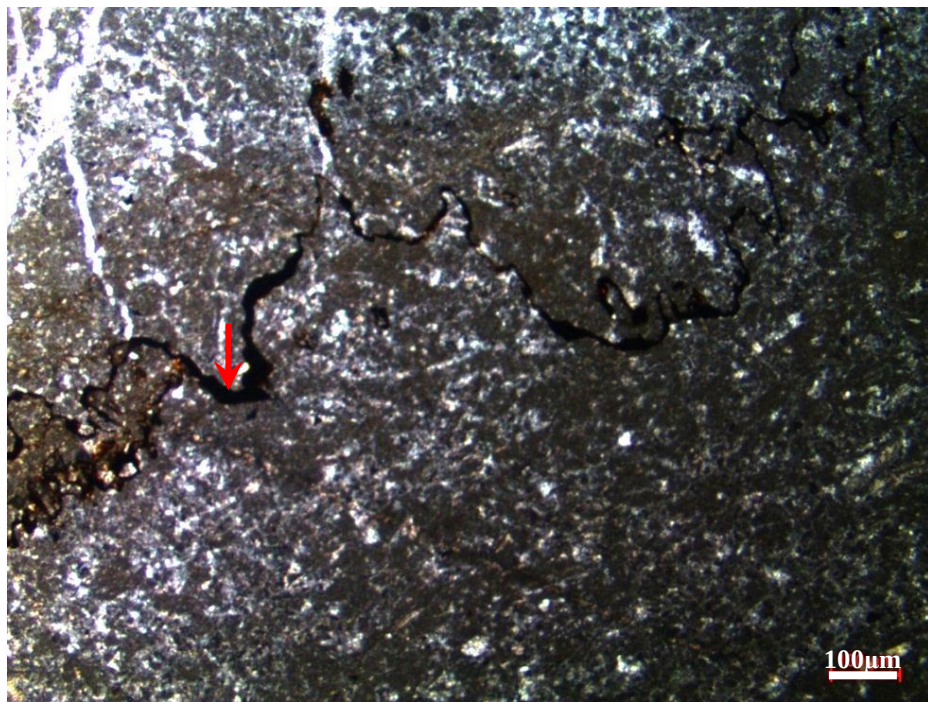
Figure 136. Stylolites filled with organic matter and clay from the thin section at 1765.40 m of the K-11 well
