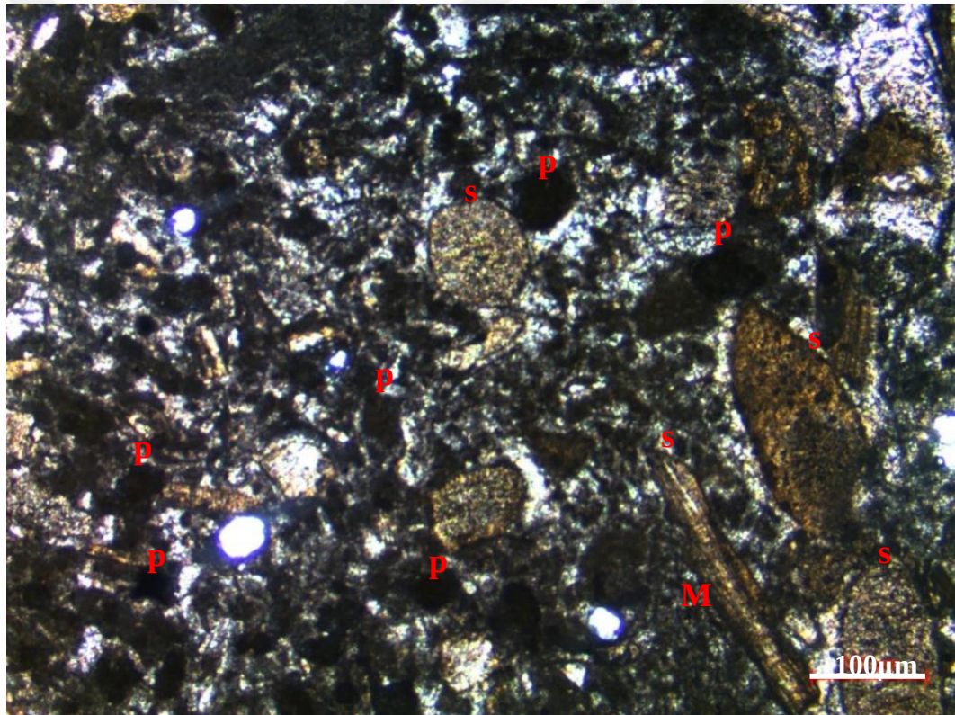
Figure 47. Skeletal peloidal packstone to grainstone microfacies from the thin section at 1773.35 m of the K-11 well (s: skeletal fragments; p: peloid; M: micritic envelope)
