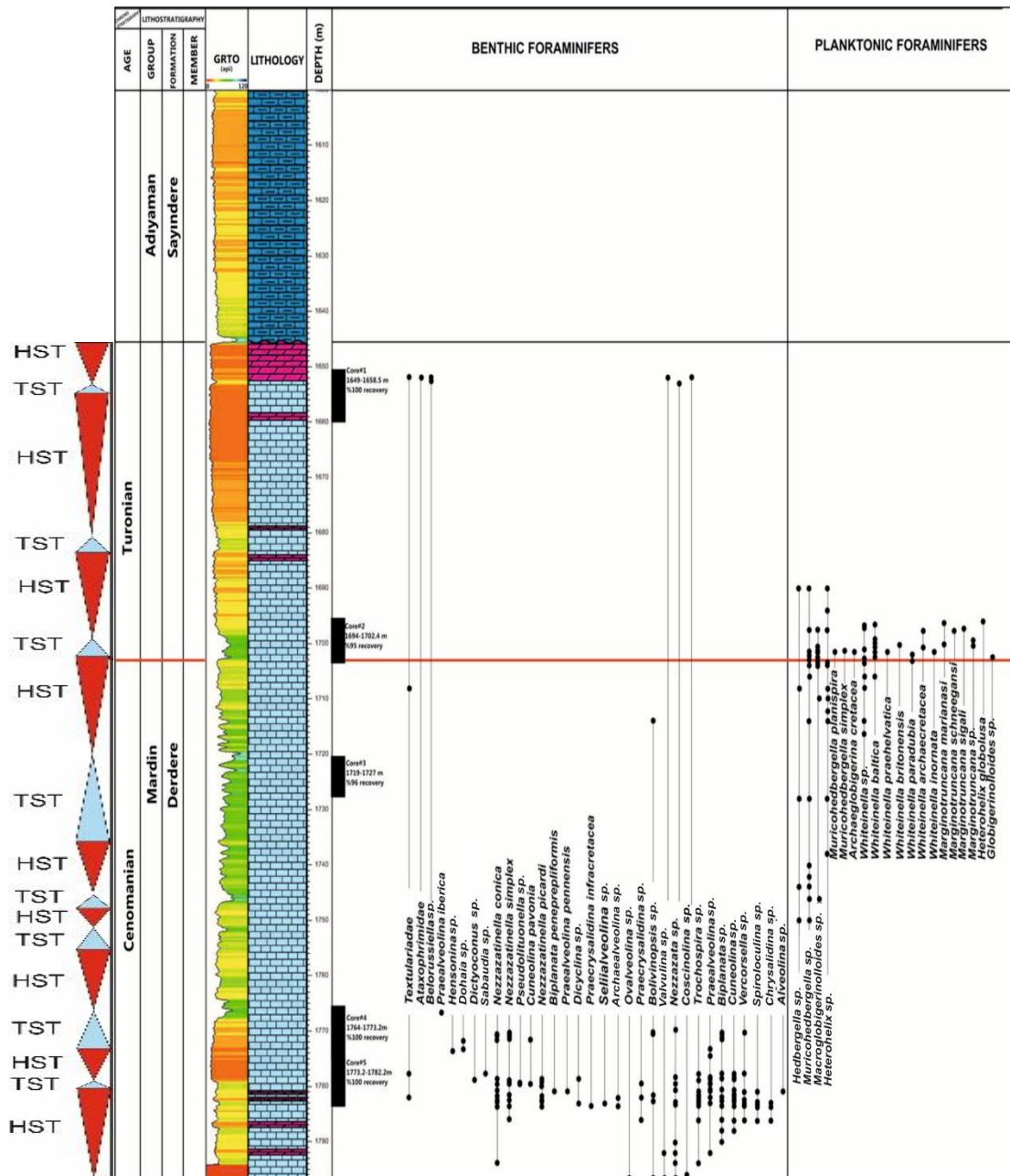
Figure 88. Benthic and planktonic foraminifer assemblage of the Derdere Formation observed in the K-11 well (Red line shows the Cenomanian-Turonian boundary.)
