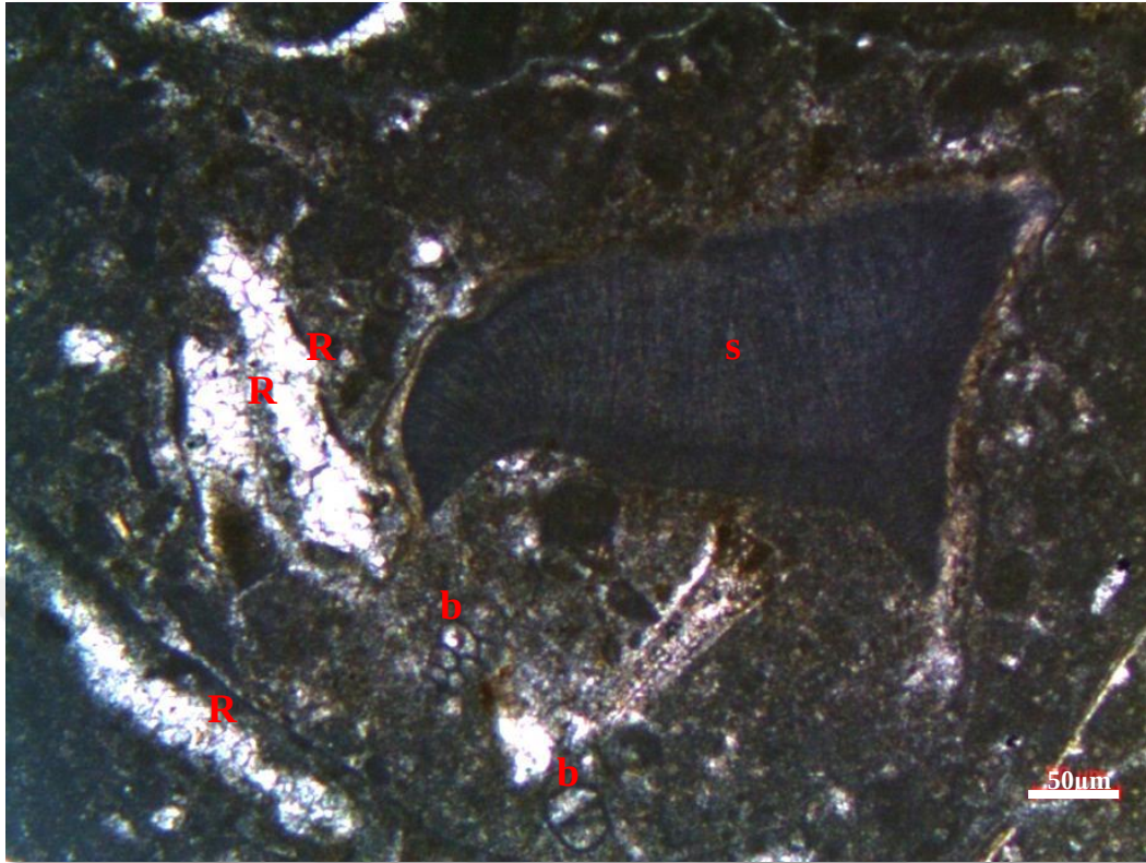
Figure 42. Benthic foraminiferal skeletal mudstone to wackestone microfacies from the thin section at 1651.07 m of K-11 well (b: benthic foraminifera; s: undefined skeletal fragment; R: recrystallization of the soft parts of the skeletal fragments)
