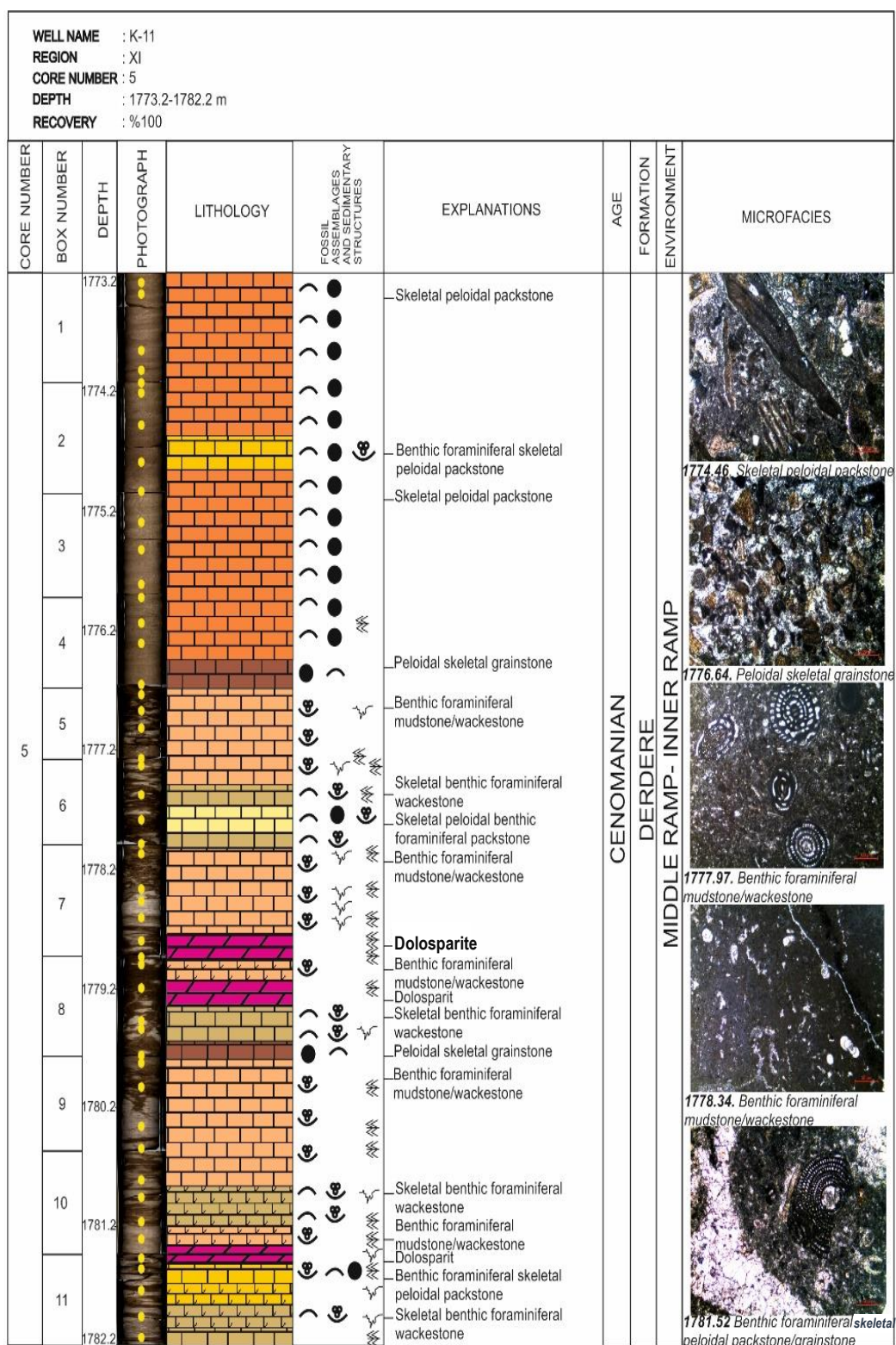
Figure 30. Sedimentological log of Core#5 of the K-11 well, 1773.2-1782.2 m, the Derdere Formation with %100 recovery
