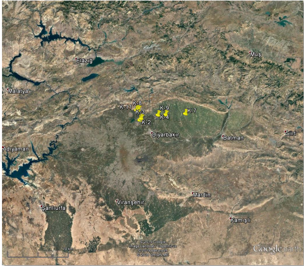
Figure 2. Locations of the studied wells from west to east K-11, K-8, K-2, K-3, K-9, K-4 and K-7 are plotted on Google Earth image.
