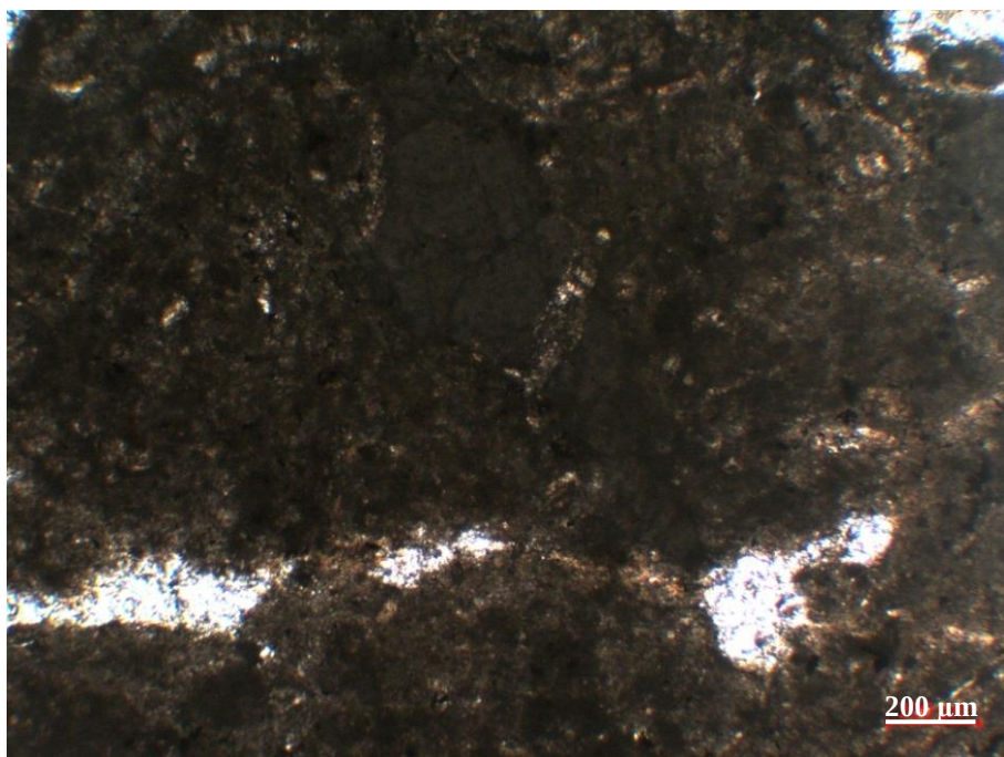
Figure 5. Plane polarized light microscopy photomicrograph of peloidal facies and fracture of K-2 well
