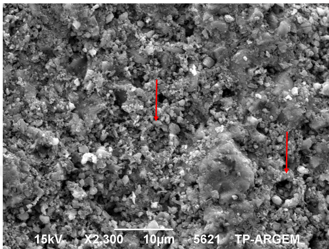
Figure 75. Possible calcareous nannofossils (indicated with red arrows) are shown on the SEM photomicrograph. Thin section is from 1699.21 m
