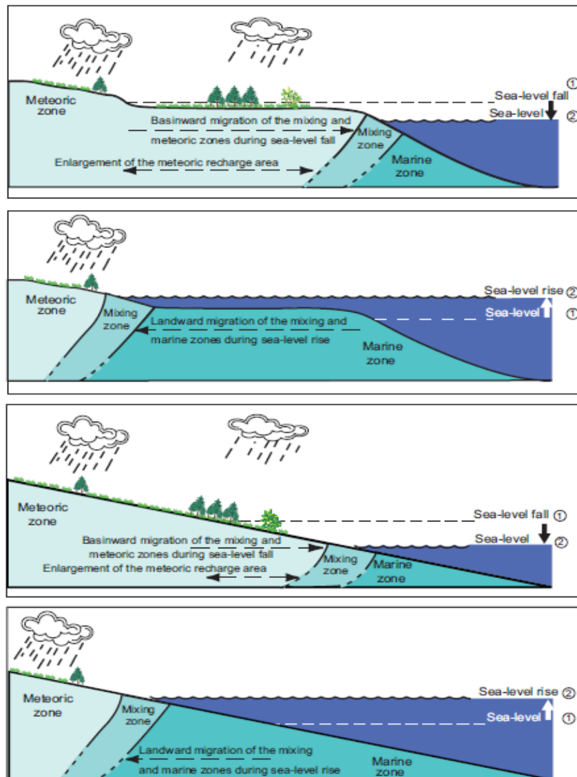
Figure 116. Change in the meteoric, mixing and marine phreatic zones in platforms and ramps during relative sea level rise and fall. Large area is affected in platforms rather than homoclinal ramps (Morad et. al., 2012)
