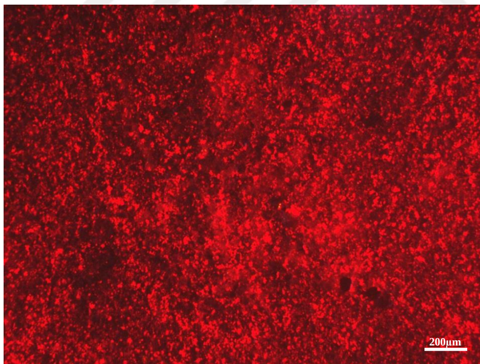
Figure 114. Dolomicrosparite and pore spaces of K-11 well, plane polar light
