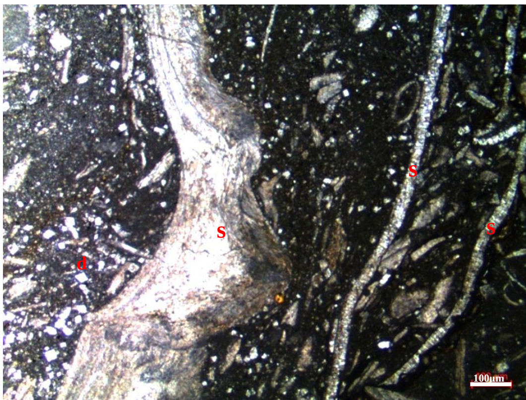
Figure 53. Skeletal wackestone microfacies from the thin section at 1764.54 m of the K-11 well (s: skeletal fragments (brachiopod); d: dolomite crystal)
