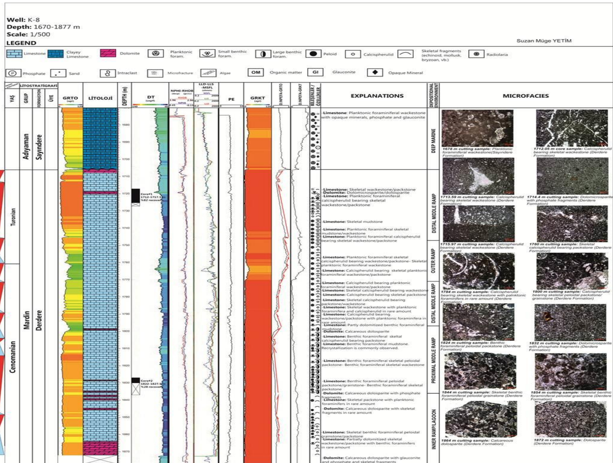
Figure 87. Sedimentological log and sequences of the Derdere Formation in the K-8 well (1670-1877m)
