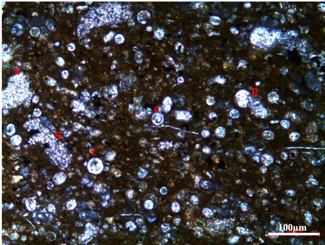
Figure 76. Planktonic foraminiferal skeletal calcisphaerulid-bearing wackestone to packstone microfacies from the thin section at 1722.96 m of the K-11 well (p: planktonic foraminifer; s: skeletal fragment (echinoderm); c: calcisphaerulid ( Pithonella spherica ))
