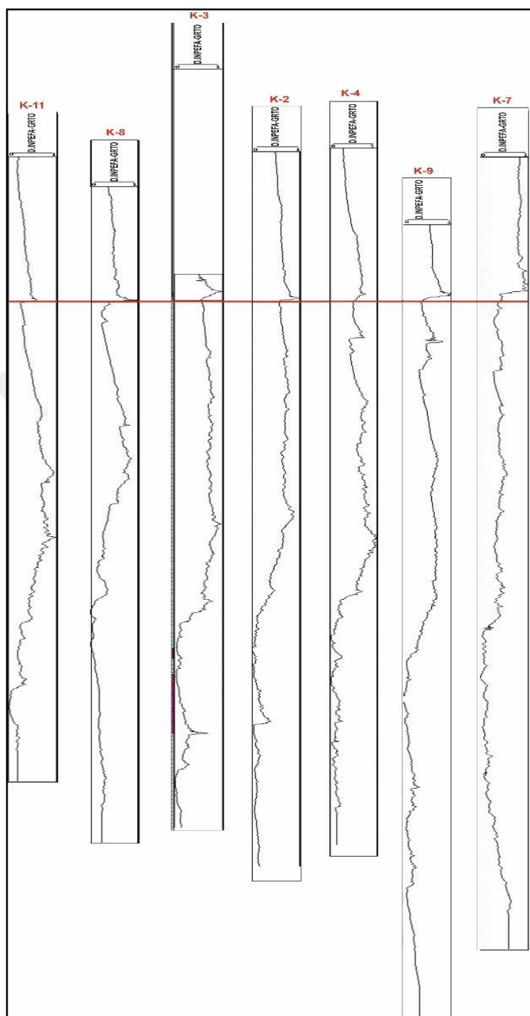
Figure 84. From west to east INPEFA log responses without interpretation (K-11, K-8, K-3, K-2, K-4, K-9, and K-7) (Red line shows the boundary between Derdere and Sayindere formations.)
