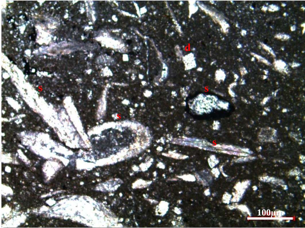
Figure 54. Skeletal wackestone microfacies from the thin section at 1764.57 m of the K-11 well [s: skeletal fragments (possible “ Saccocoma ”); d: dolomite crystal]
