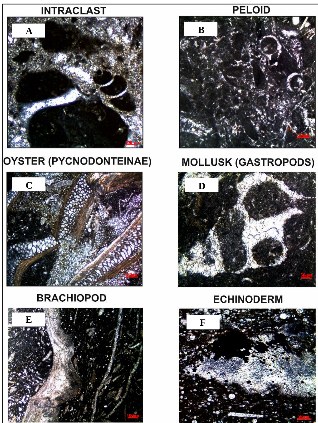
Figure 21. Photomicrographs, which show the primary constituents of the Derdere Formation, are from the samples of K-11 well with the scale of 50 \mu\text{m} (on the right) and 100 \mu\text{m} (on the left). [Depths of samples are 1649.35 m (A), 1650.23 m (B), 1650.79 m (C), 1651.07 m (D), 1764.54 m (E), and 1722.82 (F).]
