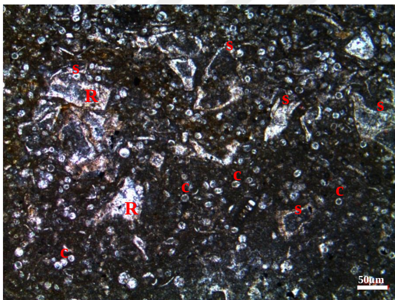
Figure 63. Calcisphaerulid-bearing skeletal wackestone to packstone microfacies from the thin section at 1720.27 m of the K-11 well [c: calcisphaerulid ( Pithonella spherica ); s: skeletal fragments ( Saccocoma ); R: recrystallization]
