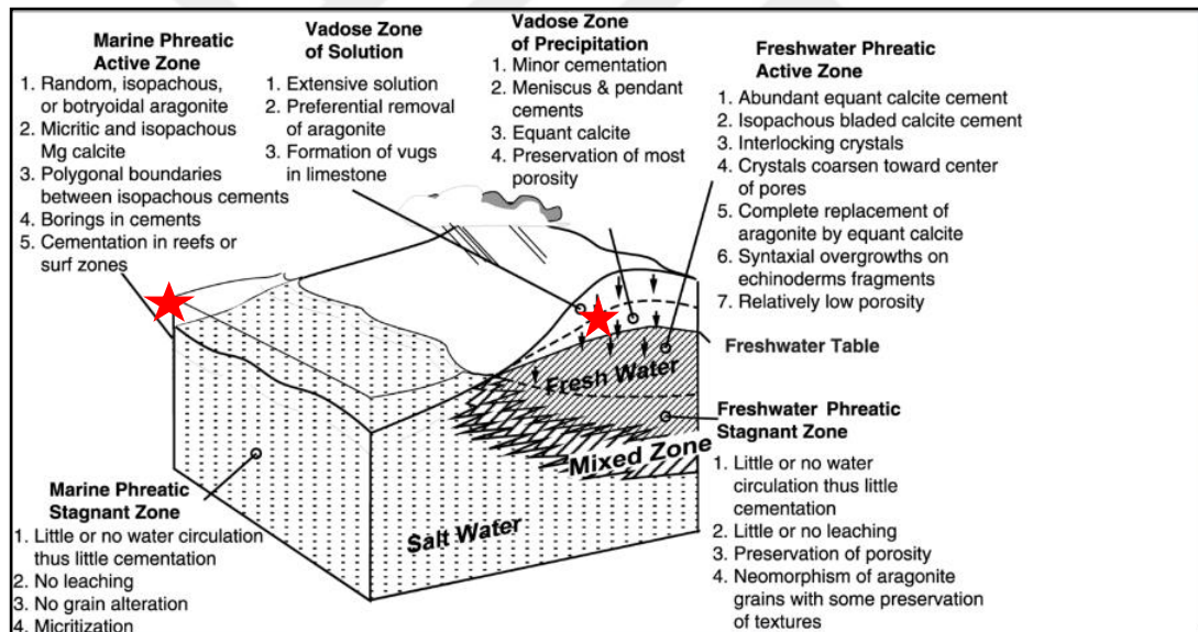
Figure 141. Common carbonate cements and diagenetic features formed in different diagenetic environments (Longman, 1980) (Red stars show the diagenetic environments of the Derdere Formation)
