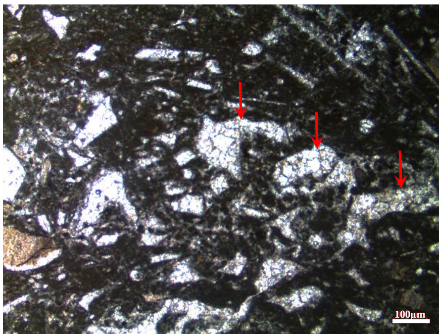
Figure 123. Sparry calcite cement formed as a result of neomorphism inside the skeletal fragments from the thin section at 1765.16m of the K-11 well
