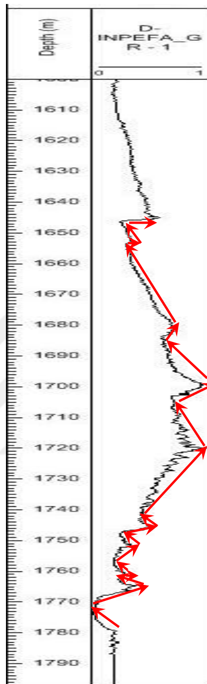
Figure 10. INPEFA log curves of K-11 pilot well on which going through lowest “zero” value shows shoaling trend and going through highest “one” value shows deepening trend. Red arrows show negative INPEFA trend which is shoaling and positive INPEFA trend which is deepening.
