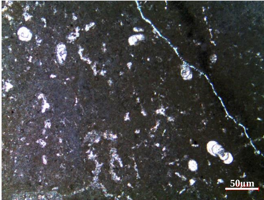
Figure 39. Fenestral fabric in benthic foraminiferal mudstone of the peritidal environment of inner ramp setting at 1778.45 m of the K-11 well
