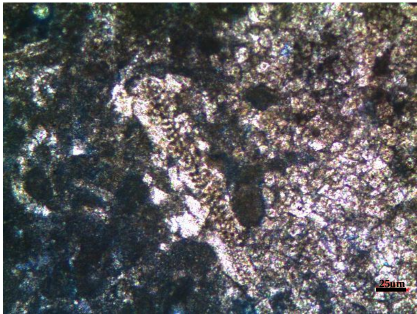
Figure 105. Partially dolomitized benthic foraminiferal, skeletal, peloidal packstone to grainstone microfacies from the thin section at 1650.23 m of the K-11 well (Note that original fabric of the peloidal facies is partly preserved.)
