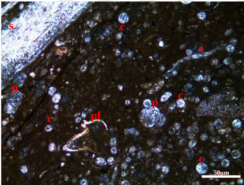
Figure 61. Skeletal planktonic foraminiferal calcisphaerulid-bearing wackestone to packstone microfacies from the thin section at 1721.16 m of the K-11 well (pf: phosphate fragment; s: skeletal fragments; p: planktonic foraminifers; c: calcisphaerulids ( Pithonella spherica ))
