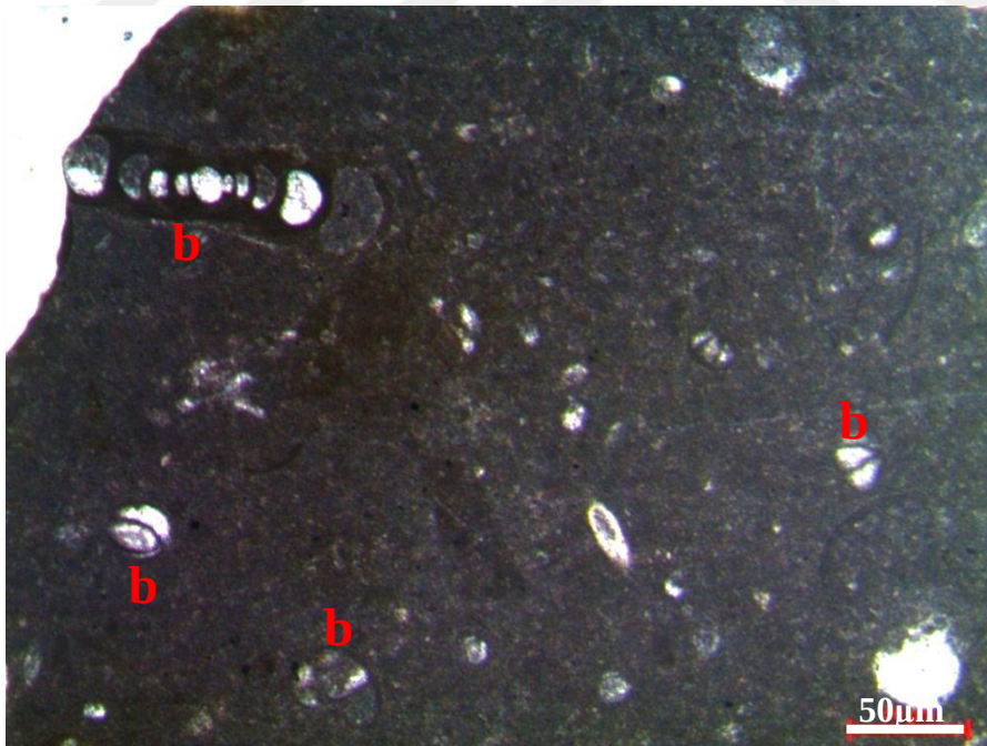
Figure 36. Benthic foraminiferal mudstone microfacies from the thin section at 1786 m of K-11 the well (b: benthic foraminifera)
