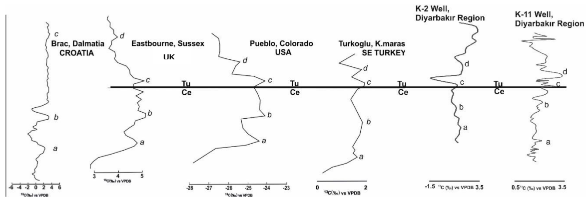
Figure 101. Correlation of C-isotope curve of K-2 and K-11 wells with the curves of Türkoğlu section, the Cenomanian-Turonian time of Eastbourne and Pueblo reference sections and Brac succession (modified from Mülâyim et. al., 2019)
