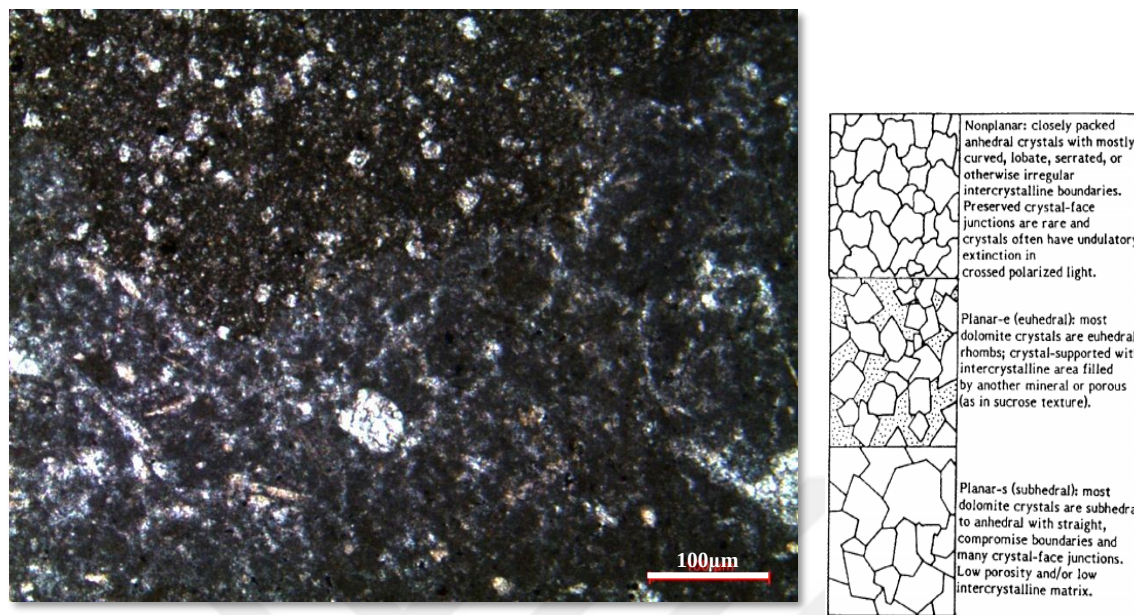
Figure 106. Planar-e dolomite with unreplaced peloids, recrystallized skeletal fragments and matrix microfacies from the thin section at 1764.67 m of the K-11 well [(Note that original fabric of the peloidal facies is preserved.) (Dolomite rock texture classification of Gregg and Sibley (1984) is on the right).]
