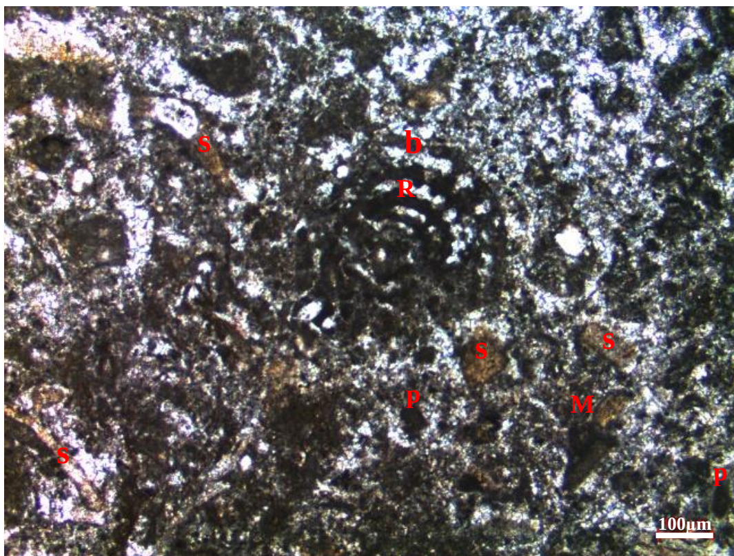
Figure 46. Benthic foraminiferal skeletal peloidal packstone/grainstone microfacies from the thin section at 1771.01 m of the K-11 well (b: benthic foraminifera; s: skeletal fragment; p: peloid; R: recrystallization of the soft parts; M: micritic envelope at around the skeletal fragments)
