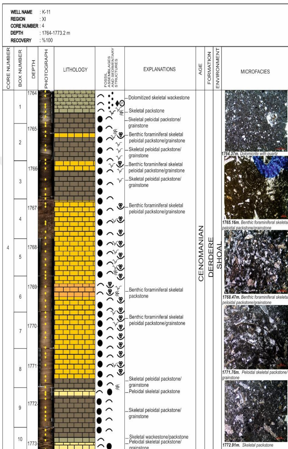
Figure 29. Sedimentological log of Core#4 of the K-11 well, 1764-1773.2 m, the Derdere Formation with %100 recovery
