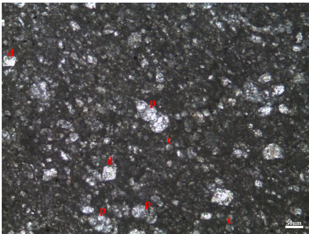
Figure 68. Calcisphaerulid-bearing planktonic foraminiferal mudstone to wackestone microfacies from the thin section at 1696.75 m of the K-11 well [c: calcisphaerulid ( Pithonella spherica ); p: planktonic foraminifer; d: dolomite]
