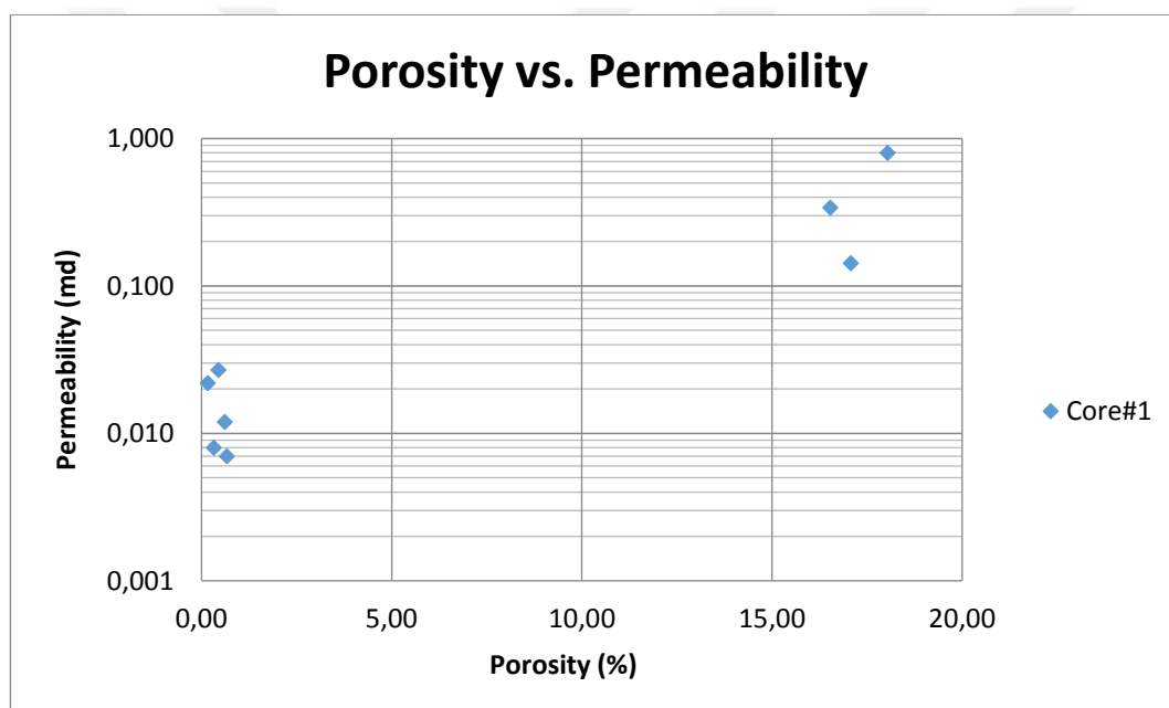
Figure 146. Porosity vs. Permeability Graph of Cores of the K-9 well
