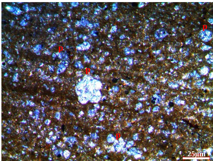
Figure 71. Planktonic foraminiferal wackestone microfacies from the thin section at 1704 m of the K-11 well (p: planktonic foraminifer)
