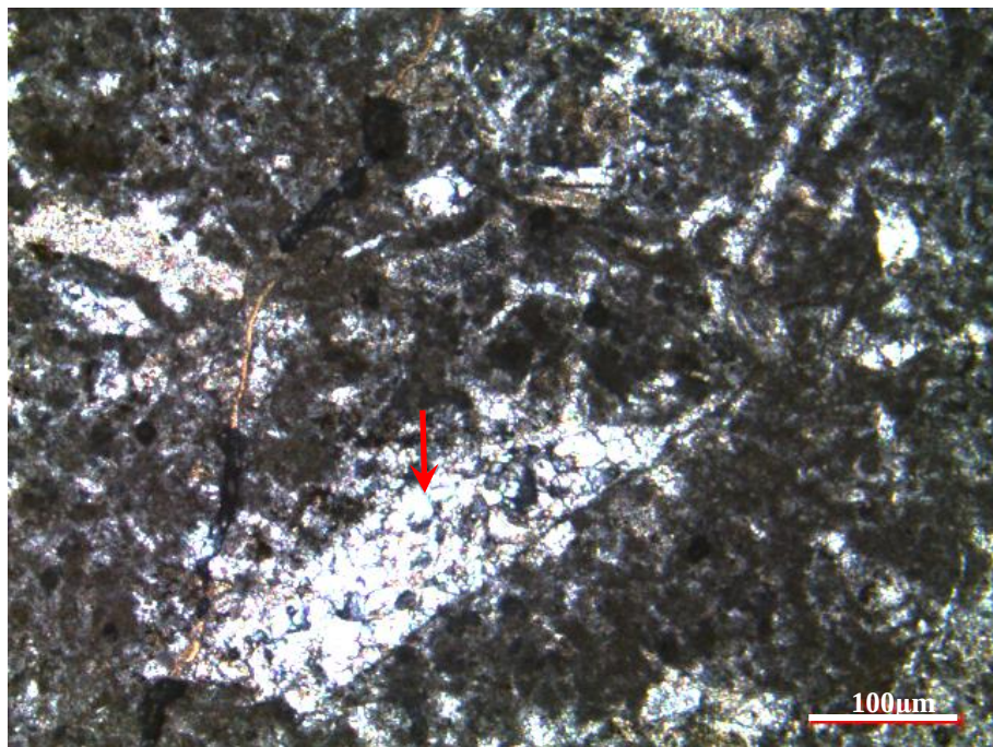
Figure 124. Sparry calcite cement formed as a result of neomorphism inside the skeletal fragments from the thin section at 1765.78 m of the K-11 well
