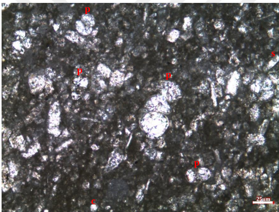
Figure 55. Skeletal calcisphaerulid-bearing planktonic foraminiferal wackestone/packstone microfacies from the thin section at 1694.55 m of the K-11 well (s: skeletal fragments; c: calcisphaerulid ( Pithonella spherica ); p: planktonic foraminifer)
