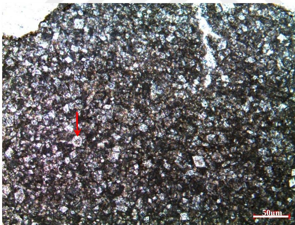
Figure 109. Calcareous dolosparite from the thin section at 1866 m of the K-8 well (Note that original fabric including calcisphaerulids is partially preserved.)
