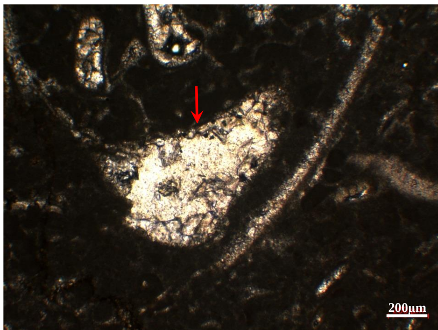
Figure 127. Isopachous bladed calcite cement inside the pore space of the skeletal fragments from the thin section at 1650.69 m of the K-11 well
