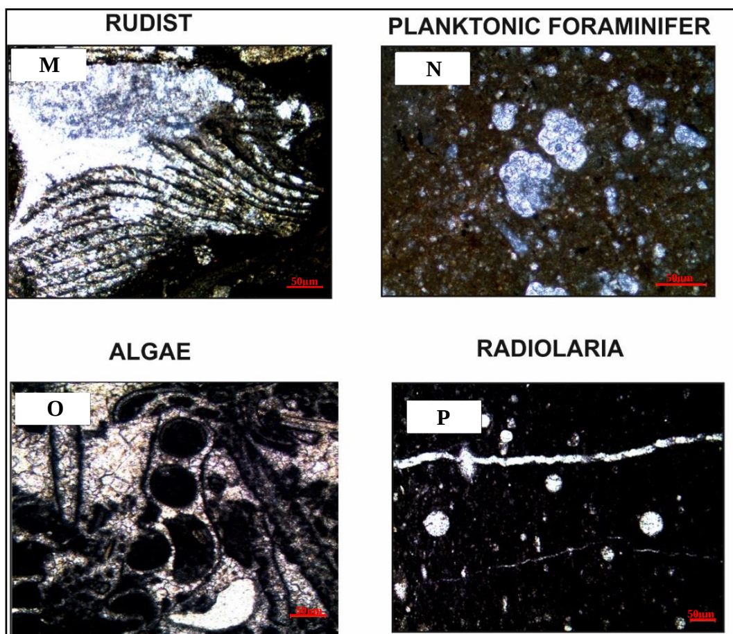
Figure 23. Photomicrographs, which show the primary constituents of the Derdere Formation, are from the samples of K-11 well with the scale of 50 \mu\text{m} .) [Depths of samples are 1781.69 m (M), 1700.03 m (N), 1650.57 m (O) and 1697.42 m (P).]
