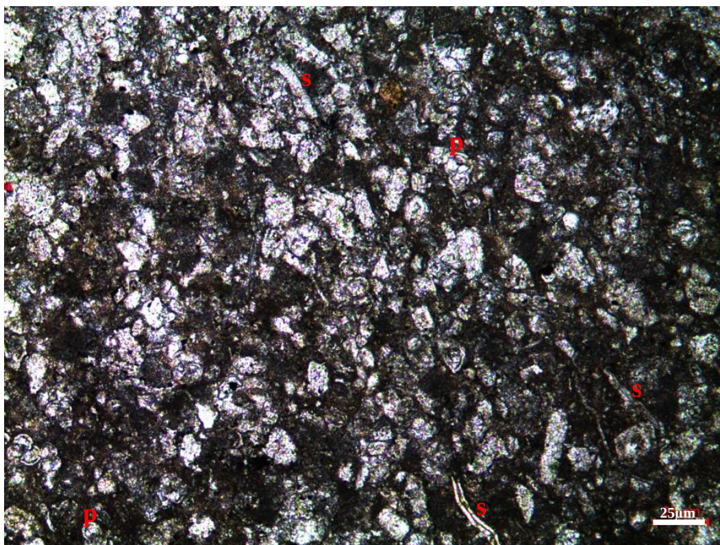
Figure 58. Skeletal calcisphaerulid-bearing planktonic foraminiferal wackestone to packstone microfacies from the thin section at 1695.09 m of the K-11 Well (s: skeletal fragment (broken pelecypod due to compaction); p: planktonic foraminifer)
