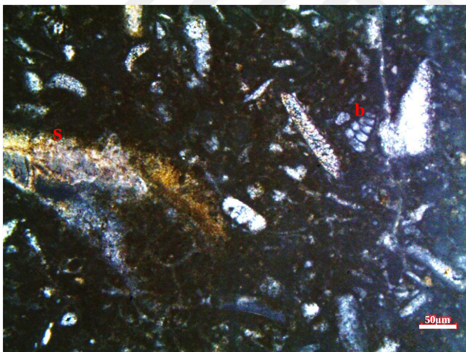
Figure 41. Benthic foraminiferal skeletal mudstone to wackestone microfacies from the thin section at 1650.85 m of the K-11 well [b: benthic foraminifera; s: diagenetically altered skeletal fragment (oyster)]
