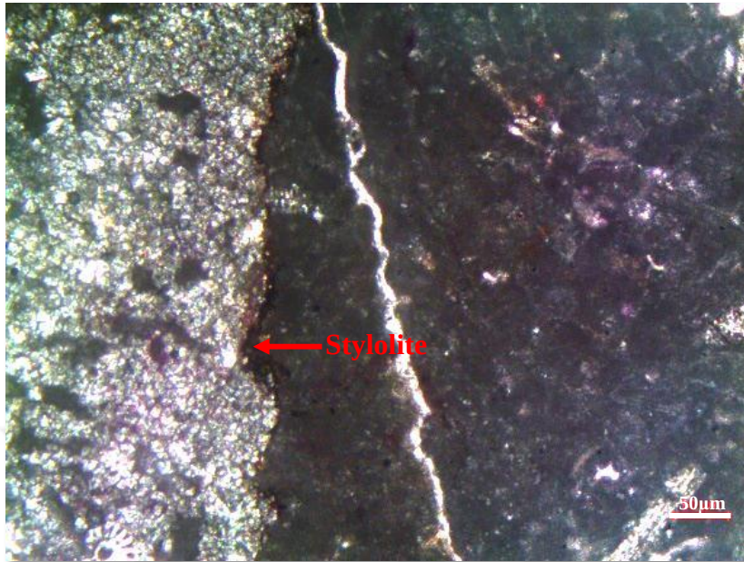
Figure 104. Partially dolomitized skeletal, peloidal packstone to grainstone microfacies from the thin section at 1650.11 m of the K-11 well (Note that original fabric of the peloidal facies is partly preserved and Stylolite enhances dolomitization.)
