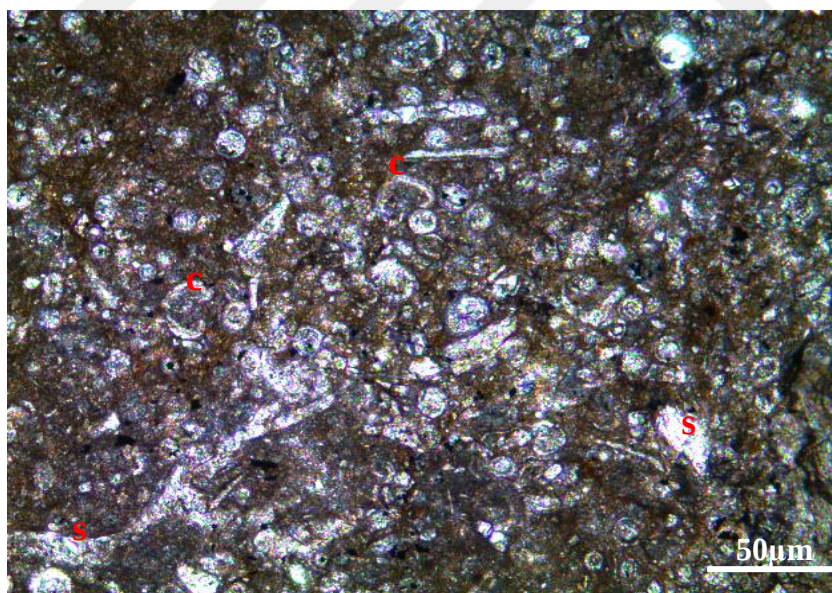
Figure 79. Skeletal calcisphaerulid-bearing wackestone to packstone microfacies from the thin section at 1719.91 m of the K-11 well [pf: phosphate fragments; s: skeletal fragments (thin walled mollusk (pelecypod)); c: calcisphaerulids ( Pithonella spherica )]
