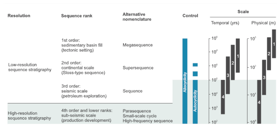
Figure 83. Classification of stratigraphic sequences including temporal and physical scales compiled from the study of Vail et. al. (1977), Vail (1991), Williams (1988) Van Wagoner et. al. (1990) Carter et. al. (1991), Einsele et. al. (1991), Reid and Dorobek (1993), Duval et. al. (1998), Lehrmann and Goldhammer (1999), Schkager (2004, 2010), Miall (2010), Catuneanu (2019)
