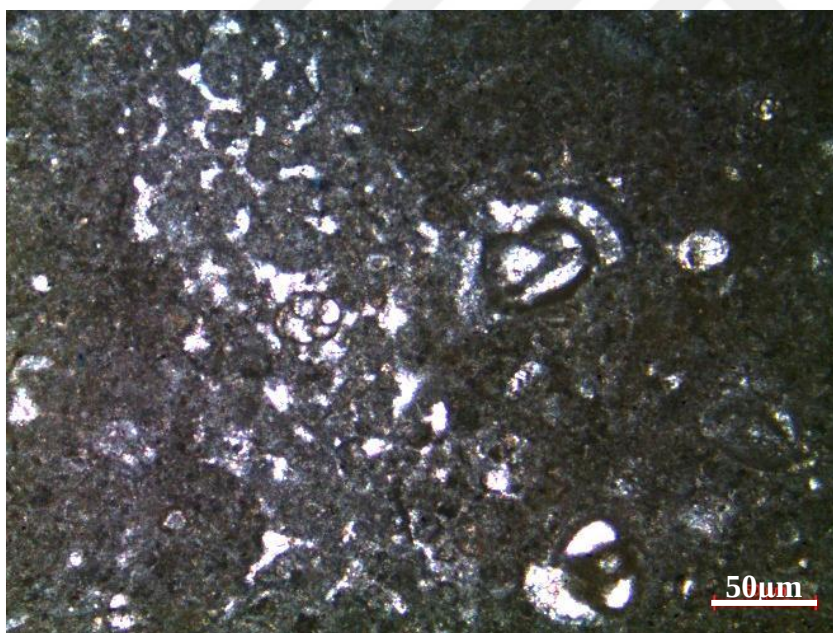
Figure 38. Fenestral fabric in benthic foraminiferal mudstone of peritidal environment of inner ramp setting at 1780.79 m of the K-11 well
