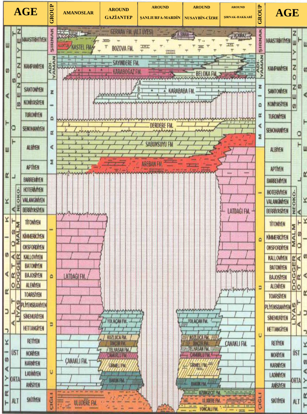
Figure 17. Stratigraphy and correlation of Mesozoic aged autochthonous units at the southern part of Southeastern Turkey (modified after Yılmaz and Duran, 1997)
