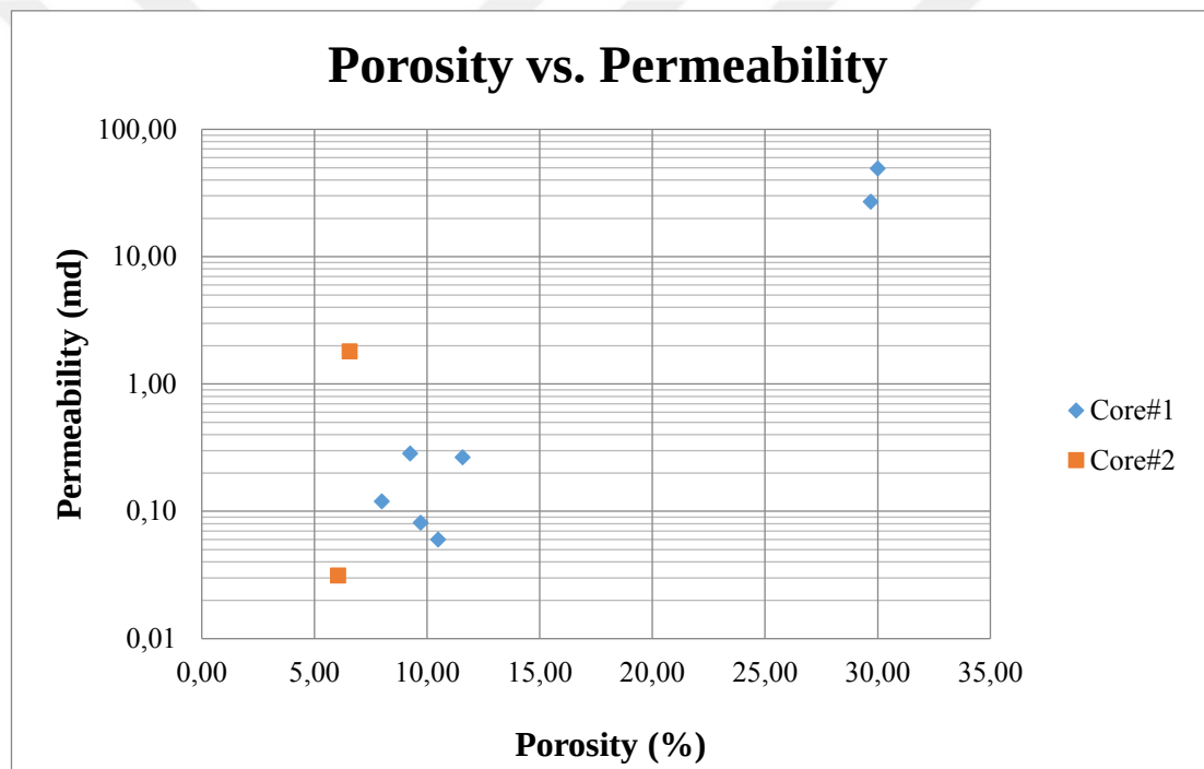
Figure 145. Porosity vs. Permeability Graph of the cores of K-8 well
