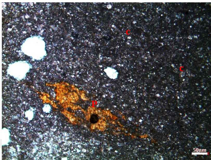
Figure 66. Calcisphaerulid-bearing planktonic foraminiferal mudstone to wackestone microfacies from the thin section at 1697.20 m of the K-11 well [c: calcisphaerulid ( Pithonella spherica ); P: phosphatization]
