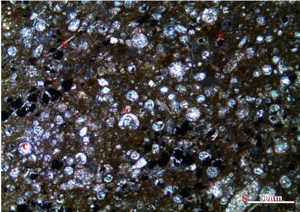
Figure 81. Skeletal calcisphaerulid-bearing wackestone to packstone microfacies from the thin section at 1726.99 m of the K-11 well (s: skeletal fragments; c: calcisphaerulids ( Pithonella spherica and Bonetocardiella conoidea ))
