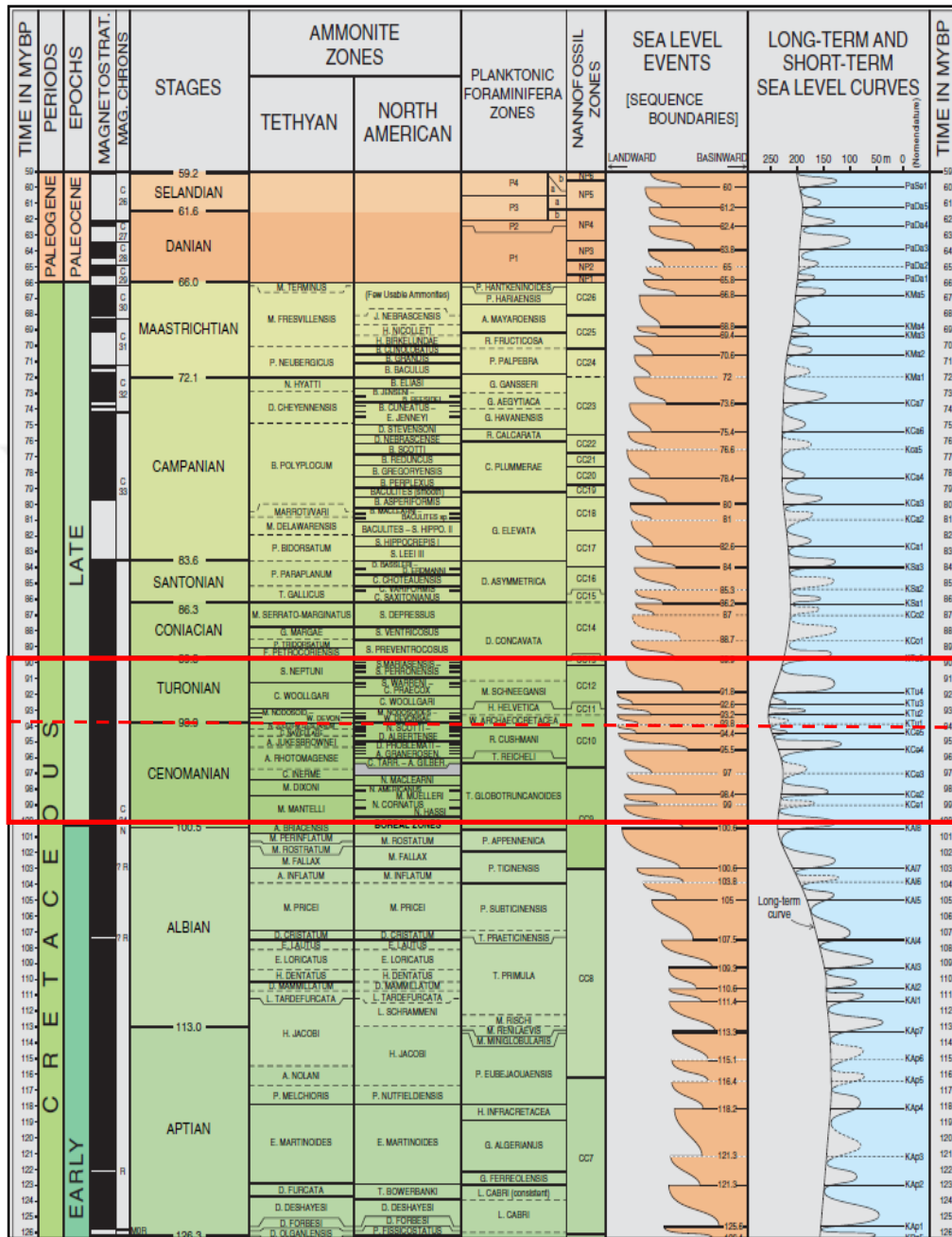
Figure 93. Cretaceous-Paleocene Eustatic Cycle Chart with the correlation of biozones after Hardenbol et al. (1998) and Ogg and Hinnov (2012) (modified after Haq, 2014) (Red rectangle shows the Cenomanian-Turonian time interval and red dotted line shows Cenomanian-Turonian boundary.)
