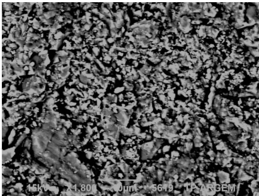
Figure 131. Scanning electron microscope photomicrograph of radiolaria-bearing mudstone microfacies from the thin section of 1697.42 m of K-11 well
