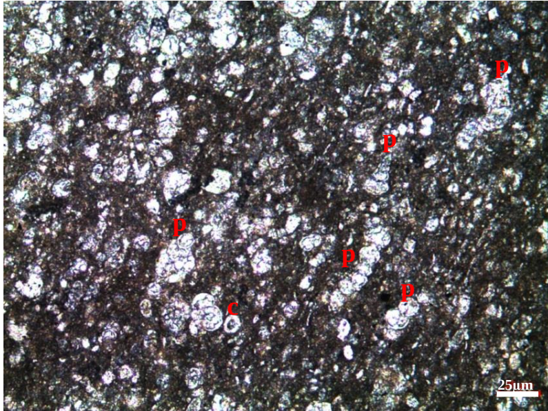
Figure 57. Skeletal calcisphaerulid-bearing planktonic foraminiferal wackestone to packstone microfacies from the thin section at 1695.09 m of the K-11 well (c: calcisphaerulid (partially compacted Pithonella spherica ); p: planktonic foraminifer)
