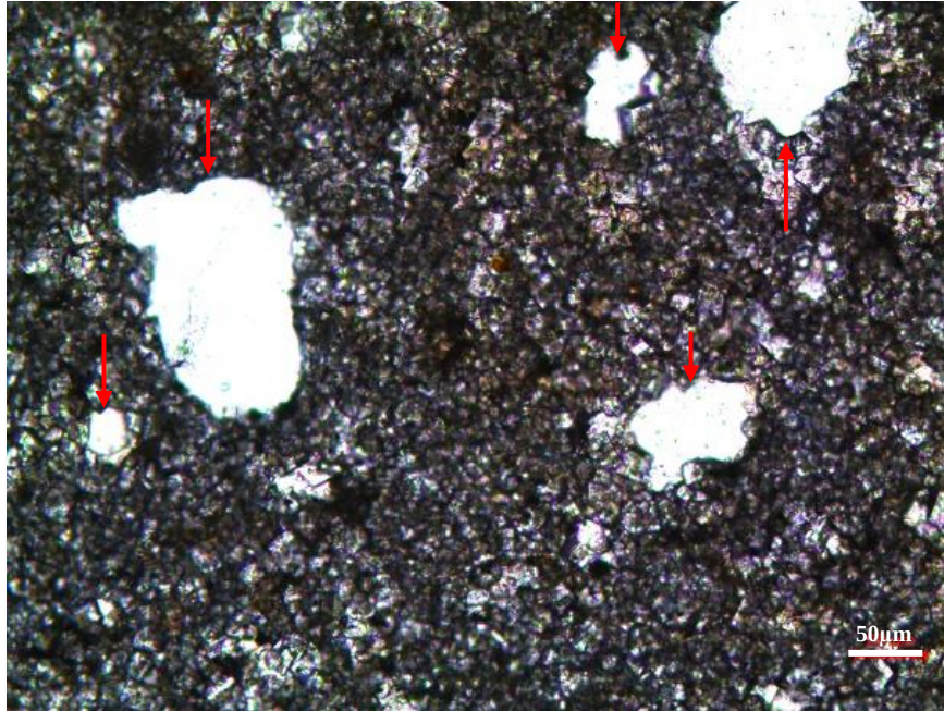
Figure 117. Vuggy porosity in dolomicrosparite formed as a result of dissolution from the thin section at 1649.76 m of the K-11 well (Red arrows show pore spaces.)
