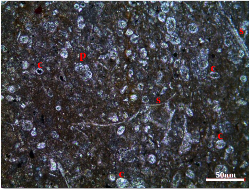
Figure 60. Skeletal planktonic foraminiferal calcisphaerulid-bearing wackestone to packstone microfacies from the thin section at 1721.05 m of the K-11 well [s: skeletal fragments (broken bivalves); p: planktonic foraminifers; c: calcisphaerulids ( Pithonella ovalis )]
