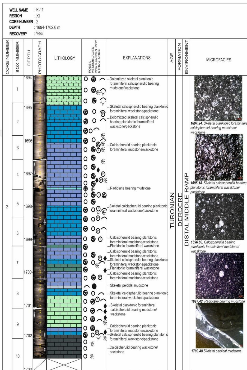
Figure 27. Sedimentological log of Core#2 of the K-11 well, 1694-1702.6 m, the Derdere Formation with %95 recovery
