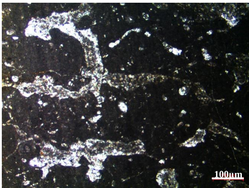
Figure 37. Fenestral fabric in benthic foraminiferal mudstone of the peritidal environment of inner ramp setting at 1779.80 m of the K-11 well
