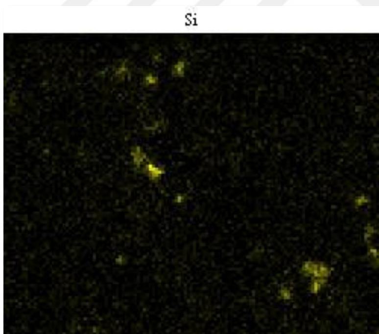
Figure 132. X-ray mapping of silica element shown in Figure 131 (bright yellow areas show the presence of authigenic silica due to its size and anhedral shape)
