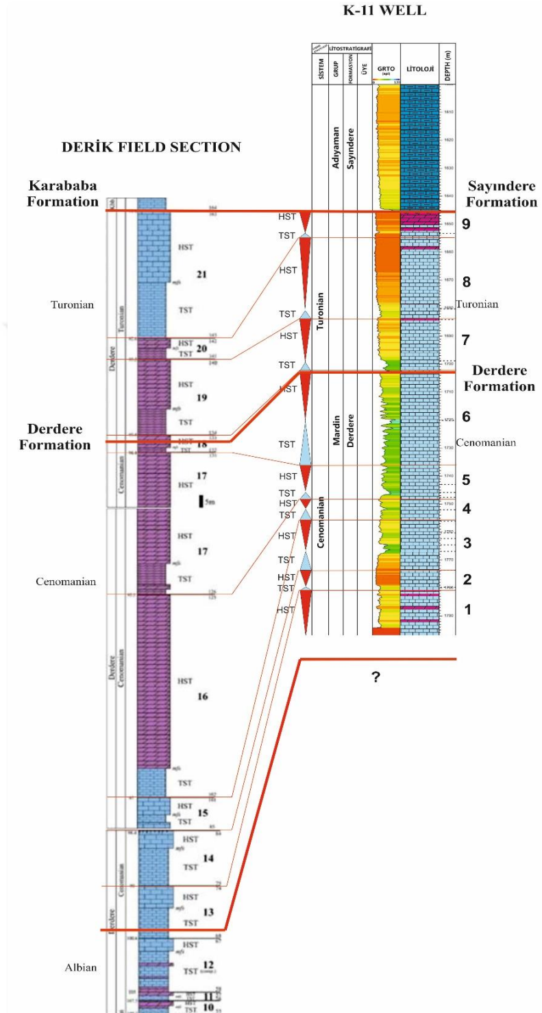
Figure 92. Sequence stratigraphic correlation between the K-11 Well and the Derik field section [Sequences defined in the Derik field section is modified from the study of Özkan and Altınar (2019)]
