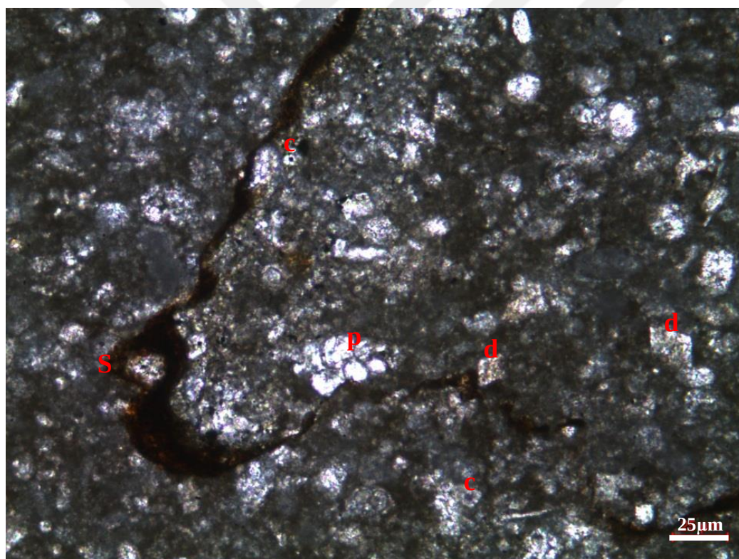
Figure 65. Calcisphaerulid-bearing planktonic foraminiferal mudstone to wackestone microfacies from the thin section at 1694.46 m of the K-11 well [d: dolomite; p: planktonic foraminifer; c: calcisphaerulid ( Pithonella spherica ); S: stylolitization]
