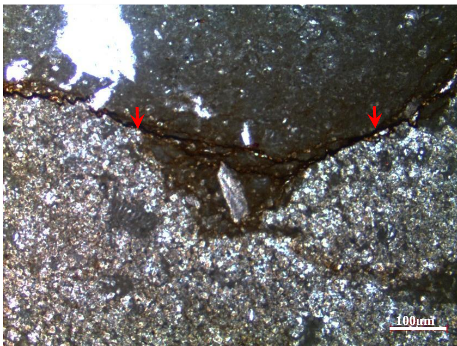
Figure 139. Stylolites associated with dolomitization from the thin section at 1779.53 m of the K-11 well
