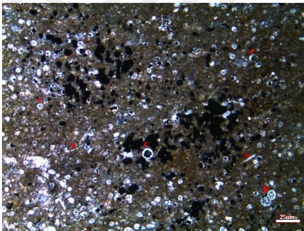
Figure 59. Skeletal planktonic foraminiferal calcisphaerulid-bearing wackestone to packstone microfacies from the thin section at 1719.06 m of the K-11 well [s: skeletal fragments; p: planktonic foraminifers; c: calcisphaerulid ( Pithonella spherica )]
