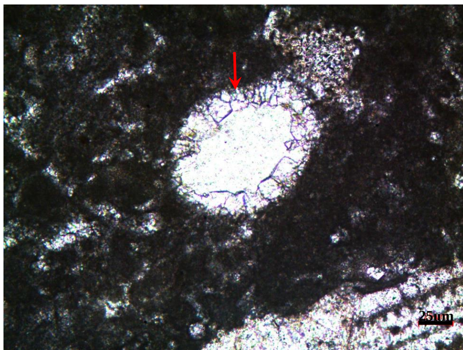
Figure 125. Isopachous equant rim cement formed in the pore space of the skeletal fragment from the thin section at 1650 m of the K-11 well
