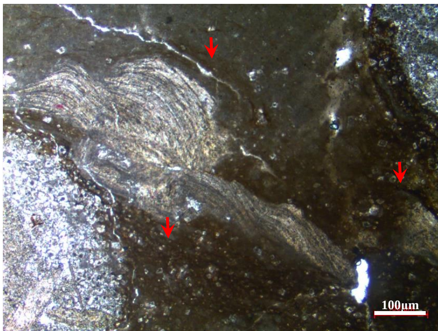
Figure 138. Stylolites associated with dolomitization from the thin section at 1776.86 m of the K-11 well
