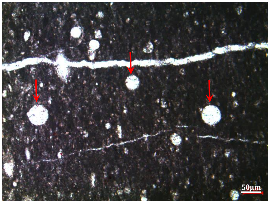
Figure 129. Calcite replaces silica in radiolaria-bearing mudstone microfacies from the thin section at 1697.42 m of the K-11 well
