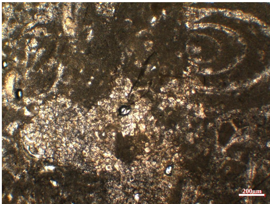
Figure 112. Partially dolomitized recrystallized skeletal fragments and pore spaces, at 1650.69 m of the K-11 well, plane polar light
