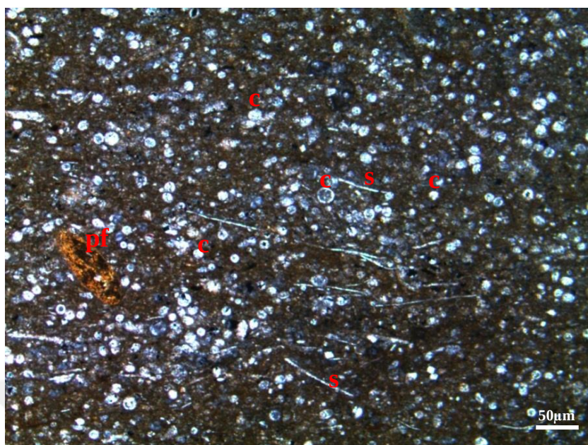
Figure 79. Skeletal calcisphaerulid-bearing wackestone to packstone microfacies from the thin section at 1719.91 m of the K-11 well [pf: phosphate fragments; s: skeletal fragments (thin walled mollusk (pelecypod)); c: calcisphaerulids ( Pithonella spherica )]
