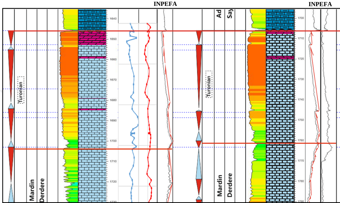
Figure 95. Number of sequences and sequence boundaries of K-11 well (on the left) and K-8 well (on the right) on the scale of 1/500 defined in Turonian time interval which is correlated with global cycle chart of Haq (2014) (Red lines shows the top of Turonian (top of the Derdere Formation) and Cenomanian-Turonian boundary and red arrows show the interpreted shifts on INPEFA log)
