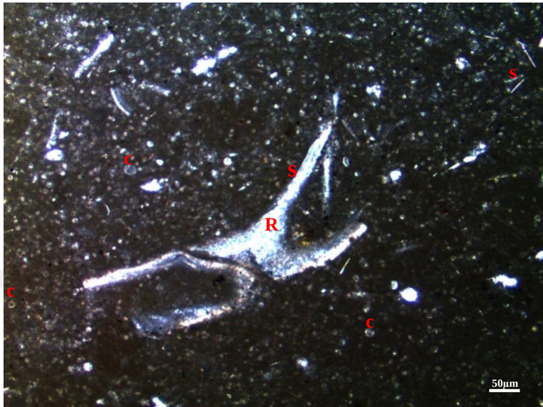
Figure 64. Calcisphaerulid-bearing skeletal wackestone to packstone microfacies from the thin section at 1720.81 m of the K-11 well [c: calcisphaerulid ( Pithonella spherica ); s: skeletal fragments; R: recrystallization]
