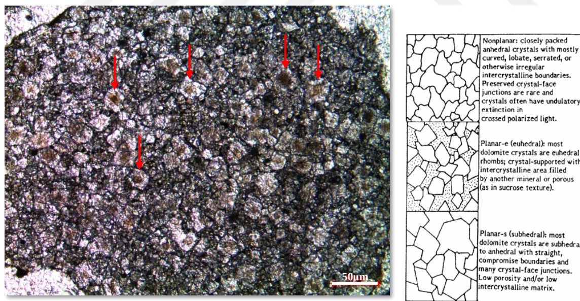
Figure 107. Planar-s cloudy core-clear rimmed dolomite with low porosity and low intercrystalline matrix showing zoning from the thin section at 1872 m of the K-8 well [Dolomite rock texture classification of Gregg and Sibley (1984) is on the right.]
