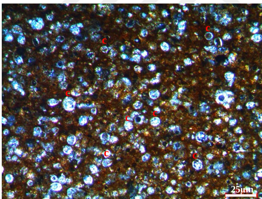
Figure 74. Calcisphaerulid-bearing wackestone to packstone microfacies from the thin section at 1718 m of the K-11 well (c: calcisphaerulid ( Pithonella spherica ))
