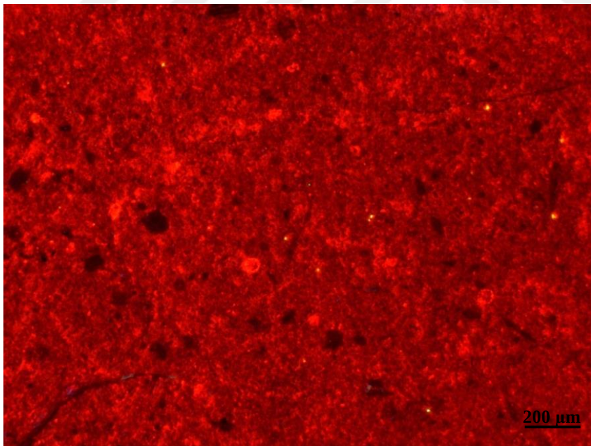
Figure 8. Light microscope based cathodoluminescence photomicrograph of calcisphaerulid-bearing wackestone facies and microfractures and micro pores of K-2 well
