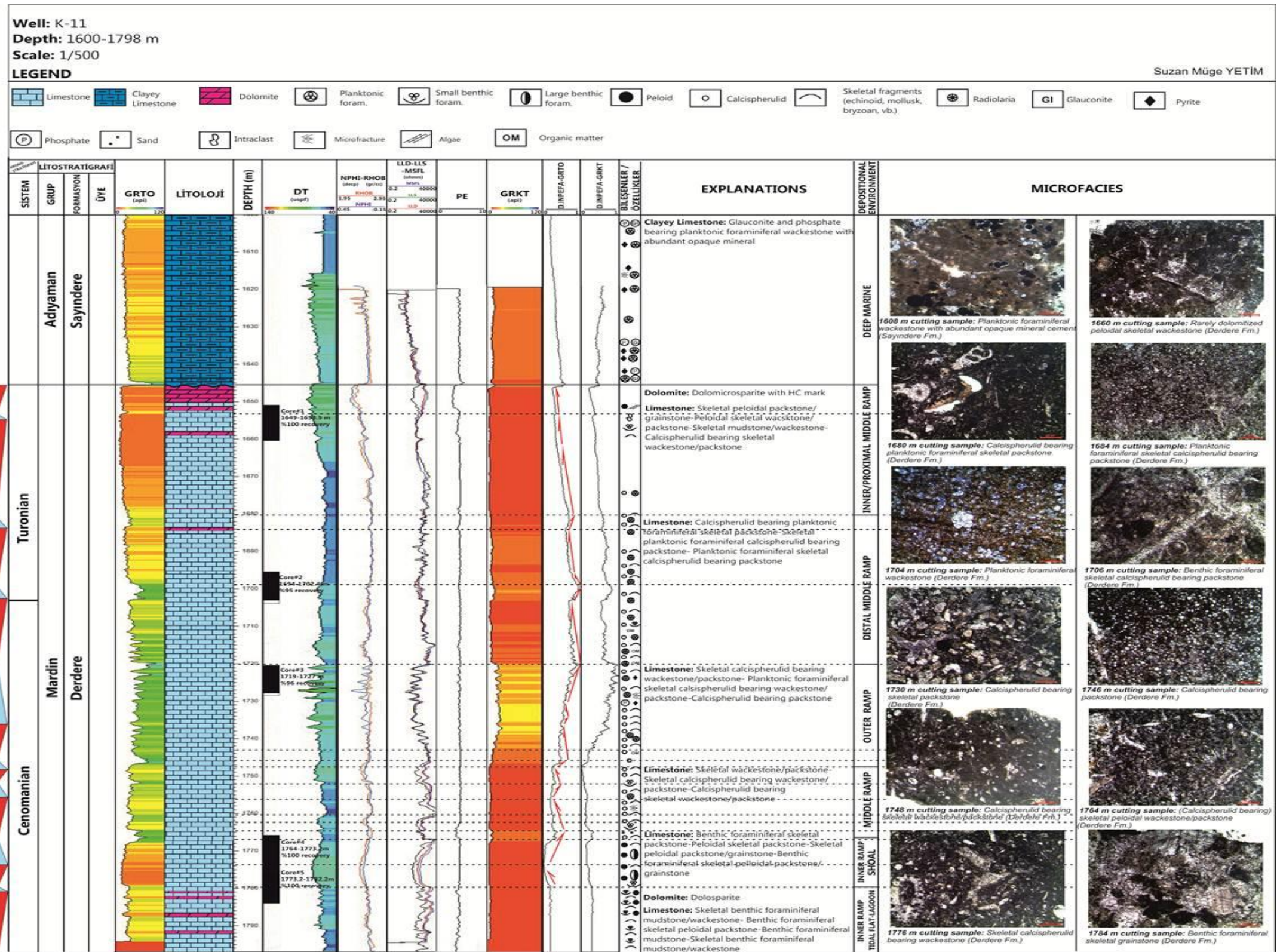
Figure 86. Sedimentological log and sequences of the Derdere Formation in the K-11 well (1600-1798m)
