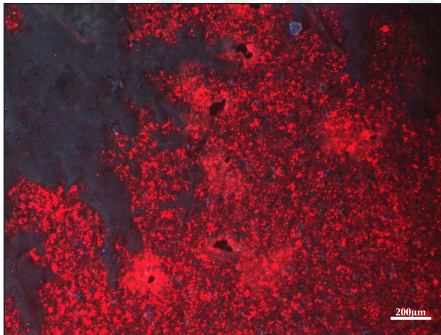
Figure 110. Dolomicrosparite and pore spaces of the K-11 well, plane polar light
