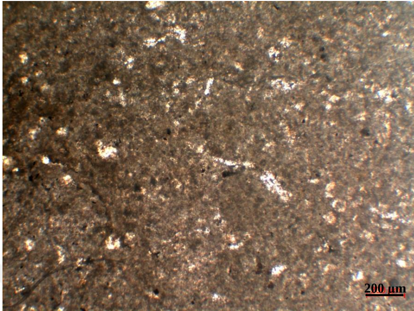
Figure 7. Plane polarized light microscopy photomicrograph of calcisphaerulid-bearing wackestone facies and microfractures and micro pores of K-2 well
