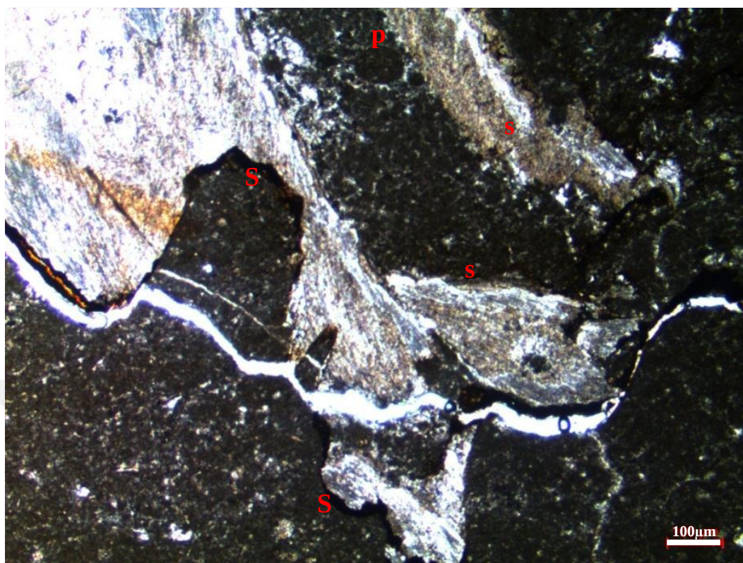
Figure 52. Peloidal skeletal wackestone microfacies from the thin section samples of 1764.89 m of the K-11 well [p: peloid; s: skeletal fragments (possible rudist); S: stylolitization at around skeletal fragment]
