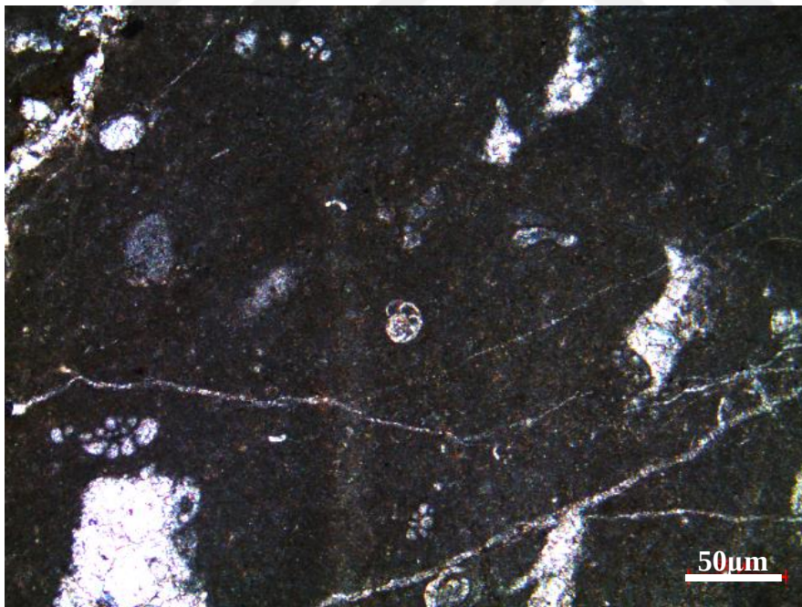
Figure 40. Fenestral fabric in benthic foraminiferal mudstone of the peritidal environment of inner ramp setting at 1778.34 m of the K-11 well
