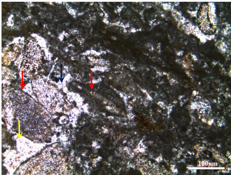
Figure 122. Micritic isopachous Mg calcite and sparry calcite cement as interparticle pore filling from the thin section at 1771.4 m of the K-11 well (Red arrows show the micritic isopachous cement. Yellow arrows show sparry calcite cement.)
