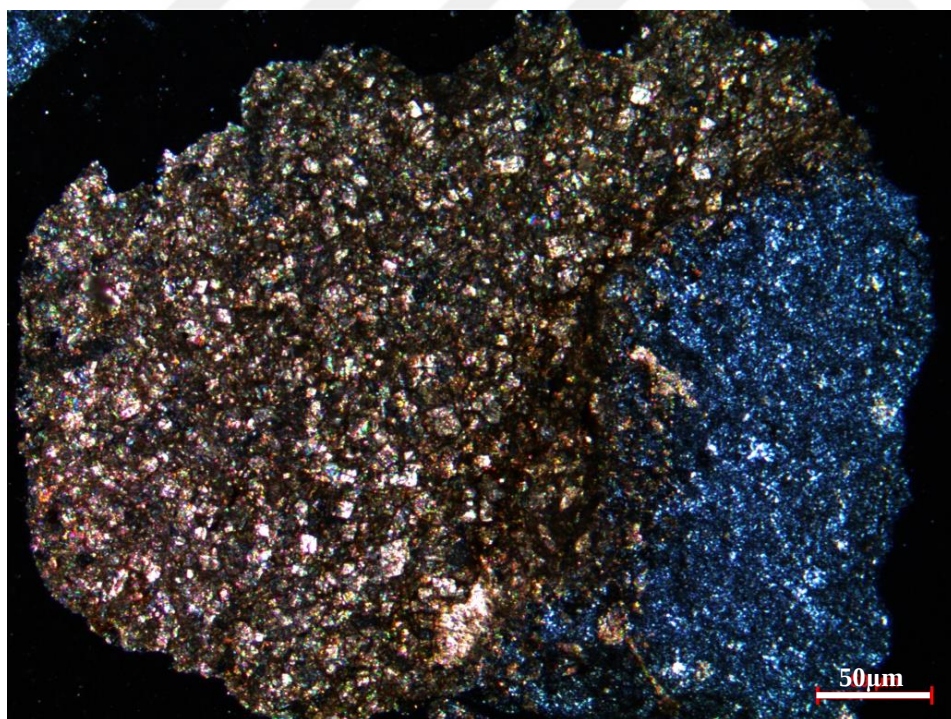
Figure 134. Silica replacement of dolosparite from the thin section at 1866 m of the K-8 well, cross polar light
