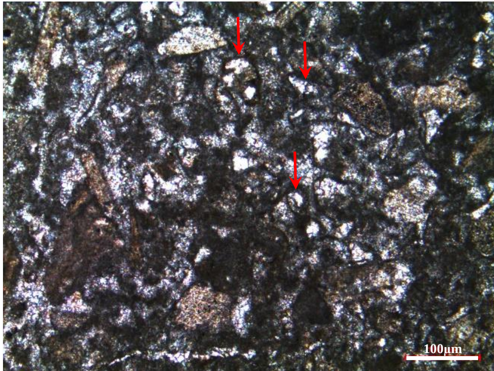
Figure 121. Micritic isopachous Mg calcite and sparry calcite cement as interparticle pore filling from the thin section at 1770.8 m of the K-11 well (Red arrows show the micritic isopachous cement at around the skeletal grains.)
