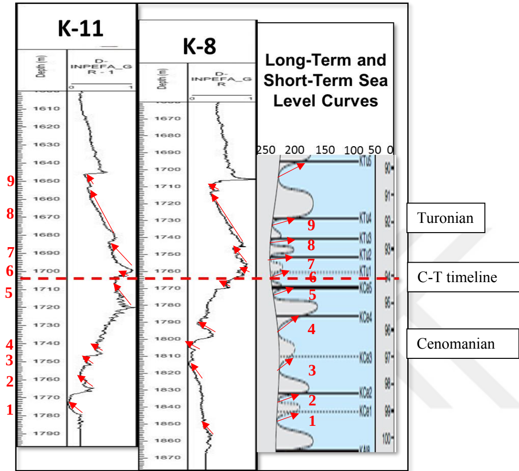
Figure 94. Raw INPEFA log data of K-11(on the left), K-8 wells (on the right) on the scale of 1/1000 and long term and short term sea level curves belongs to the Cenomanian-Turonian time interval of Haq (2014) [Red line shows Cenomanian-Turonian boundary, red arrows show the locations of sequence boundaries on the INPEFA logs and sea-level curve of Haq (2014), and red numbers show the number of the sequences defined in the wells and correlated sequences on the sea-level curve of Haq (2014)]
