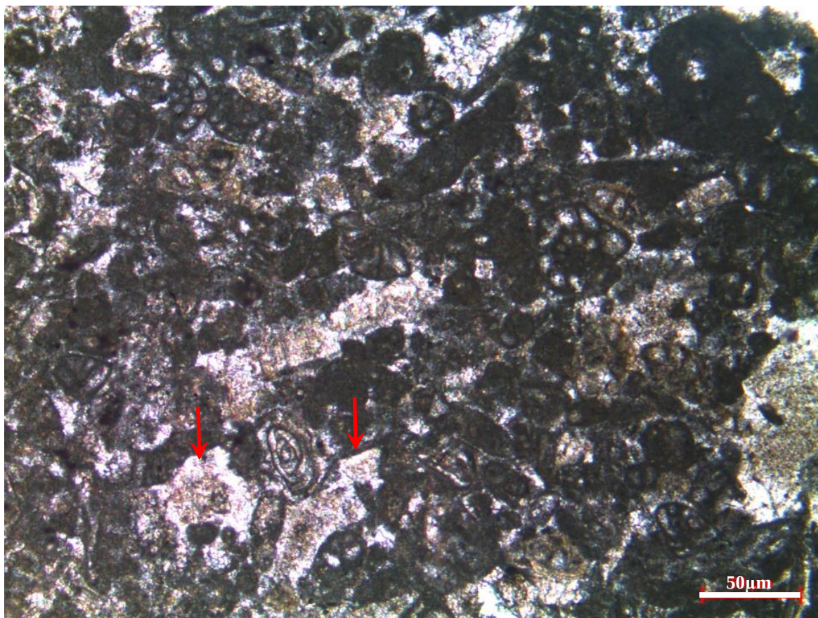
Figure 126. Syntaxial overgrowth of echinoderm particles in the thin section sample at 1808 m of the K-8 well
