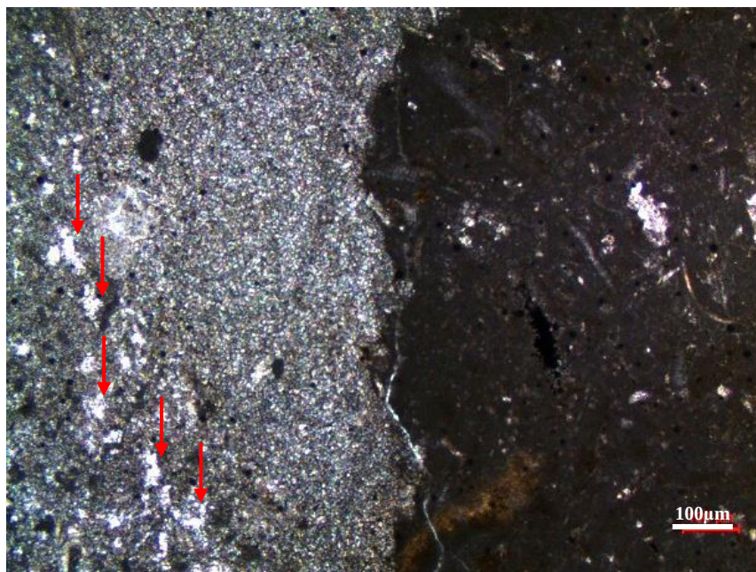
Figure 103. Partially dolomitized skeletal, peloidal packstone to grainstone microfacies from the thin section at 1649.35 m of the K-11 well (Note that the original fabric of peloidal facies is partially preserved. Red arrows show pore spaces.)
