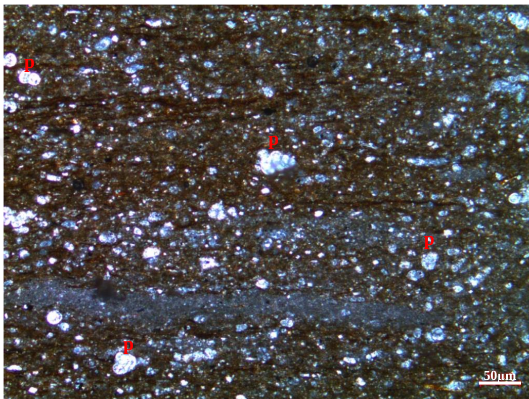
Figure 70. Planktonic foraminiferal wackestone microfacies from the thin section at the K-11 well (p: planktonic foraminifer)
