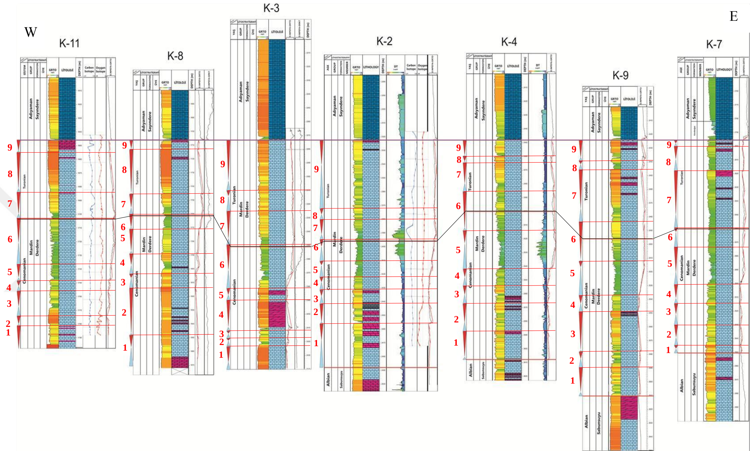
Figure 90. 3 rd order sequence correlation between the wells of the study area from west to east (K-11, K-8, K-3, K-2, K-4, K-9, and K-7) (Red lines show sequence boundaries, black line shows C-T boundary and blue boundary shows the boundary between Derdere and Sayindere formations)
