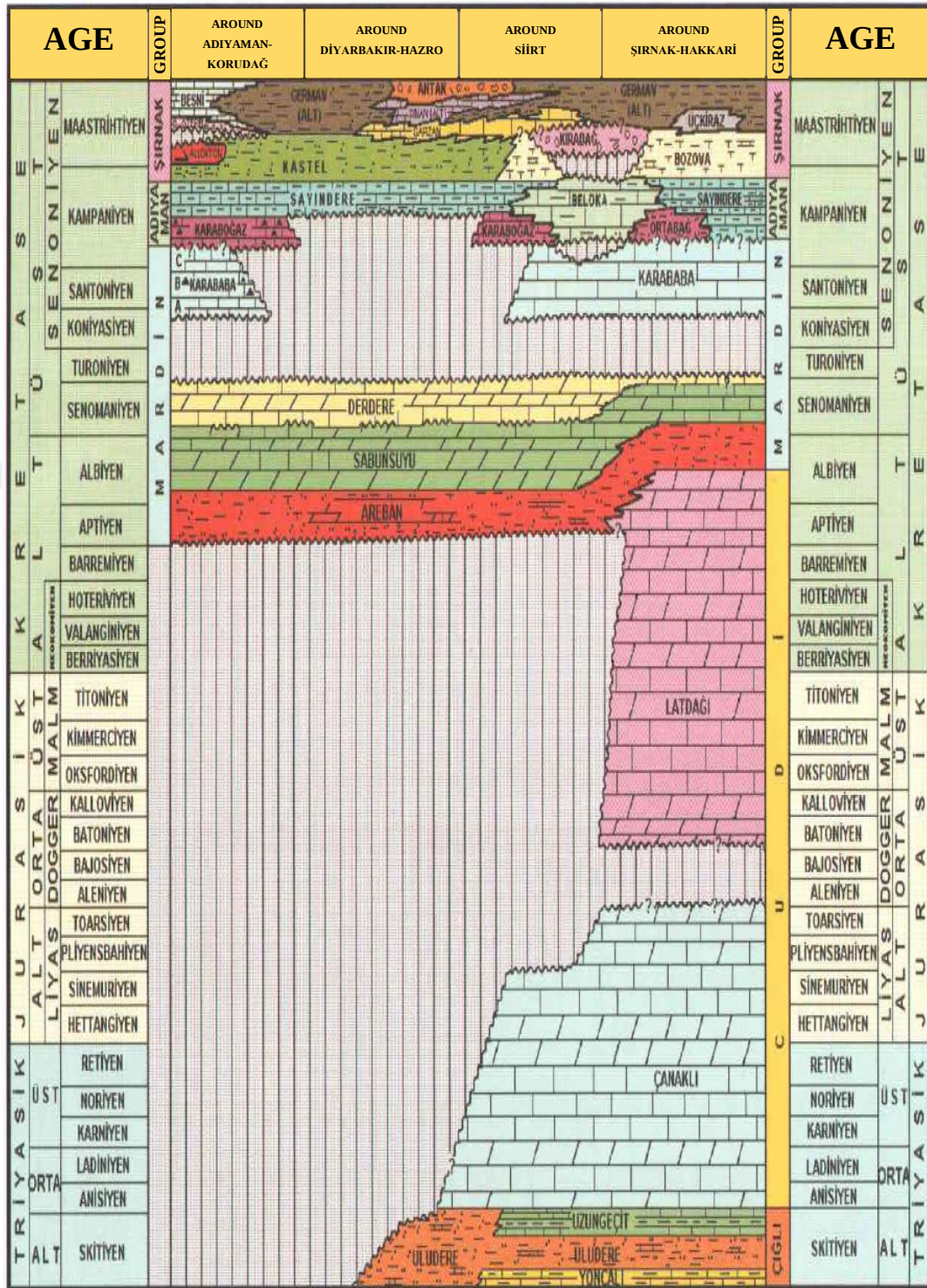
Figure 18. Stratigraphy and correlation of Mesosoic aged autochthonous units at the northern part of Southeastern Turkey (modified after Yılmaz and Duran, 1997)
