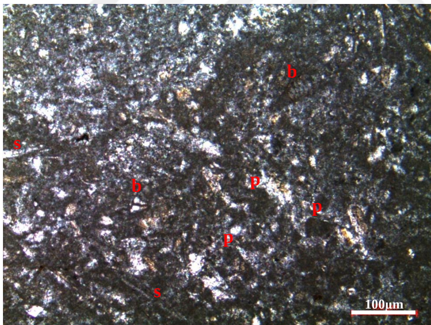
Figure 51. Peloidal skeletal packstone microfacies from the thin section at 1765.84 m of the K-11 well [p: peloid; s: skeletal fragments; b: benthic foraminifera (rare)]
