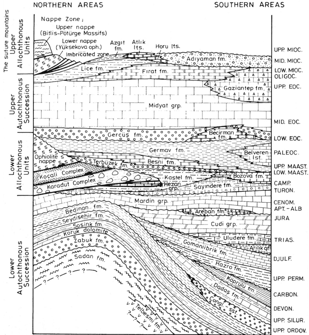
Figure 15. Stratigraphic section of the Arabian platform in southeast Anatolia (Yalçın 1976; Yılmaz 1993; Okay, 2008)
