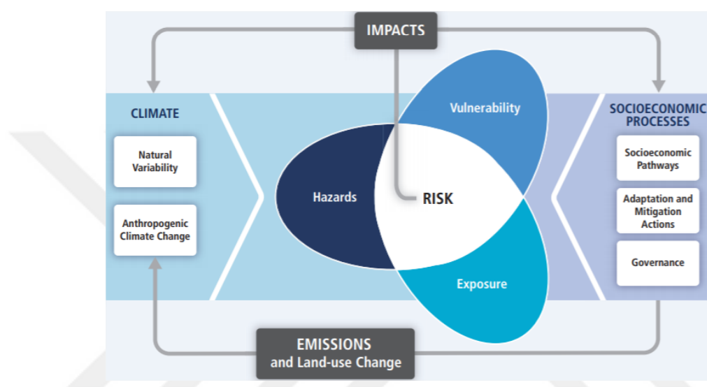
Figure 5: Risk-Based Framework in the Fifth Assessment Report (AR5) of IPCC in 2014
