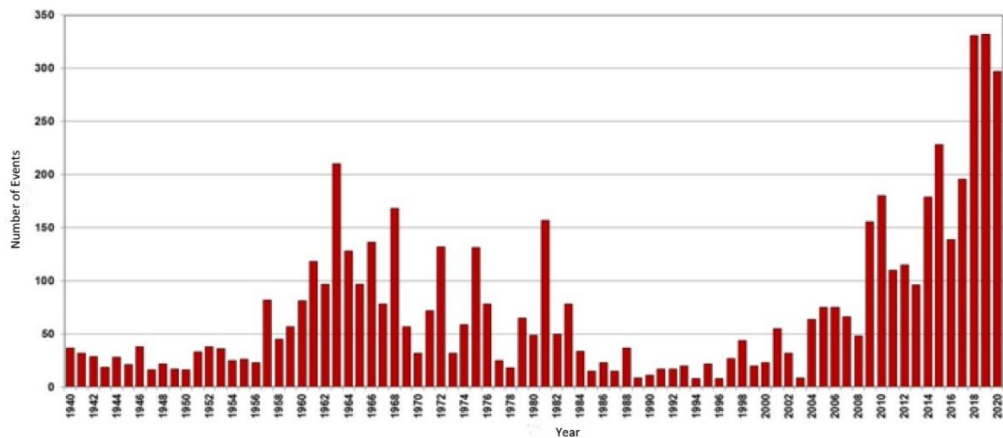
Figure 30: Number of Flood Events, 1940-2020 (Turkish State Meteorological Service, 2021)
