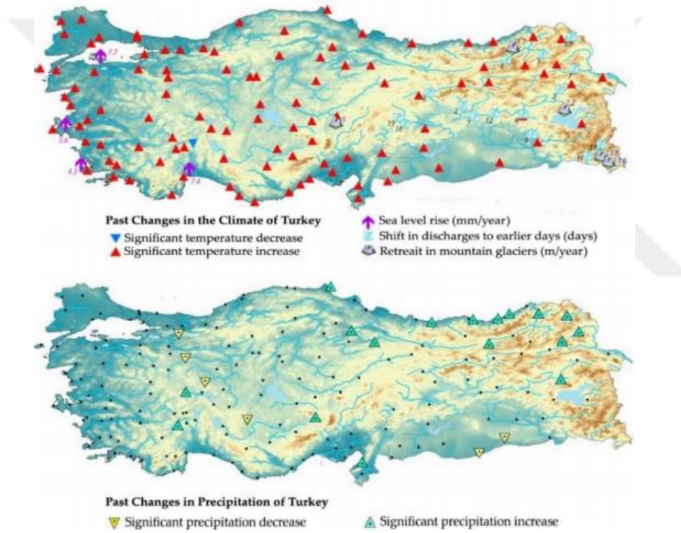
Figure 7: Past Changes in the Climate of Turkey (Şen, 2013)
