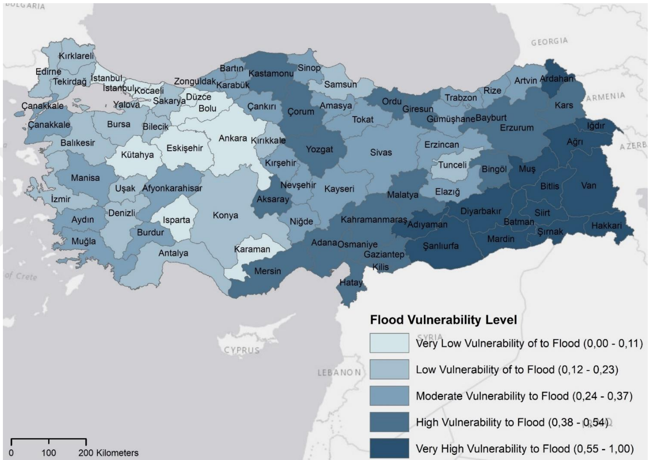
Figure 85: Flood Vulnerability Level of the Provinces in Turkey
