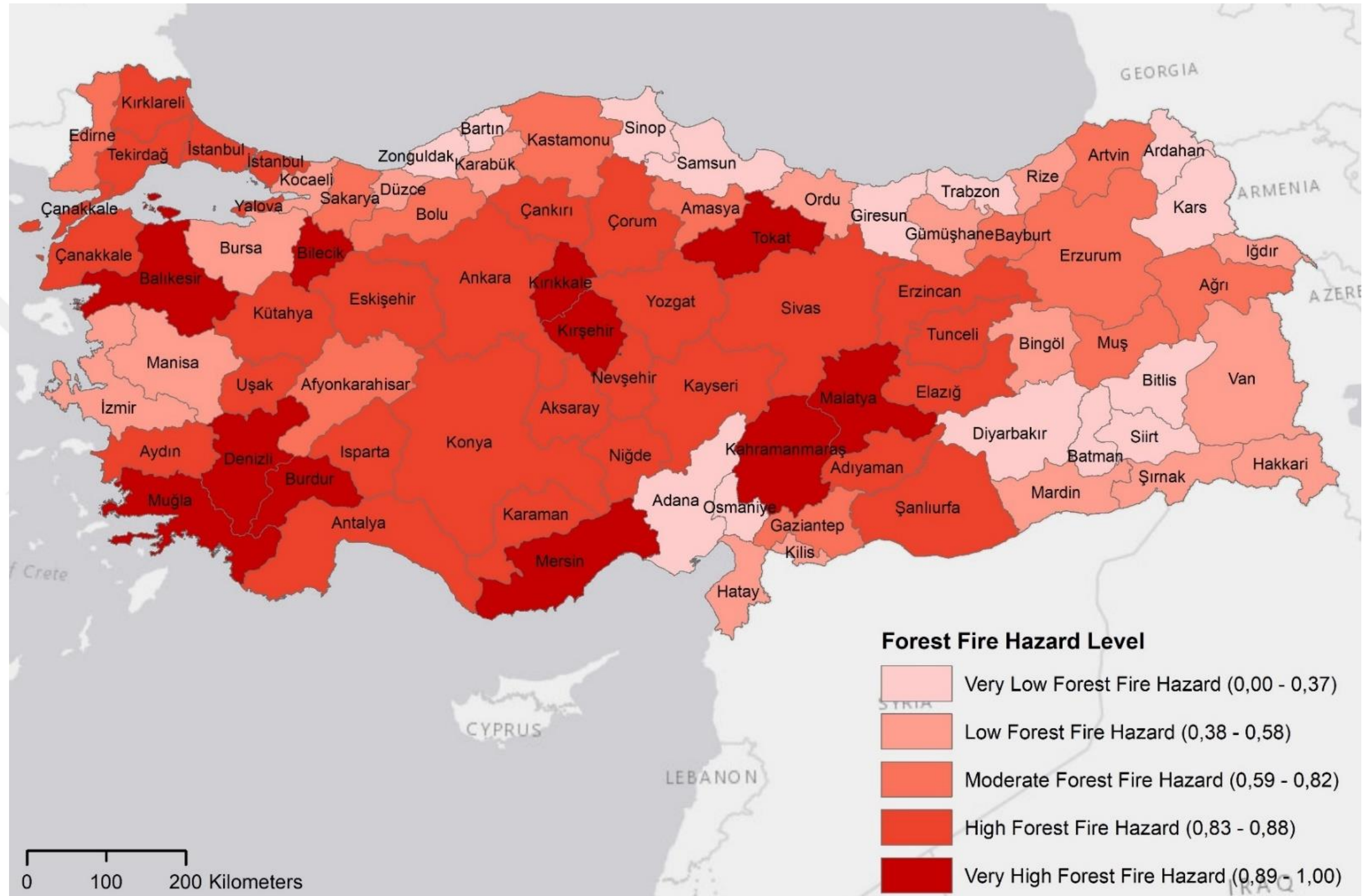
Figure 69: Forest Fire Hazard Level of the Provinces in Turkey
