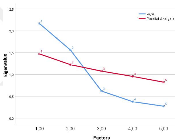
Figure 59: Scree Plot of Parallel Analysis
