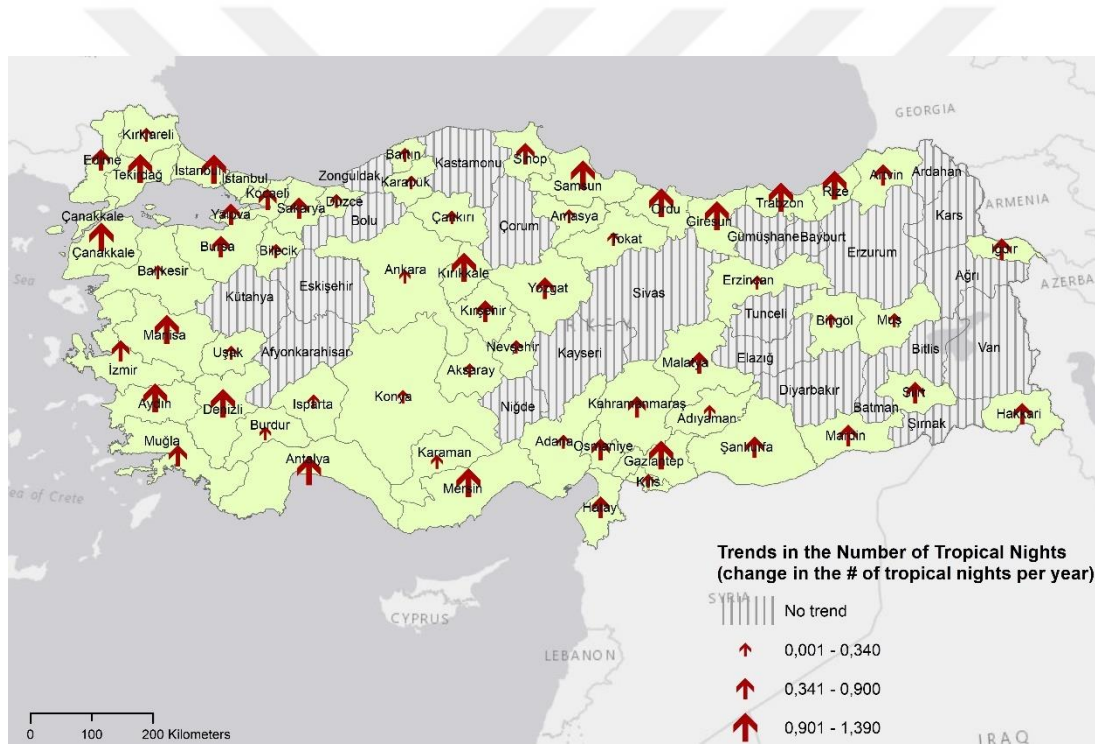
Figure 46: Mann-Kendall Test and Sen's Slope Estimator Results of the Number of Tropical Nights per year ( T_{min} > 20^{\circ}\text{C} ) for 81 provinces for the time period 1971-2018 (natural breaks data classification) (Prepared by the author)
