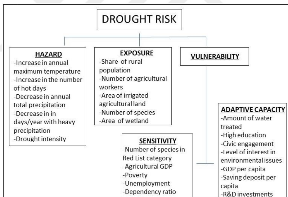
Figure 58: Indicators Scheme for Drought Risk
