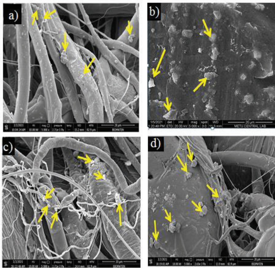
Figure 3.14 SEM images of scaffolds before and after 1 st day of SBF immersion. a) PCL, b) PCL-Zn HA, c) PCL-Zn HA-BNMF, d) PCL-BNMF (Scale bar: 20 \mu m). (Yellow arrows: CaP deposition on the fibers)
