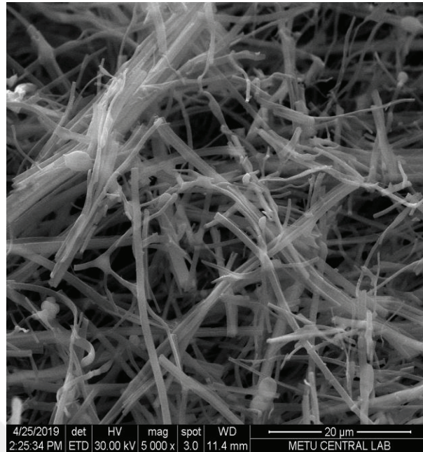
Figure 3.7 SEM image of BNNF with scale bar of 20 μm. Fiber morphology was observed after freeze drying.
