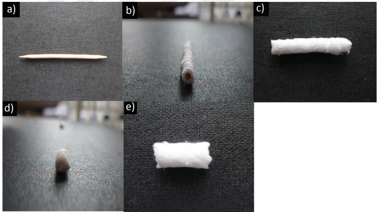
Figure 2.1 Preparation of the scaffolds for the compression test, a) stick with 0.5 mm diameter, b) front image after wrapping fibers around stick, c) top image after wrapping around stick, d) after removing stick from fibers, e) cutting of cylindrical shaped of fibers into small pieces with 4 mm diameters and 8 mm length
