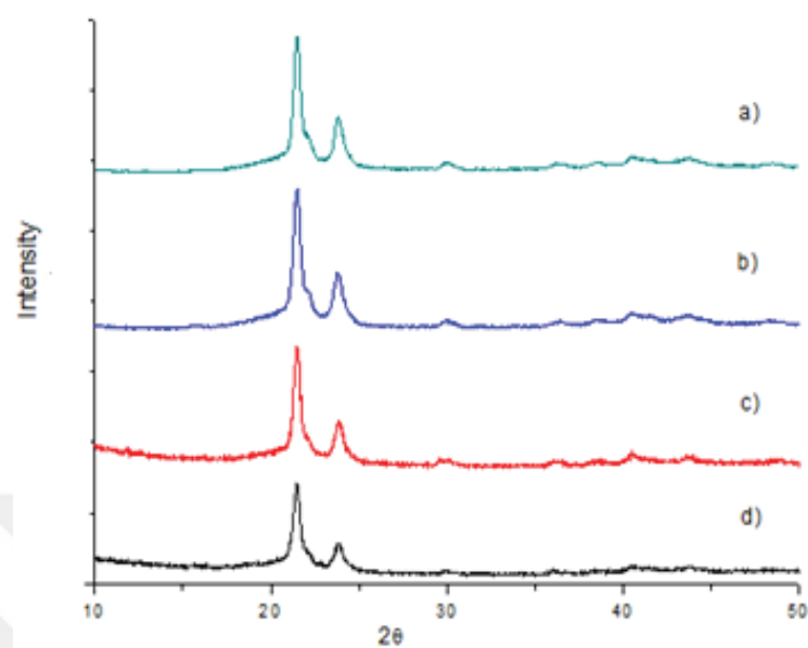
Figure 3.17 XRD analysis of PCL scaffolds after SBF immersion at 1 st day: a) PCL-BNNF, b) PCL-Zn HA-BNNF, c) PCL-Zn HA, d) PCL
