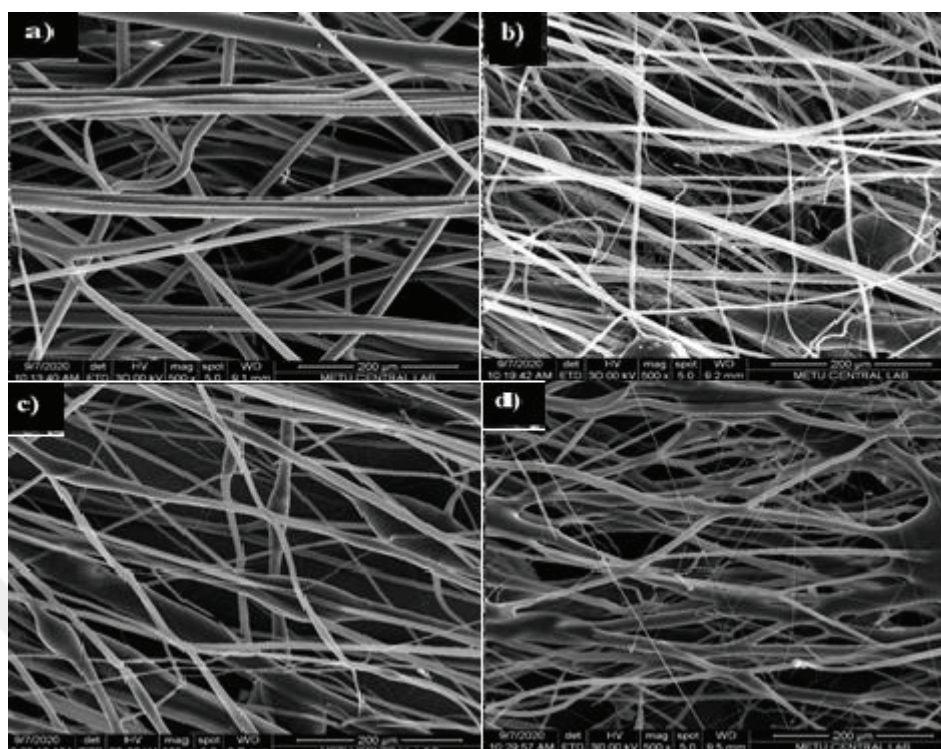
Figure 3.9 SEM images of a) PCL, b) PCL- Zn HA, c) PCL-Zn HA-BNNF, d) PCL-BNNF scaffolds (Scale bar: 200 µm).
